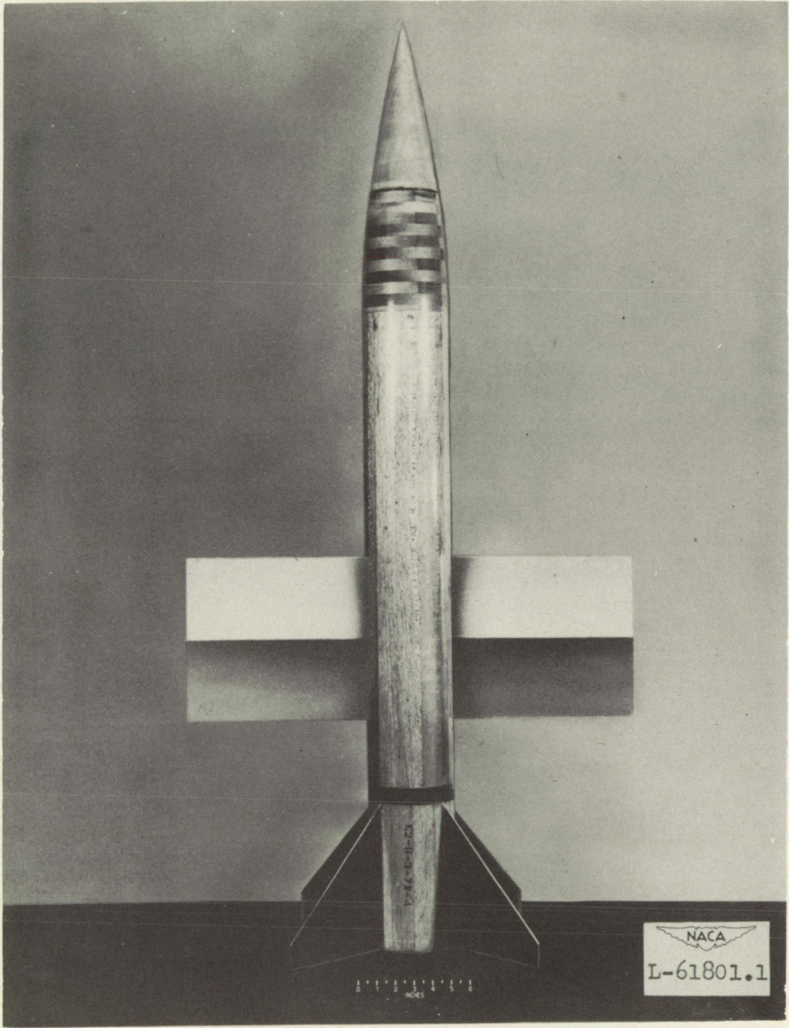
Figure 2.- Photograph showing plan form of diamond-wing-section vehicle.
