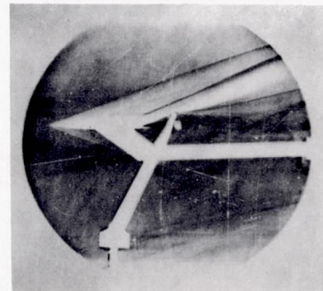
(g) Elapsed time, 28 milliseconds; flap angle, -19^{\circ} .
