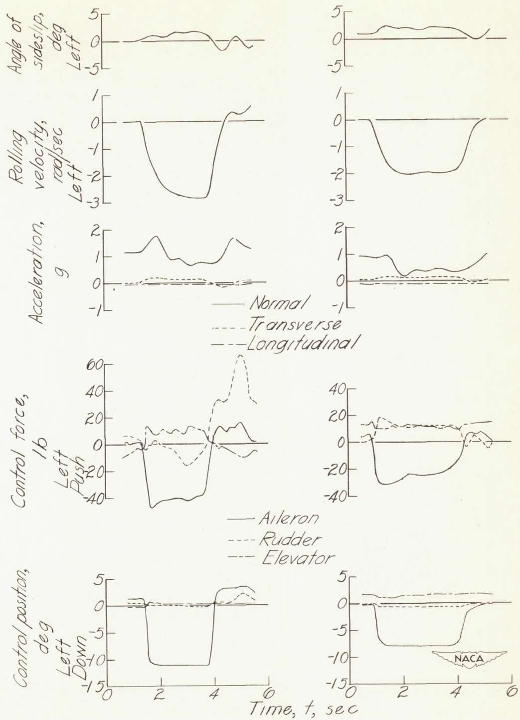
(c) M=0.82 ; H=24,000 ft
