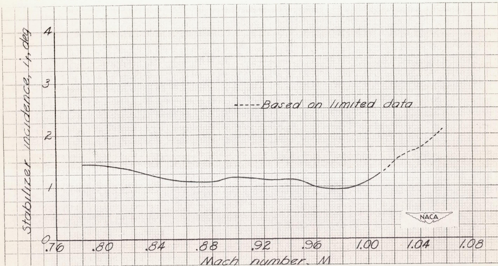
Figure 6.- Variation of stabilizer incidence required for trim with Mach number. Elevator angle, 0^\circ ; normal-force coefficient, 0.3; pressure altitude, 40,000 feet.
