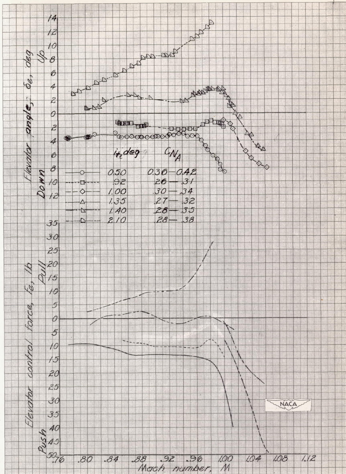
Figure 2.- Variation of elevator angle and control force with Mach number at various stabilizer settings. X-1 airplane; pressure altitude, about 40,000 feet.
