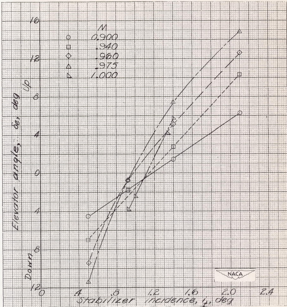
Figure 4.- Effect of Mach number on variation of elevator angle with stabilizer incidence at a normal-force coefficient of 0.3.
