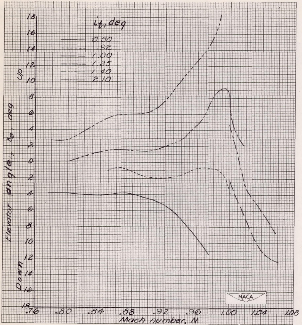
Figure 3.- Variation of elevator angle with Mach number for various stabilizer settings at a normal-force coefficient of 0.3.
