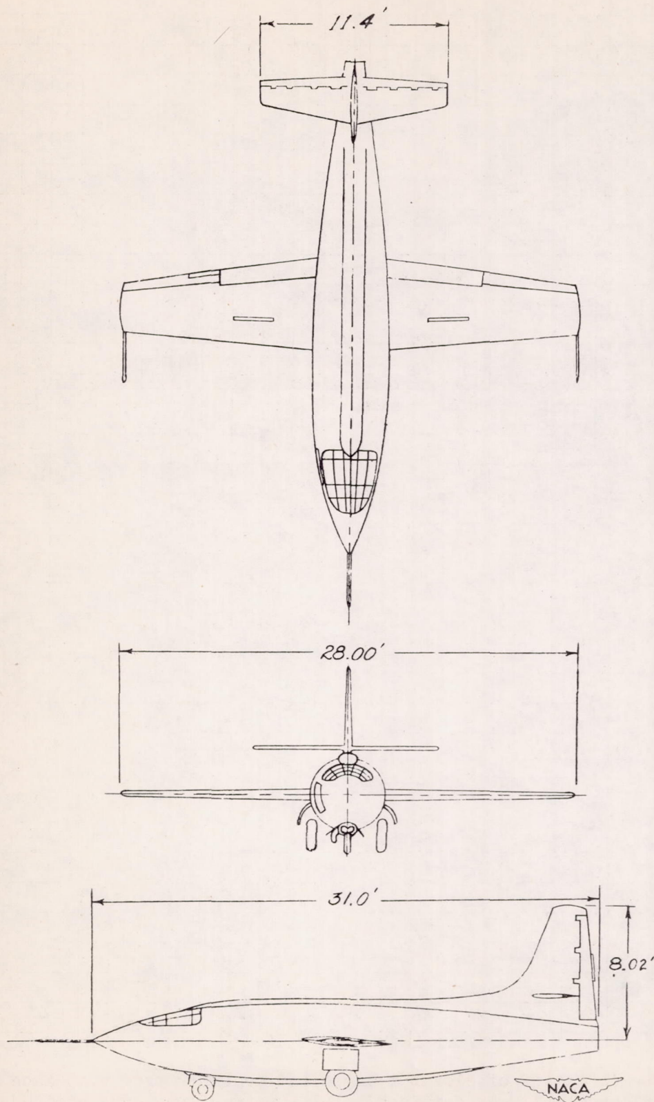
Figure 1.- Three-view sketch of X-1 research airplane.
