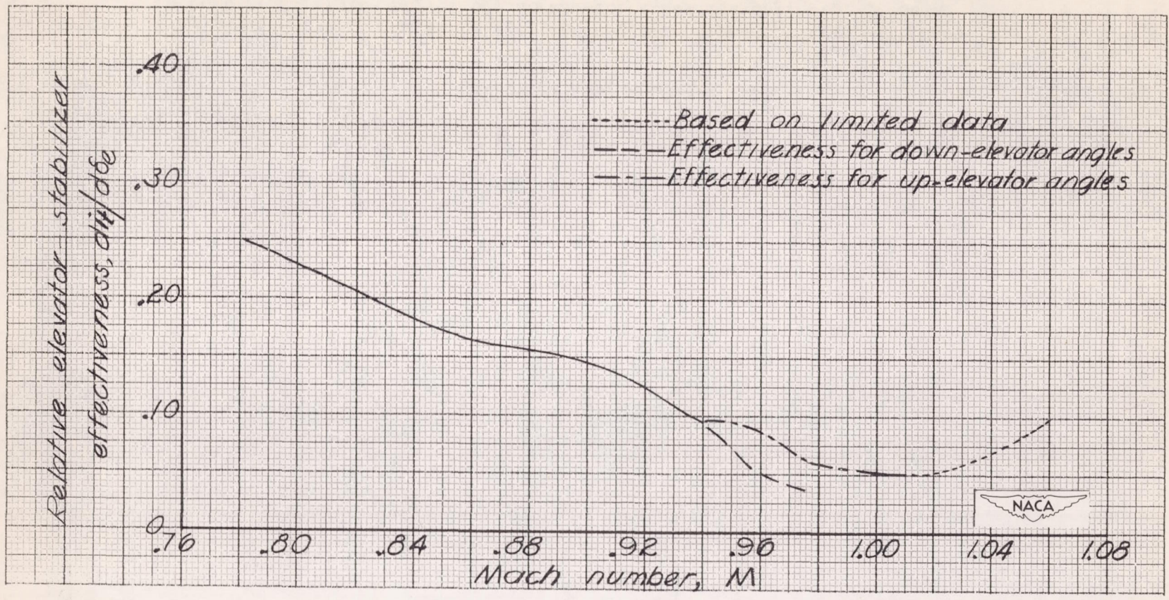
Figure 5.- Variation of relative elevator-stabilizer effectiveness with Mach number for the X-1 airplane at a normal-force coefficient of 0.3 and an altitude of about 40,000 feet.
