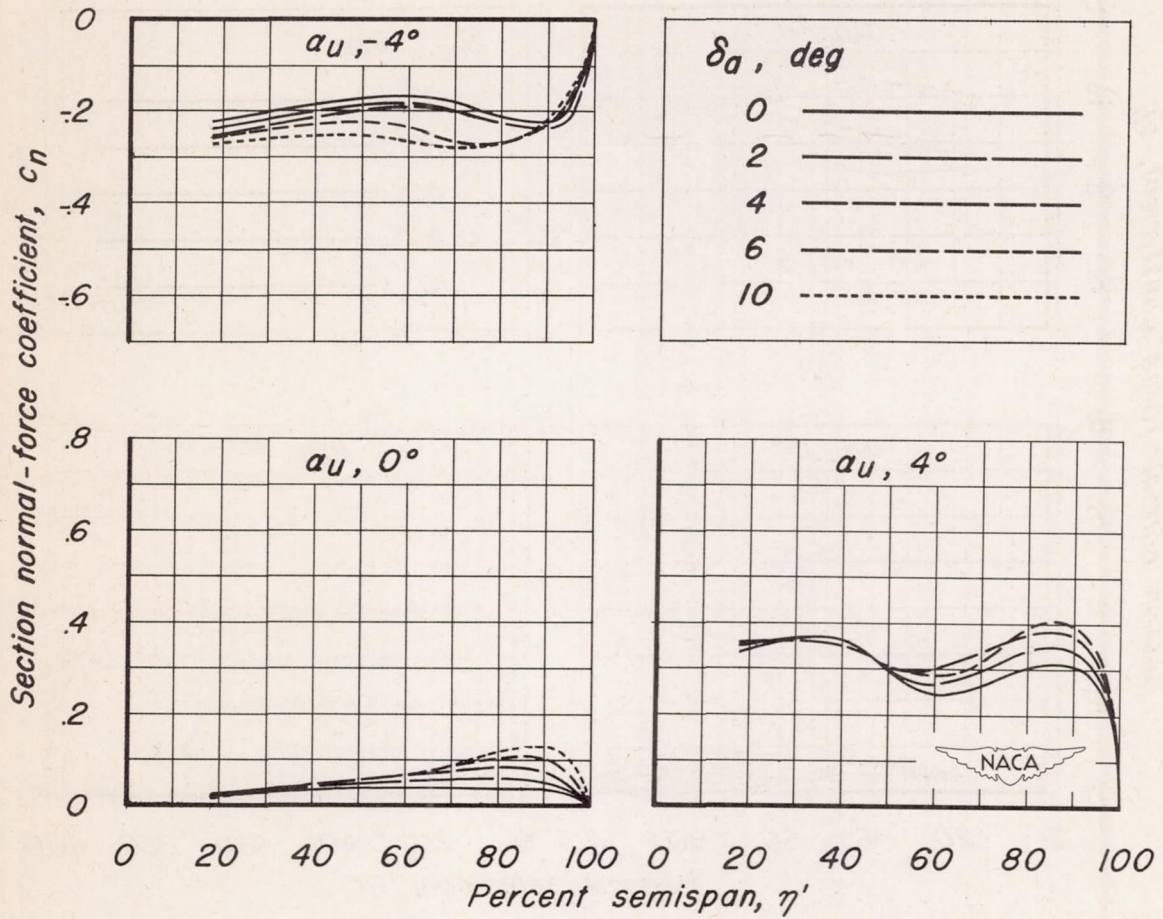
(e) M, 0.875 . Figure 5.- Continued.
