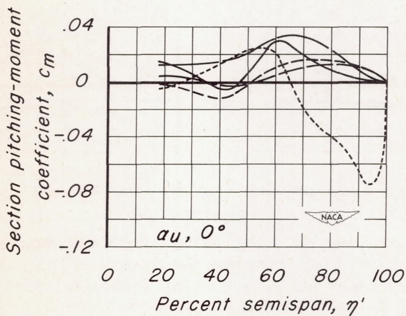
(f) M, 0.90 . Figure 7.- Concluded.
