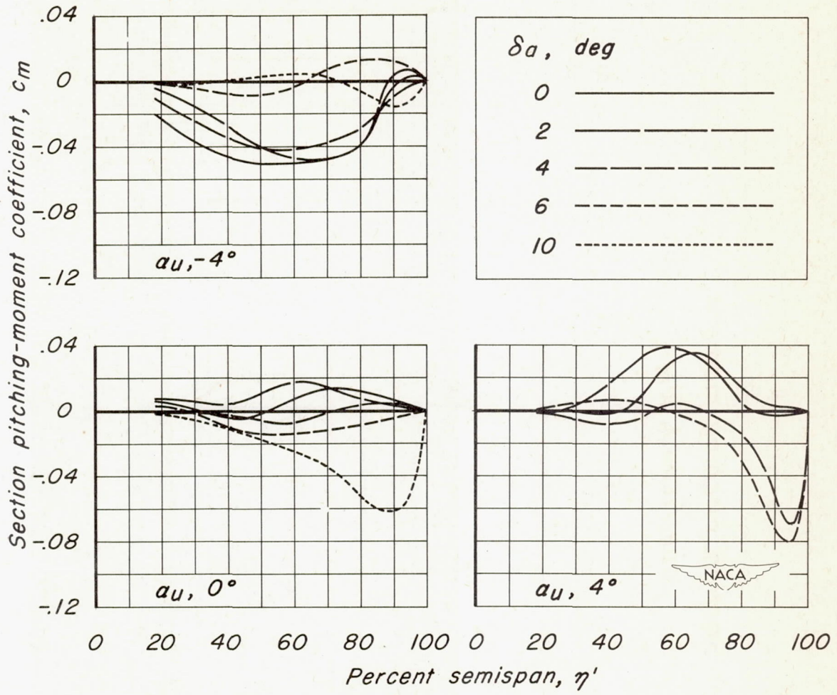
(e) M, 0.875 . Figure 7.-Continued.
