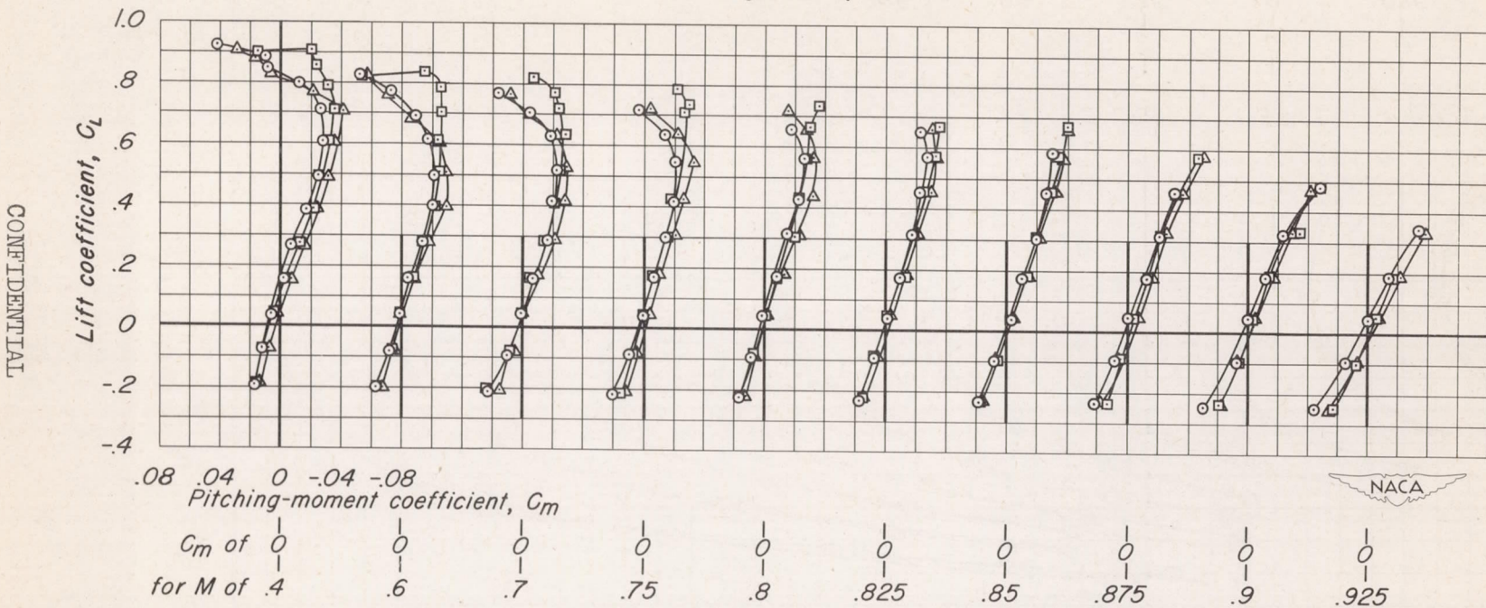
Figure 11.- Variation of the pitching-moment coefficient with lift coefficient for the wing swept back 45° with and without upper surface fences. Ailerons undeflected.
