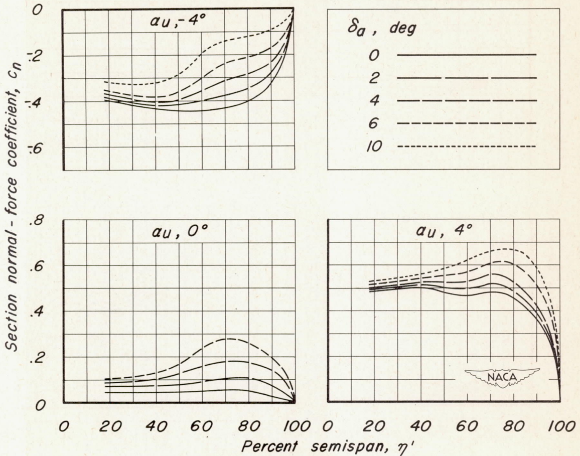
(b) M, 0.80 . Figure 5.-Continued.
