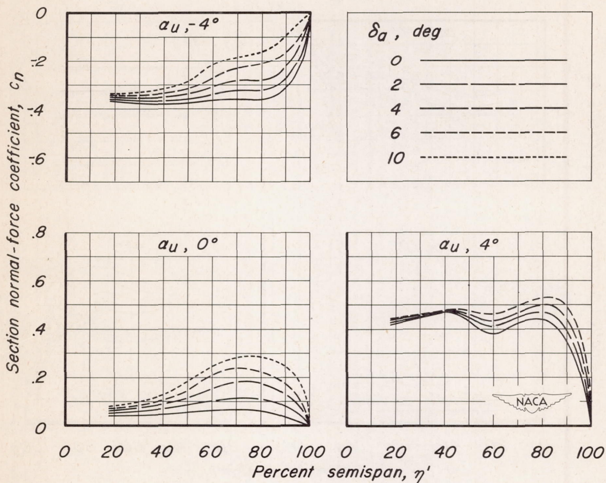
(c) M, 0.825 . Figure 5.- Continued.
