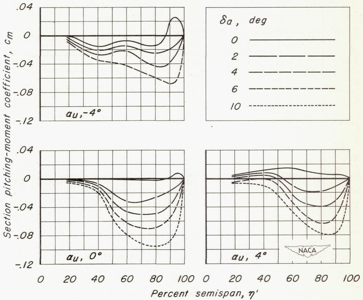
(c) M , 0.825. Figure 7.-Continued.
