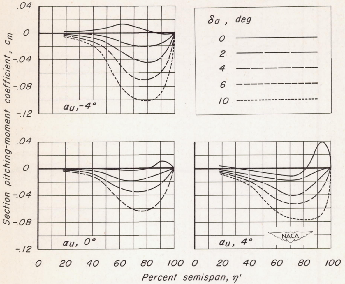
(b) M, 0.80 . Figure 7.-Continued.
