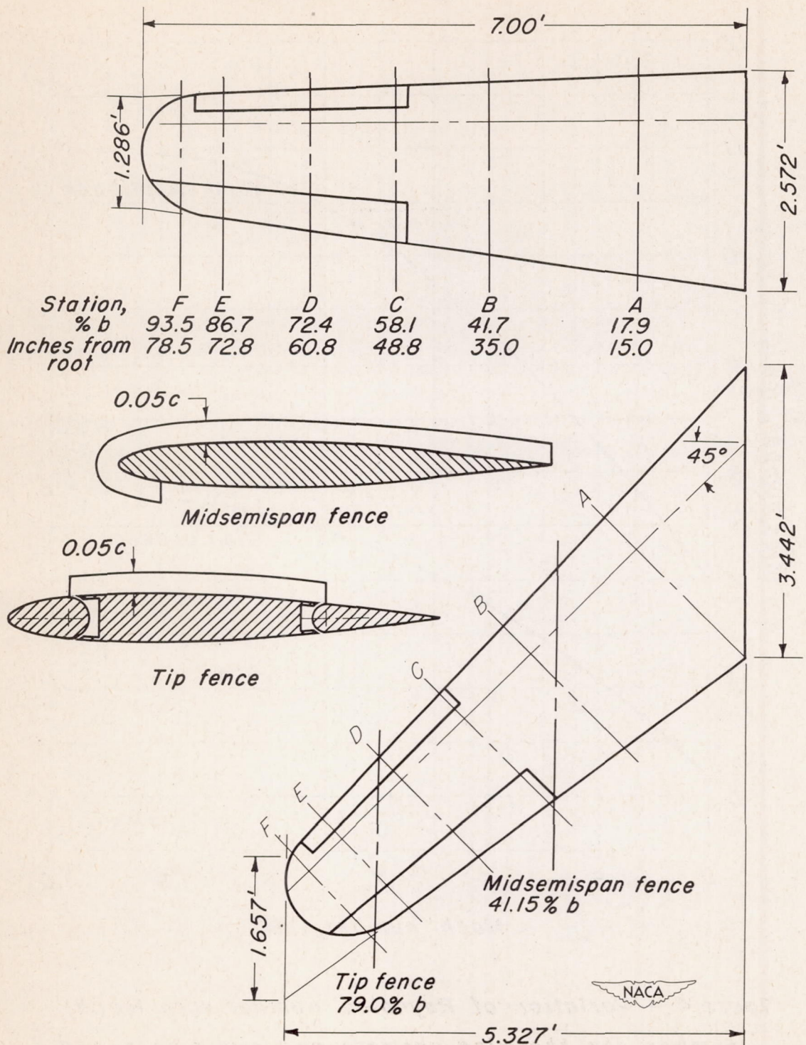
Figure 3:- Location of pressure-orifice stations and fences.
