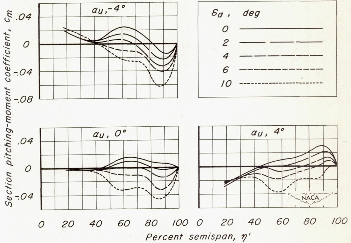
(c) M, 0.825 . Figure 8.-Continued.
