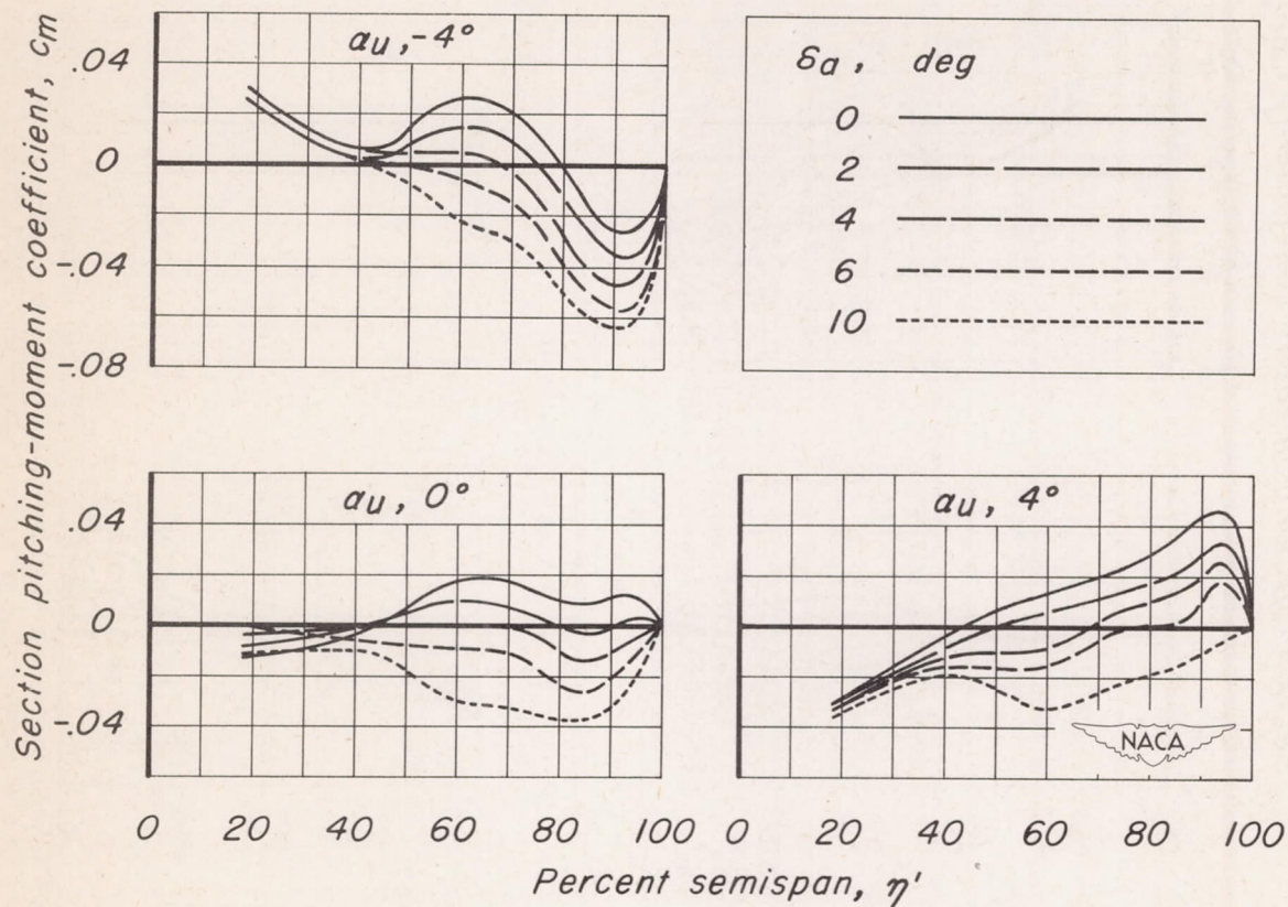
(f) M, 0.90 . Figure 8.-Continued.
