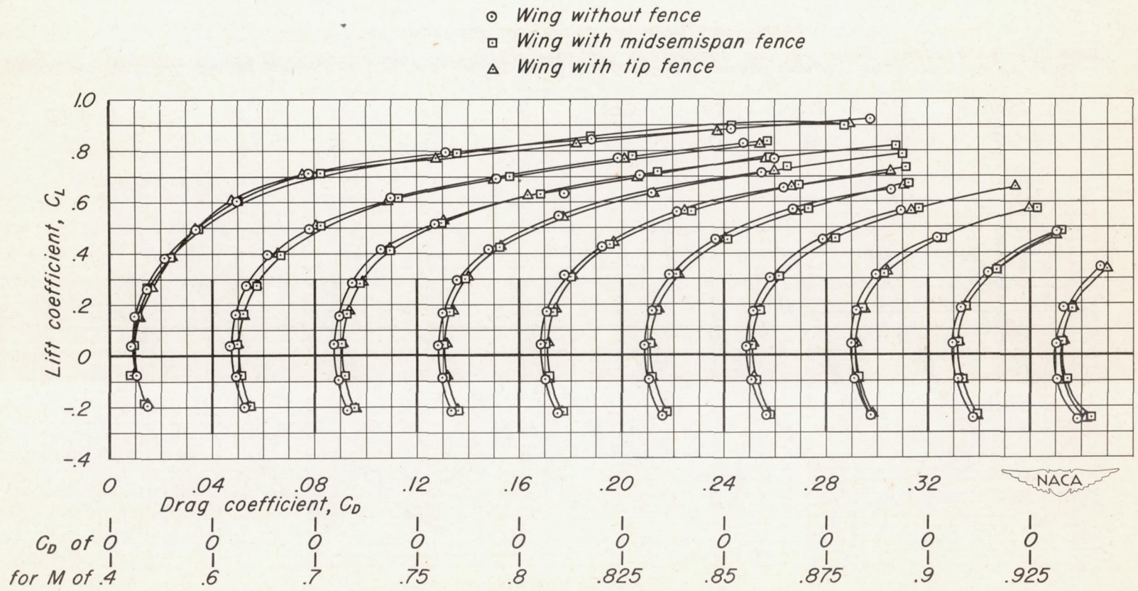
Figure 10.- Variation of the drag coefficient with lift coefficient for the wing swept back 45° with and without upper surface fences. Ailerons undeflected.
