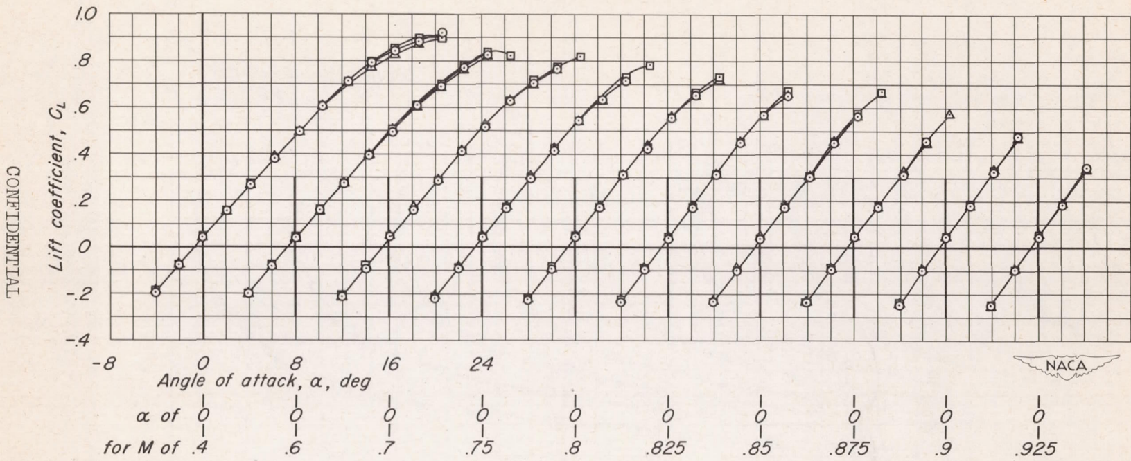
Figure 9.- Variation of the lift coefficient with angle of attack for the wing swept back 45^\circ with and without upper surface fences. Ailerons undeflected.
