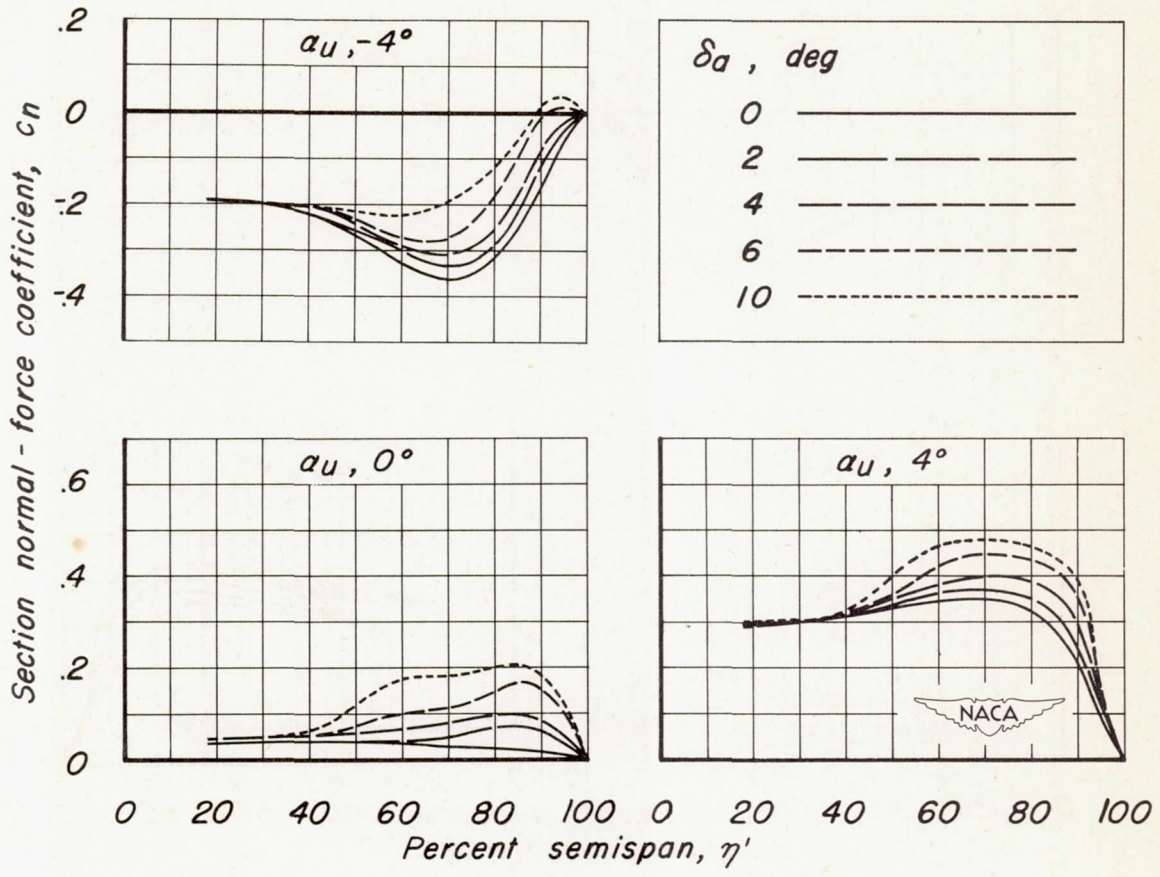
(b) M, 0.80 . Figure 6.- Continued.
