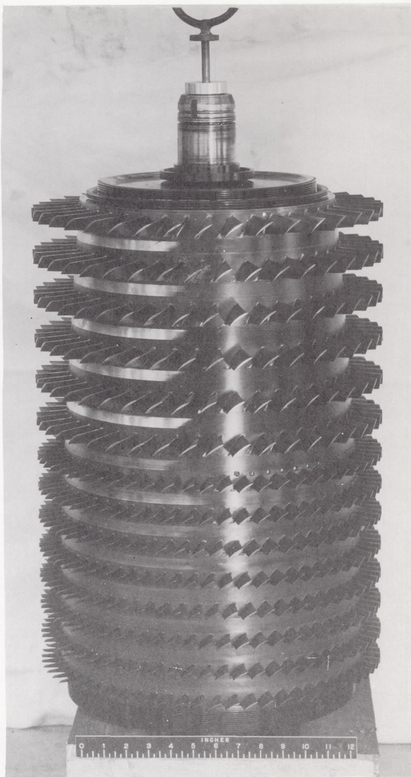
Figure 2. - Axial-flow-compressor rotor of turbine-propeller engine.
