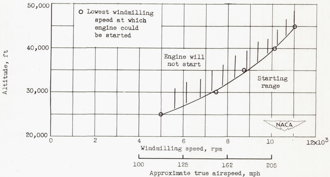
Figure 27. - Variation of minimum windmilling speed at which engine can be started with altitude.
