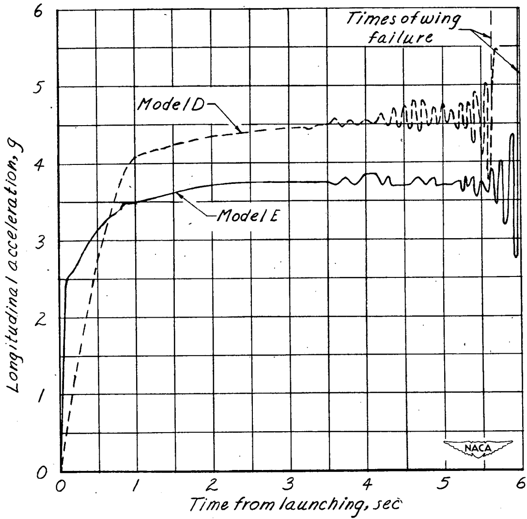
Figure 6.- Variations of longitudinal acceleration with time.
