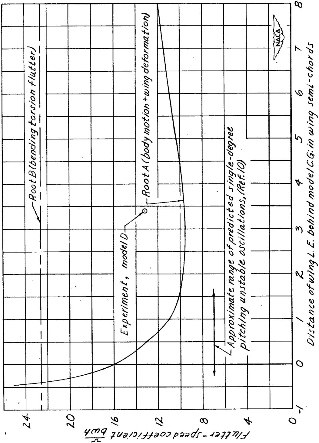
Figure 8.- Variation of flutter-speed coefficient with wing position.
