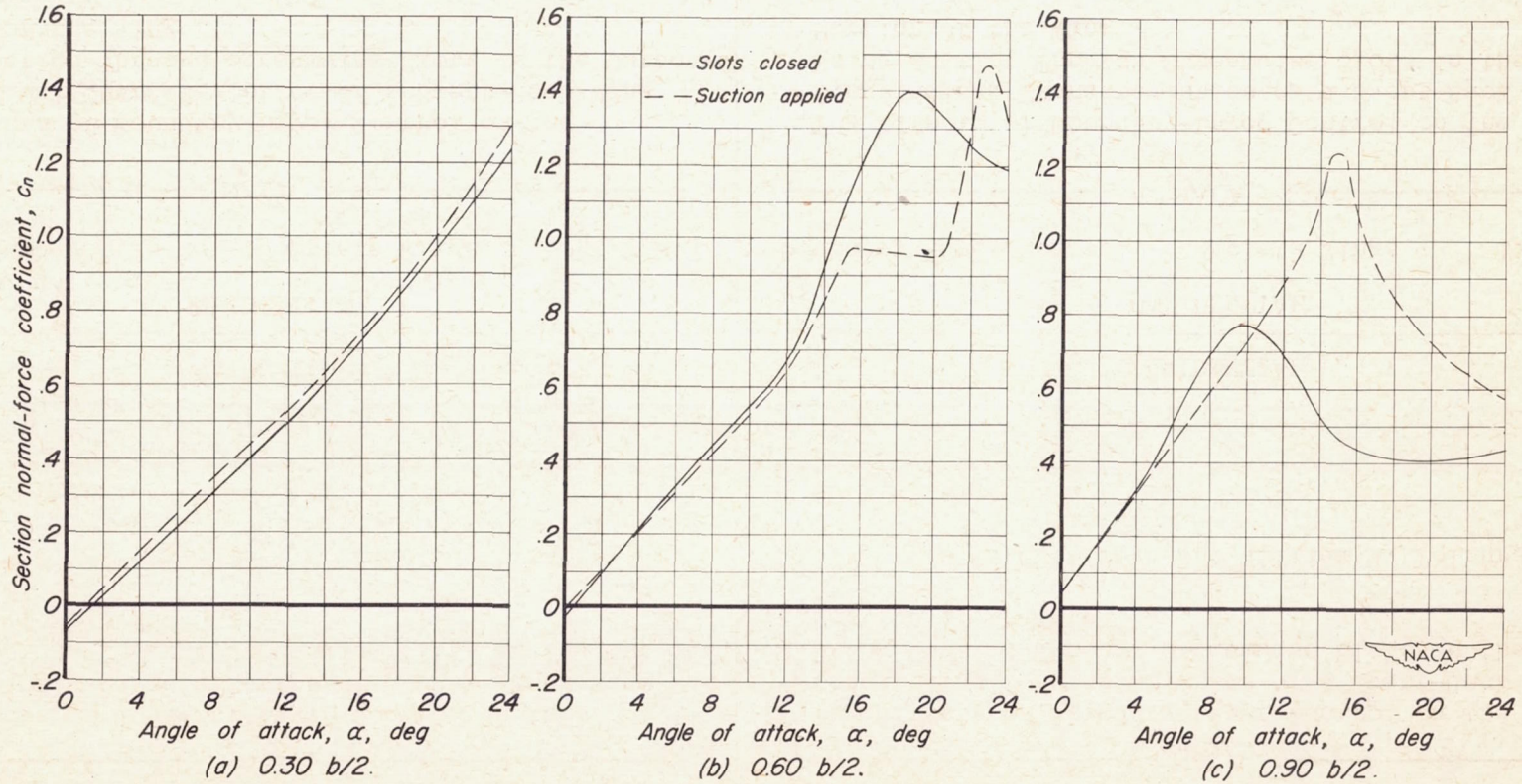
Figure 11.-Normal-force curves for various sections of the 63^\circ swept-back wing-fuselage combination with and without suction. Full-span leading-edge flaps deflected 35^\circ ; tip tanks attached; suction through slots at 0.656, 0.789, and 0.911 semispan. R, 5 \times 10^6 .
