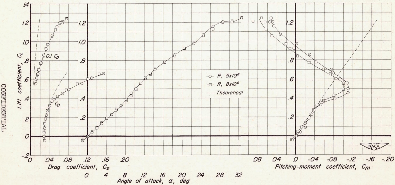
Figure 5.-The longitudinal characteristics of the 63° swept-back wing-fuselage combination.
