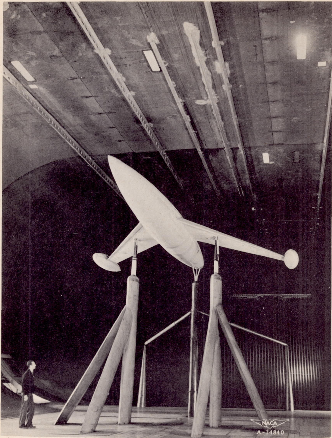
Figure 1.- The 63^\circ swept-back wing-fuselage combination in the Ames 40- by 80-foot wind tunnel.
