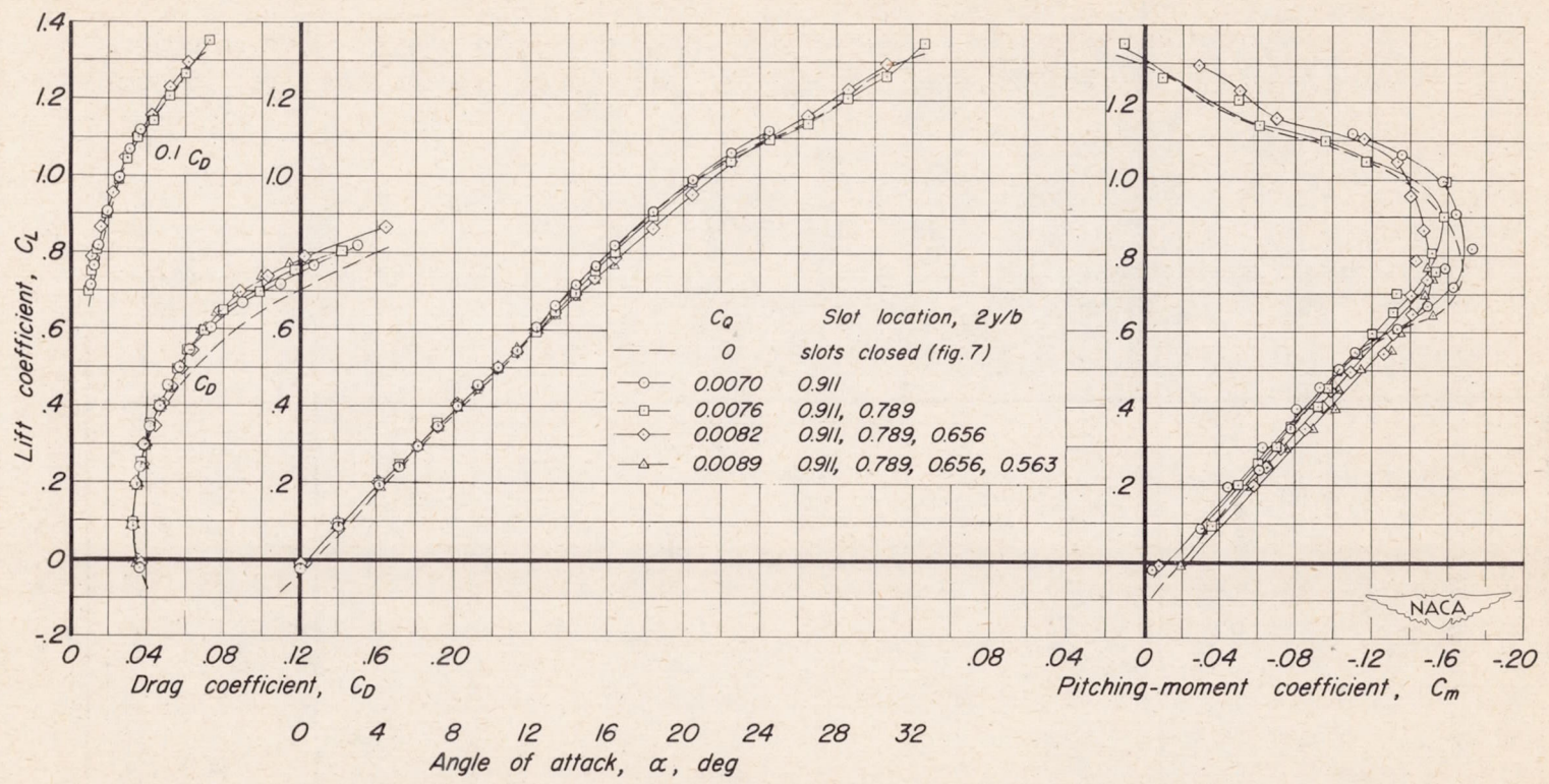
Figure 8.-The effects of suction through various slots on the longitudinal characteristics of the 63^\circ swept-back wing-fuselage combination. Full-span leading-edge flaps deflected 35^\circ . Tip tanks attached. R, 5 \times 10^6 .
