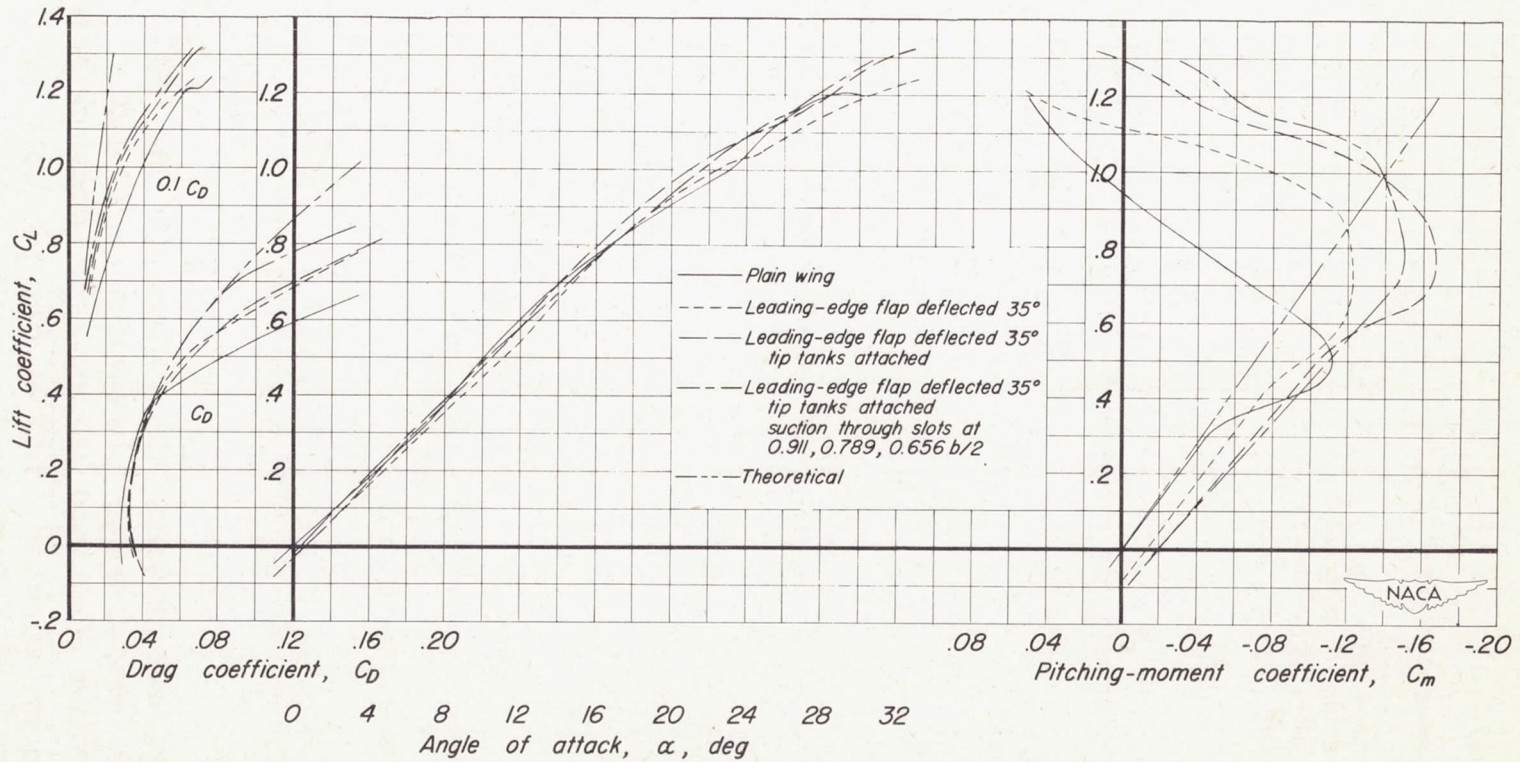
Figure 9.- Summary of the effects of the various modifications on the longitudinal characteristics of the 63° swept-back wing-fuselage combination. R, 5 \times 10^6 .
