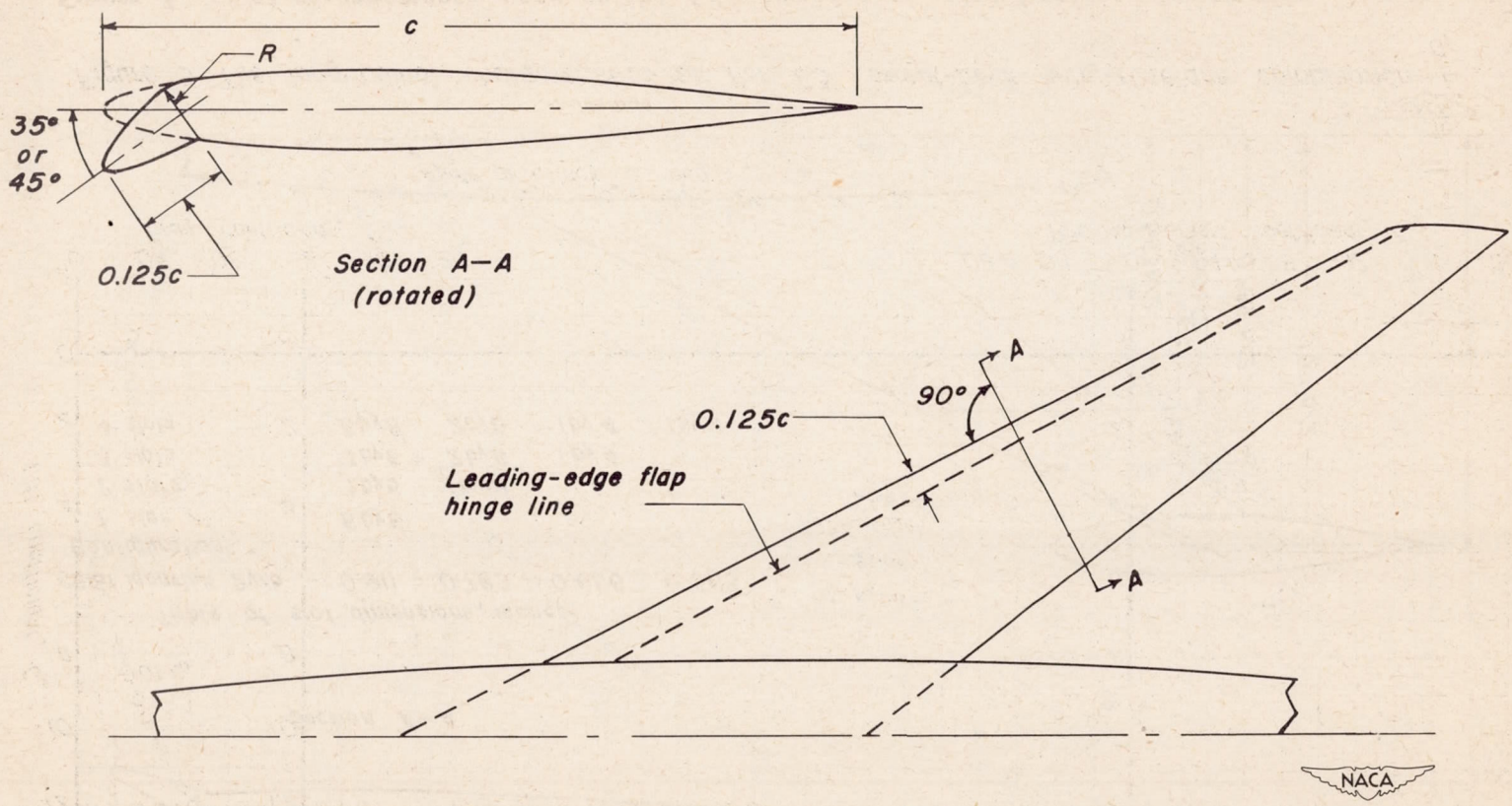
Figure 4.—Leading-edge flap used on the 63° swept-back wing-fuselage combination.
