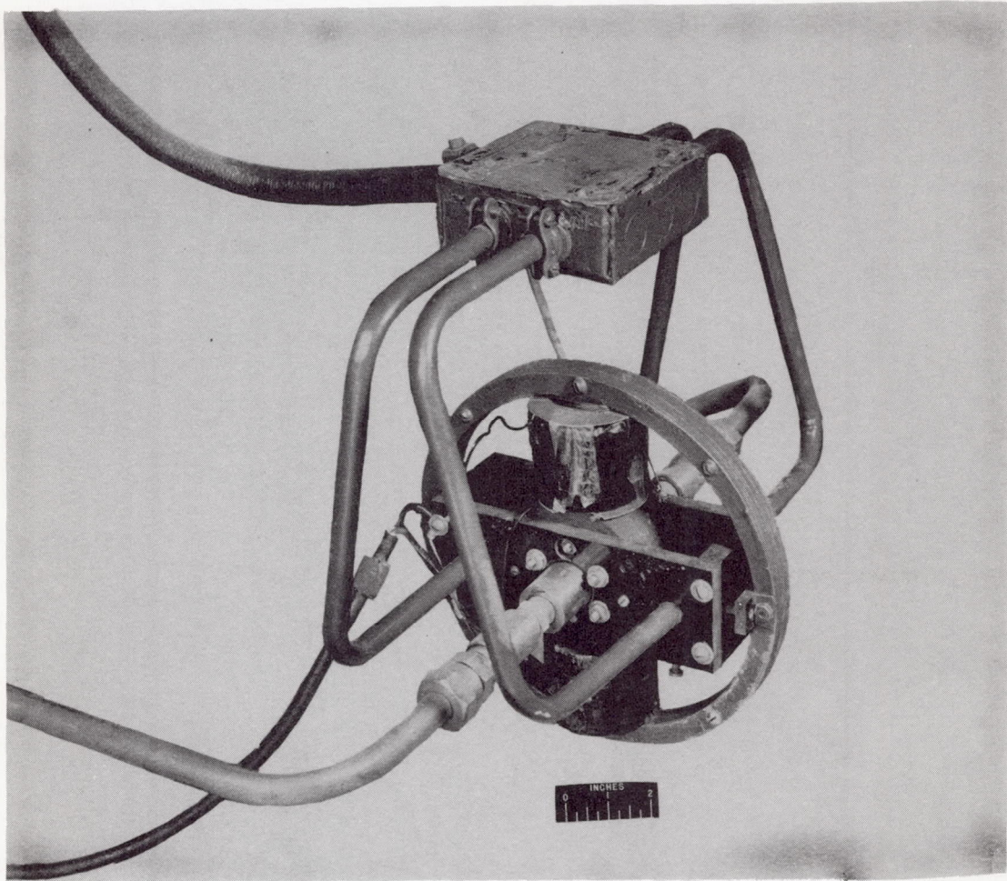
Figure 3. - Electromagnetic flowmeter.
