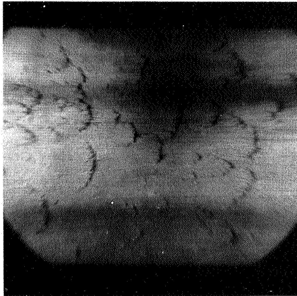
(b) Air temperature, 800° F; water flow, 0.130 pound per second per foot; pyrex tube diameter, 4 inches.
