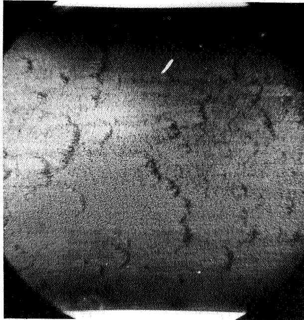
(a) Air temperature, 80° F; water flow, 0.093 pound per second per foot; Lucite tube diameter, 4 inches.
