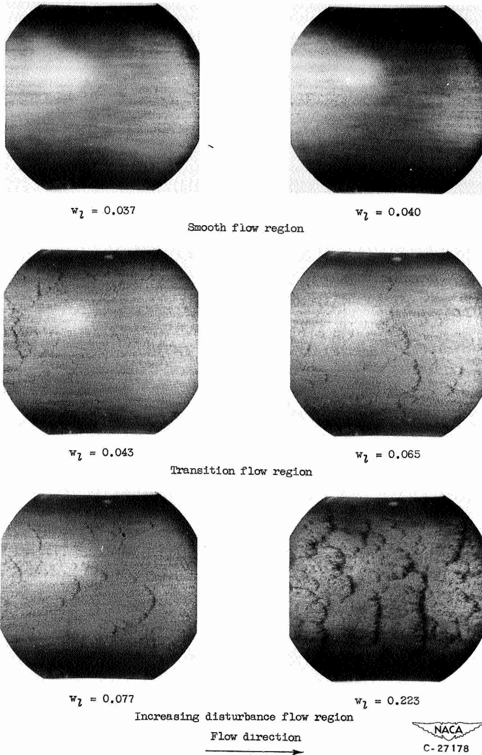
Figure 3. - Shadowgraph pictures of annular water flow with cocurrent air flow in horizontal tube. Air temperature, 80° F; Lucite tube diameter, 4 inches; liquid flow, w_l , pounds per second per foot of circumference.
