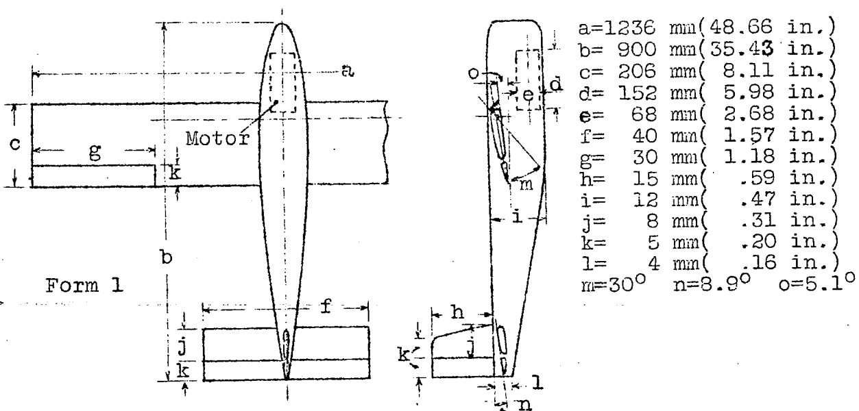
Fig. 15 Model for aileron test
