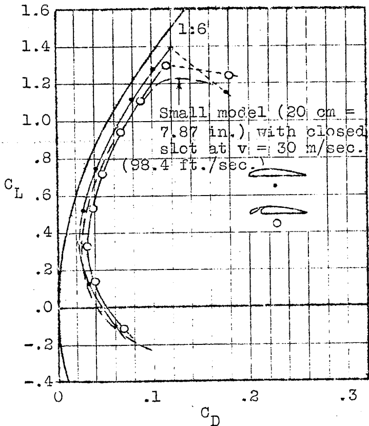
Fig. 7 Wing section O/100 (large model) with closed or stopped-up slot. v = 40 m/sec. (131.2 ft./sec.)
