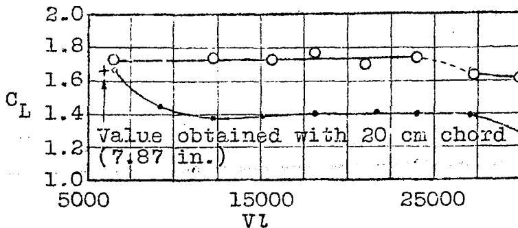
Fig. 6 Wing section O/100 with and without slot and with various index values, V_l
