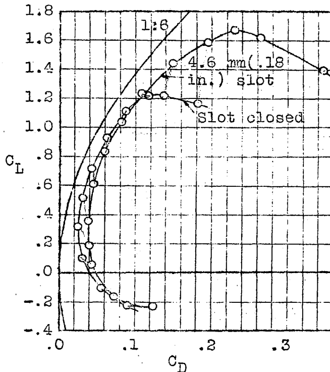
Fig. 1 Wing section O/100 (small model)
