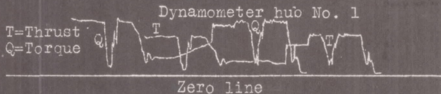
Fig. 15 Diagram of dynamometer hub for Liberty engine at different loads.
