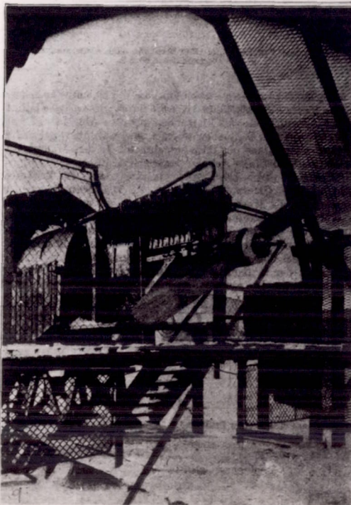
Fig. 9 Dynamometer hub on Liberty 12
