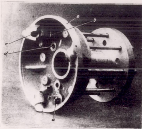
Fig. 5 Hub 103 with flange 104 a) Backward stop b) Forward stop c) Torque socket-bearing 111 d) Hole for thrust bearing 112 e) Adjustment mark
