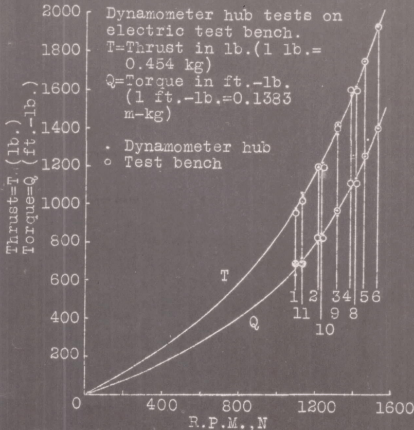
Fig. 14 Test diagram of dynamometer hub according to values obtained from Fig. 13
