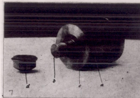
Fig. 7 Torque cylinder 140 a) Cylinder 140 b) Piston-support rod 162 c) Oil inlet d) Screw cap 164
