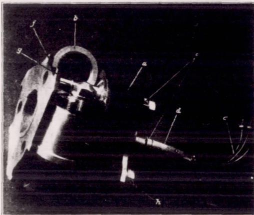
Fig. 8 Pressure-cylinder carrier 102 with pressure-cylinder and plug guide. a) Pressure-cylinder carrier 102 b) Torque cylinder c) Plug guide 120 d) Safety device e) Pipes 185 f) Front stop g) Rear stop h) Screw cap 164
