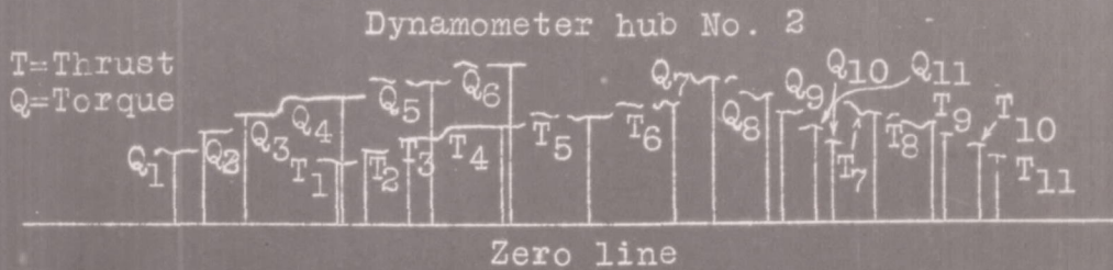
Fig. 13 Test diagram of dynamometer hub, made on electric test bench
