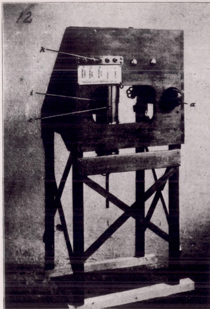
Fig.12 Rear view of instrument table a) Air cyl. c) Oil cyl. i) Oil tank k) Connections for dynamometer hub and pressure disk.
