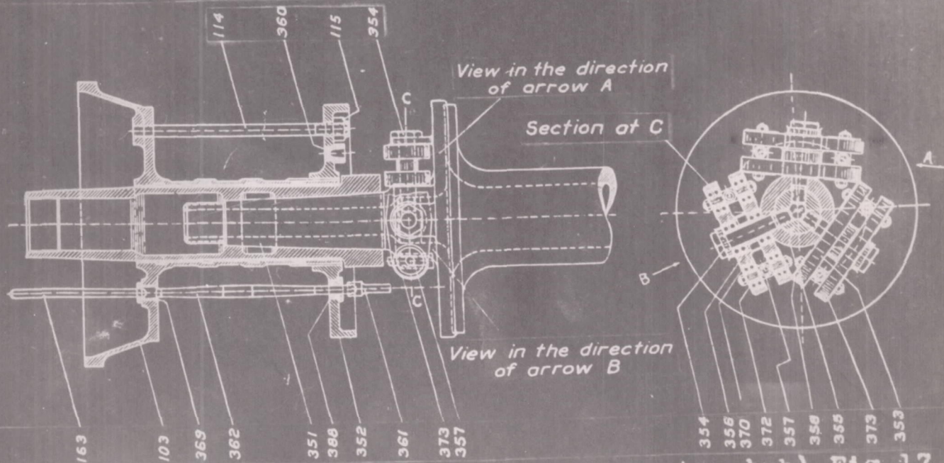
Fig. 16 (Reversing device for dynamometer hub) Fig. 17 for pusher propeller.
