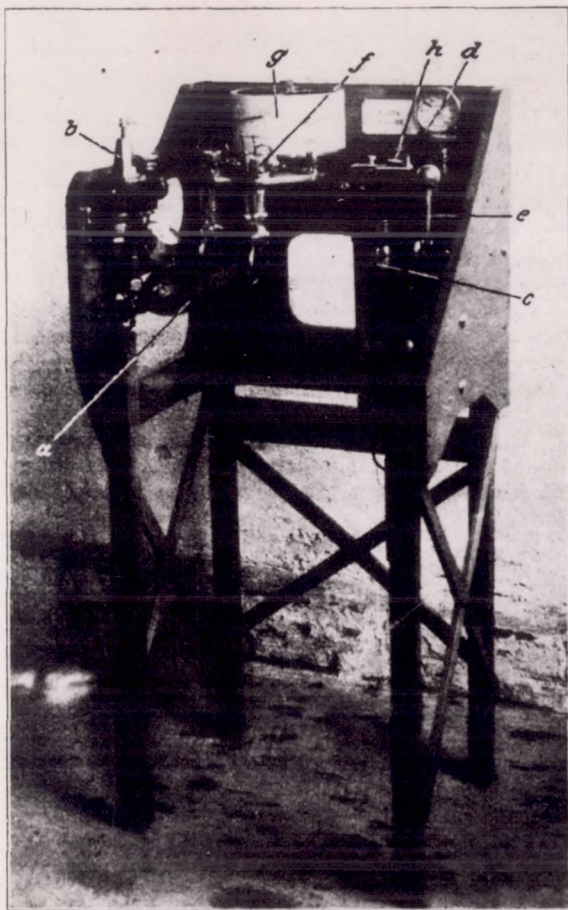
Fig.11 Instrument table
