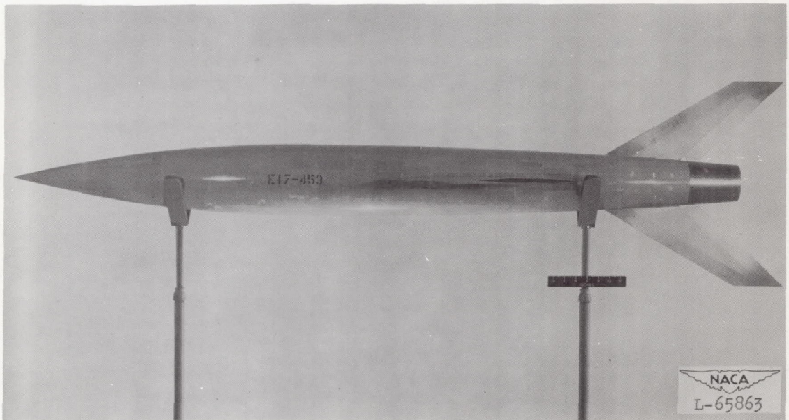
Figure 2.- Test configuration.
