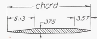
Typical streamwise fin section
