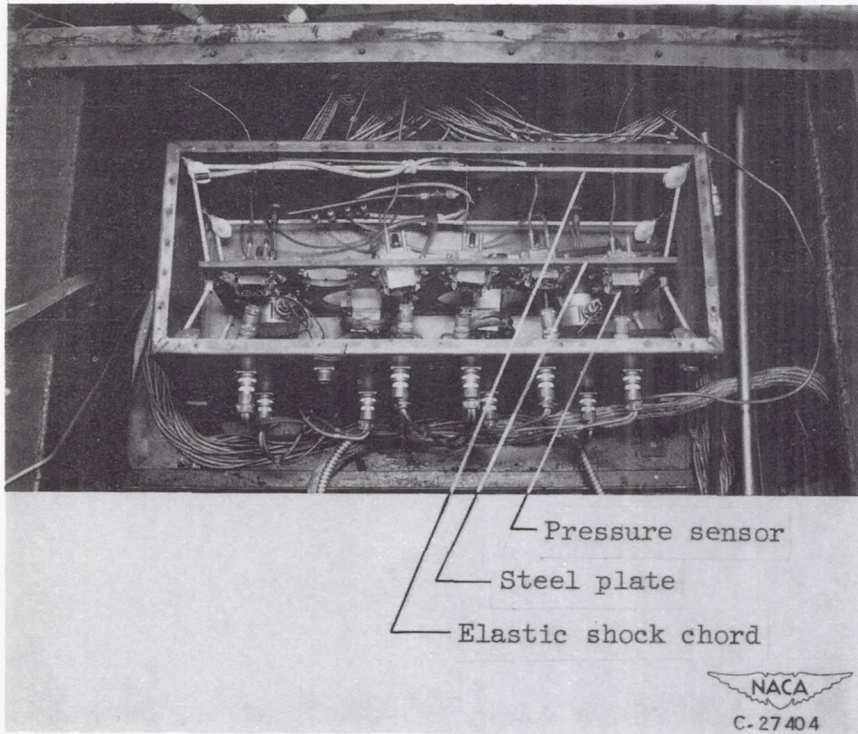
Figure 2. - Mounts to isolate pressure sensors from mechanical vibration.
