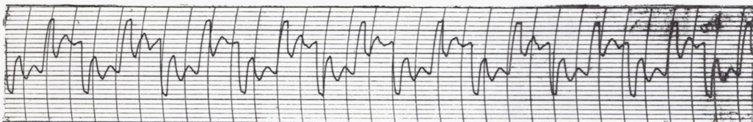
(c) Pressure sensor, underdamped; tube length, 6 feet; tube radius, 0.052 inch.
