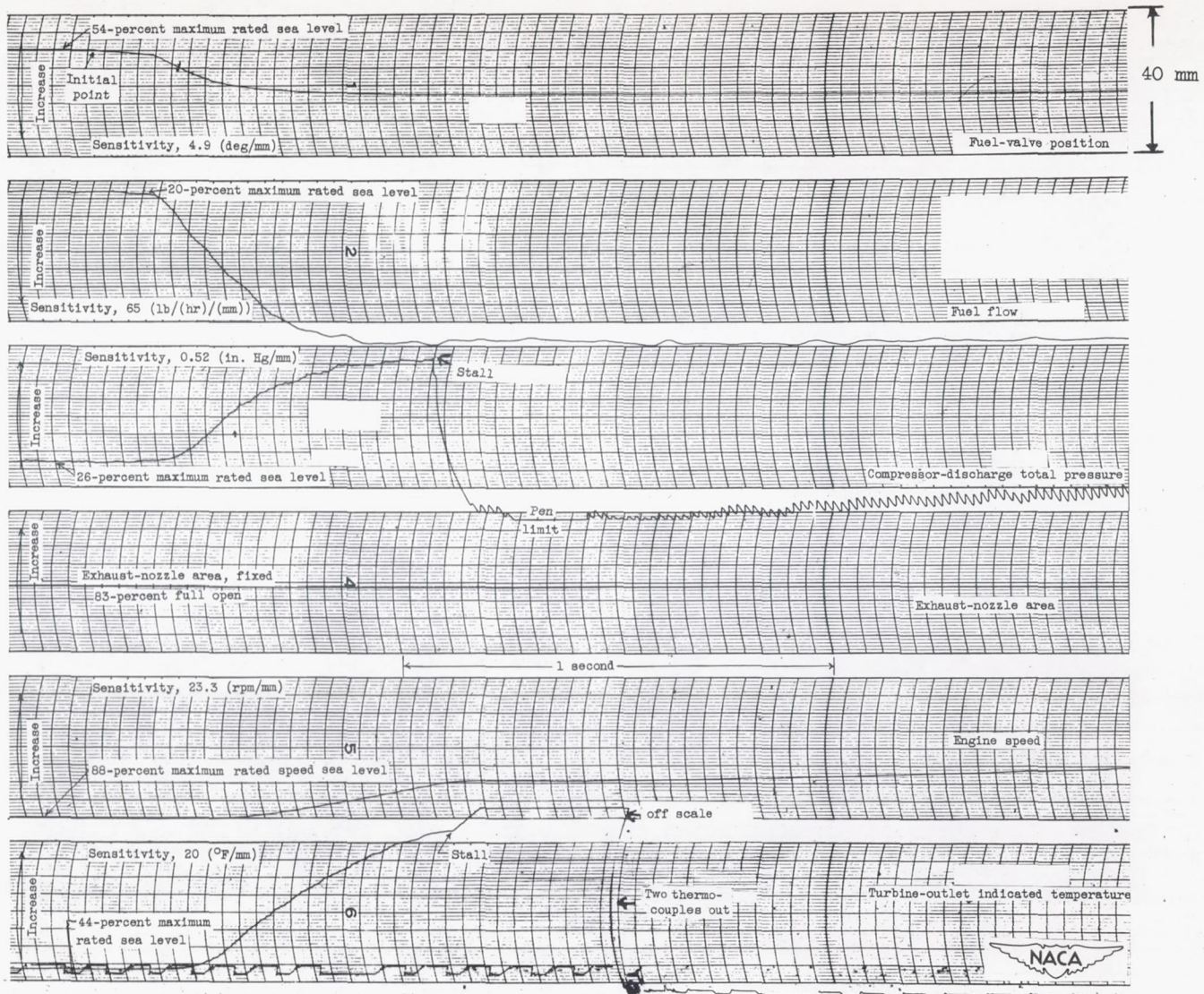
Figure 9. - Time record of several variables during compressor stall in turbojet engine.
