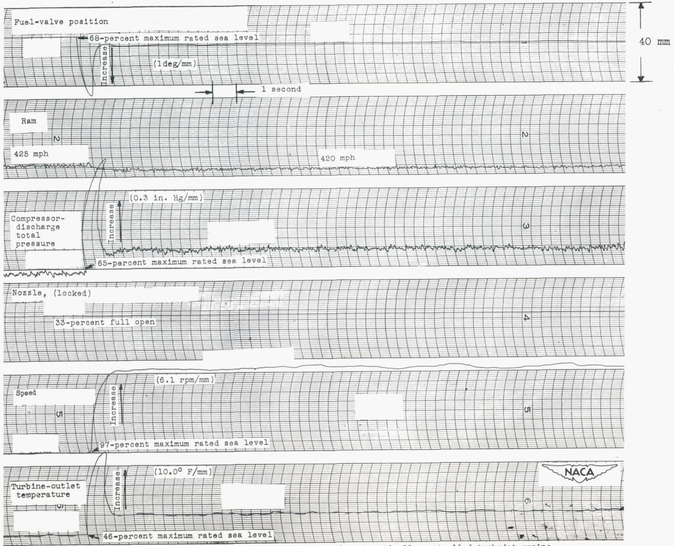
Figure 8. - Sample recording of transient events in automatically controlled turbojet engine.
