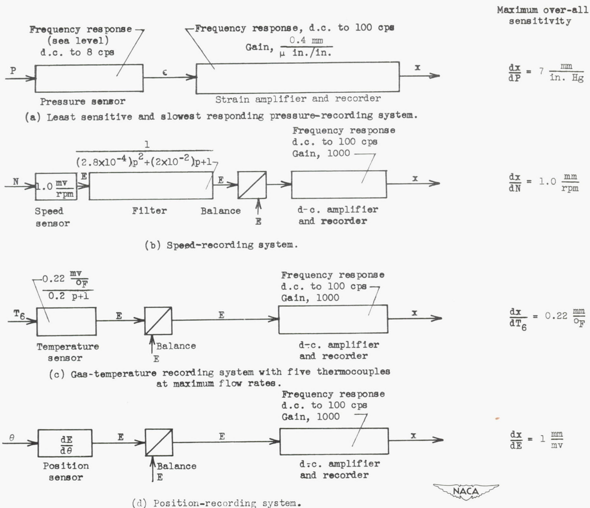
Figure 4. - Block diagrams showing component lags and gains of basic sensing systems.
