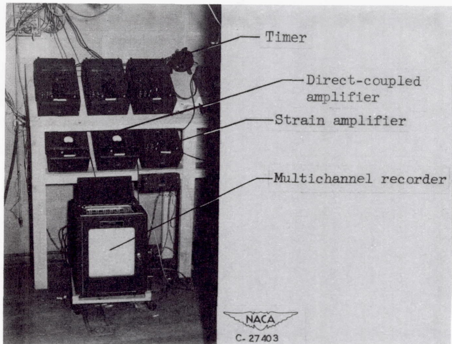
Figure 1. - Recording oscillograph with six amplifiers.
