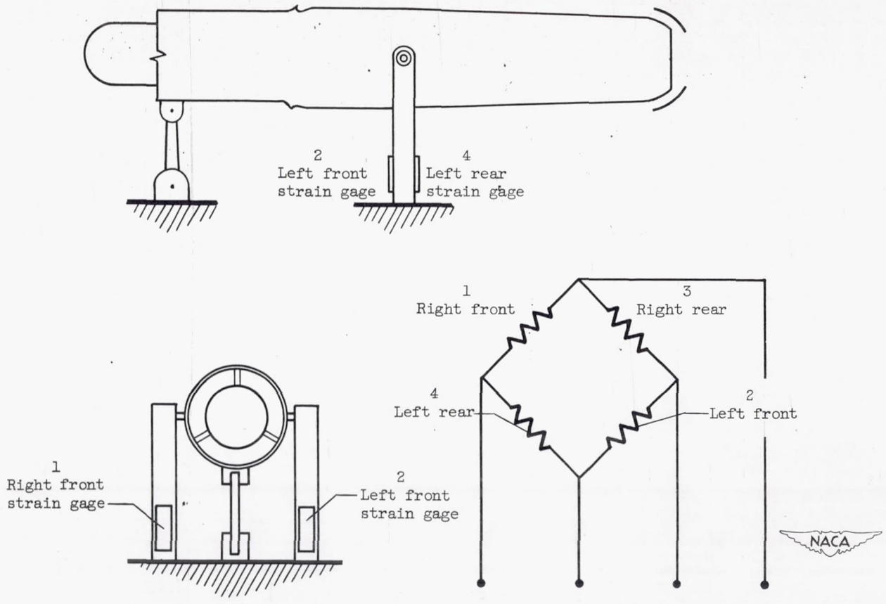
Figure 7. - Sketch showing method of mounting engine and location of strain gages for thrust-change measurements.
