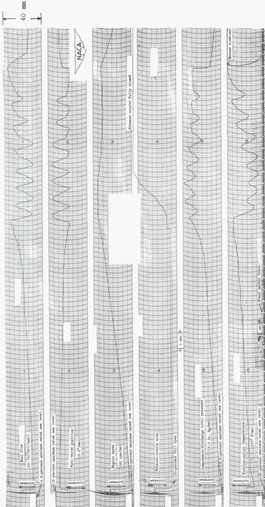
Figure 6. - Time record of variables in turbojet engine during instability resulting from improper control.
