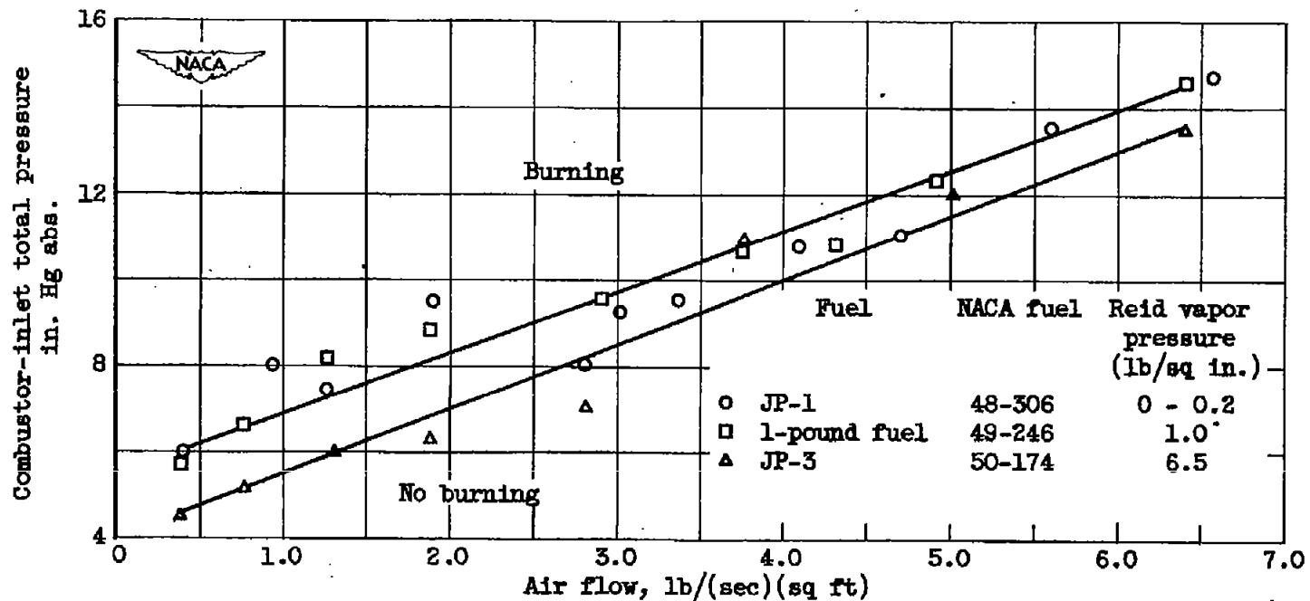
Figure 8. - Effect of fuel volatility, air-flow rate, and pressure on burning limits of single tubular combustor. Inlet-air temperature, -10^{\circ} F; inlet-fuel temperature, -40^{\circ} F.
