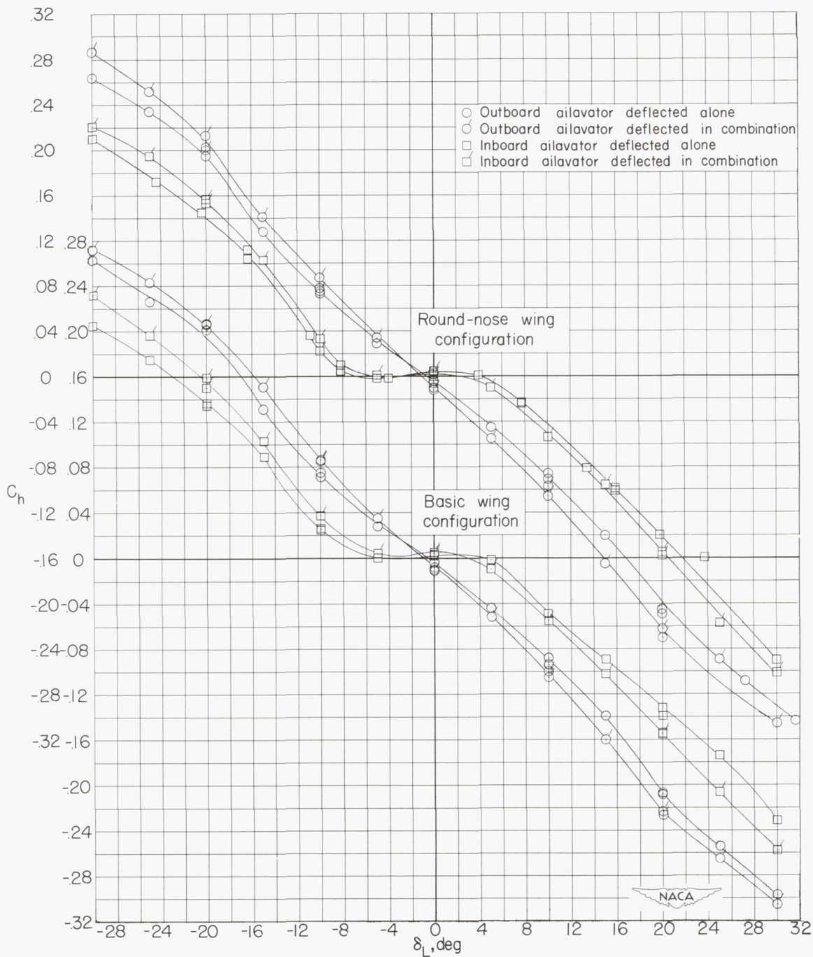
Figure 16.- Effect of ailerator plan form on the variation of C_h with \delta_L for the basic and round-nose wing configurations at zero uncorrected angle of attack.
