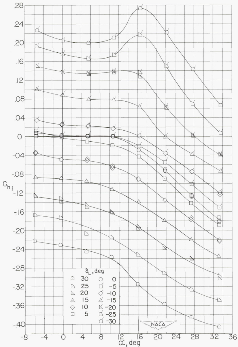
(c) Inboard ailerator deflected alone.
