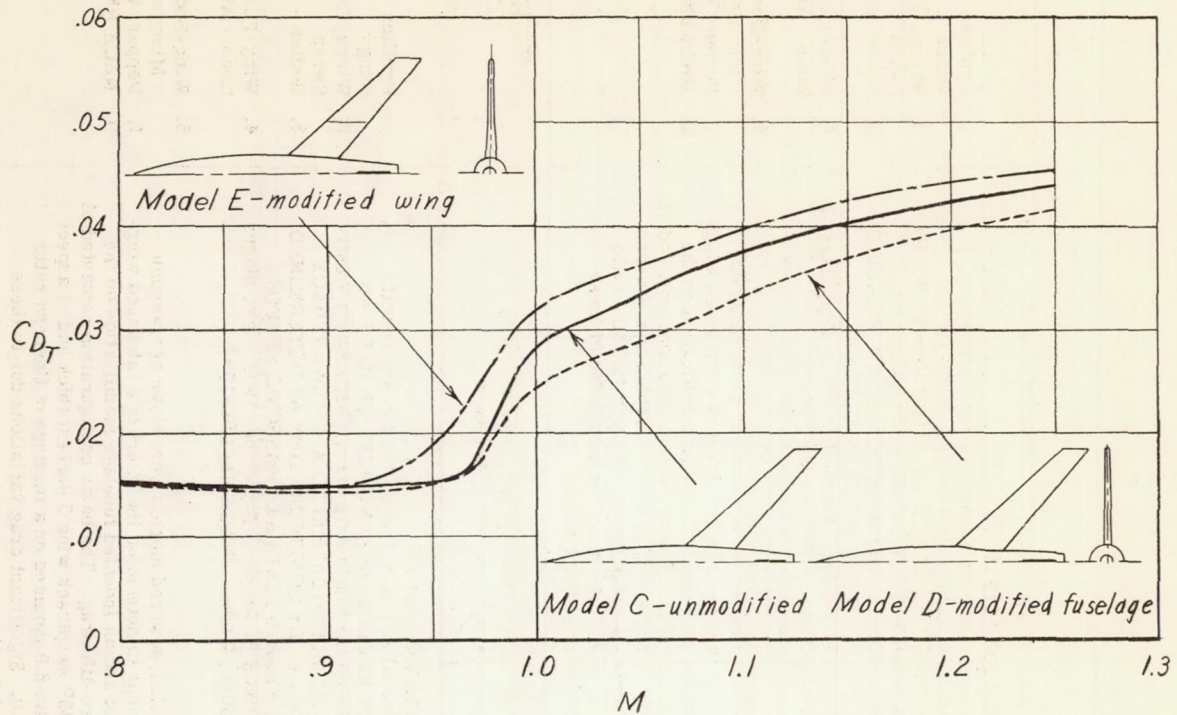
(a) Total drag coefficient.
