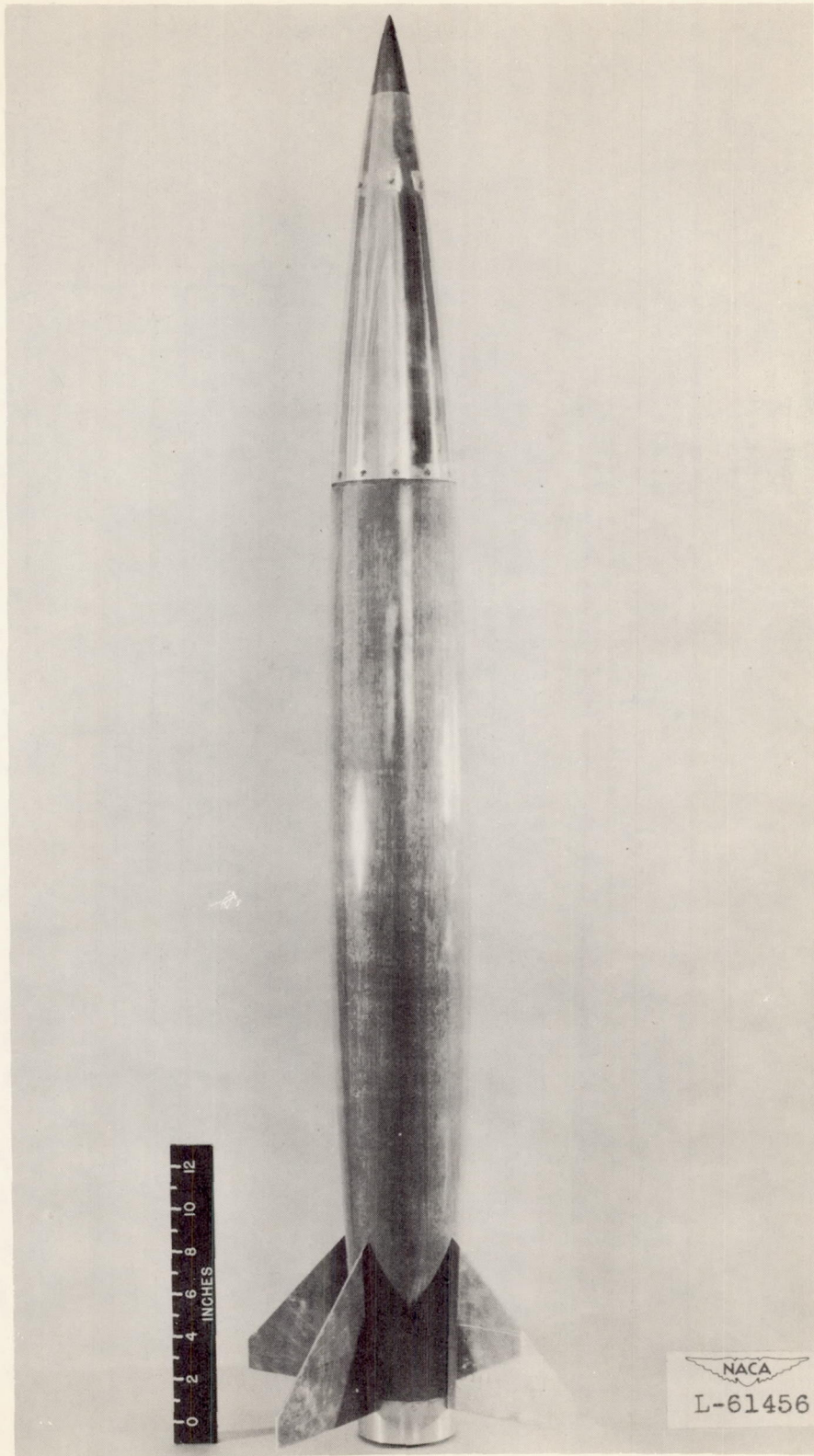
Figure 2.- Fuselage with four fins. Models A,B.
