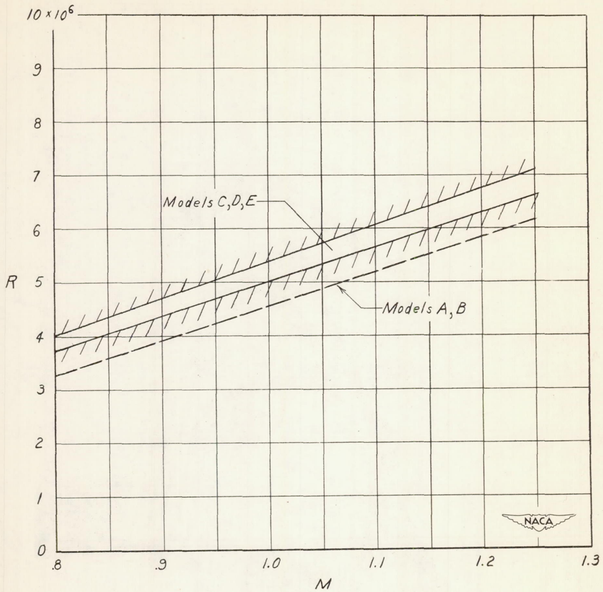
Figure 7.- Variation of Reynolds number range with Mach number for models tested. (Based on wing mean aerodynamic chord.)
