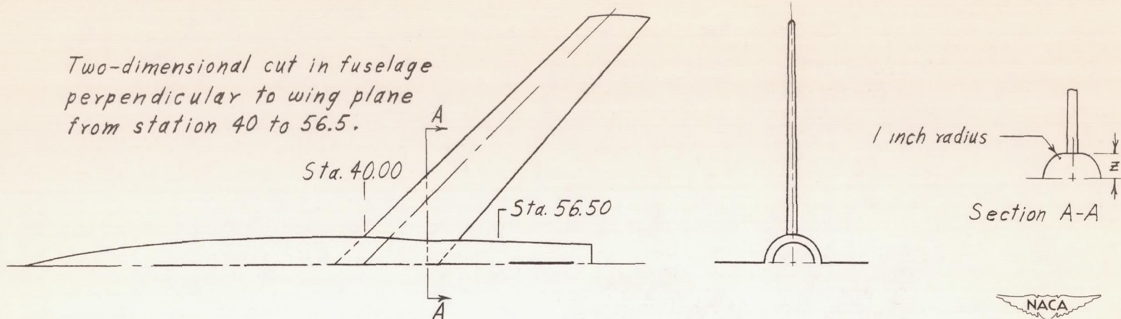
(a) Model D - modified fuselage.
