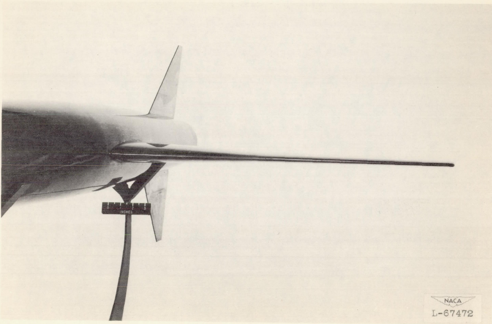
Figure 5.- Front three-quarter view of thickened wing root. Model E.
