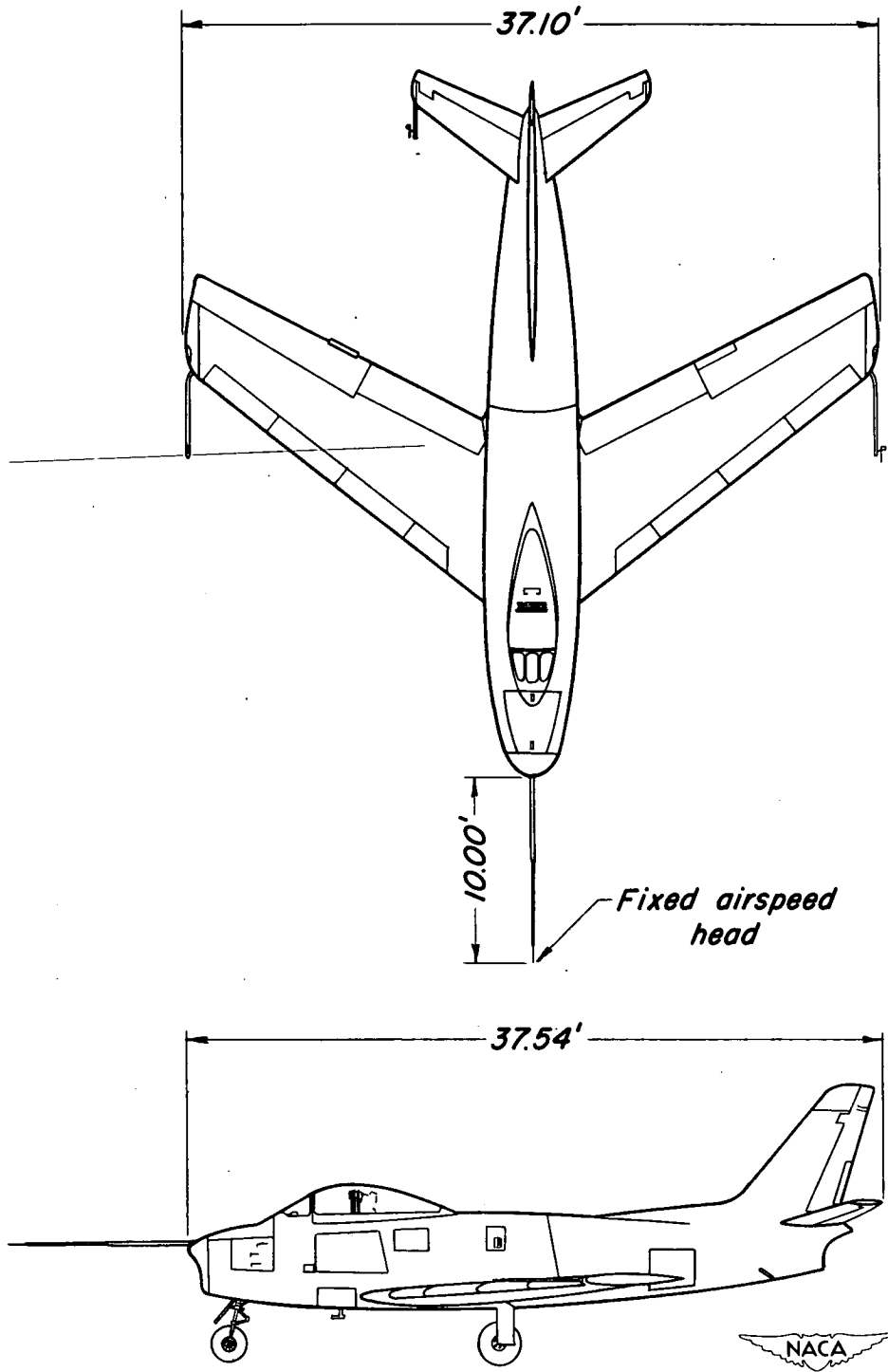
Figure 2.-Two-view drawing of test airplane.
