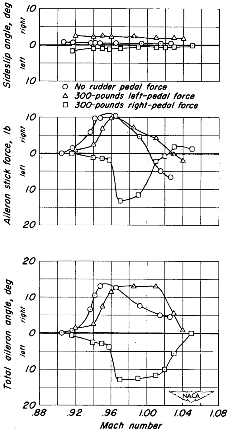
(a) Production airplane.
