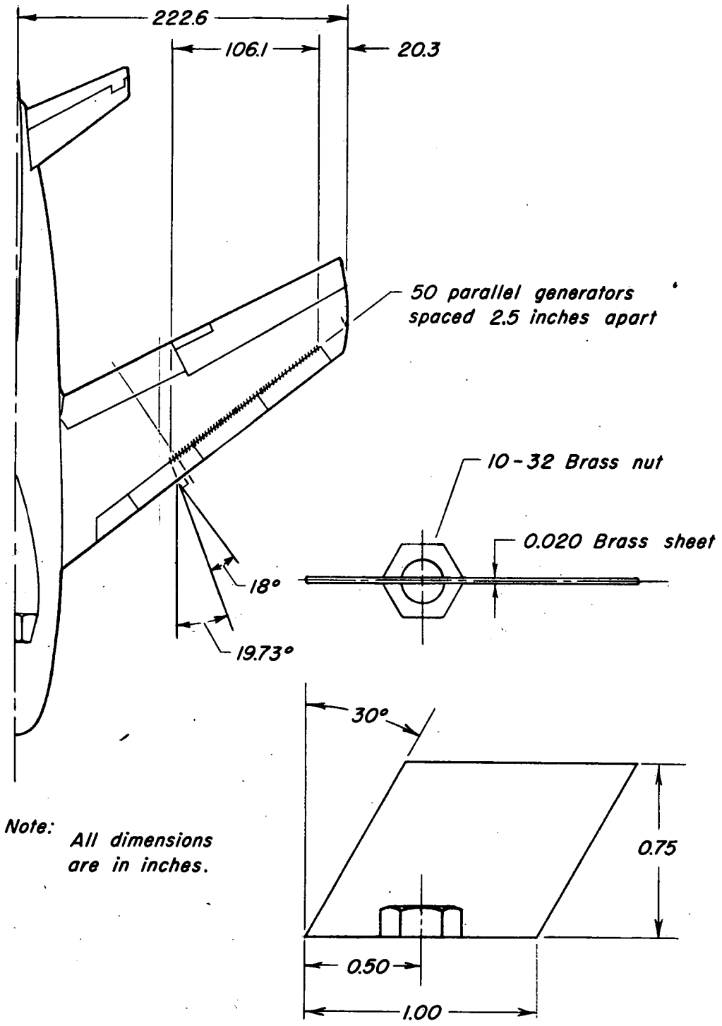
(c) Dimensions. Figure 3.- Concluded.
