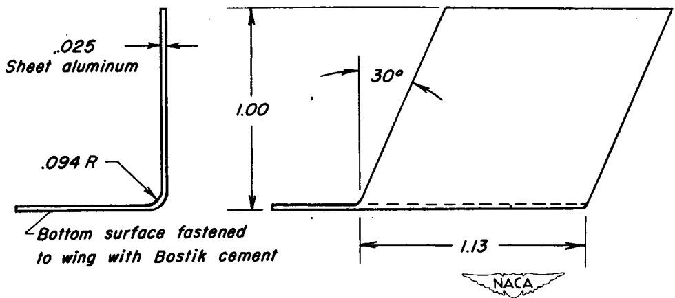
(b) Dimensions.
