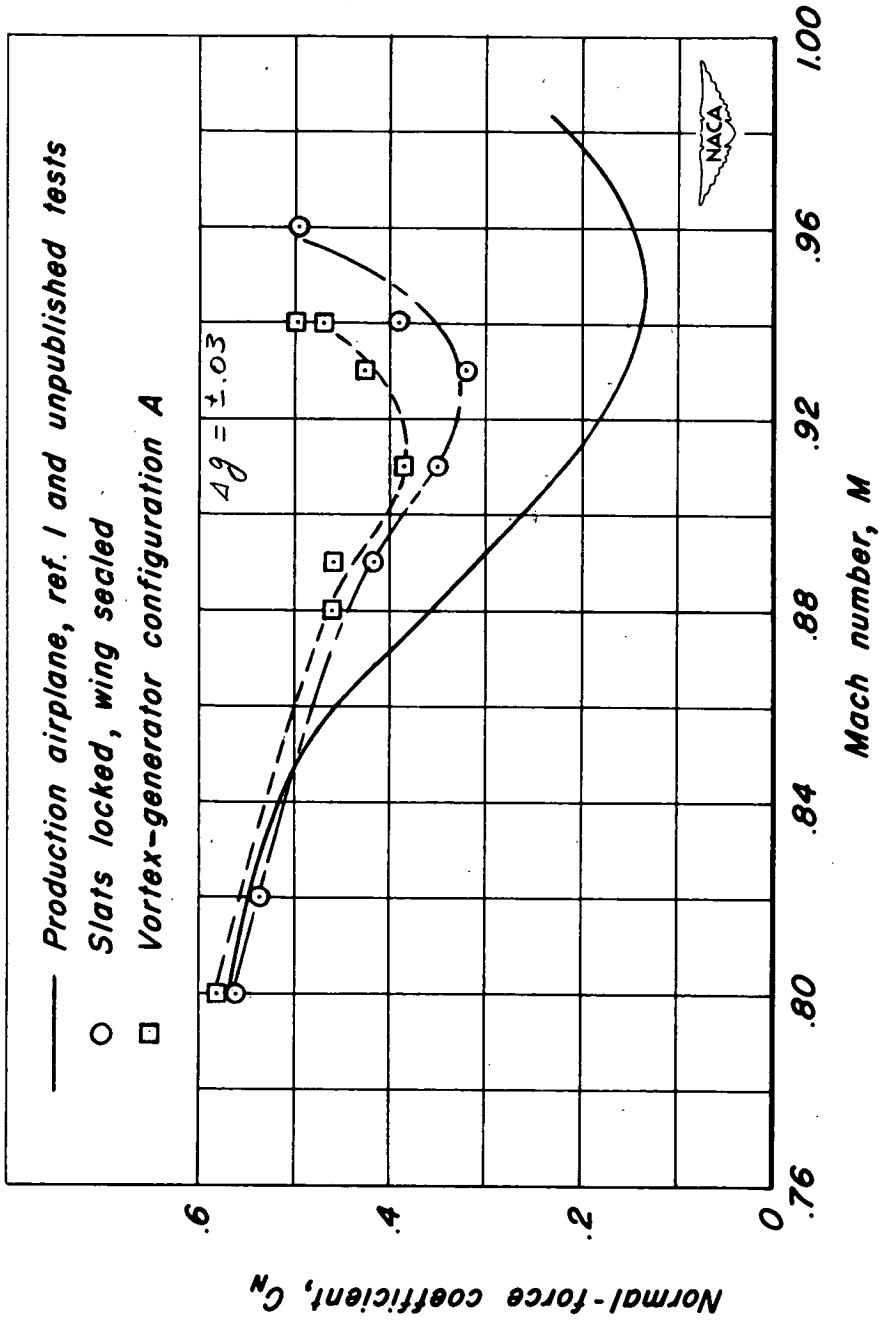
Figure 7.- The effects of the slats-locked and vortex-generator modifications on the buffet boundary.
