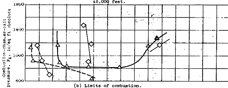
(b) Limits of combustion.
