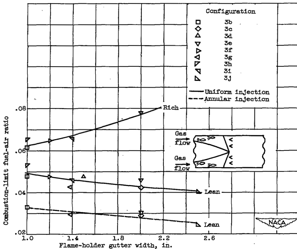
Figure 12. - Effect of flame-holder gutter width on limits of combustion. Combustion-chamber-exit pressure, 1400 pounds per square foot absolute.
