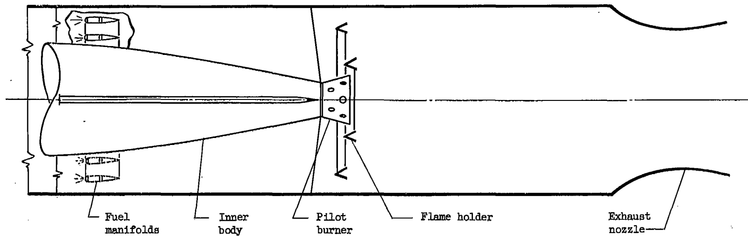
Figure 5. - Schematic diagram of combustion chamber for configuration 4.
