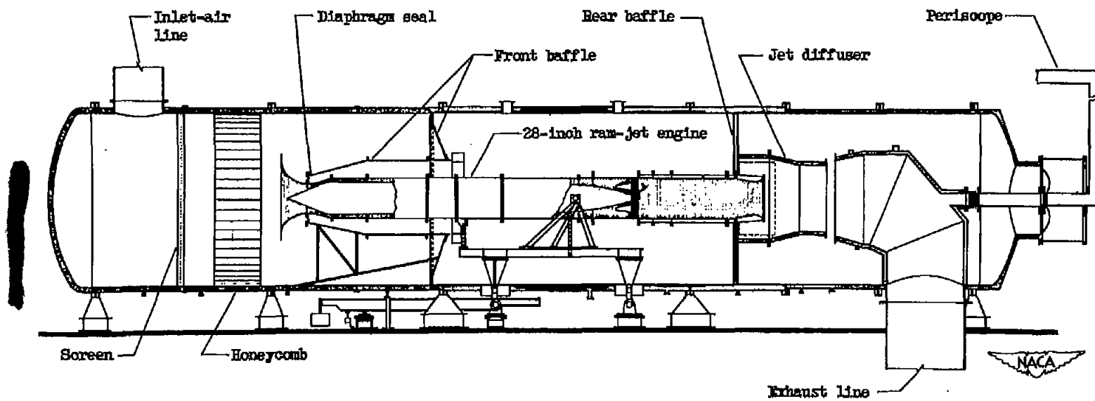
Figure 7. - Schematic diagram of 28-inch ram-jet engine installed in 10-foot altitude test chamber.
