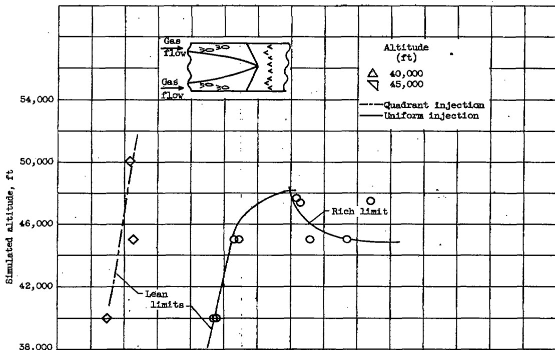
(a) Limits of combustion.
