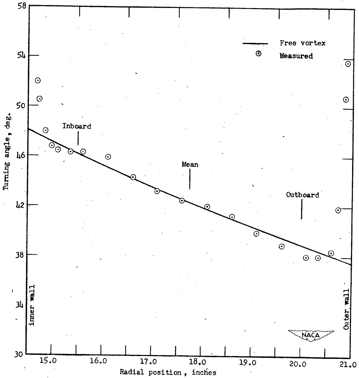
Figure 4.- Comparison of measured guide-vane turning angle with angles required for free-vortex flow.
