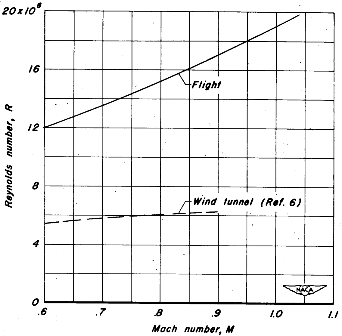
Figure 16.- Variation of average Reynolds number with Mach number.
