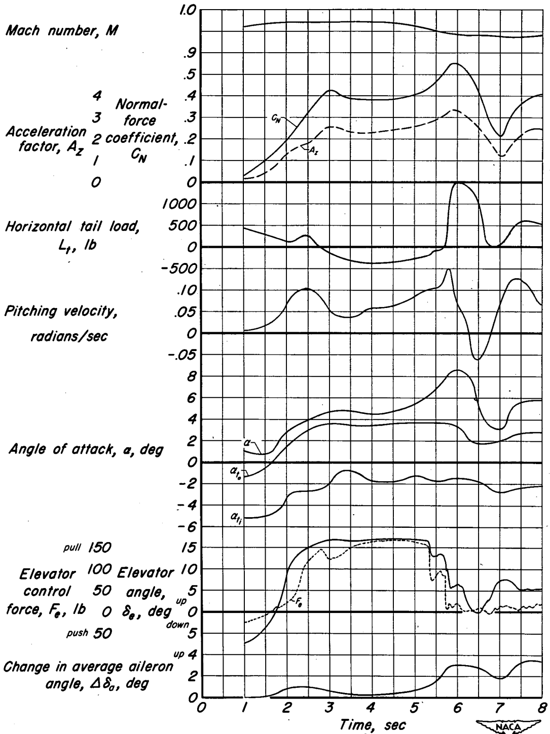
Figure 12.-Time-history plot of a pull-out in which a pitch-up occurred as the Mach number decreased.
