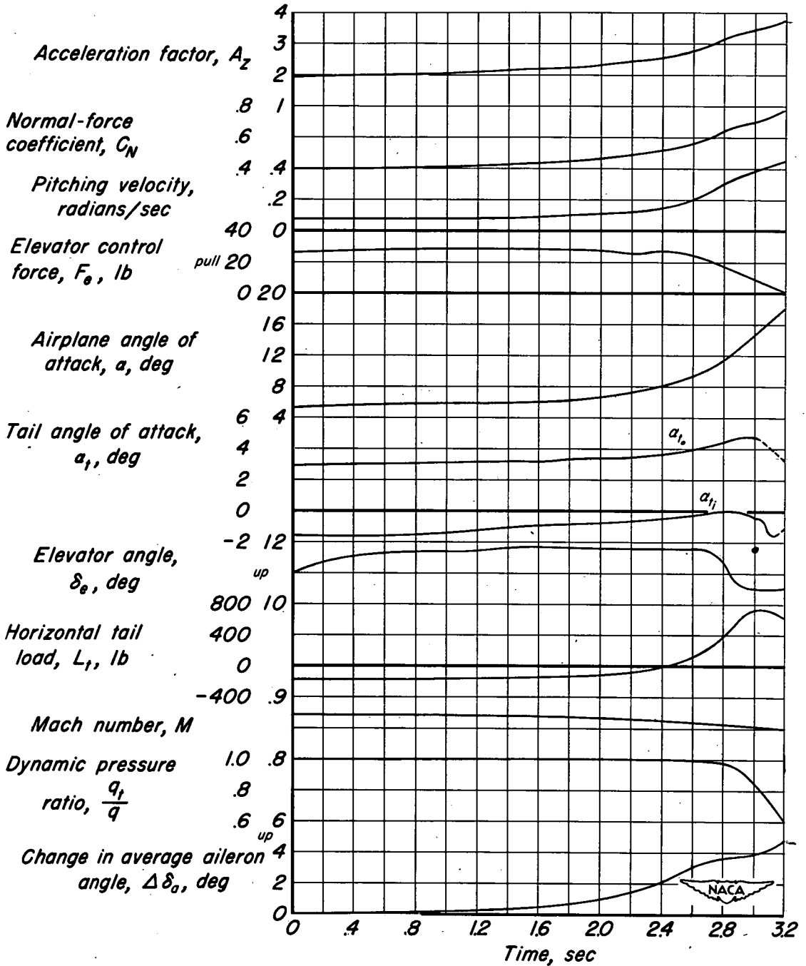
Figure 4.- Time-history plot of a pitch-up encountered in a wind-up turn.
