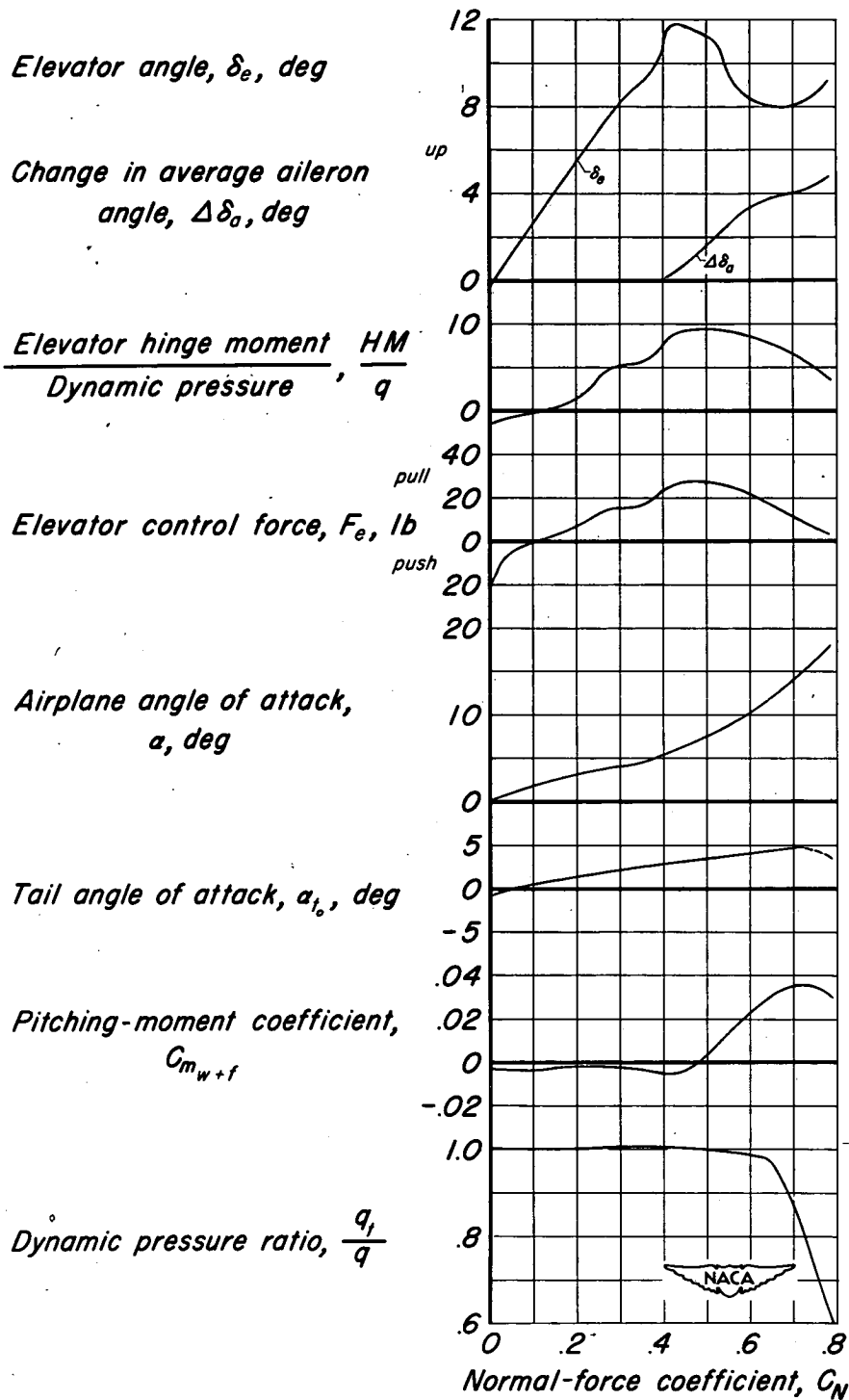
Figure 5.- Variation of the longitudinal control characteristics with normal-force coefficient. Mach number, 0.87.
