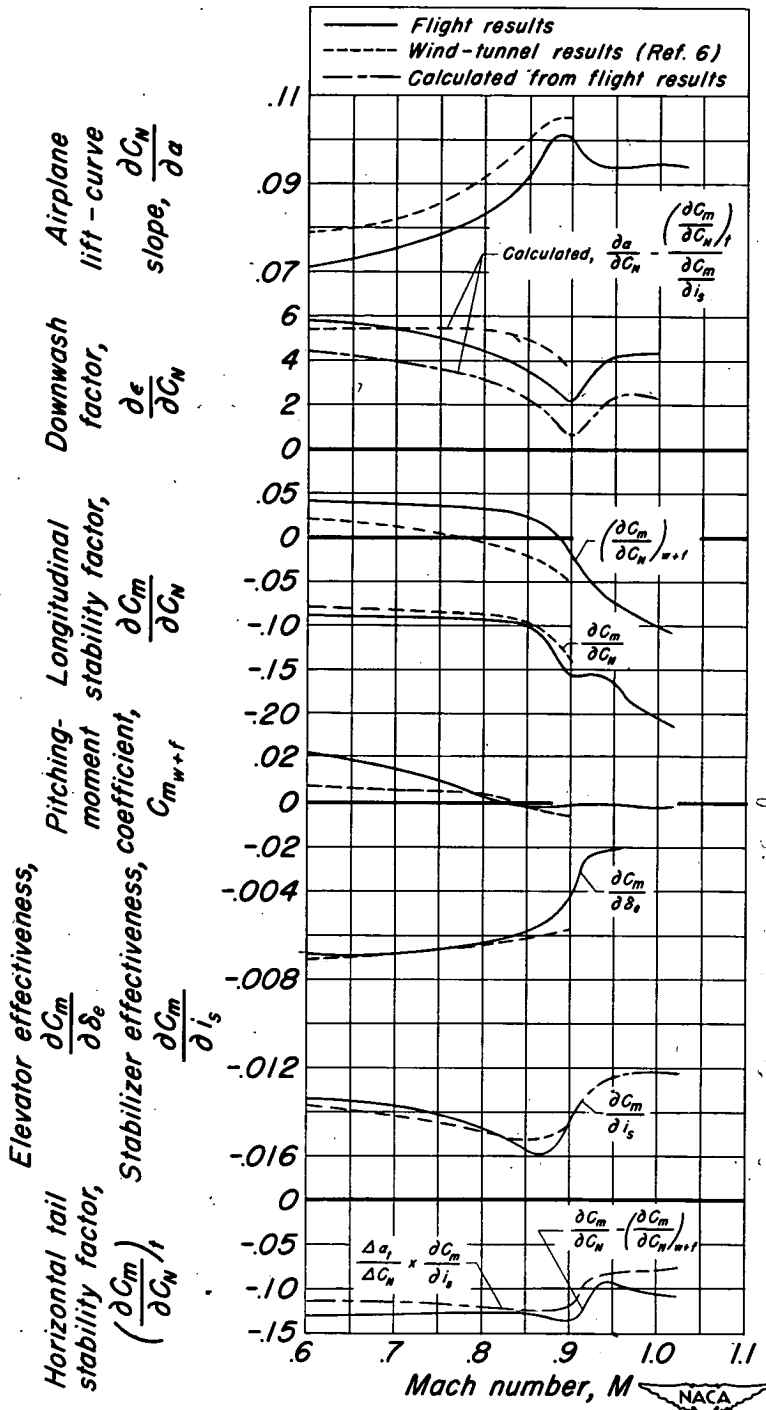
Figure 15.- Variation with Mach number of a number of aerodynamic parameters and a comparison with wind tunnel results for steady level flight.
