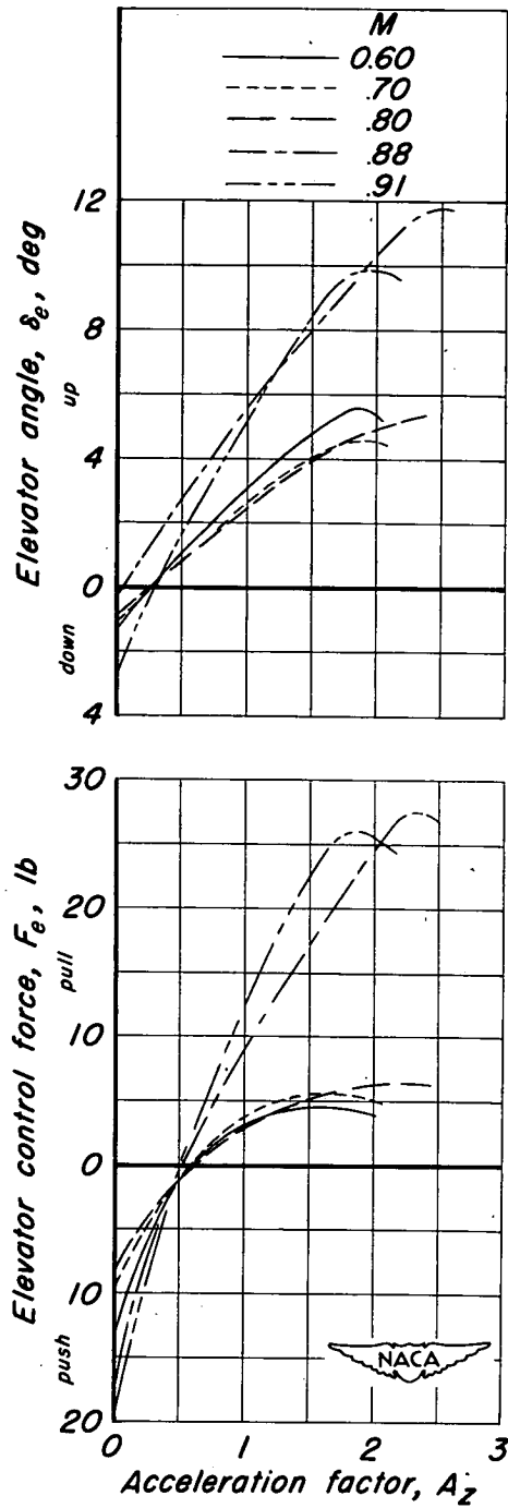
Figure 3.- Variation of elevator angle and force with normal acceleration for several Mach numbers.
