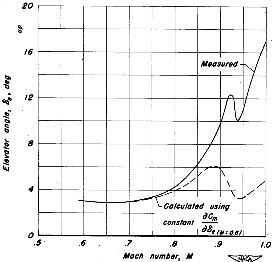
Figure 14.- Variation with Mach number of elevator angle required for balance at C_N = 0.3 .
