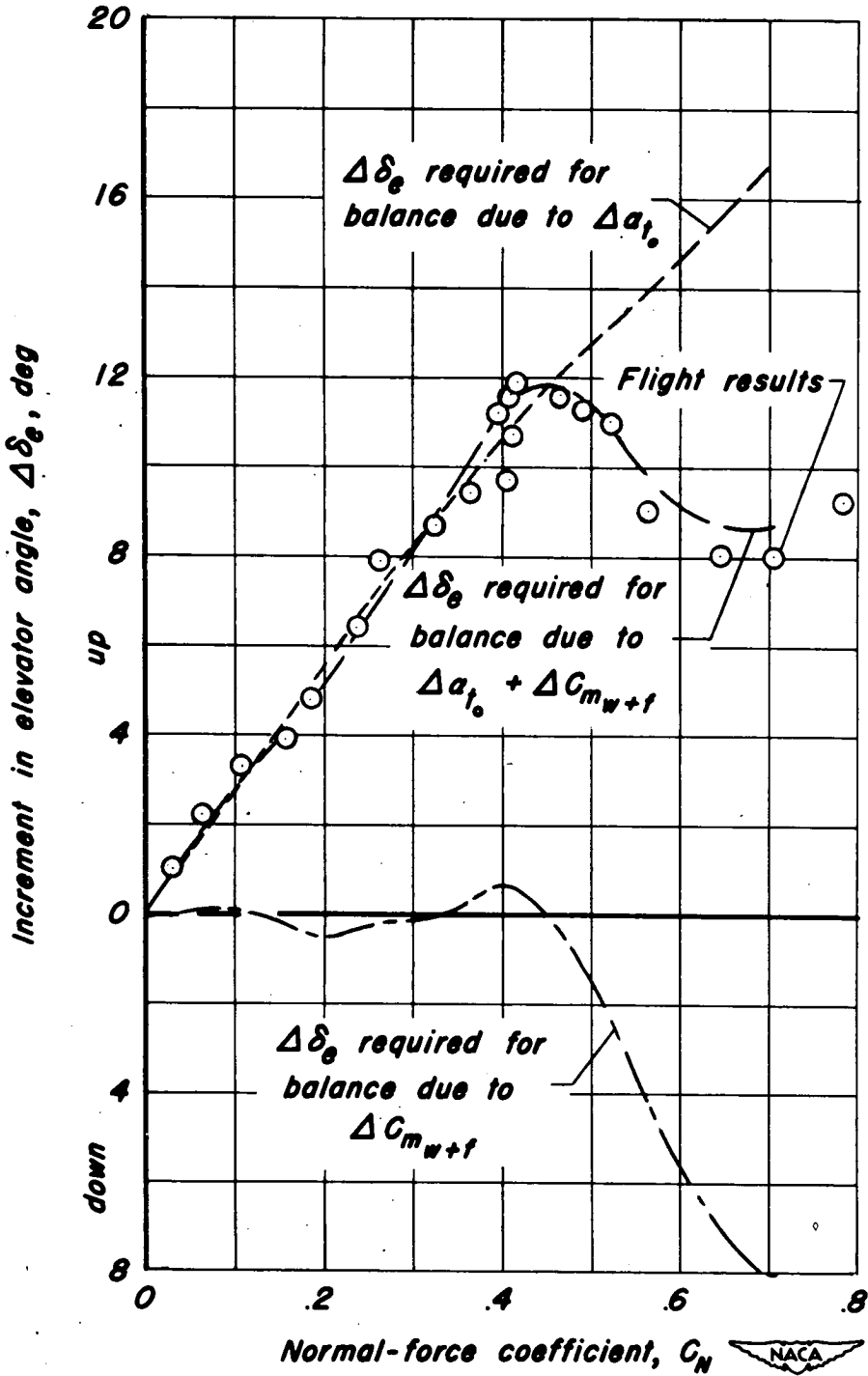
Figure 6.- Variation with C_N of elevator angle required for balance. Mach number, 0.87.
