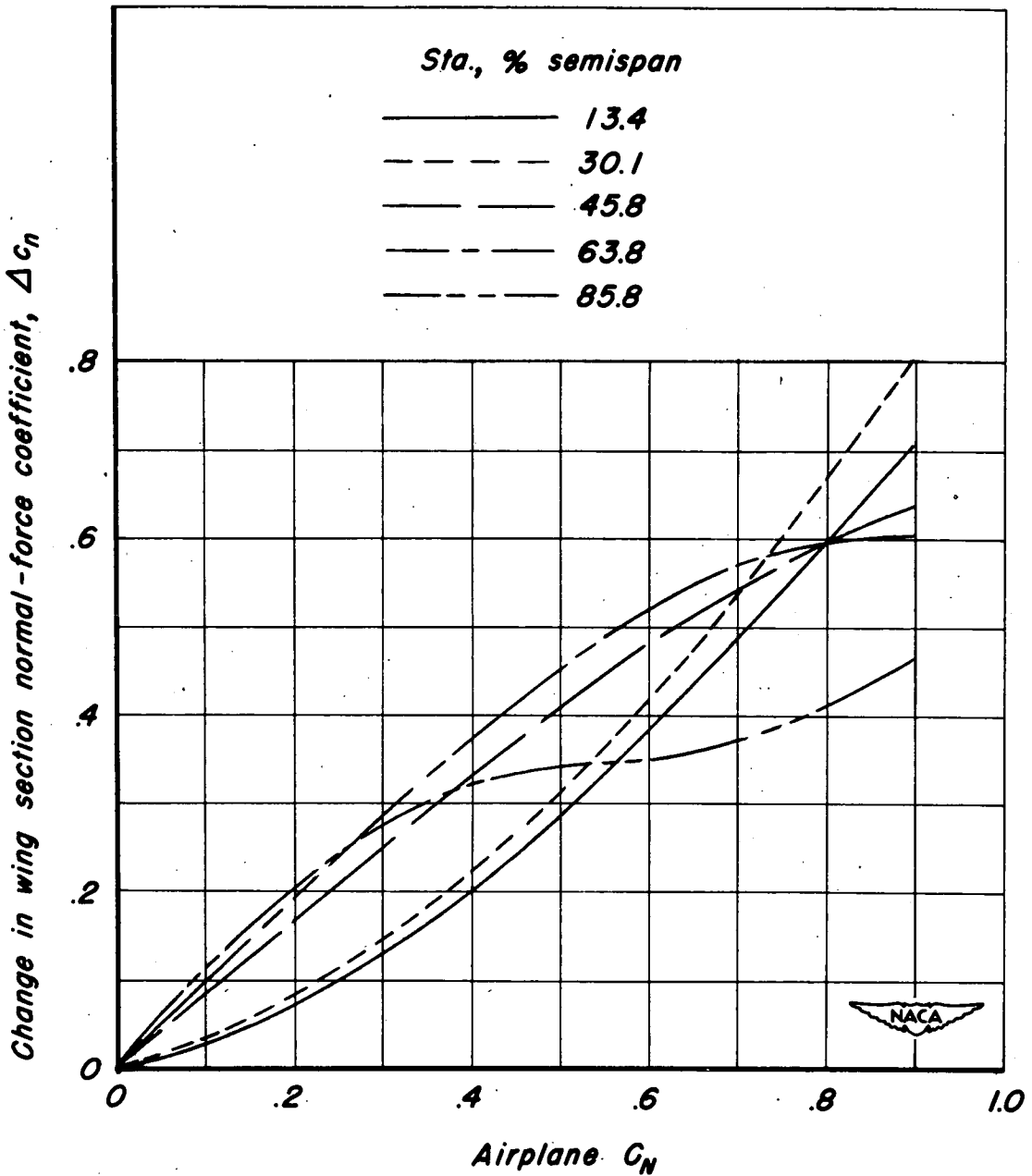
Figure 9.—Variation of \Delta c_n with airplane C_N for various spanwise stations. Mach number, 0.87.
