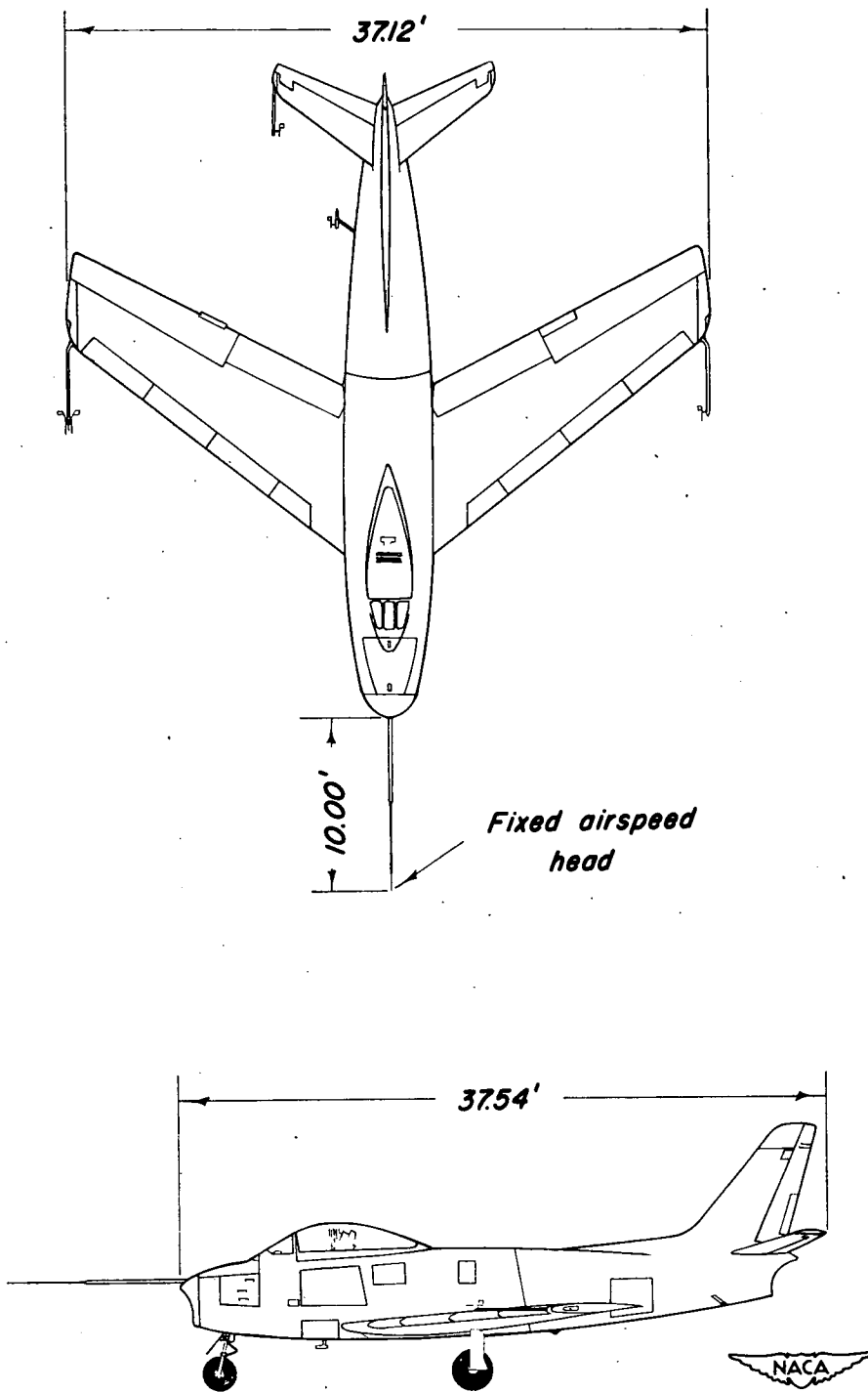
Figure 2.—Two-view drawing of test airplane showing research airspeed installation.
