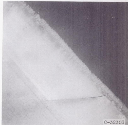
Upper surface. Icing time, 10\frac{1}{2} minutes; section drag coefficient, 0.0321.
