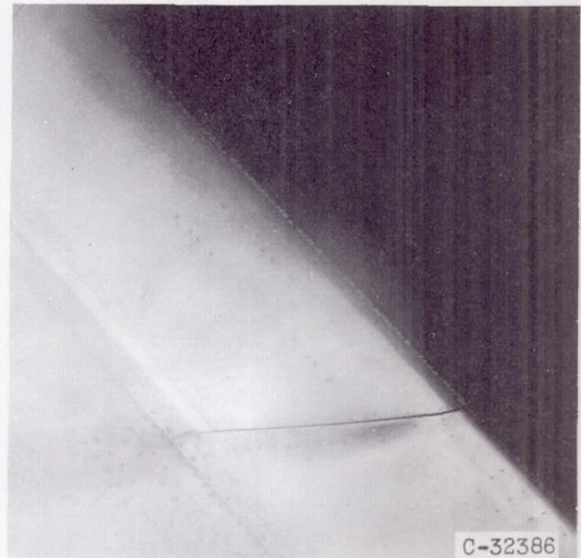
Upper surface. Icing time, 4\frac{1}{2} minutes; section drag coefficient, 0.0115.
