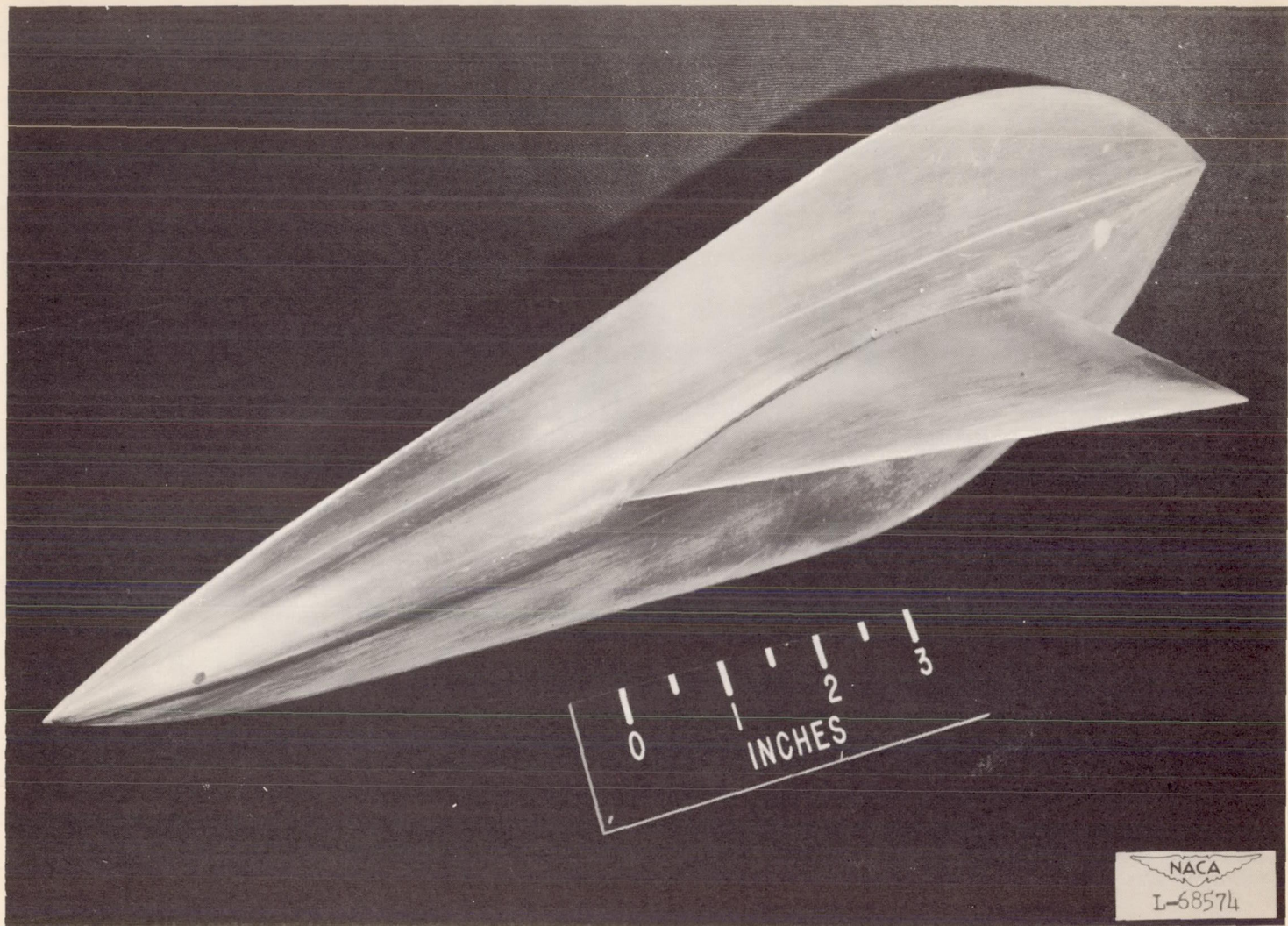
Figure 1.- Photograph of semispan wing-fuselage model and end plate. A = 2.31; 9-percent-thick biconvex section.
