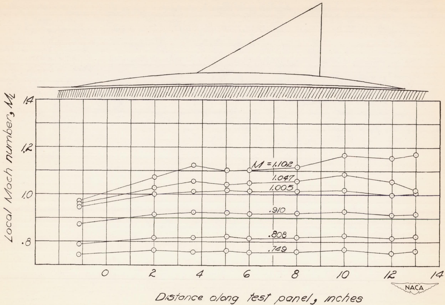
Figure 3.- Typical chordwise variation of Mach number in the test region on the surface of the airplane wing for several effective Mach numbers at the wing of the model. Chordwise location of model is also shown.
