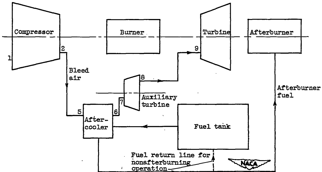
(b) Aftercooler heat exchange to fuel and expansion through auxiliary turbine.
