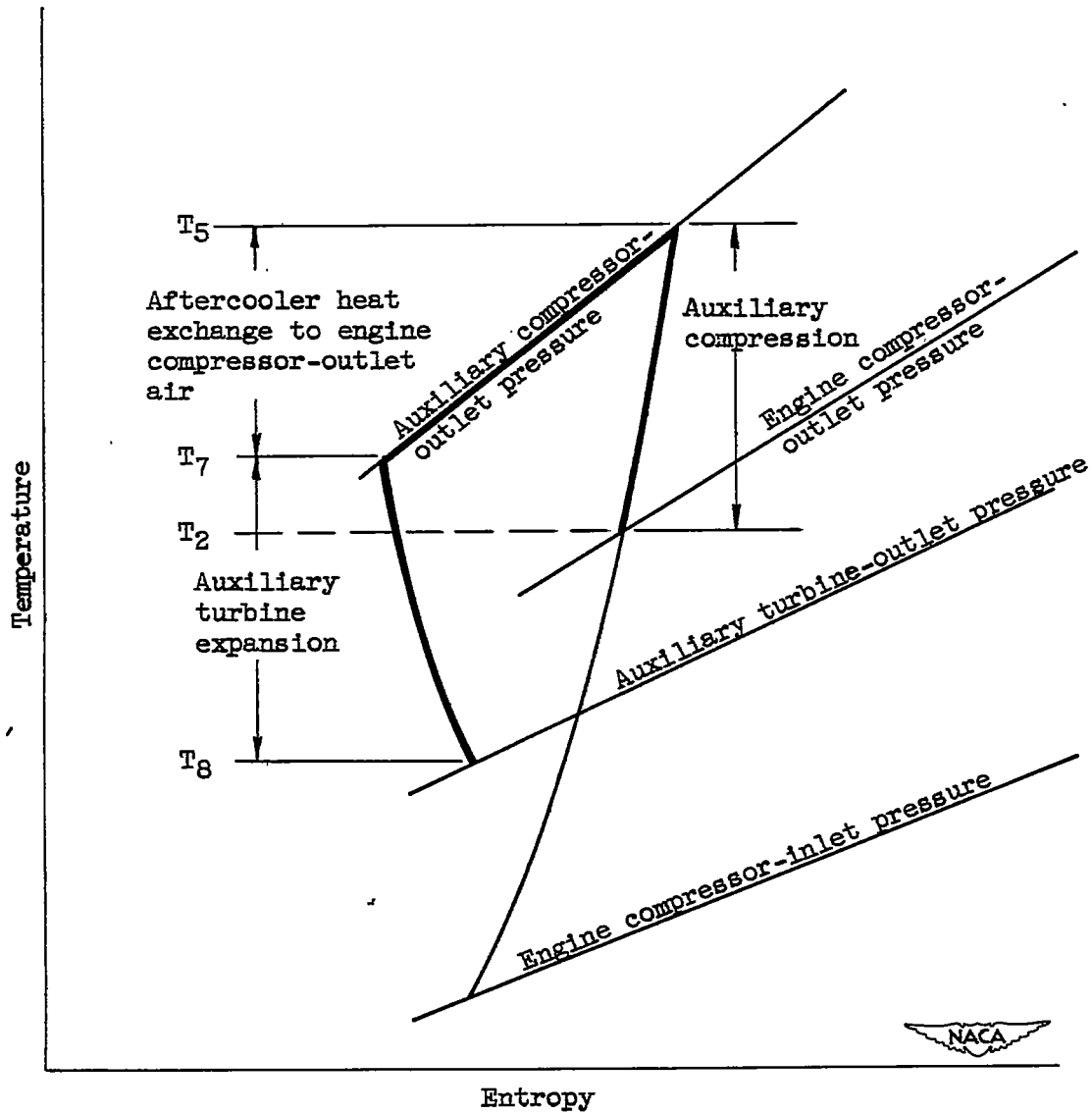
(c) Auxiliary compression, aftercooling by heat rejection at compressor outlet, and expansion in auxiliary turbine.
