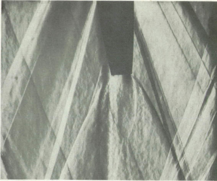
(a) Representative schlieren photograph.
