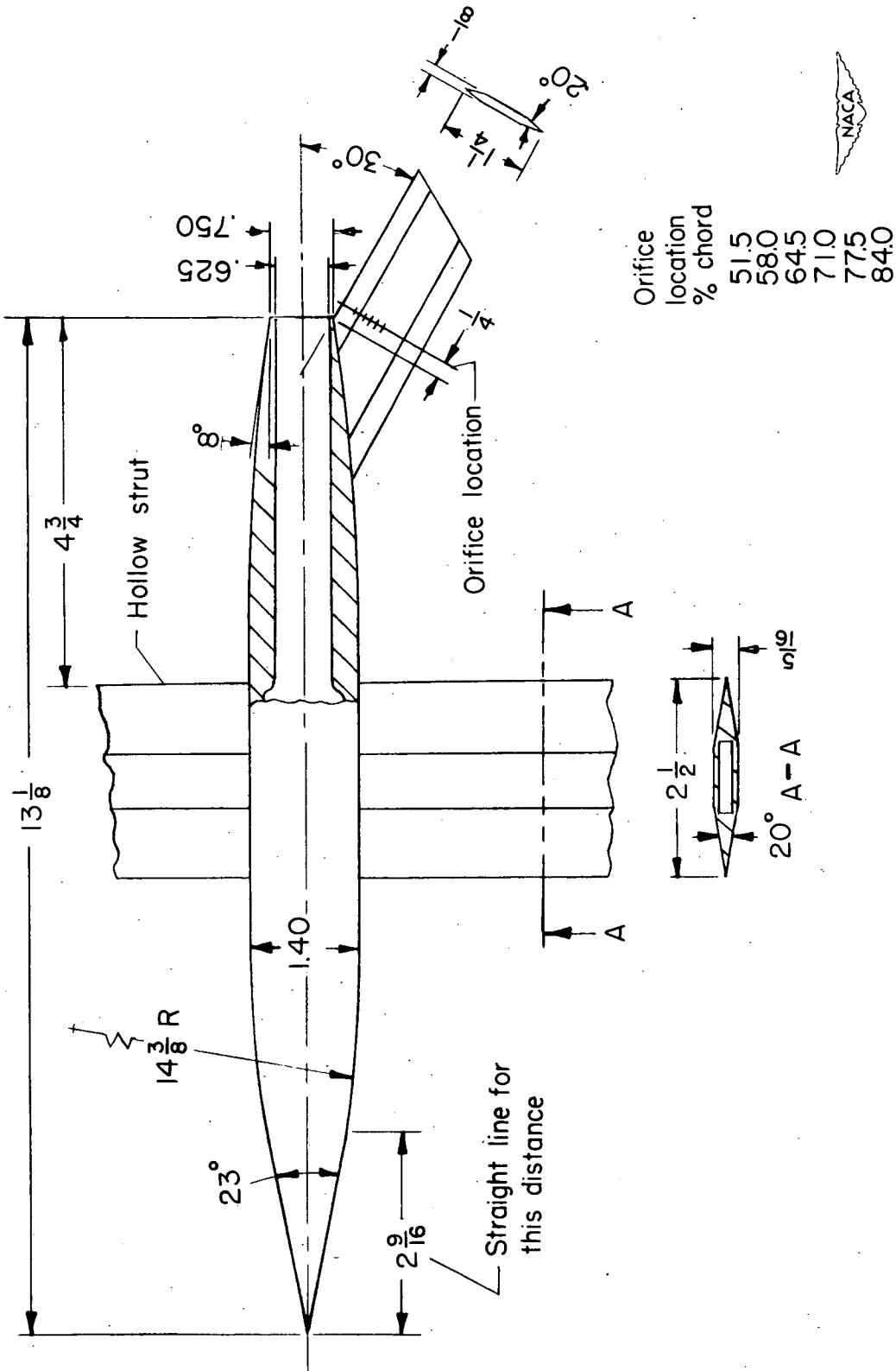
Figure 1.- Jet exhaust model (all dimensions in inches unless otherwise indicated).
