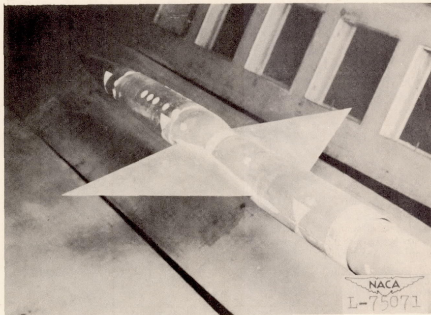
Figure 2.- Front and rear three-quarter views of the indented wing-body combination installed in the Langley 8-foot transonic tunnel.
