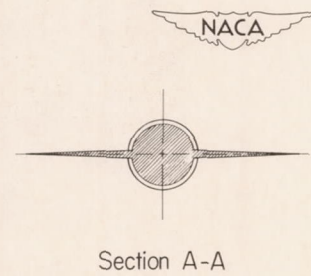
Figure 1.- Plan views and dimensional details of the wing-body combinations investigated. All dimensions are in inches.
