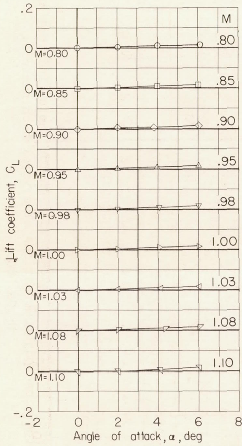
Figure 4.- Basic aerodynamic characteristics for the cylindrical body alone at several Mach numbers.
