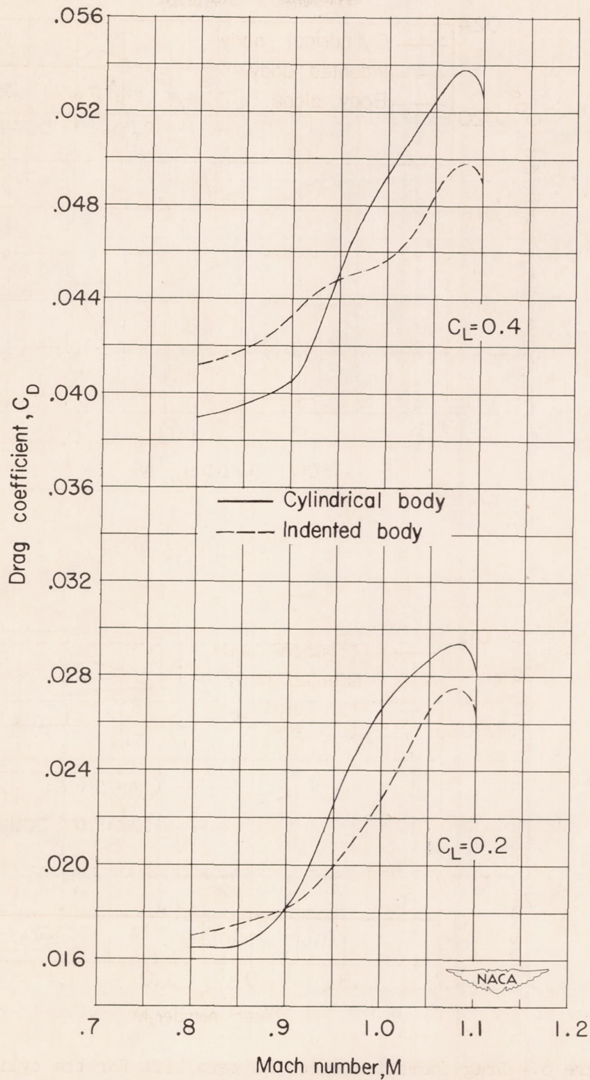
Figure 7.- Drag characteristics at lift coefficients of 0.2 and 0.4 for the wing-body combinations investigated.
