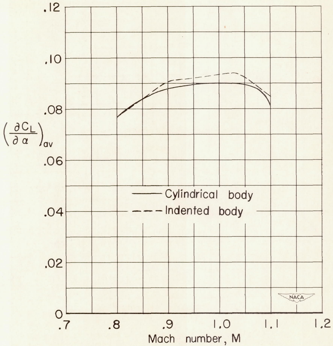
Figure 10.- Average lift-curve slope comparisons for the wing-body combinations.
