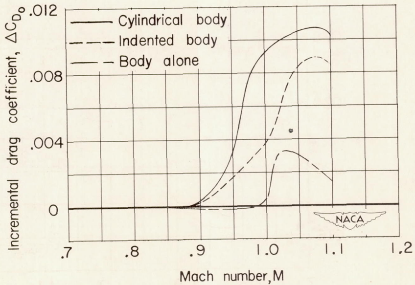
Figure 6.- Drag characteristics at zero lift for the cylindrical and indented wing-body combinations and for the cylindrical body alone. (Data obtained from ref. 1.)
