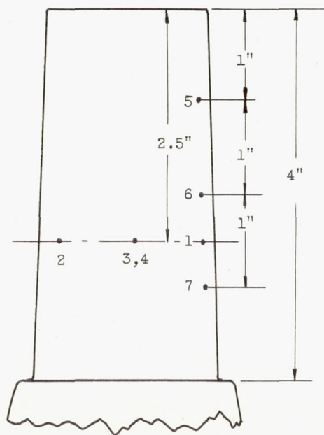
(a) Rotor blade.
