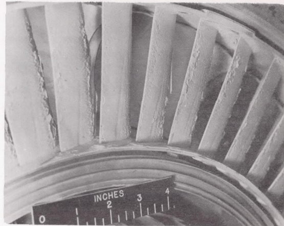
Figure 9. - Stator blades before and after operation with silicone oil, SF-99, added to the fuel.
