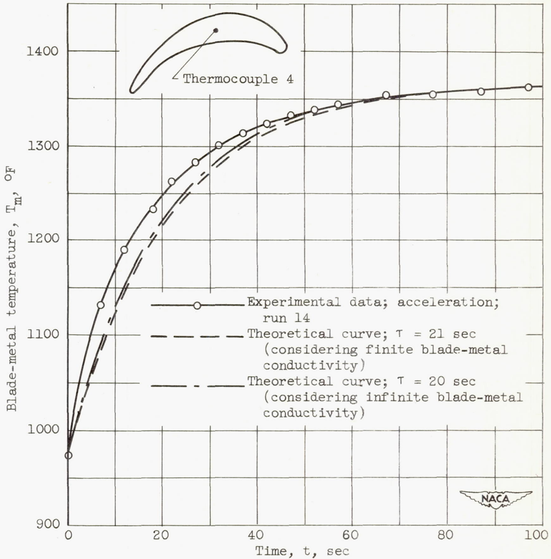
Figure 6. - Comparison of experimental and theoretical time-temperature relations at midchord, midthickness of uncoated rotor blade. Blade-metal initial temperature, 972^{\circ} F; blade-metal final temperature, 1365^{\circ} F.
