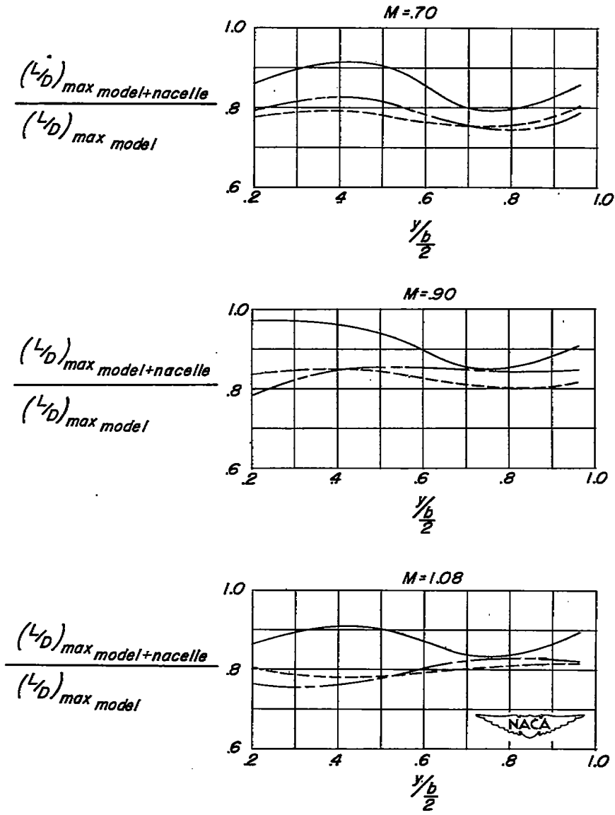
Figure 14.- Variation of the ratios of the maximum lift-drag ratio of the model with nacelle to the maximum lift-drag ratio of the model without nacelle with nacelle spanwise location.
