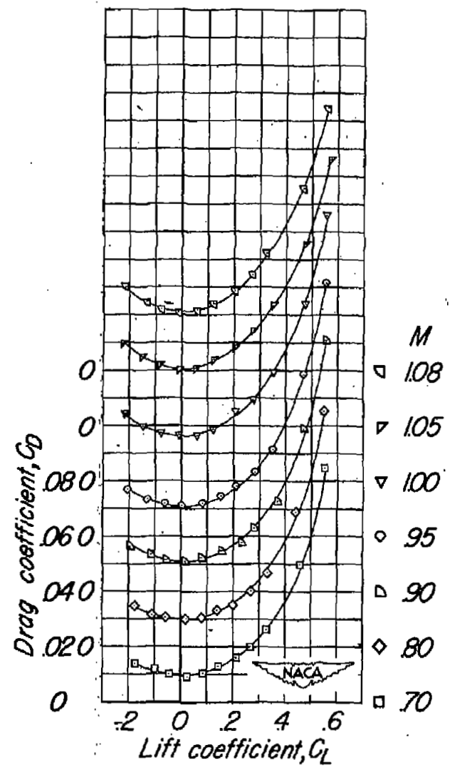
Figure 5.- Aerodynamic characteristics of the semispan wing.
