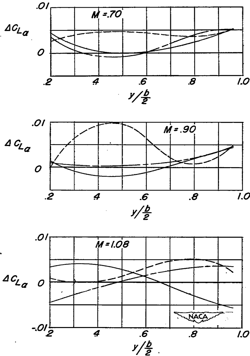
Figure 16.- Variation of the increments in lift-curve slopes with nacelle spanwise location.
