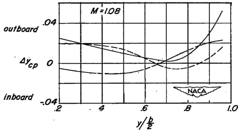
Figure 20.- Variation of the increments in lateral center-of-pressure locations with nacelle spanwise location as obtained from figure 19.
