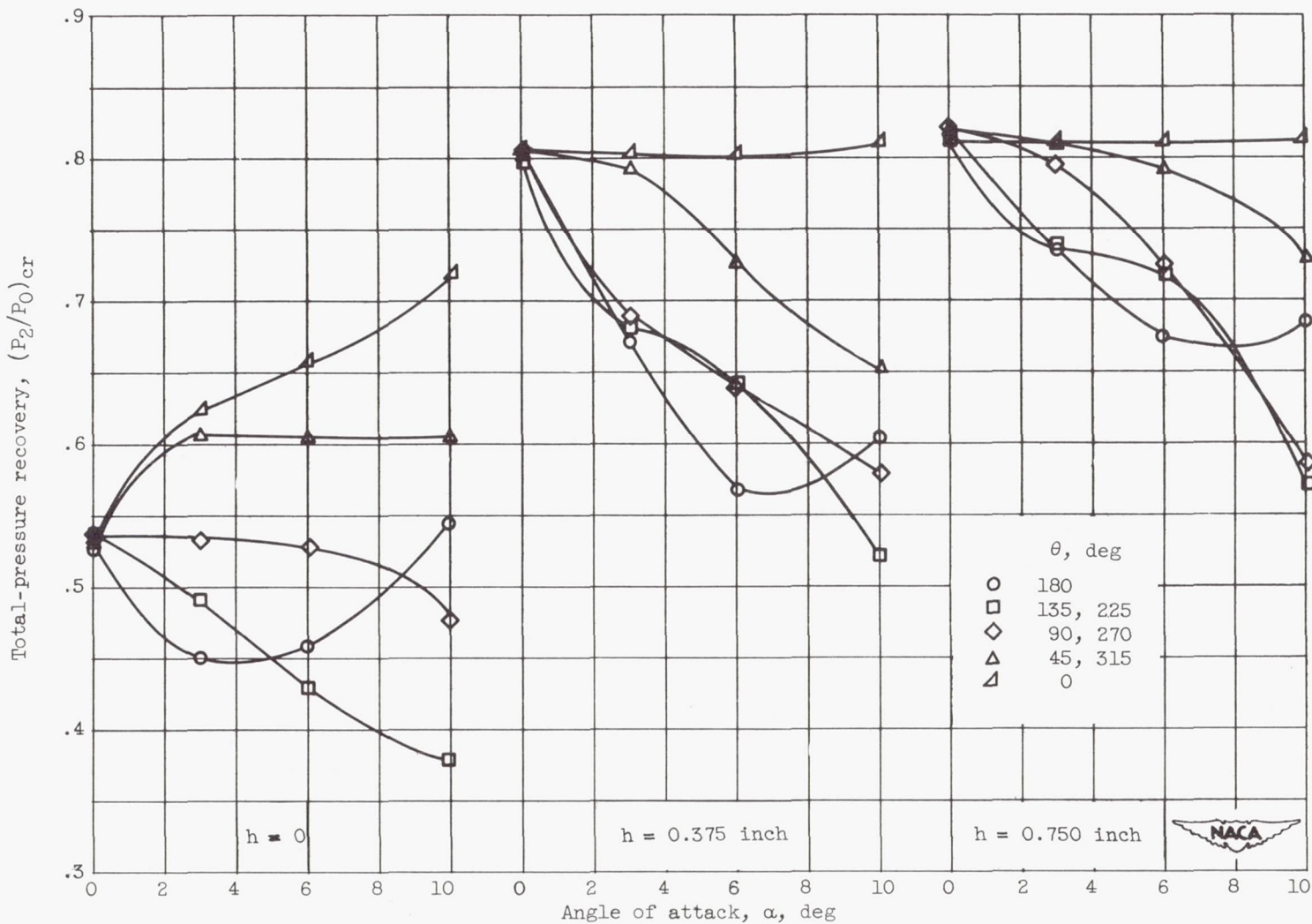
(a) Free-stream Mach number, 1.99.
