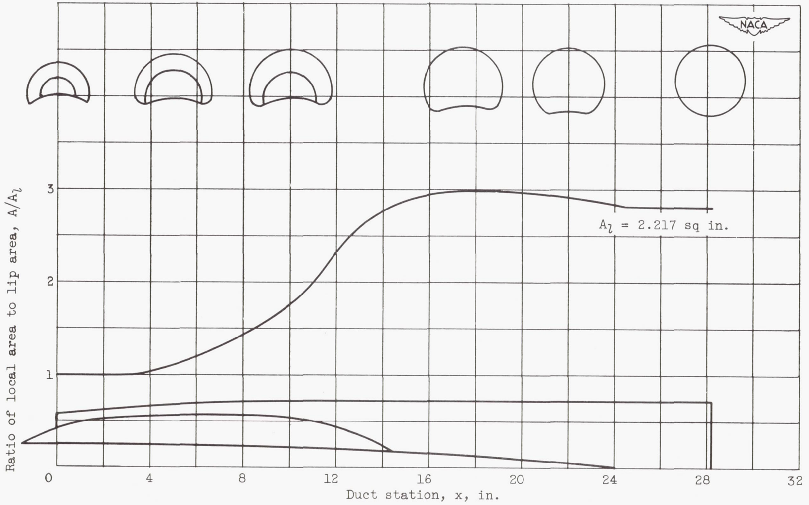
Figure 4. - Area variation of inlet.
