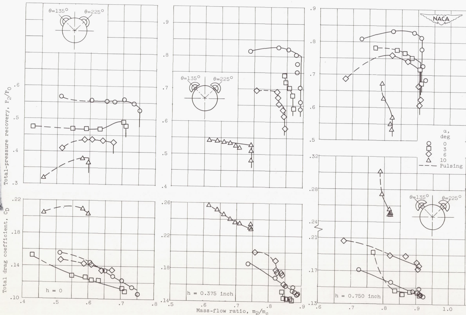
(a) Free-stream Mach number, 1.99.
