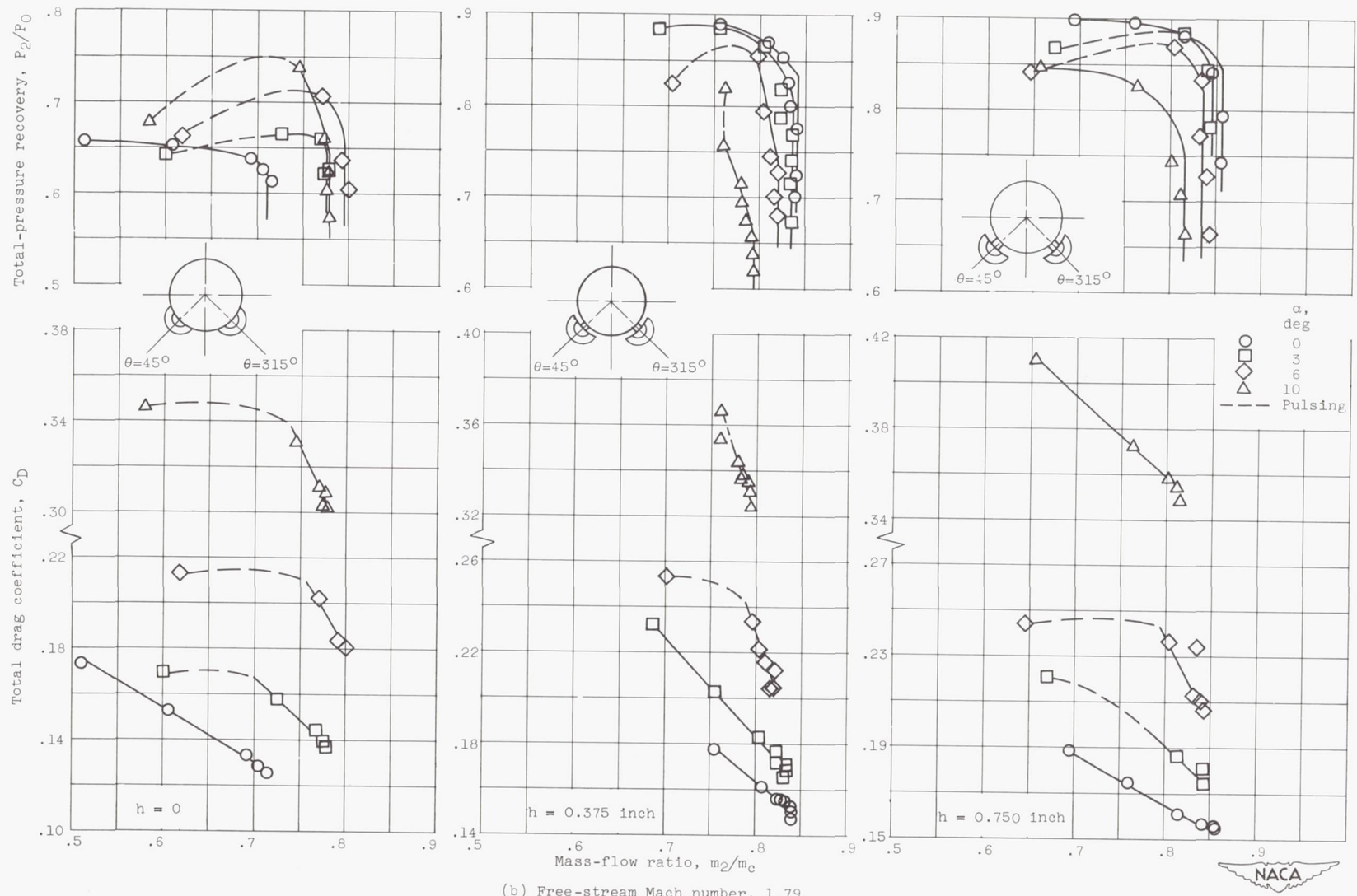
(b) Free-stream Mach number, 1.79. Figure 10. - Continued. Angle of attack characteristics of RM-10 inlet configuration. \theta = 45^\circ and 315^\circ .
