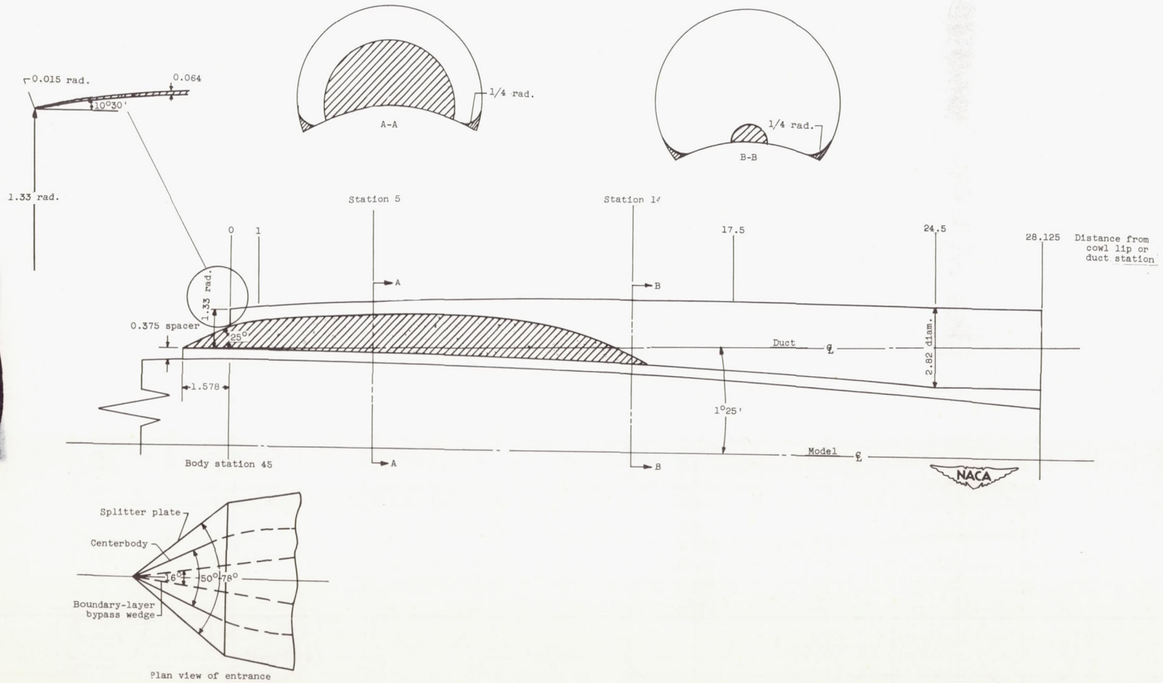
Figure 3. - Schematic diagram of inlet. (All dimensions are in inches.)
