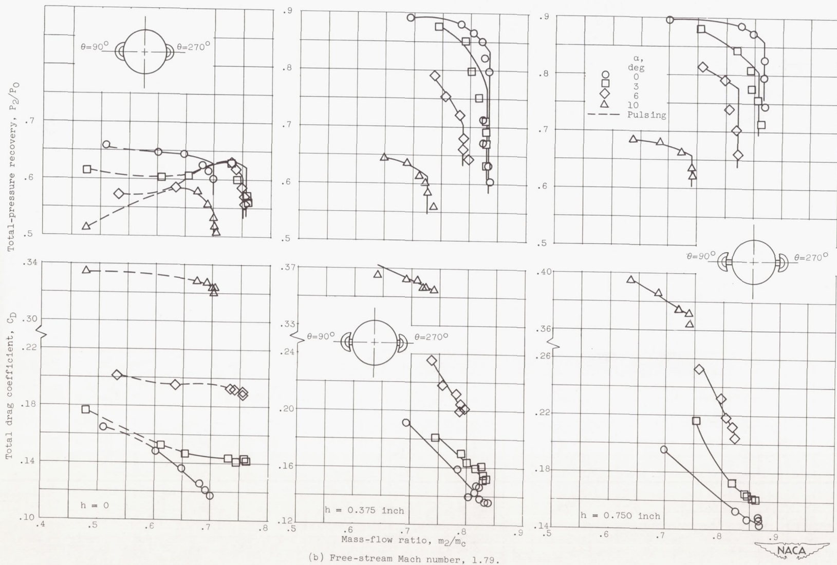
Figure 9. - Continued. Angle of attack characteristics of RM-10 inlet configuration. \theta = 90^\circ and 270^\circ .
