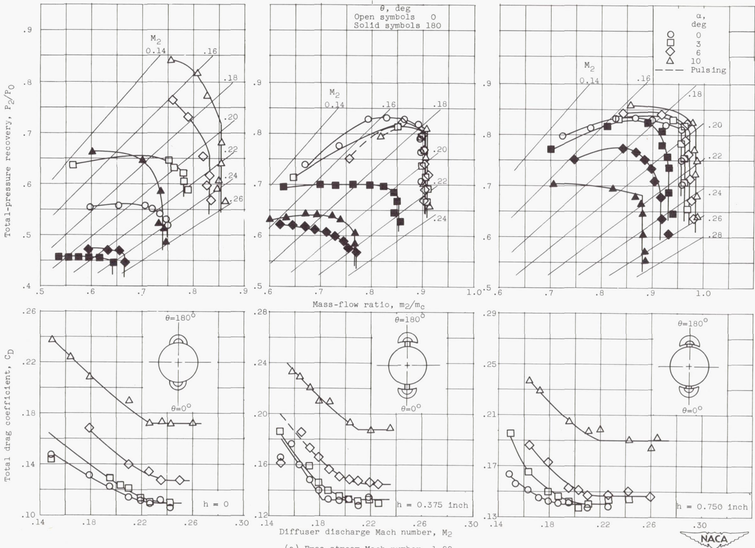
Figure 11. - Angle of attack characteristics of RM-10 inlet configuration. \theta = 0^\circ and 180^\circ .
