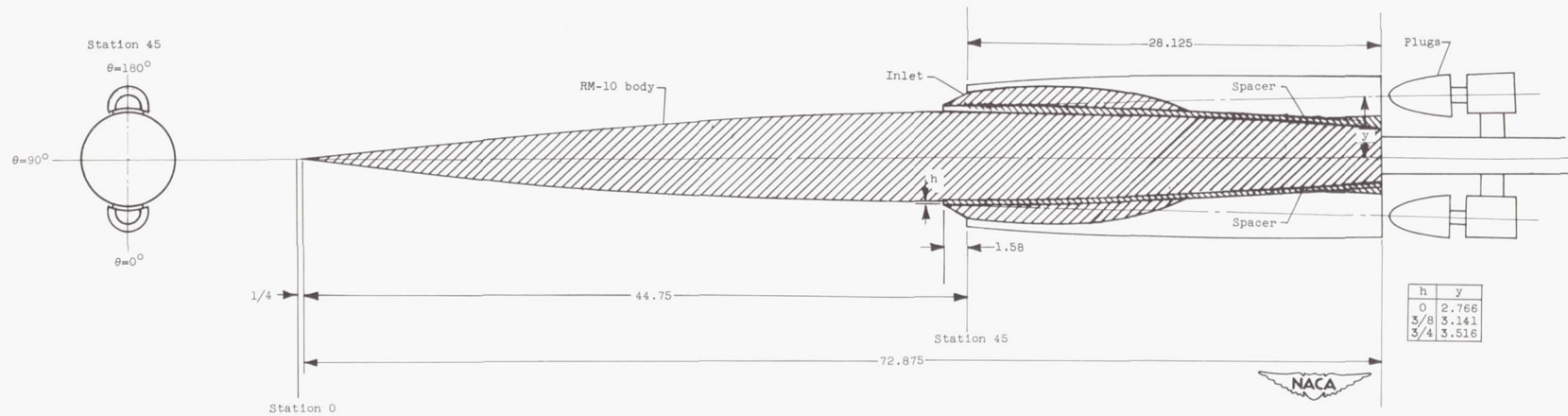
Figure 2. - Schematic diagram of twin scoop inlets mounted on RM-10 body. (All dimensions are in inches.)
