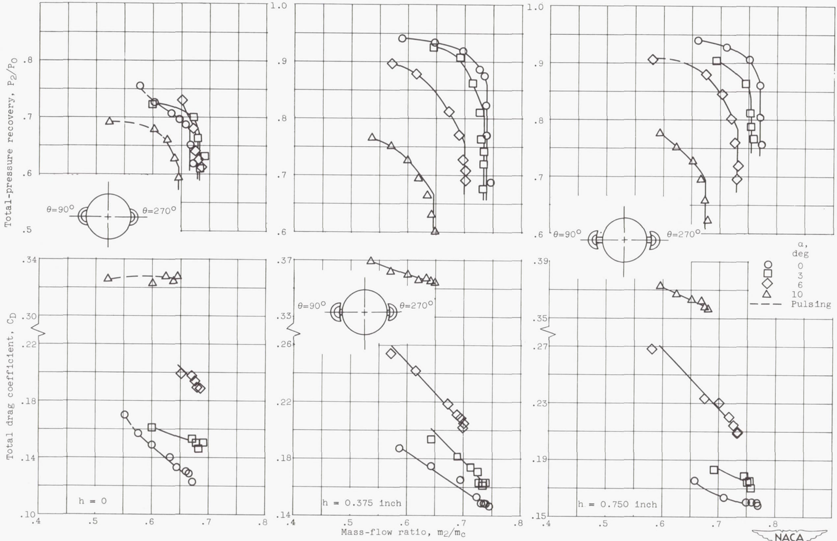
(c) Free-stream Mach number, 1.49.
