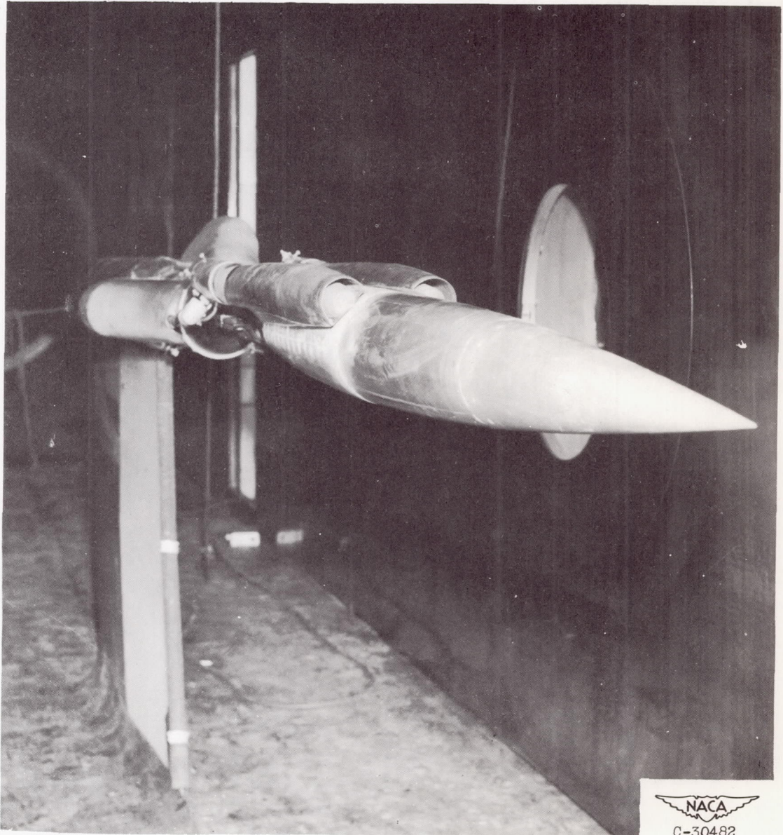
Figure 1. - Photograph of model installation.
