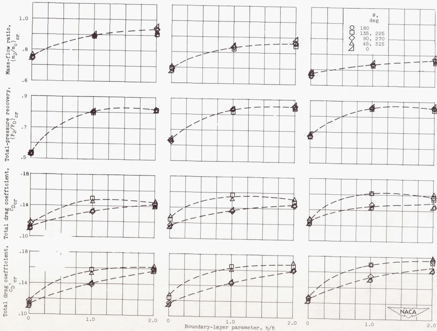
(b) Free-stream Mach number, 1.79.
