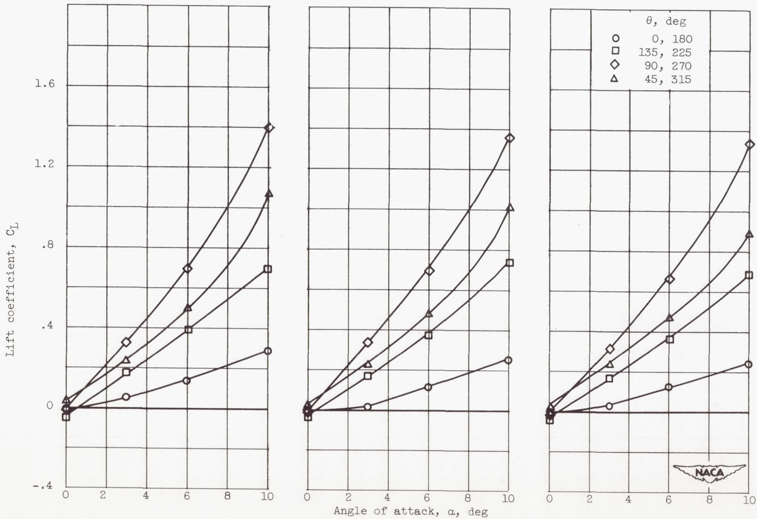
(a) Free-stream Mach number, 1.99. (b) Free-stream Mach number, 1.79. (c) Free-stream Mach number, 1.49.
