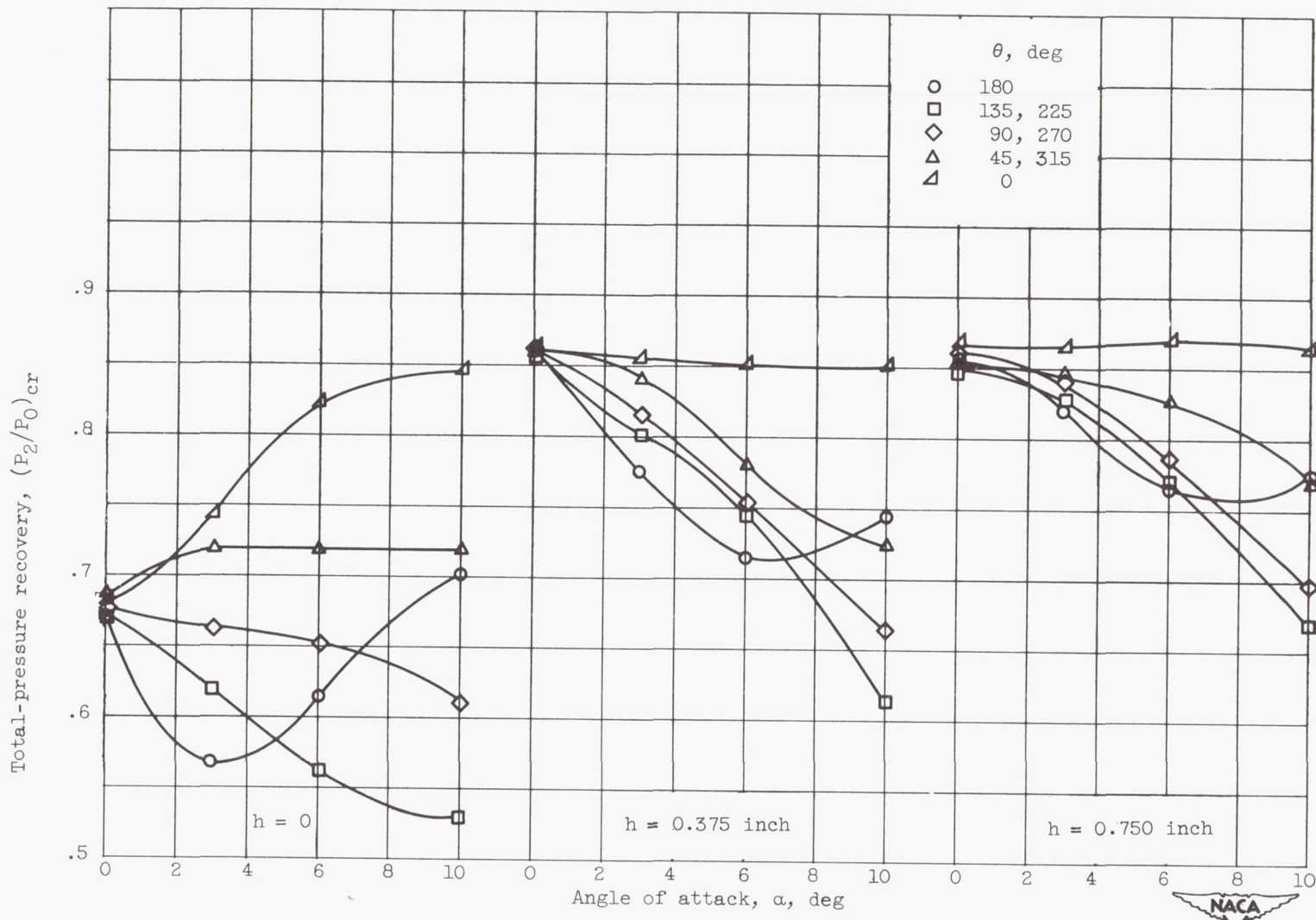
(c) Free-stream Mach number, 1.49.
