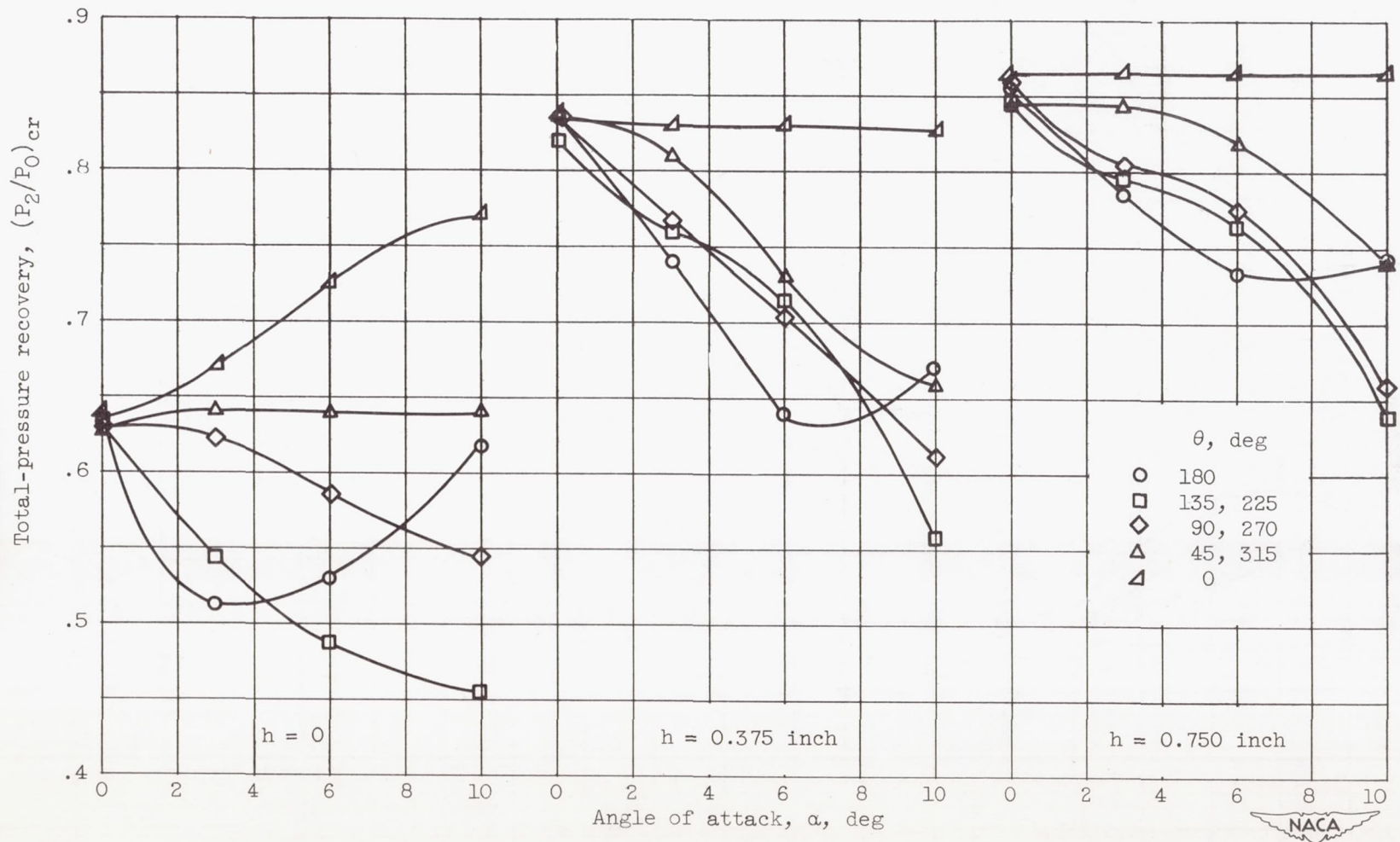
(b) Free-stream Mach number, 1.79.
