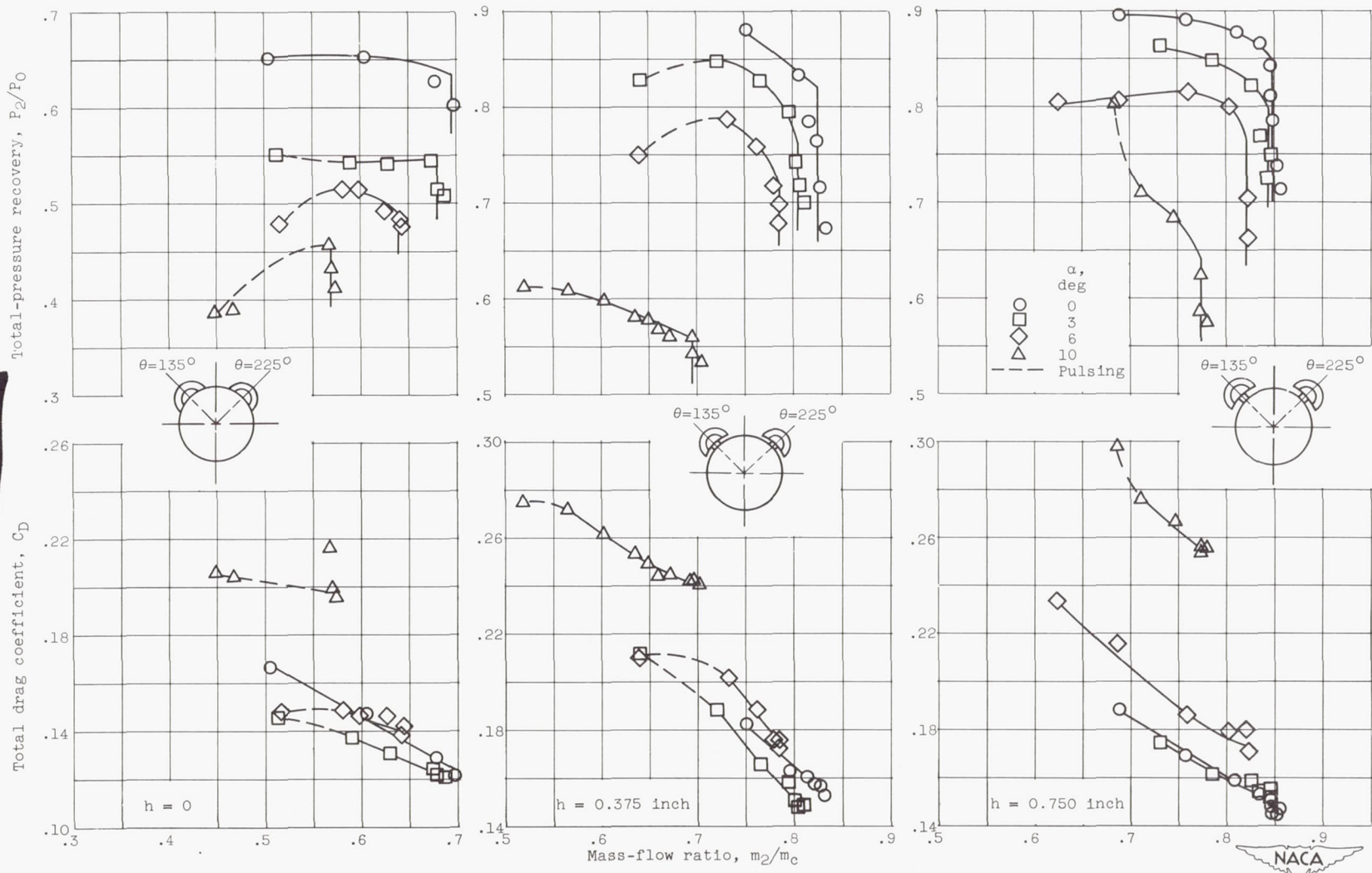
(b) Free-stream Mach number, 1.79.
