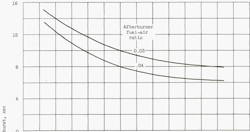
(a) Autoignition.
