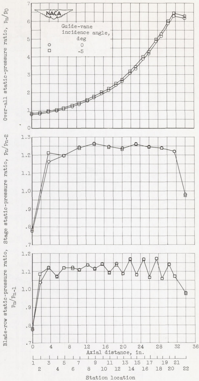
Figure 6. - Static-pressure-ratio distributions for 0^\circ and -5^\circ guide-vane incidence at over-all static-pressure ratio of approximately 6.25 at design speed.
