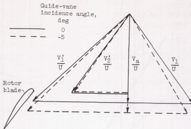
(a) Radial position a.
