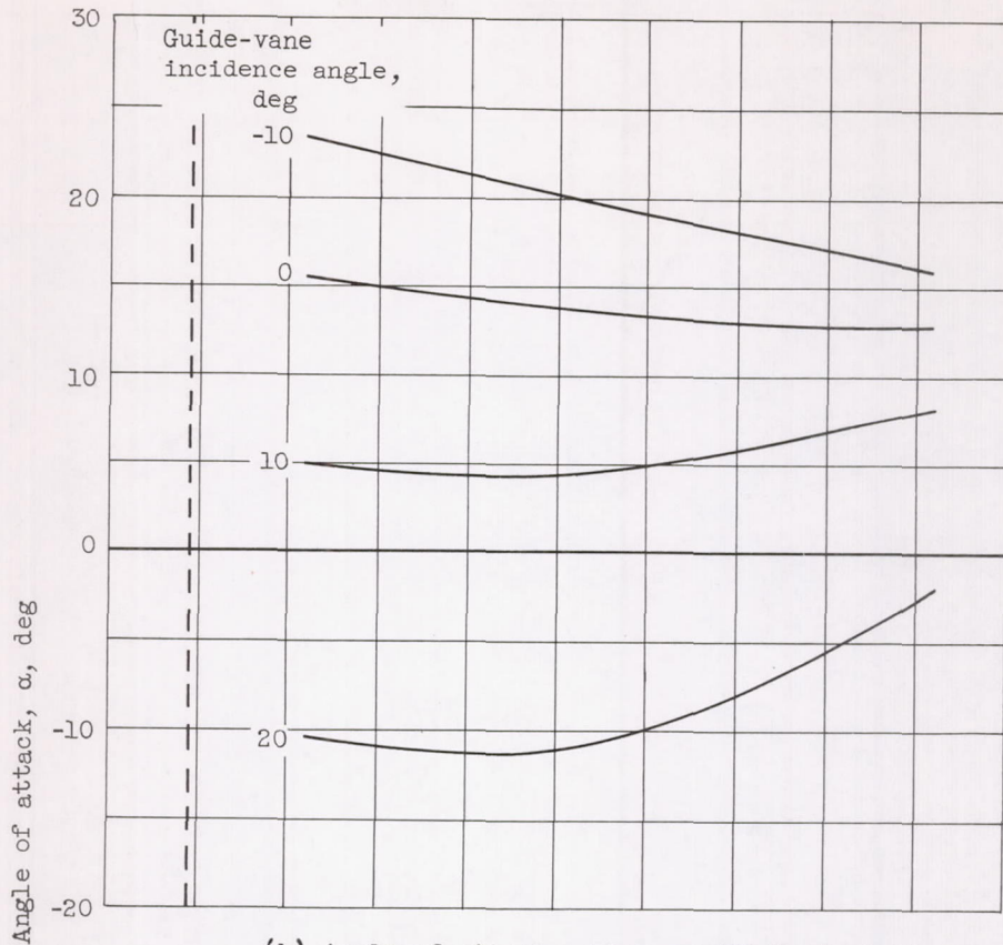
(b) Angle of attack. Flow coefficient, 0.58.
