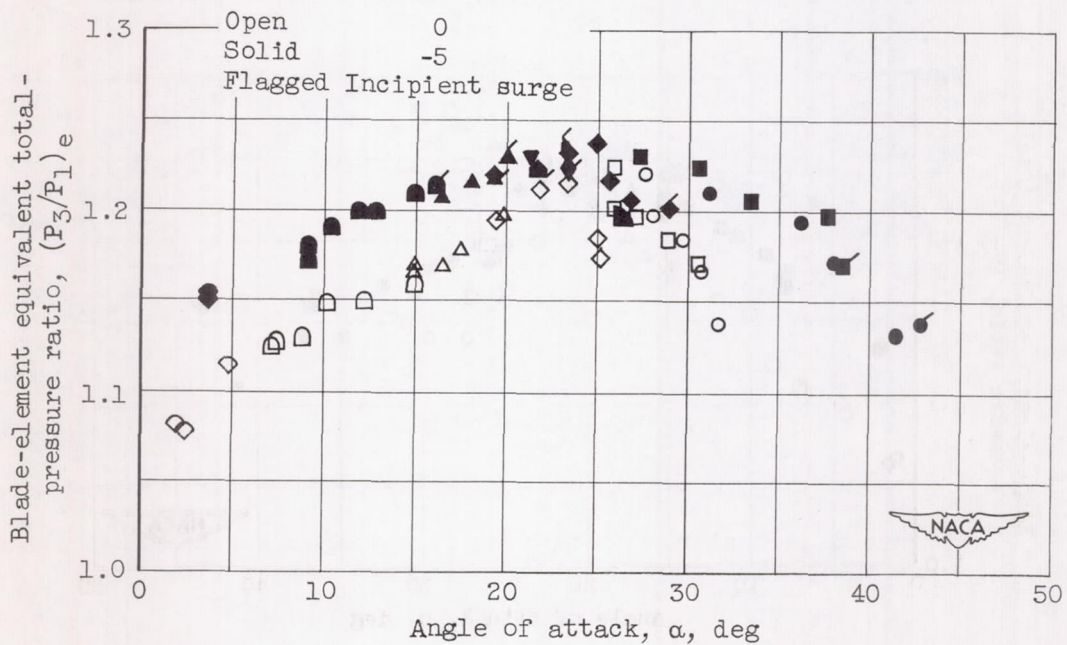
(c) Radial position c.
