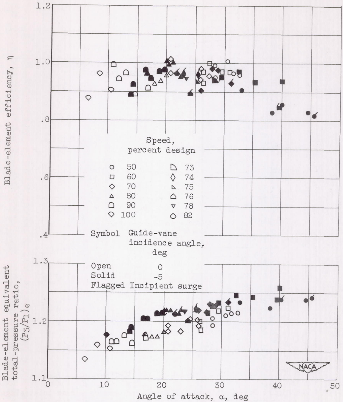
(e) Radial position e.
