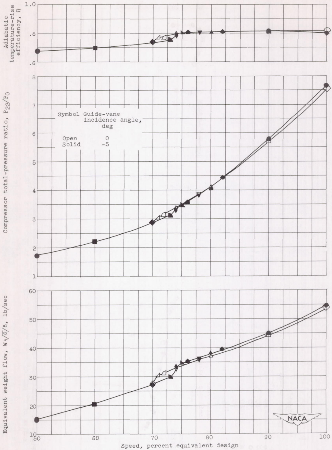
(c) Adiabatic temperature-rise efficiency, compressor total-pressure ratio, and equivalent weight flow at surge against percent of equivalent design speed.
