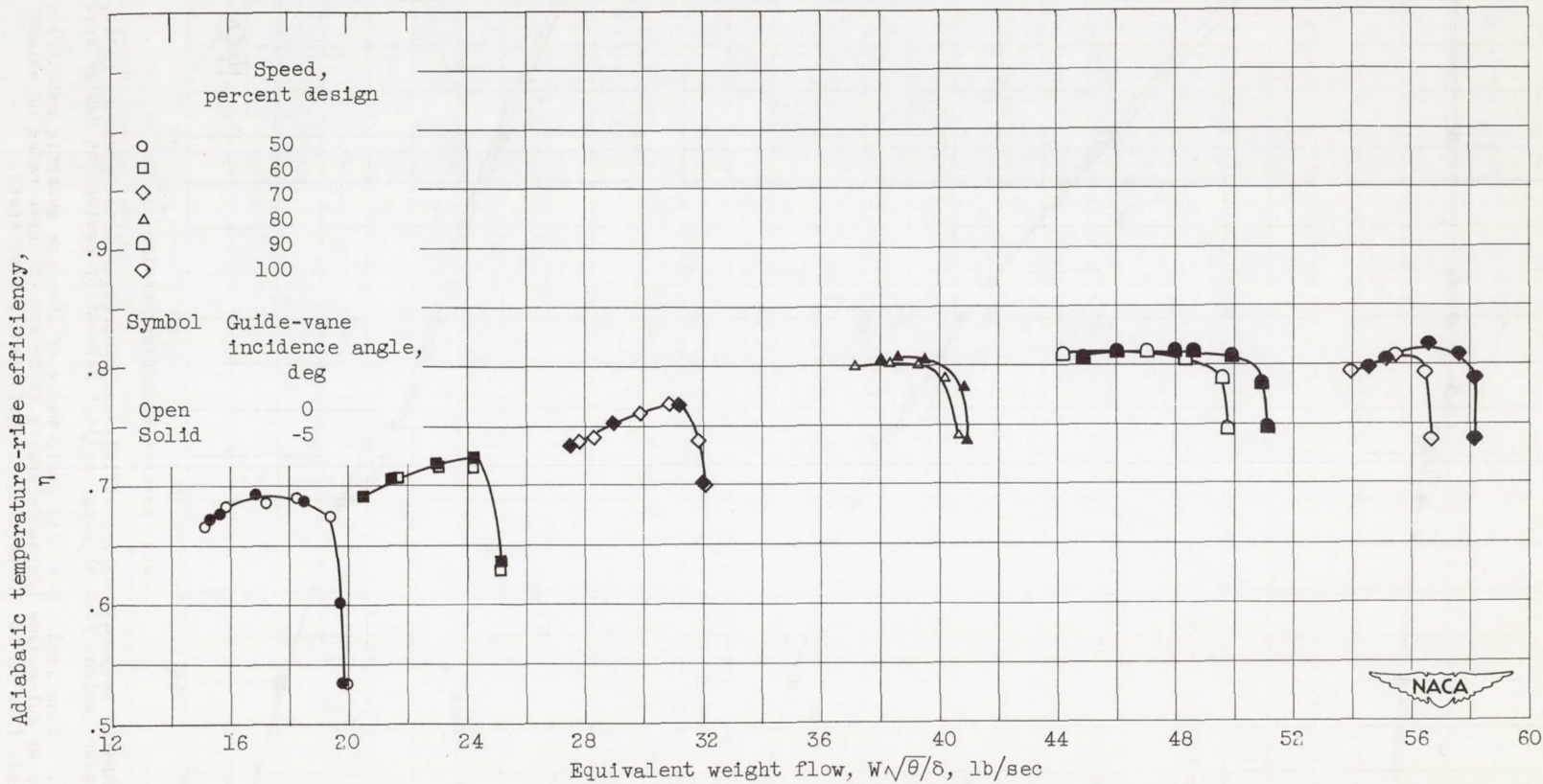
(b) Adiabatic temperature-rise efficiency.
