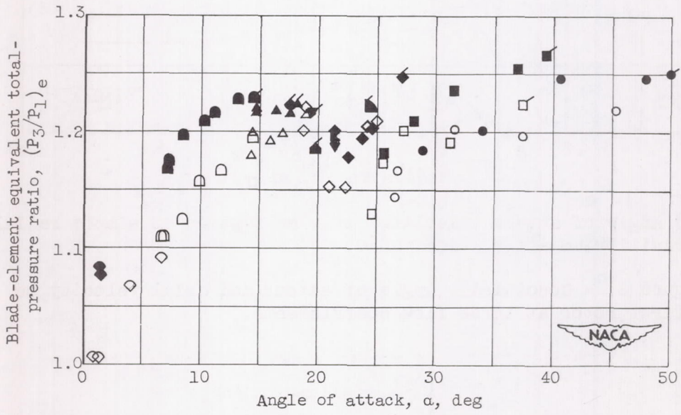
(a) Radial position a.
