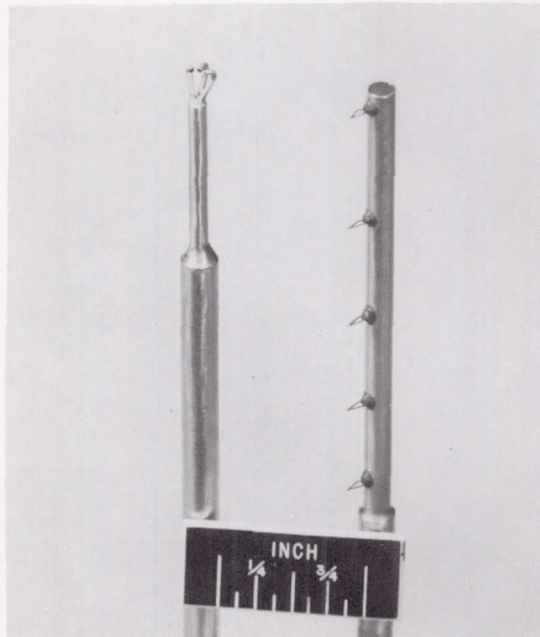
(a) Combination claw total-pressure survey probe.
