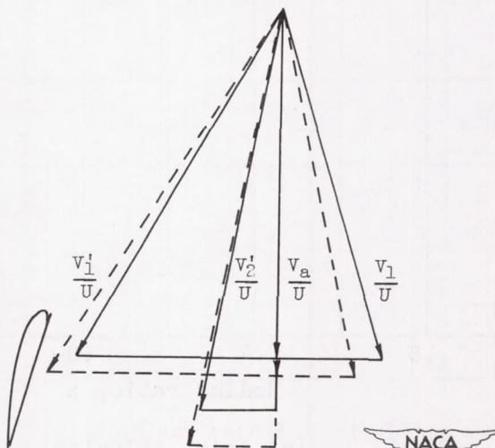
(c) Radial position e.
