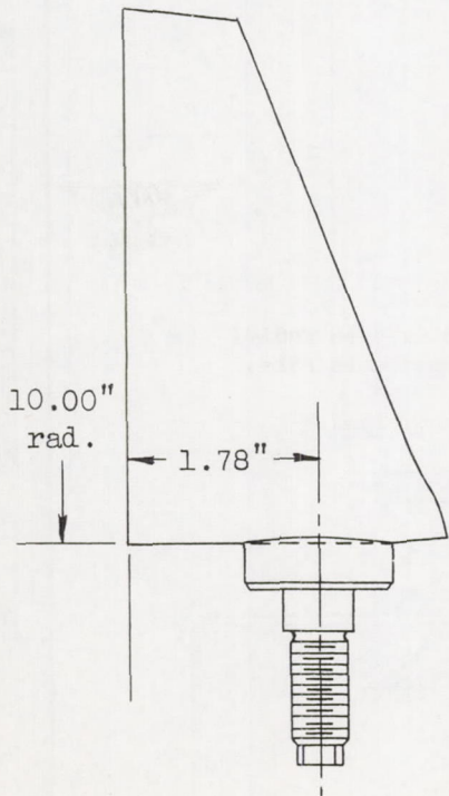
Figure 2. - Inlet guide vane. Number 14-gage (0.083) mild steel.
