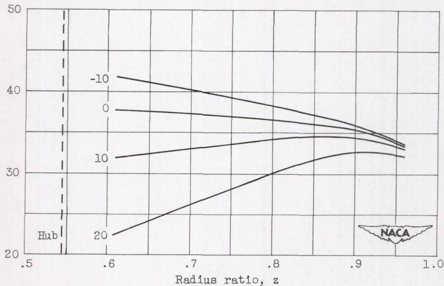
(c) Angle of attack. Flow coefficient, 0.31.
