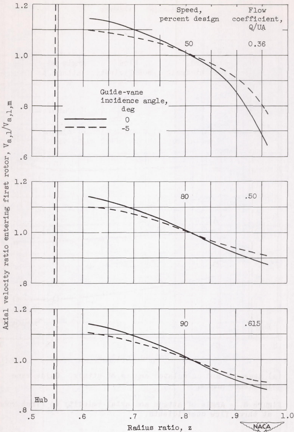
(b) Axial-velocity distribution.
