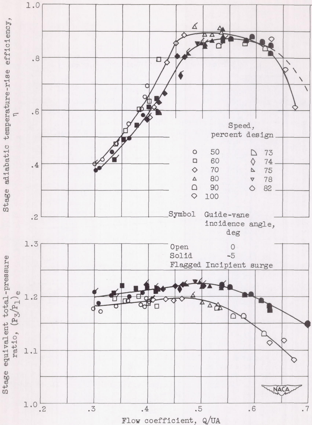
Figure 7. - Comparison of inlet-stage performance for 0° and -5° guide-vane incidence angles over range of weight flow at speeds from 50 to 100 percent of equivalent design speed.
