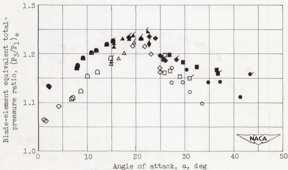
(b) Radial position b.
