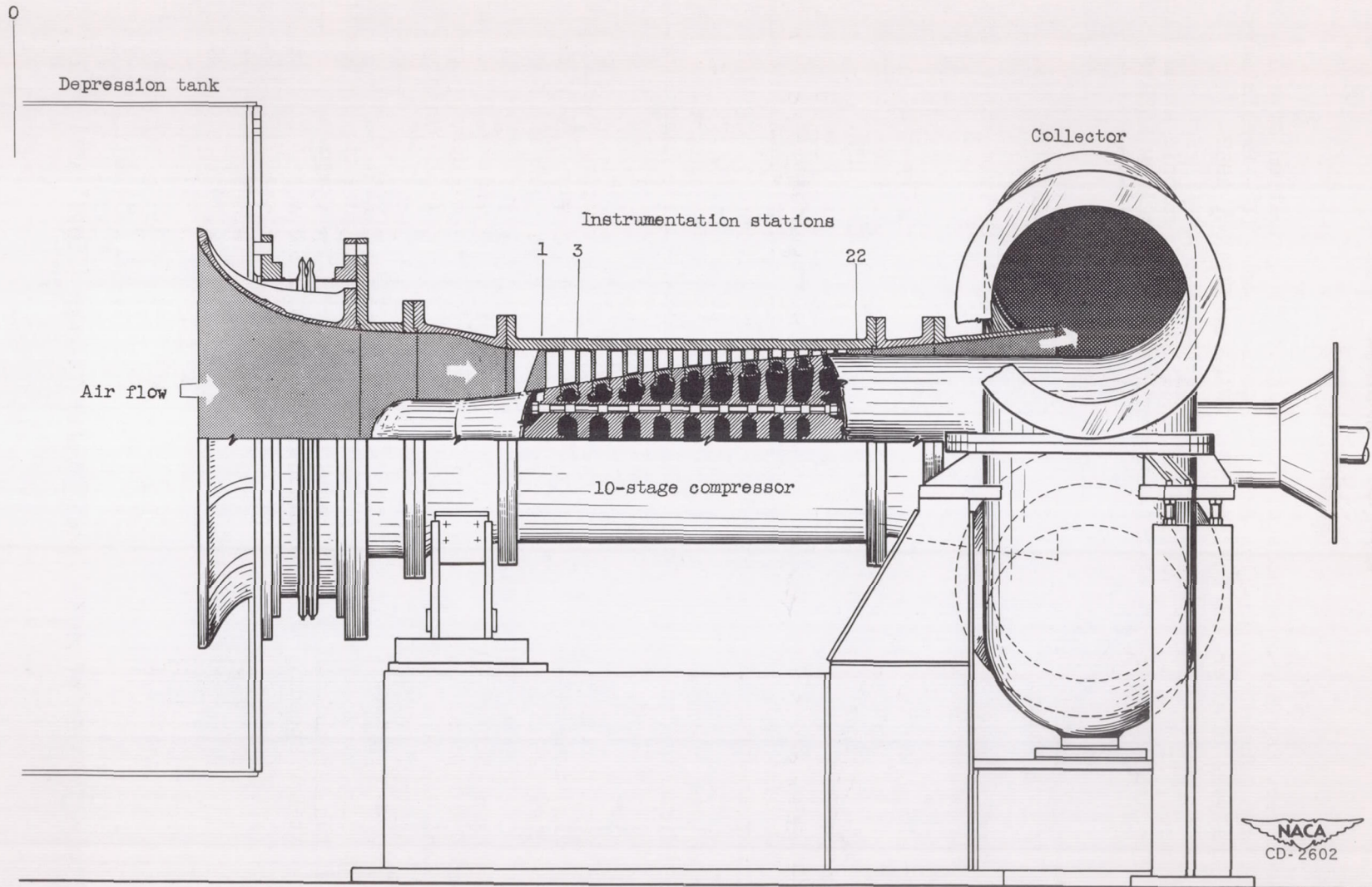
Figure 1. - Cross-sectional view of 10-stage compressor showing instrumentation stations.
