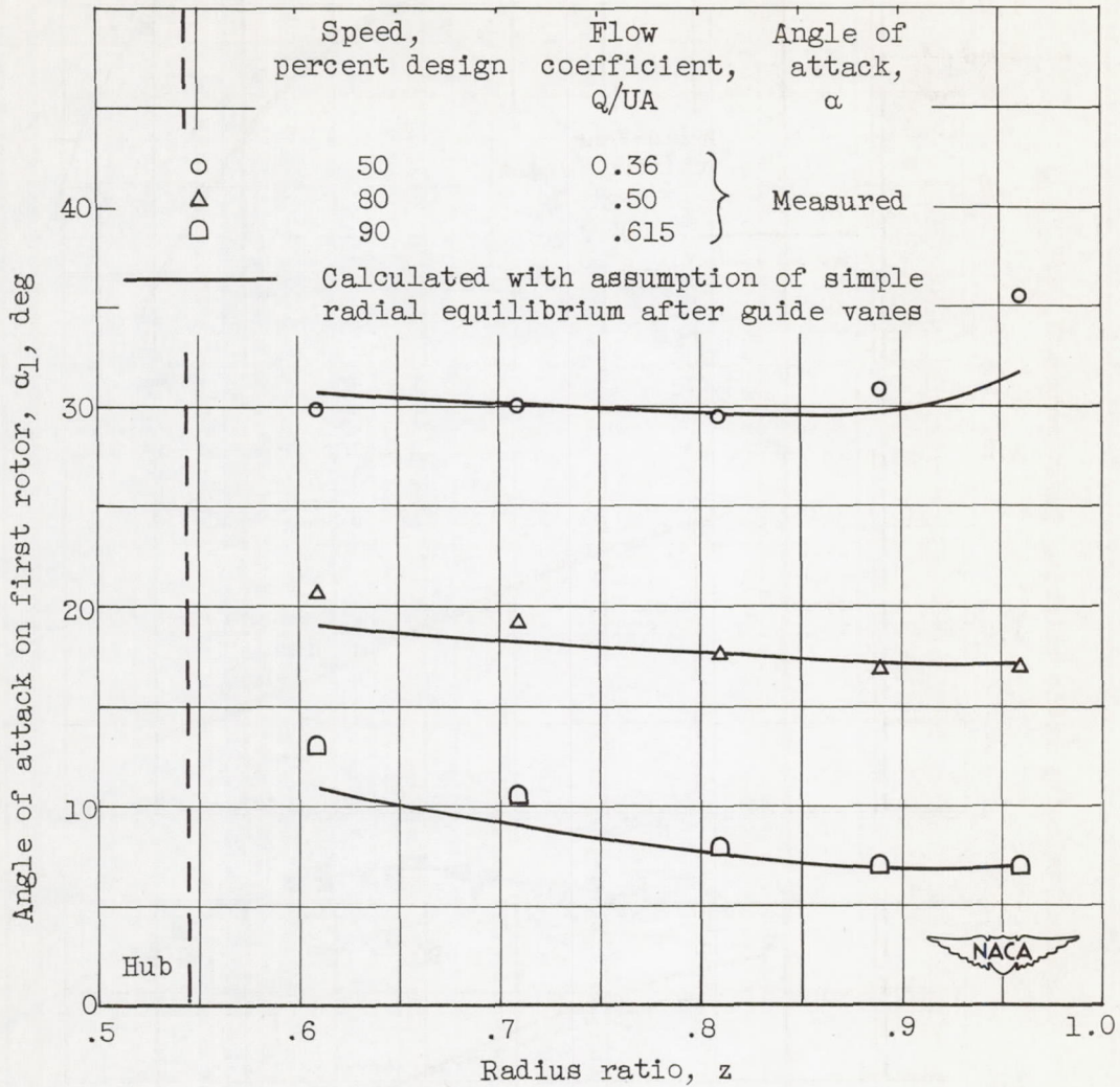
(a) Measured and calculated angles of attack. Guide-vane incidence angle, 0^\circ
