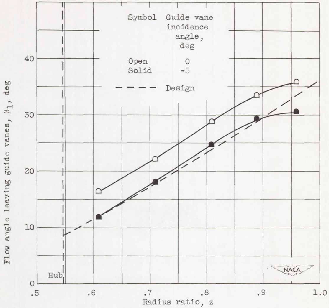
Figure 4. - Comparison of radial distribution of flow angle leaving guide vanes for 0° and -5° guide-vane incidence angles. Speed, 90-percent design; flow coefficient, 0.615.
