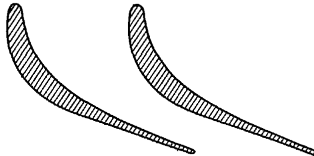
Tip, r/r_t = 1.00
