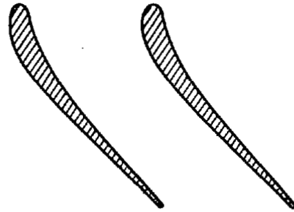
r/r_t = 0.78
