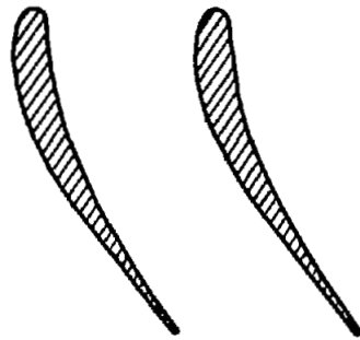
Hub, r/r_t = 0.67
