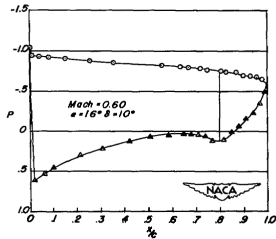
(a) M = 0.60. Concluded.
