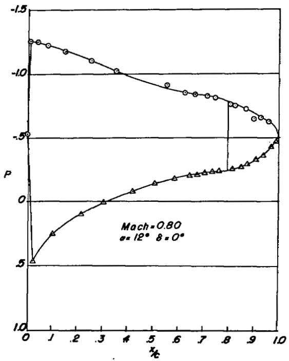
(b) M = 0.80. Concluded.
