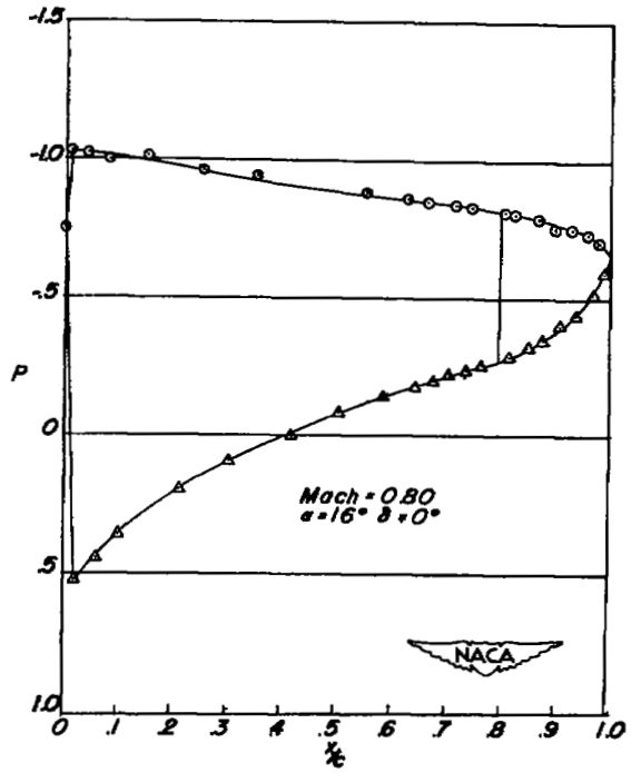
(b) M = 0.80. Concluded.
