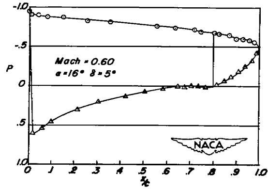
(a) M = 0.60. Concluded.
