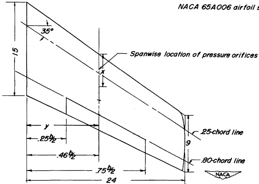
Figure 1.- Geometric characteristics of the 35° sweptback wing equipped with a flap-type aileron. All dimensions are in inches unless otherwise noted.
