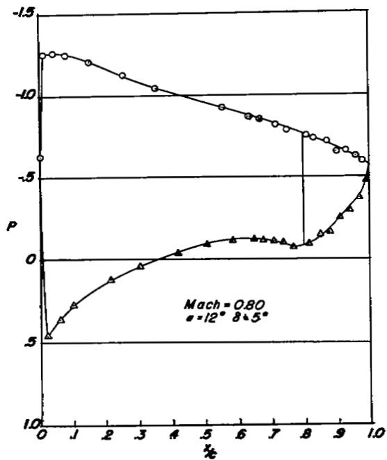
(b) M = 0.80 . Concluded.
