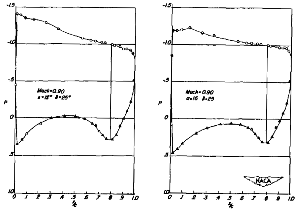
(c) M = 0.90 . Concluded.
