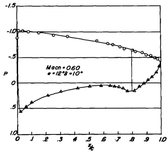
(a) M = 0.60. Concluded.
