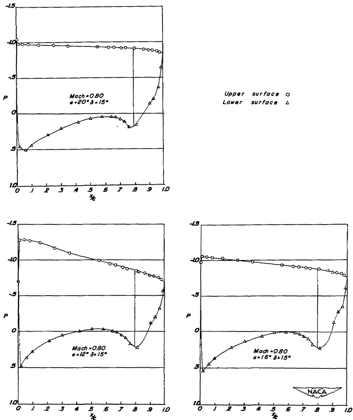
(b) M = 0.80. Concluded.
