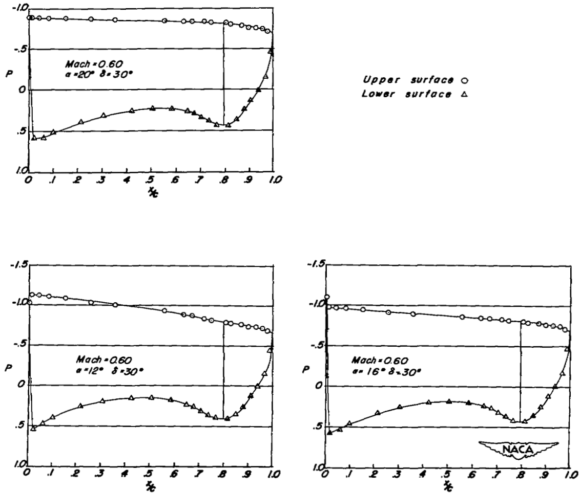
(a) M = 0.60 . Concluded.
