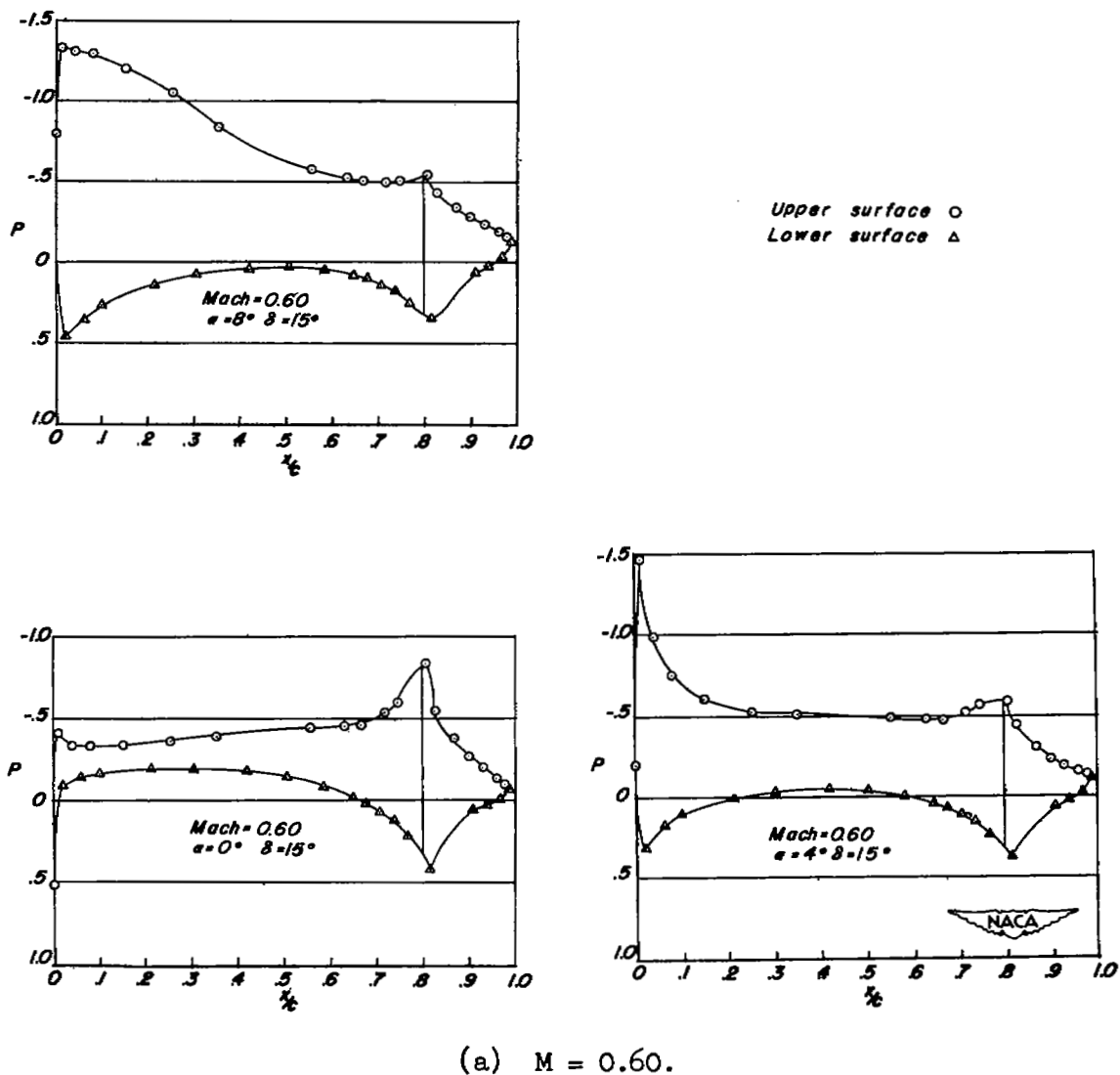
Figure 11.- Chordwise pressure distribution over a 35^\circ sweptback wing, at the 46-percent-semispan station, equipped with a flap-type aileron. \delta = 15^\circ .
