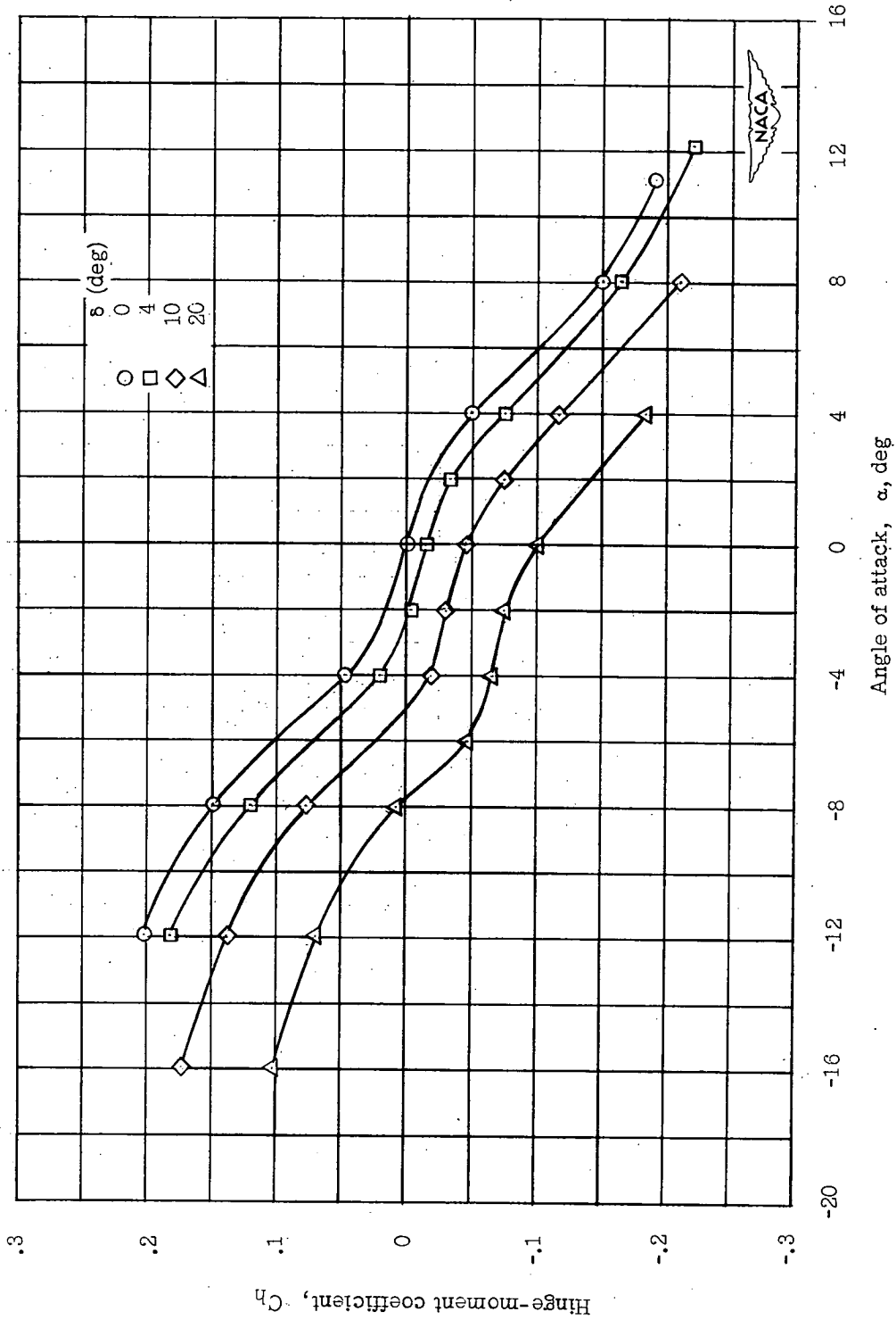
(b) M = 1.62 .
