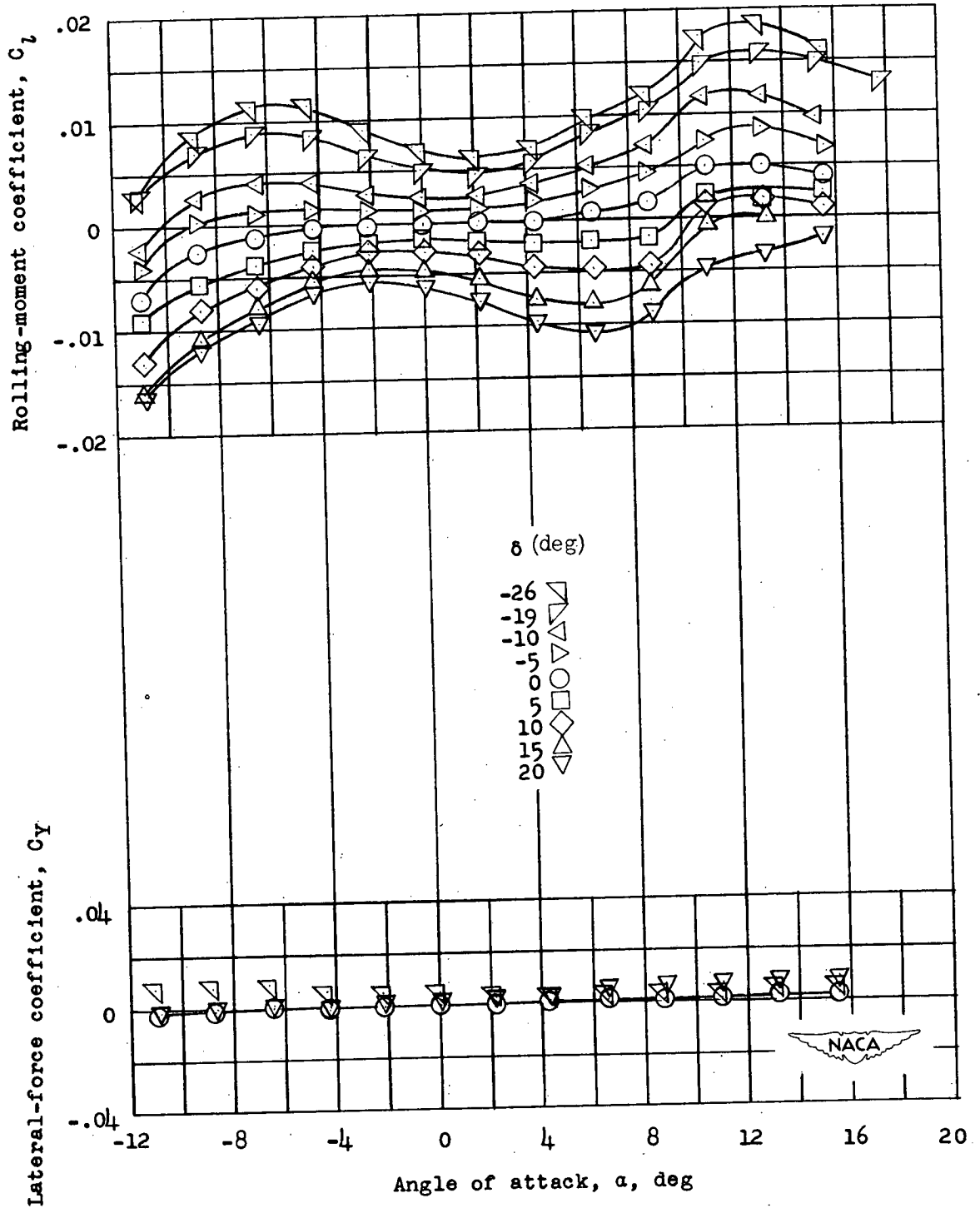
(h) M = 0.9 ; R = 9.3 \times 10^6 .
