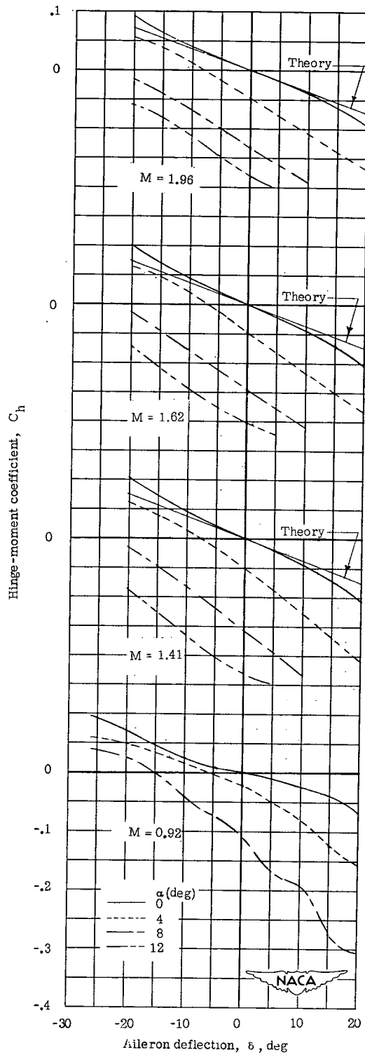
(b) Mach numbers from 0.92 to 1.96.
