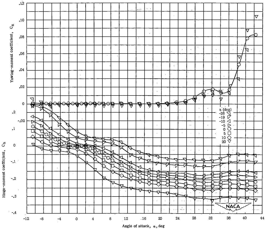
(a) M = 0.15 ; R = 9 \times 10^6 .
