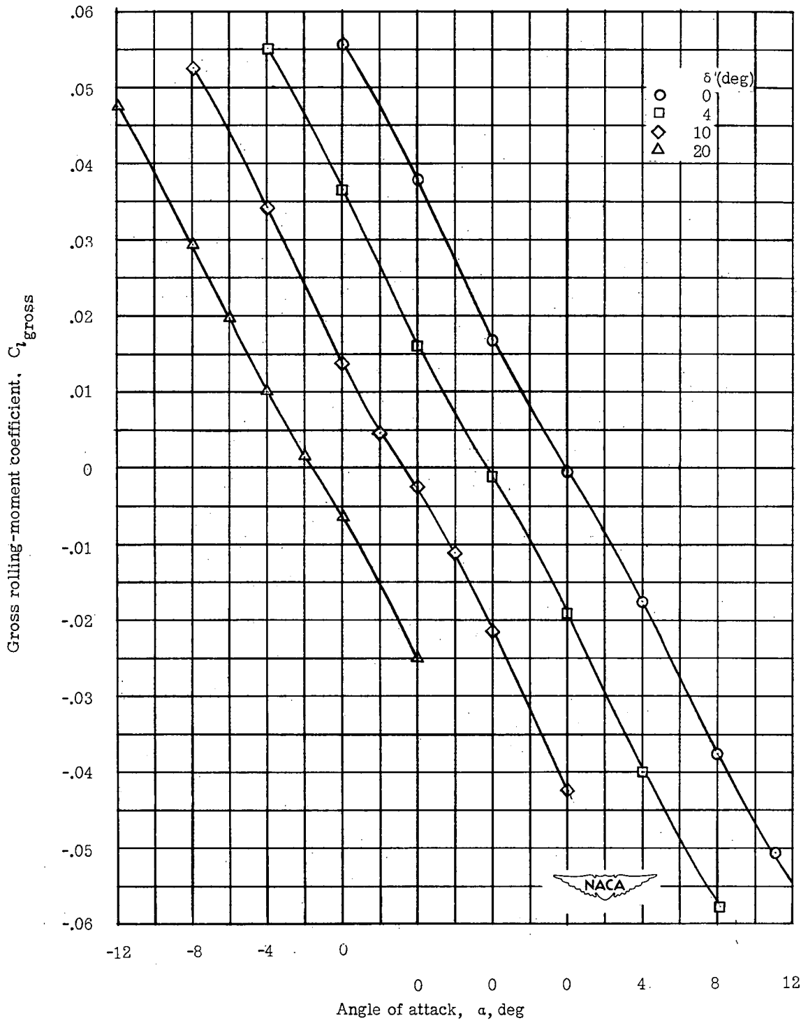
(a) M = 1.41 .
