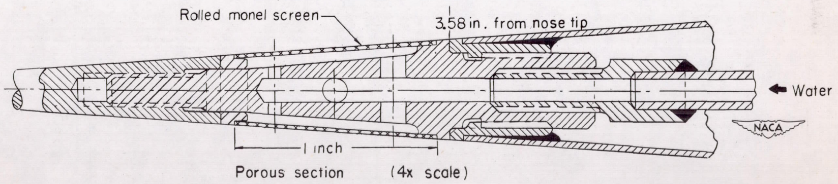
Figure 2.- Diagrammatic sketch of test model illustrating cooling mechanism.
