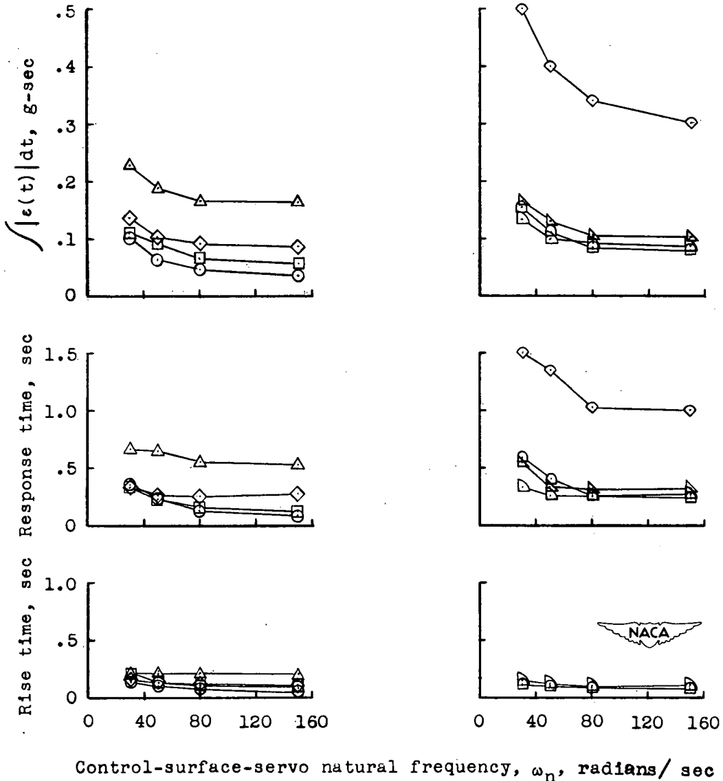
Figure 7.- Normal-acceleration transient characteristics, \int |e(t)| dt , rise time, and response time, in response to a step input n_1(t) plotted against control-surface-servo natural frequency. Static margin equals 0.564\bar{c} at M = 1.6 .
