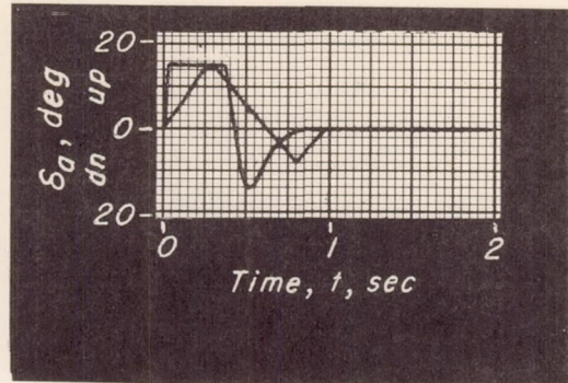
Figure 12.- Optimum responses for \dot{\delta}_{aL} of 50^\circ/\text{sec} and 300^\circ/\text{sec} ; \delta_{aL} = \pm 15^\circ .
