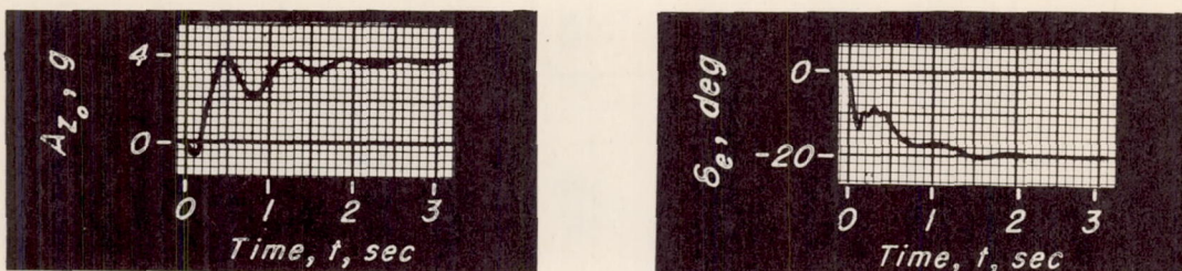
Figure 5.- Optimum response with given form of stabilizing network (no time lag); \dot{\delta}_{eL} = 100^\circ/\text{sec} .
