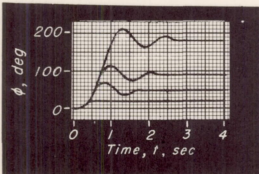
Figure 13.- Effect of input. Optimized for \phi of 45^\circ ; \dot{\delta}_{aL} = 150^\circ/\text{sec} .
