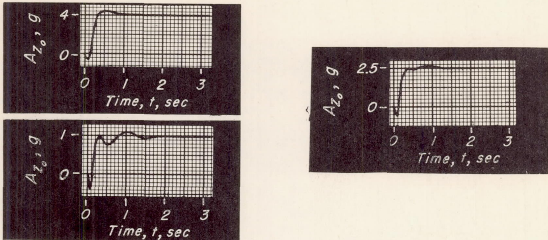
Figure 9.- Effect of input. Optimized for 4g and \dot{\delta}_{eL} of 100^\circ/\text{sec} .
