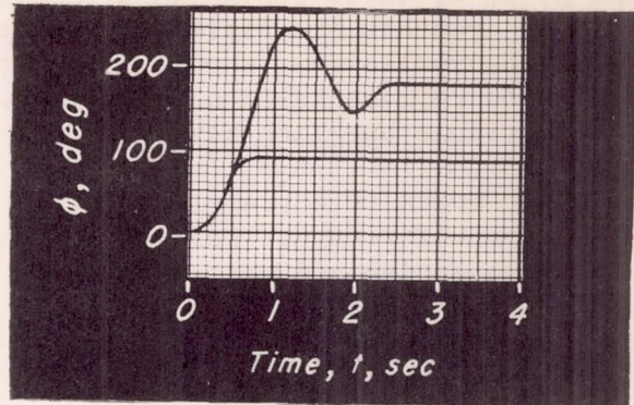
Effect of roll input. (Optimized for \phi of 90^\circ . \delta_L = \pm 15^\circ . \dot{\delta}_L = 150^\circ/\text{sec} . Incorrect simulation technique, sketch (d).) Sketch (f)
