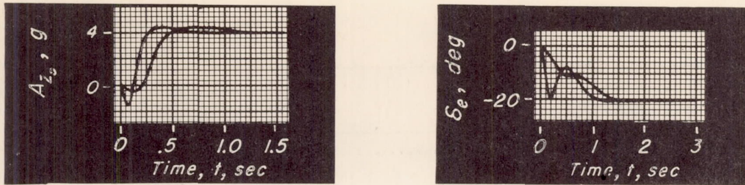
Figure 8.- Optimum responses for \dot{\delta}_{eL} of 50^\circ/\text{sec} and 300^\circ/\text{sec} .
