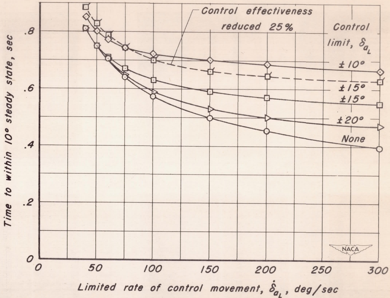
Figure 11.— Effect of limiting control deflection and rate of control movement. \phi_0 = 90^\circ .
