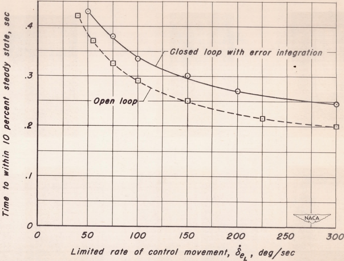
Figure 7.—Effect of limited rate of control movement on the normal acceleration response. A_{z_0} = 4g .
