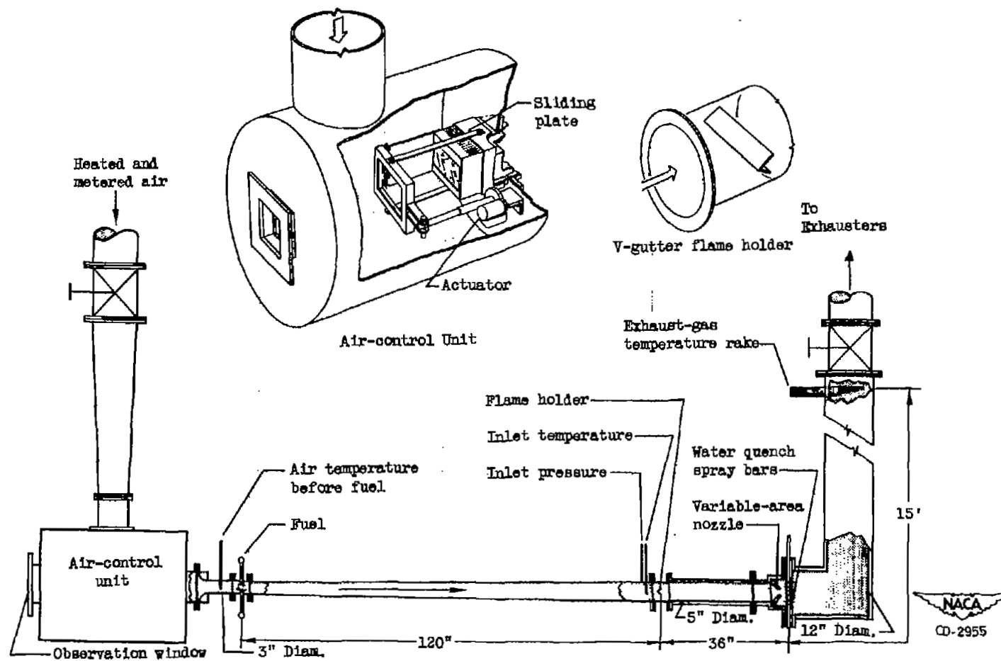
Figure 1. - Schematic illustration of 5-inch ram-jet-type combustor setup, flame holder and air-control unit.
