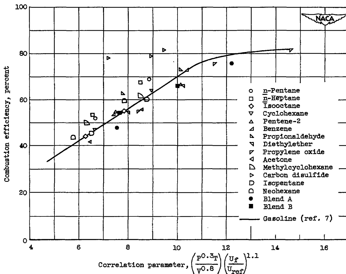
Figure 20. - Correlation of combustion efficiency for V-gutter flame holder in 5-inch ram-jet-type combustor for 14 pure fuels, a gasoline, and 2 fuel blends. (Blend A contains 2/3 propylene oxide plus 1/3 isopentane by weight; blend B, 1/3 propylene oxide plus 2/3 isopentane by weight.)
