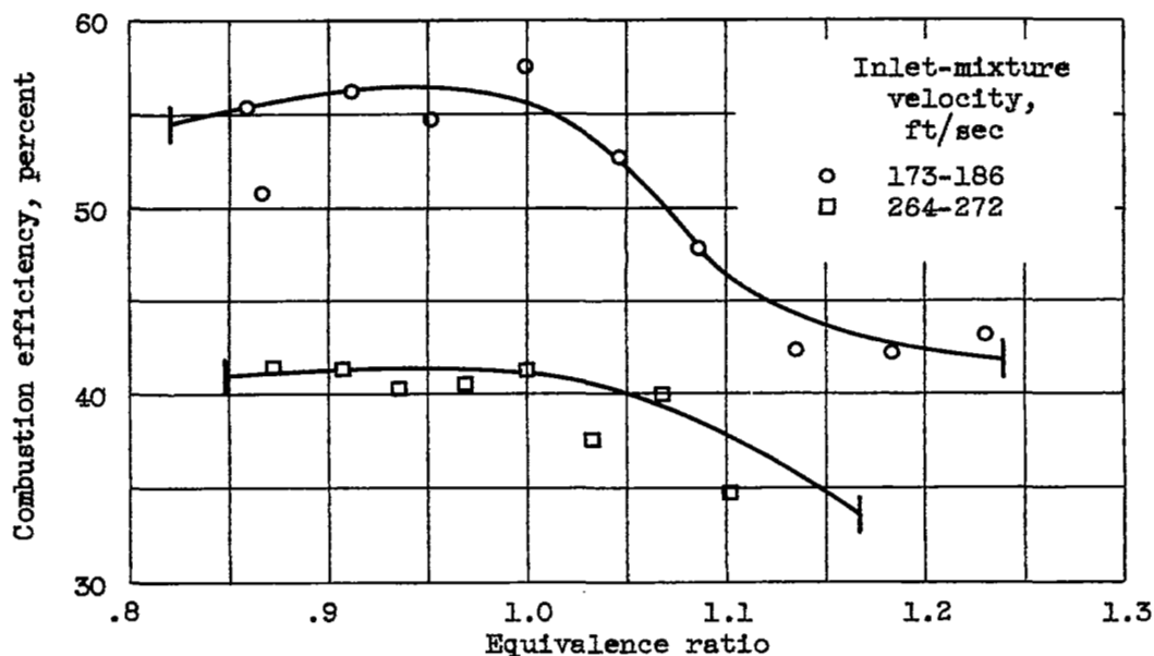
Figure 11. - Combustion efficiency of V-gutter flame holder in 5-inch ram-jet-type combustor with acetone. Combustor inlet pressure, 0.67 atmosphere; combustor inlet temperature, 579° to 624° R.
