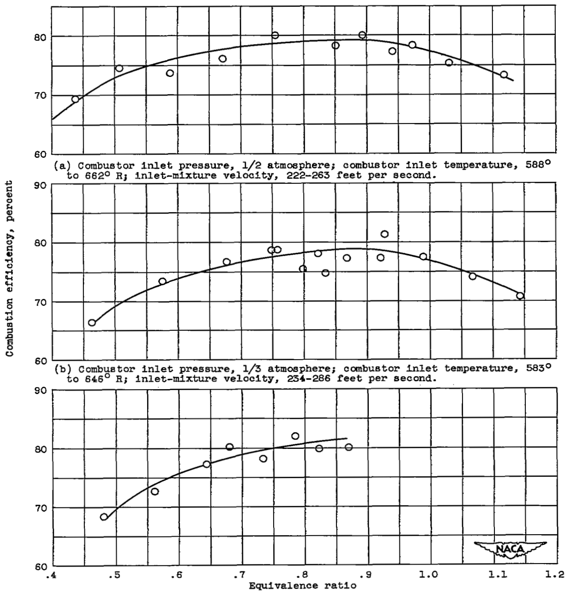
Figure 13. - Combustion efficiency of V-gutter flame holder in 5-inch ram-jet-type combustor with carbon disulfide.
