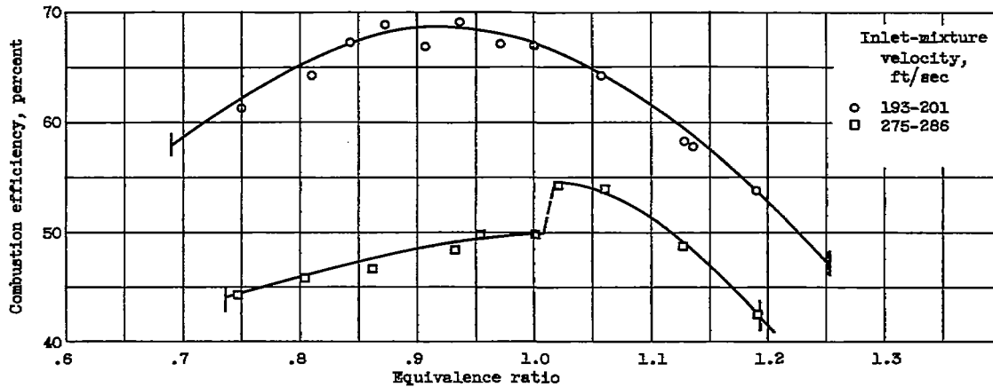
Figure 2. - Combustion efficiency of V-gutter flame holder in 5-inch ram-jet-type combustor with n -pentane. Combustor inlet pressure, 0.67 atmosphere; combustor inlet temperature, 643° to 672° R.
