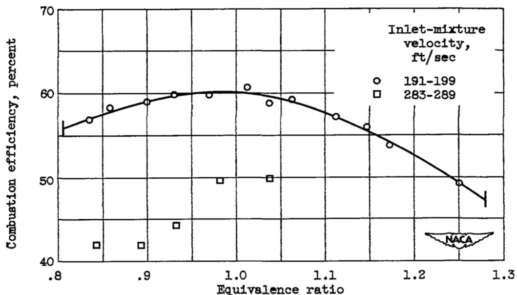
Figure 12. - Combustion efficiency of V-gutter flame holder in 5-inch ram-jet-type combustor with methylcyclohexane. Combustor inlet pressure, 0.67 atmosphere; combustor inlet temperature, 646° to 676° R.
