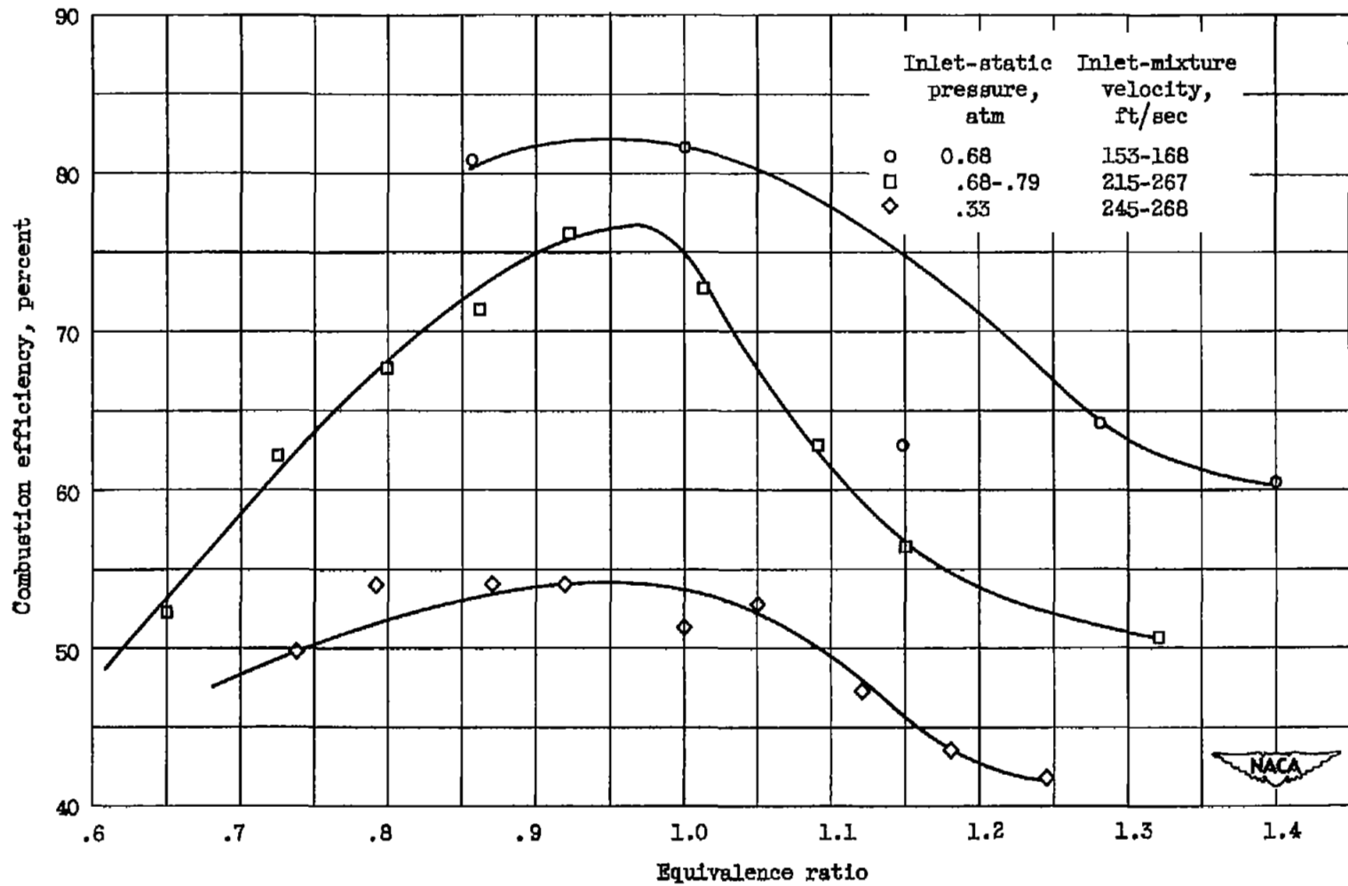
Figure 10. - Combustion efficiency of V-gutter flame holder in 5-inch ram-jet-type combustor with propylene oxide. Combustor inlet temperature, 550° to 643° R.
