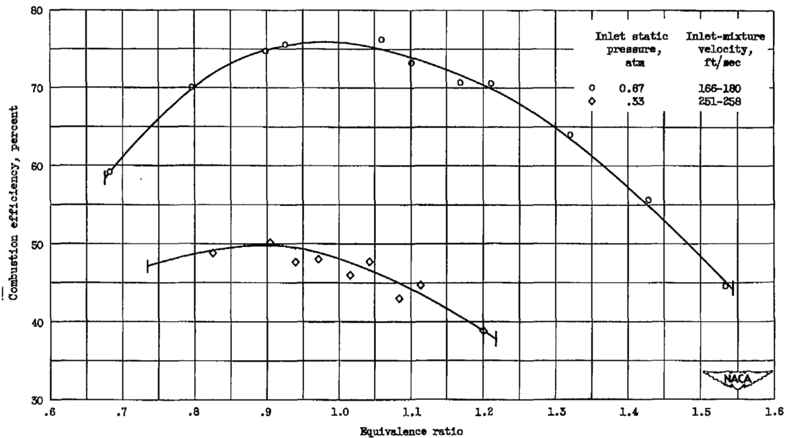
Figure 16. - Combustion efficiency of V-gutter flame holder in 5-inch ram-jet-type combustor with blend of 2/3 propylene oxide and 1/3 isopentane by weight. Combustor inlet temperature, 587° to 644° R.
