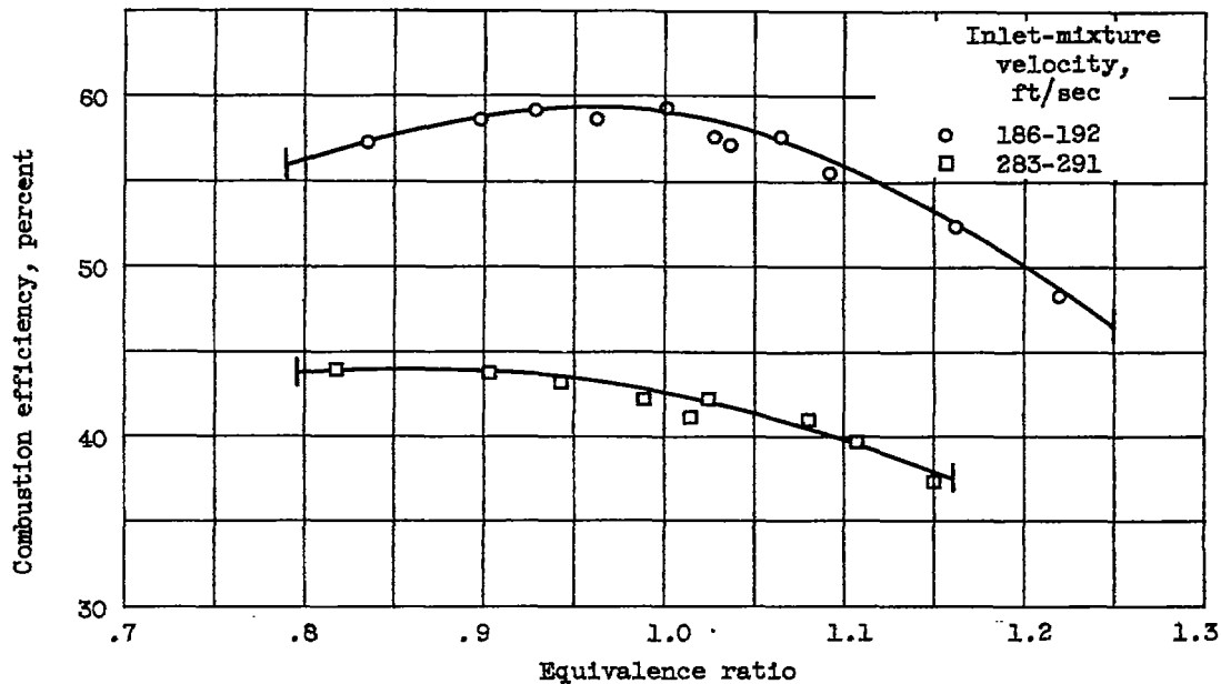
Figure 14. - Combustion efficiency of V-gutter flame holder in 5-inch ram-jet-type combustor with neohexane. Combustor inlet pressure, 0.67 atmosphere; combustor inlet temperature, 652° to 680° R.
