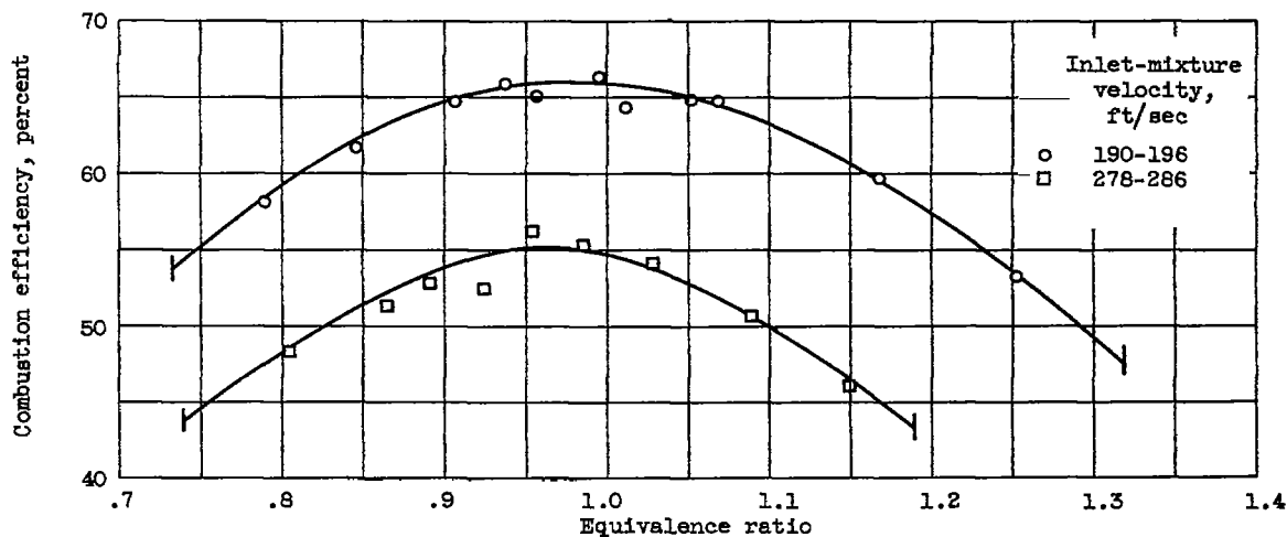
Figure 17. - Combustion efficiency of V-gutter flame holder in 5-inch ram-jet-type combustor with blend of 1/3 propylene oxide and 2/3 isopentane by weight. Combustor inlet pressure, 0.67 atmosphere; combustor inlet temperature, 638° to 676° R.
