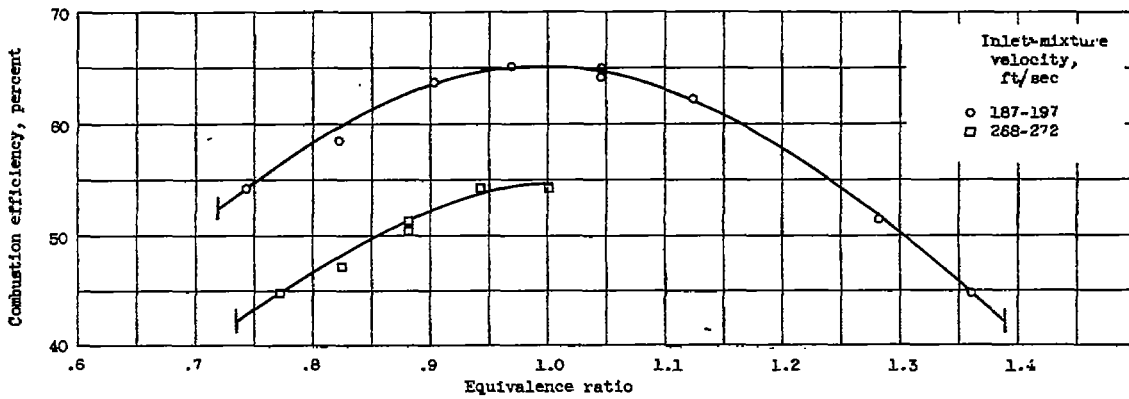
Figure 9. - Combustion efficiency of V-gutter flame holder in 5-inch ram-jet-type combustor with diethylether. Combustor inlet pressure, 0.67 atmosphere; combustor inlet temperature, 522° to 668° R.
