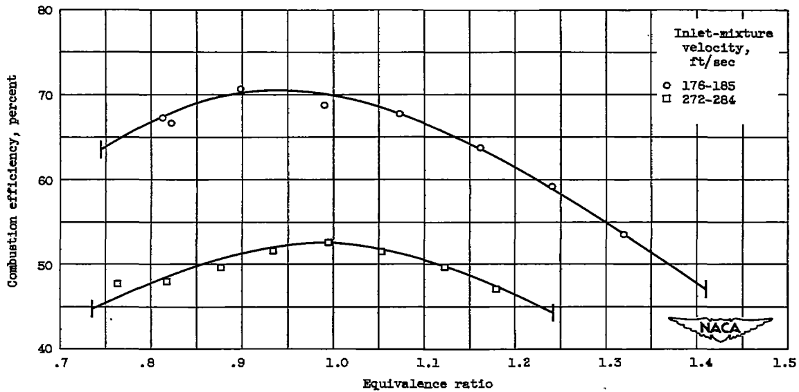
Figure 7. - Combustion efficiency of V-gutter flame holder in 5-inch ram-jet-type combustor with benzene. Combustor inlet pressure, 0.67 atmosphere; combustor inlet temperature, 639° to 680° R.
