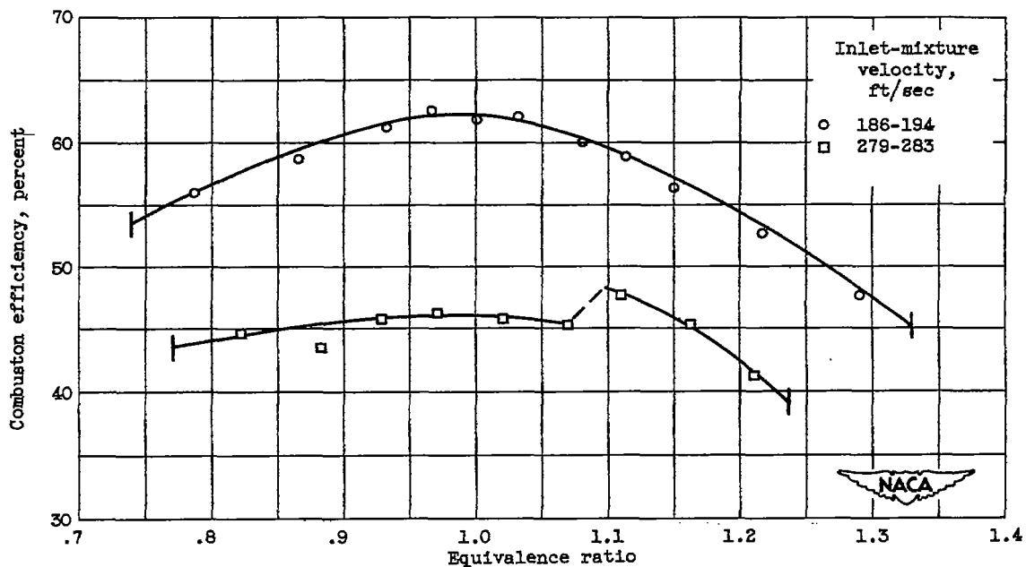
Figure 5. - Combustion efficiency of V-gutter flame holder in 5-inch ram-jet-type combustor with cyclohexane. Combustor inlet pressure, 0.67 atmosphere; combustor inlet temperature, 646° to 674° R.
