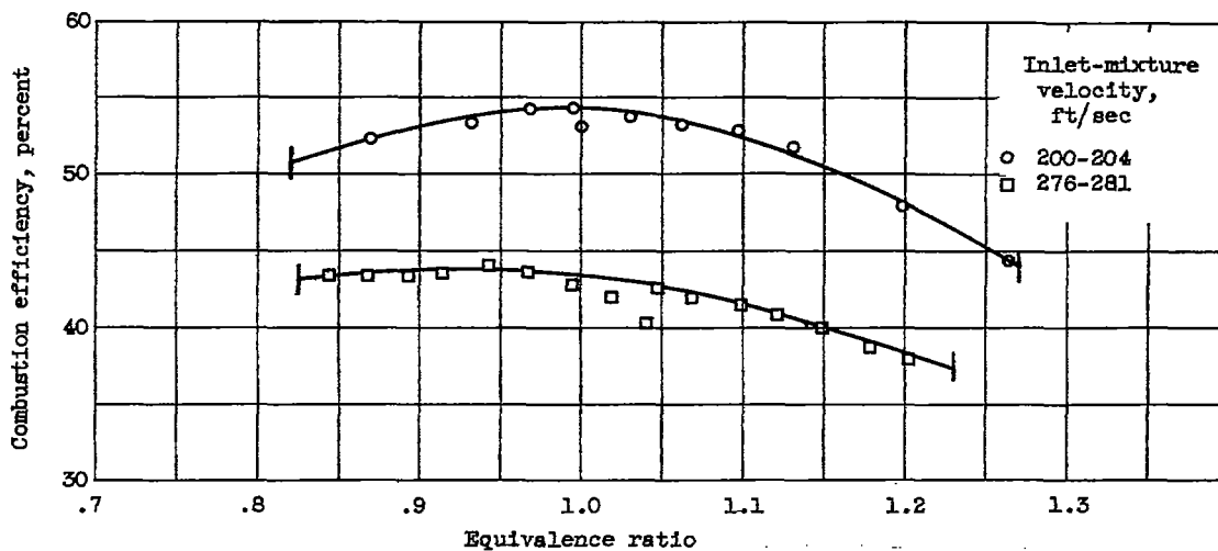
Figure 4. - Combustion efficiency of V-gutter flame holder in 5-inch ram-jet-type combustor with isooctane. Combustor inlet pressure, 0.67 atmosphere; combustor inlet temperature, 657° to 690° R.
