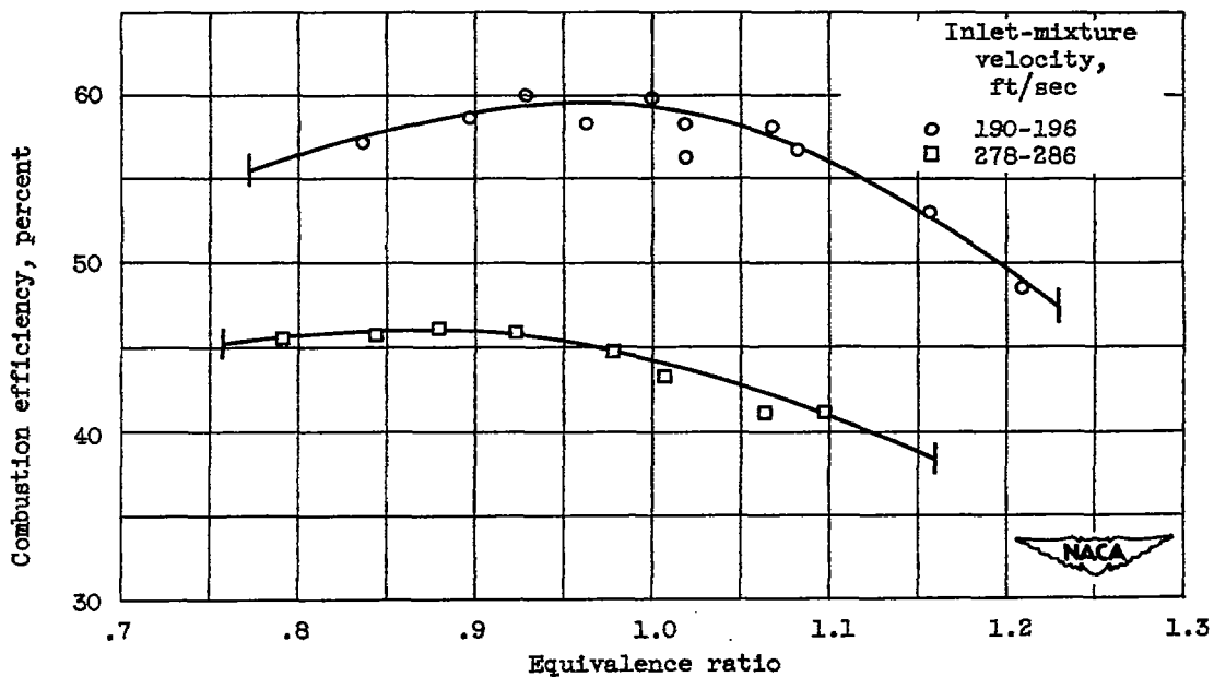
Figure 15. - Combustion efficiency of V-gutter flame holder in 5-inch ram-jet-type combustor with isopentane. Combustor inlet pressure, 0.67 atmosphere; combustor inlet temperature, 665° to 690° R.
