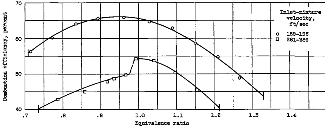
Figure 6. - Combustion efficiency of V-gutter flame holder in 5-inch ram-jet-type combustor with pentene-2. Combustor inlet pressure, 0.67 atmosphere; combustor inlet temperature, 644° to 678° R.
