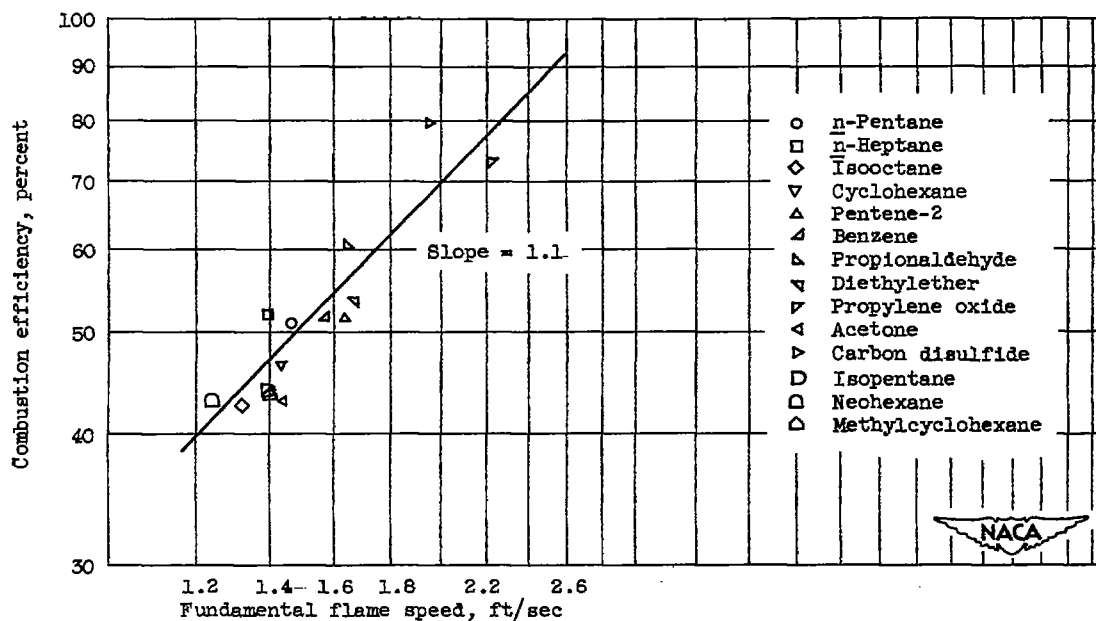
Figure 18. - Effect of fundamental flame speed on combustion efficiency at equivalence ratio of 1.0 and at inlet parameter value p_0 \cdot 3_T / v_0 \cdot 8 of about 6.5.
