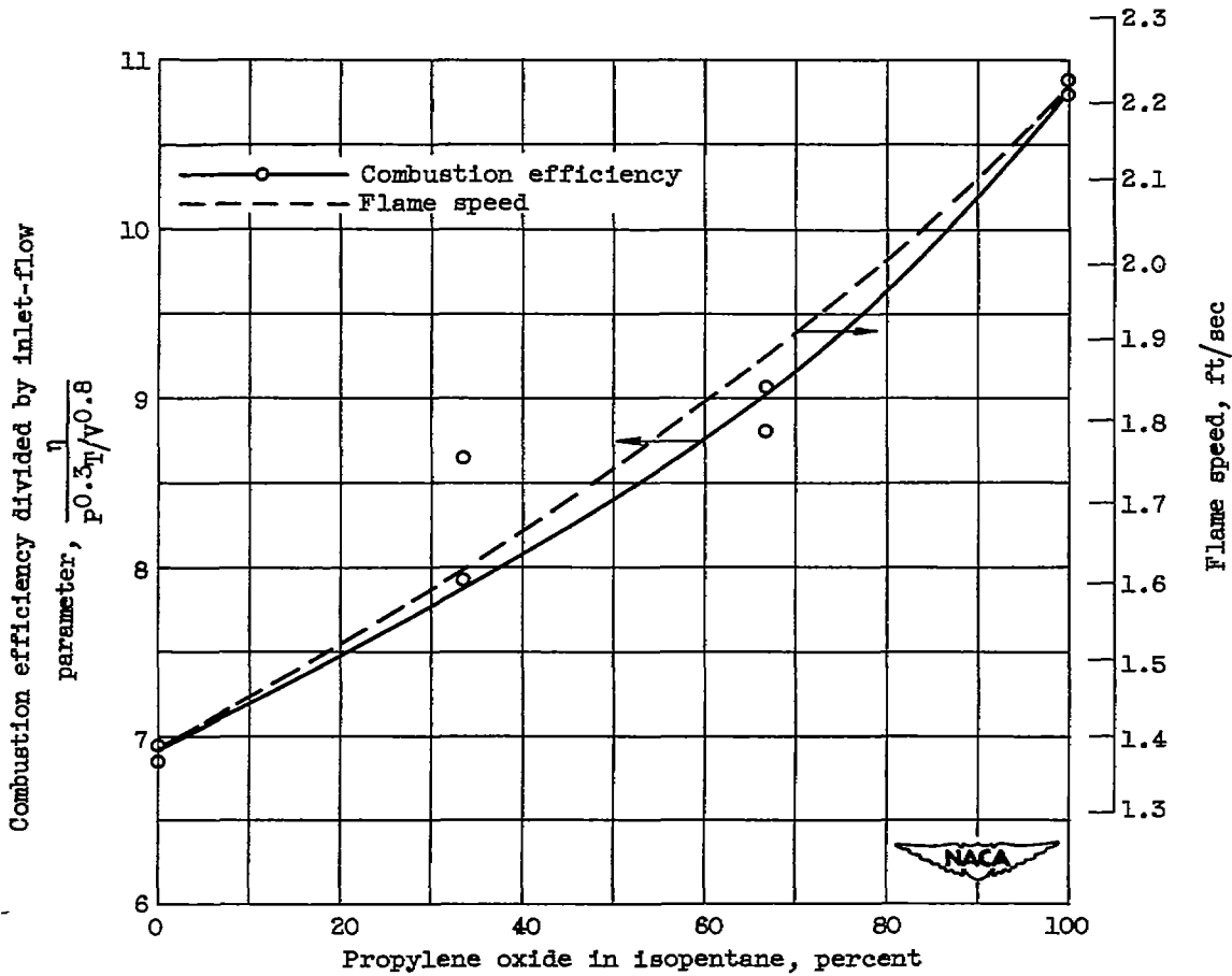
Figure 19. - Effect of blend percentage on combustion efficiency and flame speed of propylene oxide and isopentane blends at equivalence ratio of 1.0.
