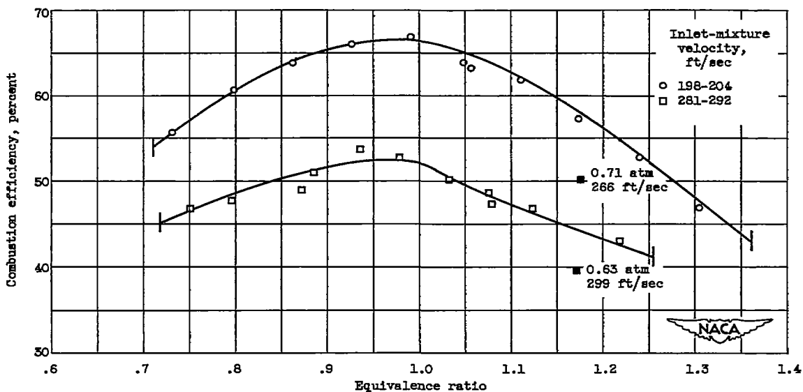
Figure 3. - Combustion efficiency of V-gutter flame holder in 5-inch ram-jet-type combustor with n -heptane. Combustor inlet pressure, 0.67 atmosphere; combustor inlet temperature, 655° to 694° R.
