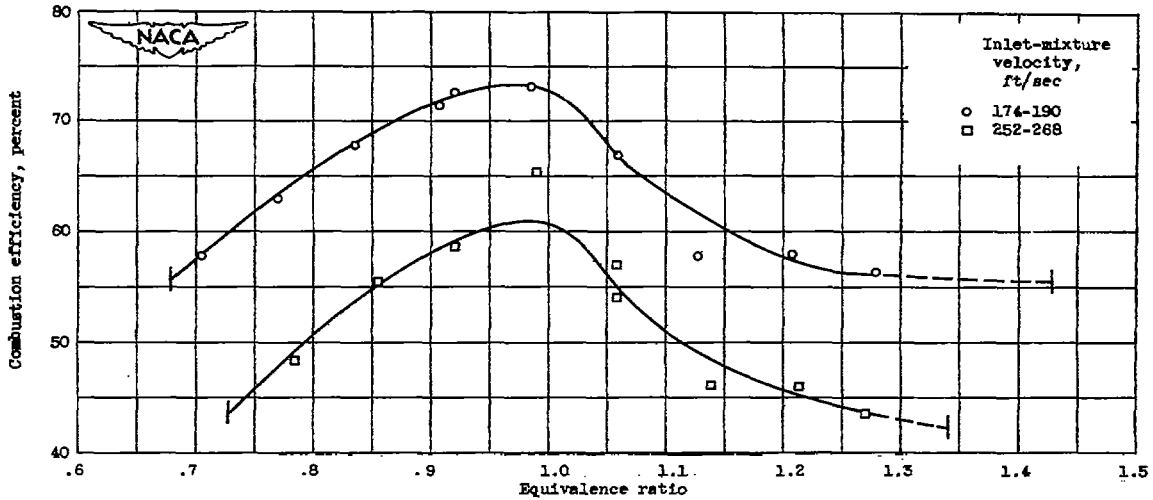
Figure 8. - Combustion efficiency of V-gutter flame holder in 5-inch ram-jet-type combustor with propionaldehyde. Combustor inlet pressure, 0.67 atmosphere; combustor inlet temperature, 590° to 643° R.
