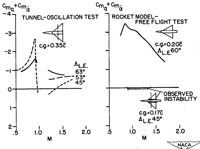
Figure 10.- Variation of the pitch-damping factor C_{m_q} + C_{m_{\dot{\alpha}}} with Mach number for tailless delta-wing aircraft.
