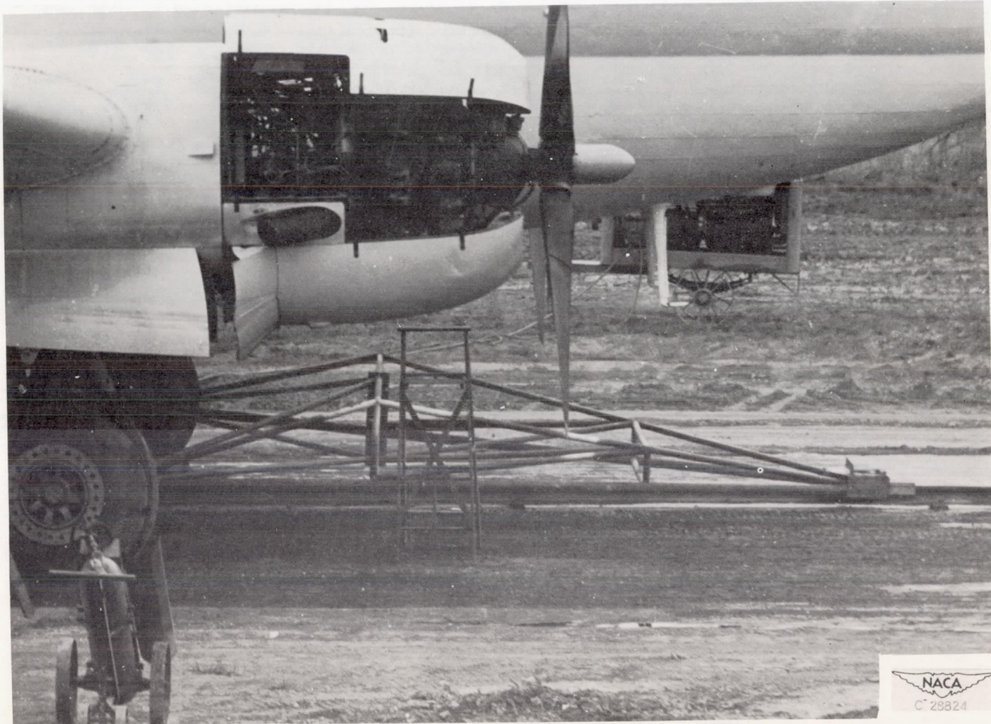
Figure 7. - Guiding truss attached to main landing wheel of C-46 airplane.
