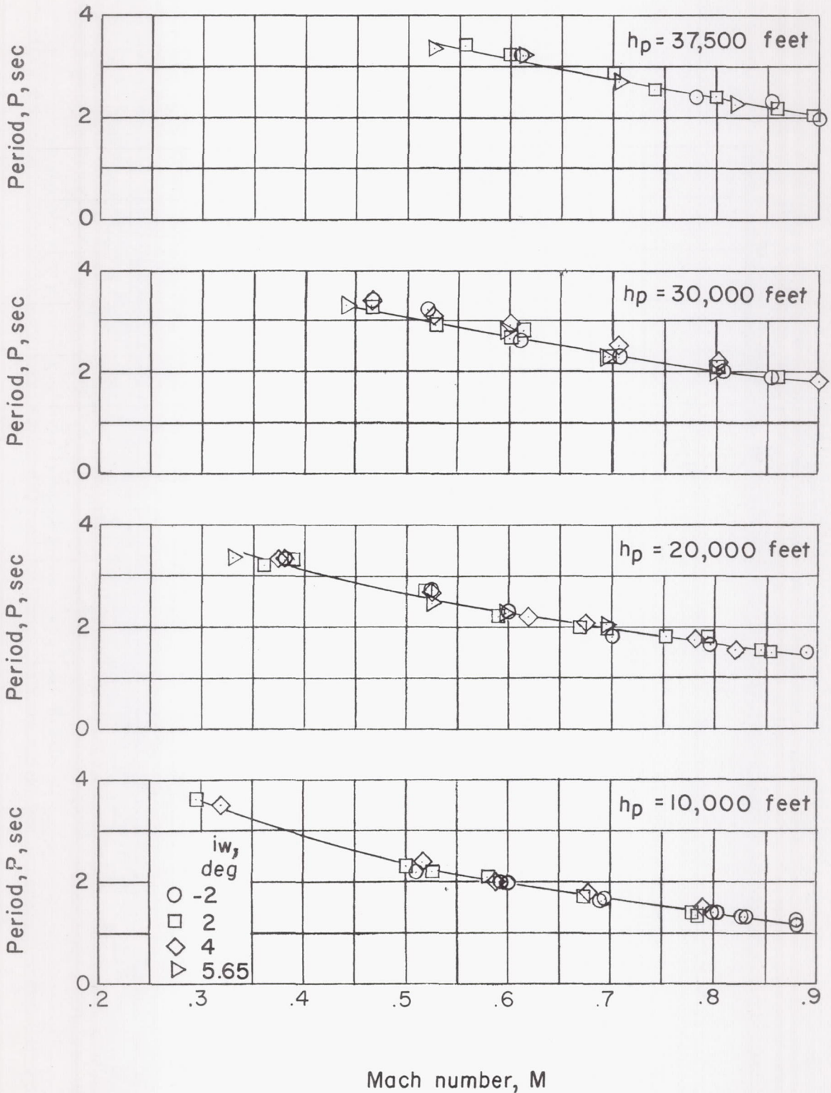
Figure 5.- Variation of period of the lateral oscillation with Mach number.
