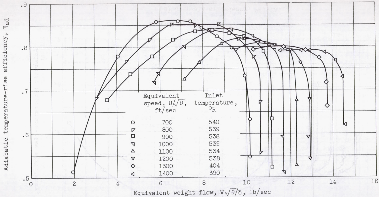
(e) Over-all efficiency, MFI-2B.
