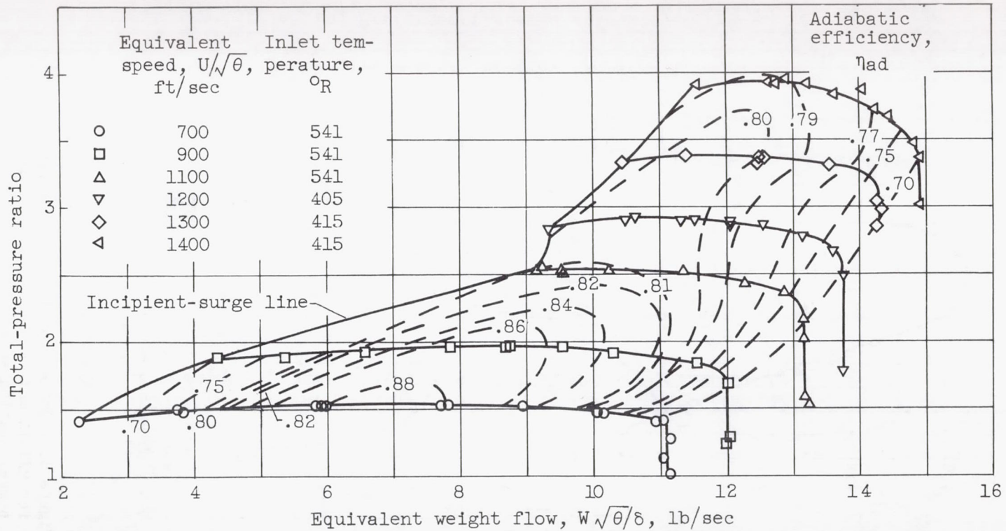
(a) Performance characteristics, MFI-2A.
