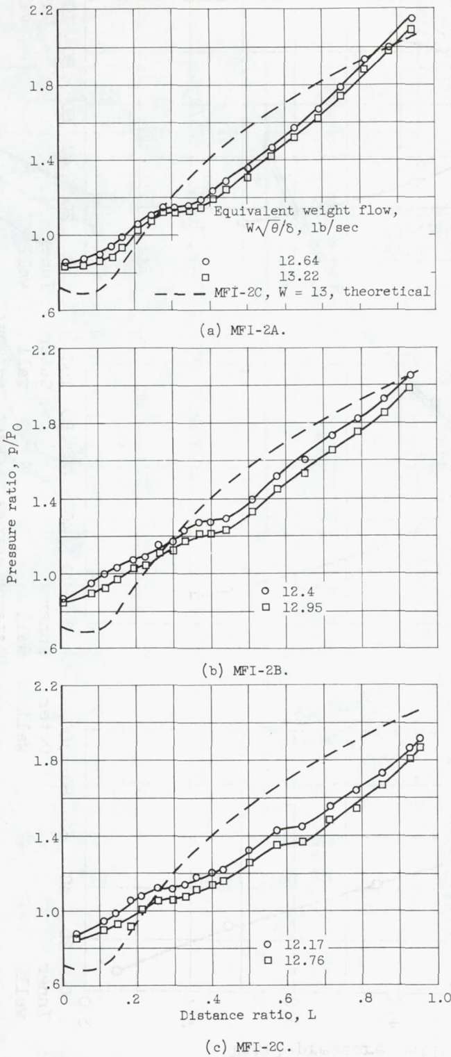
Figure 9. - Static-pressure ratios along shroud of MFI-2 for outlet speed of 1400 feet per second.
