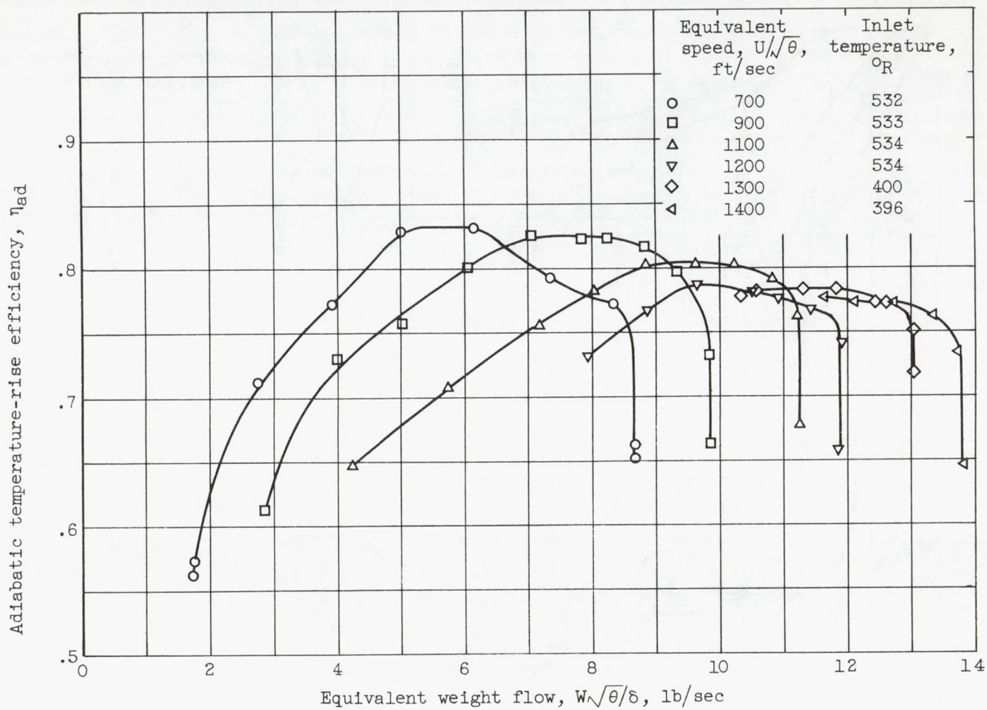
Figure 7. - Concluded. Over-all performance characteristics of MFI-2 impeller at inlet-air pressure of 14 inches of mercury absolute.
