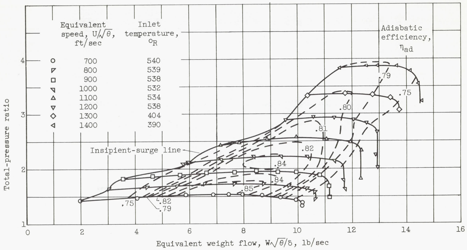
(b) Performance characteristics, MFI-2B.
