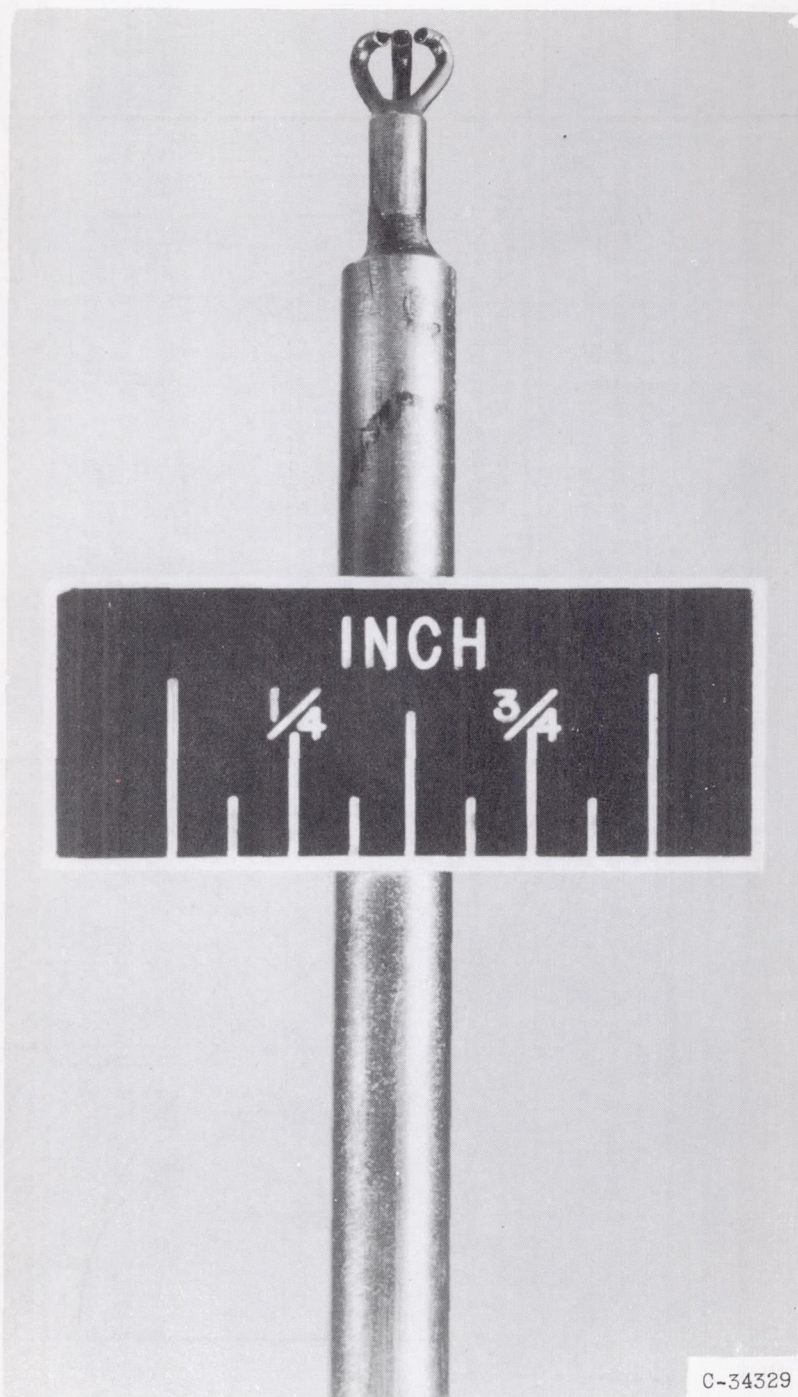
Figure 2. - Claw-type probe.
