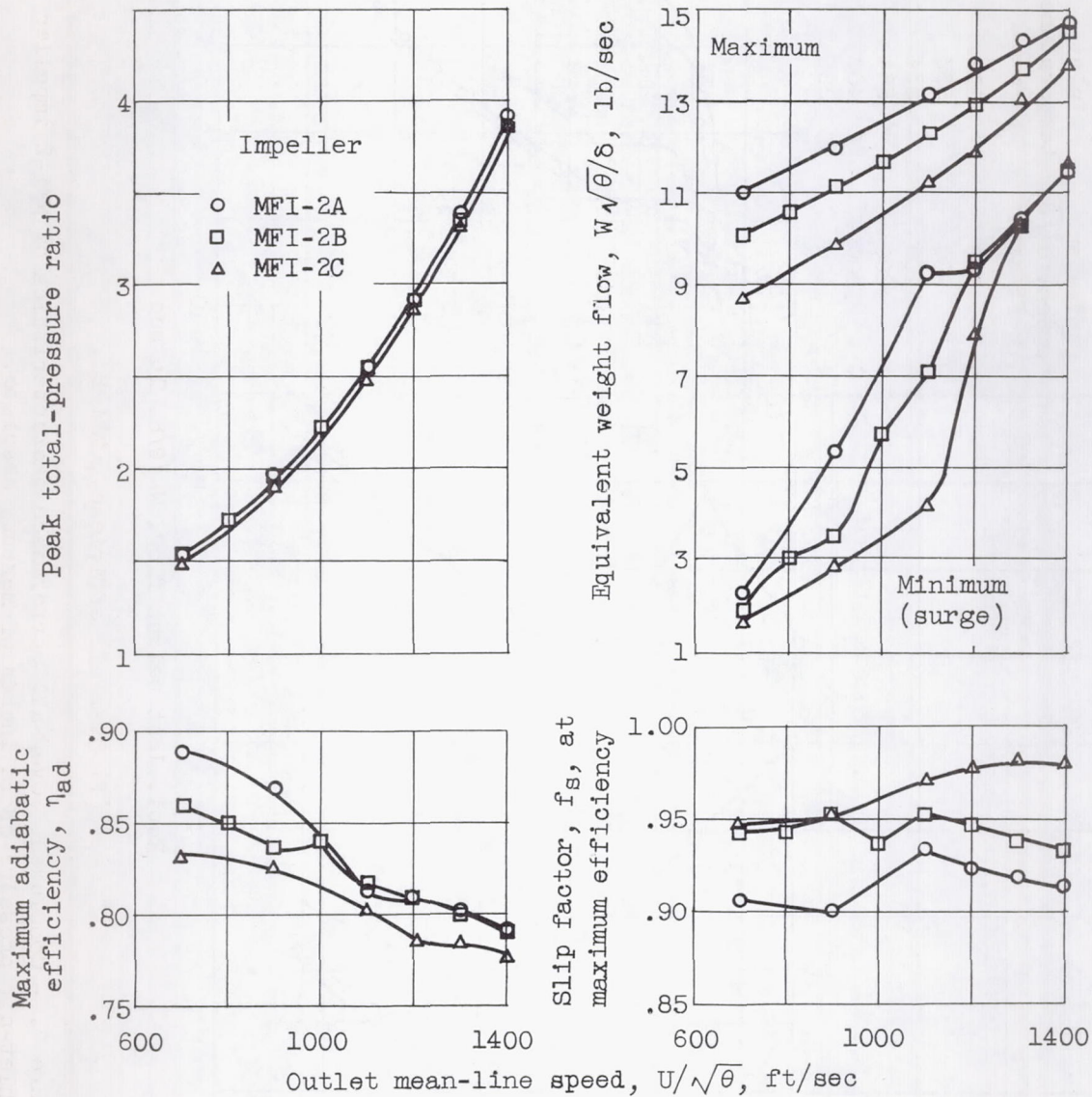
Figure 8. - Comparison of performance of impellers MFI-2A, MFI-2B, and MFI-2C.
