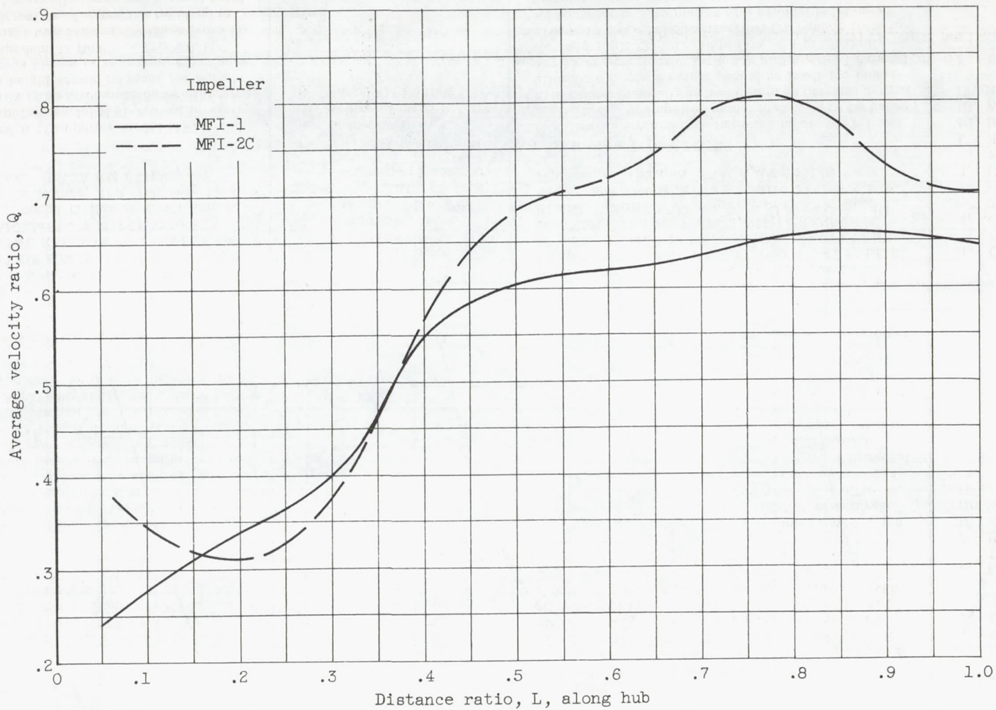
Figure 11. - Comparison of theoretical average velocity along hub for MFI-1 and MFI-2C. Outlet mean-line speed, 1400 feet per second; weight flow, 13.0 pounds per second.
