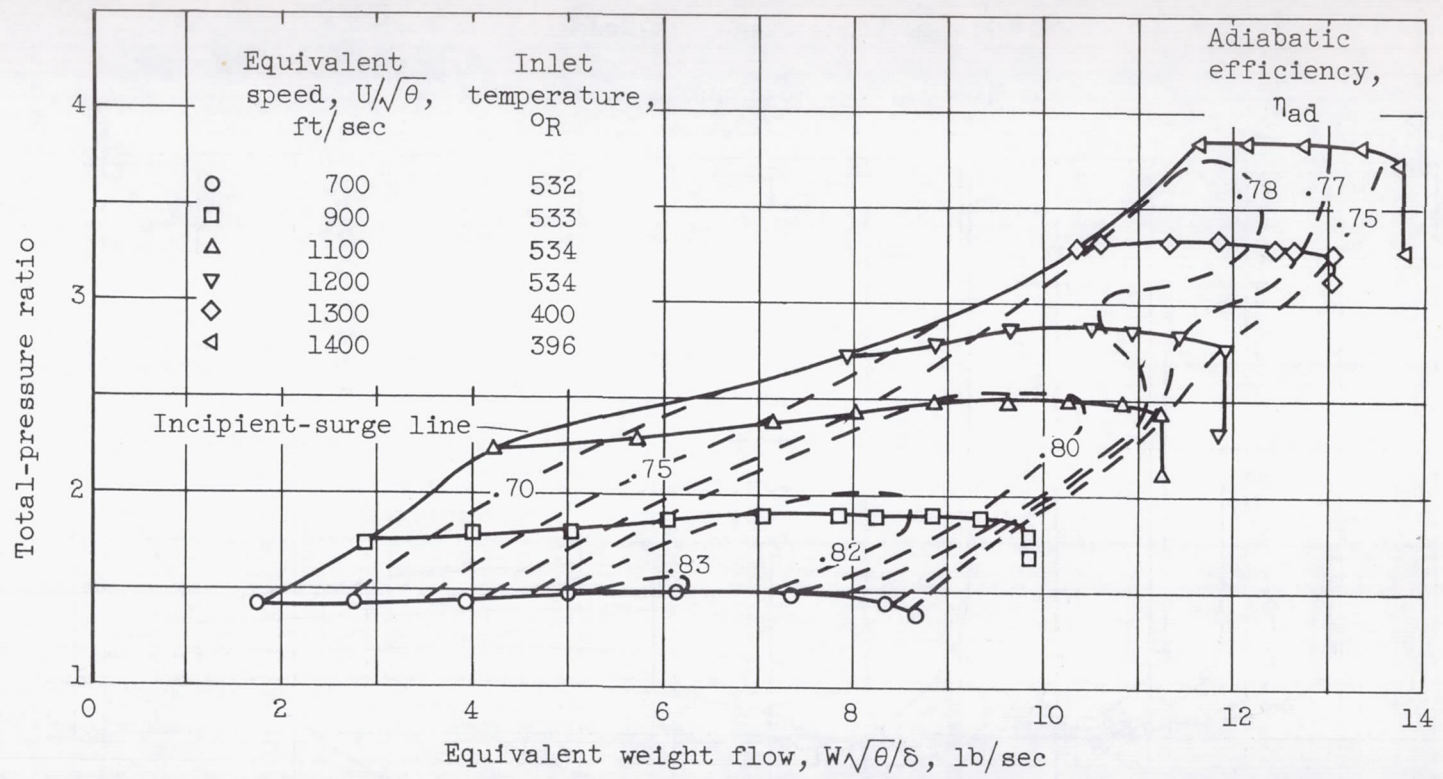
(c) Performance characteristics, MFI-2C.
