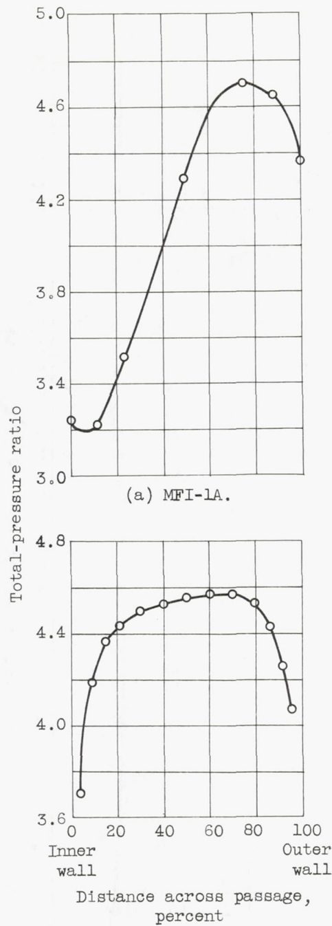
Figure 6. - Outlet total-pressure surveys for MFI-1A and MFI-1B. (Location of survey station shown in fig. 1.) Outlet mean-line speed, 1400 feet per second; equivalent weight flow, 13.5 pounds per second.
