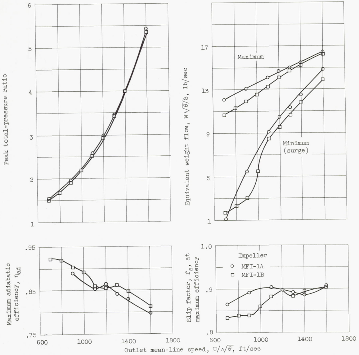
Figure 4. - Comparison of performance of impellers MFI-1A and MFI-1B.
