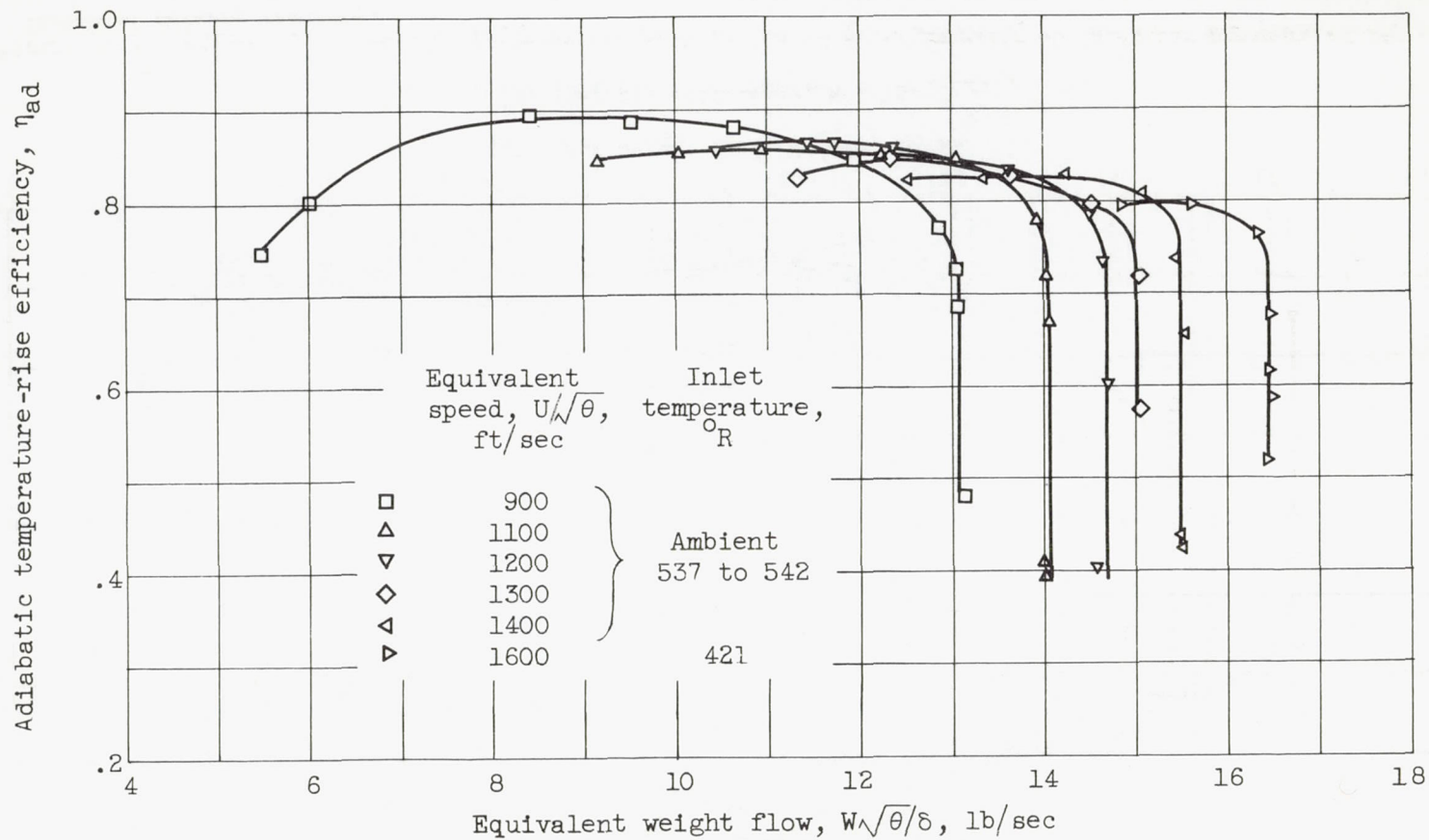
(c) Over-all efficiency, MFI-1A.
