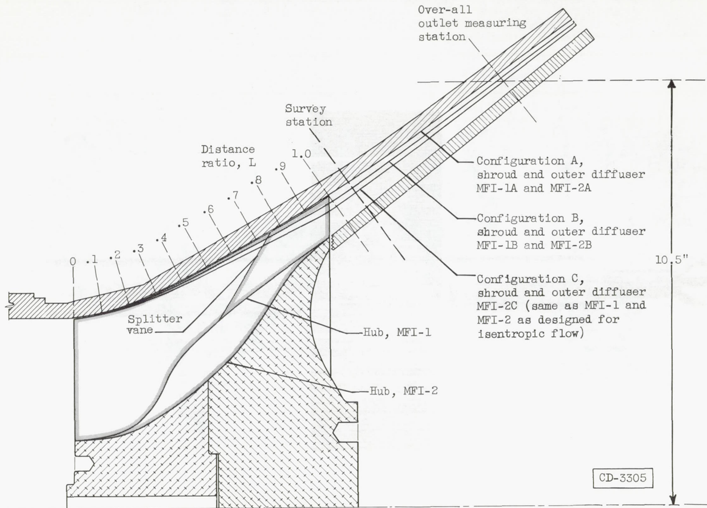
(c) Cross-sectional view showing variation in passage height.
