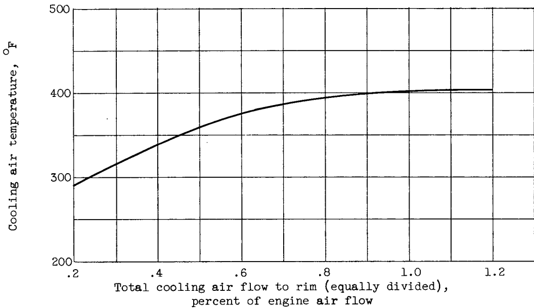
Figure 6. - Variation of cooling air temperature with cooling air flow.
