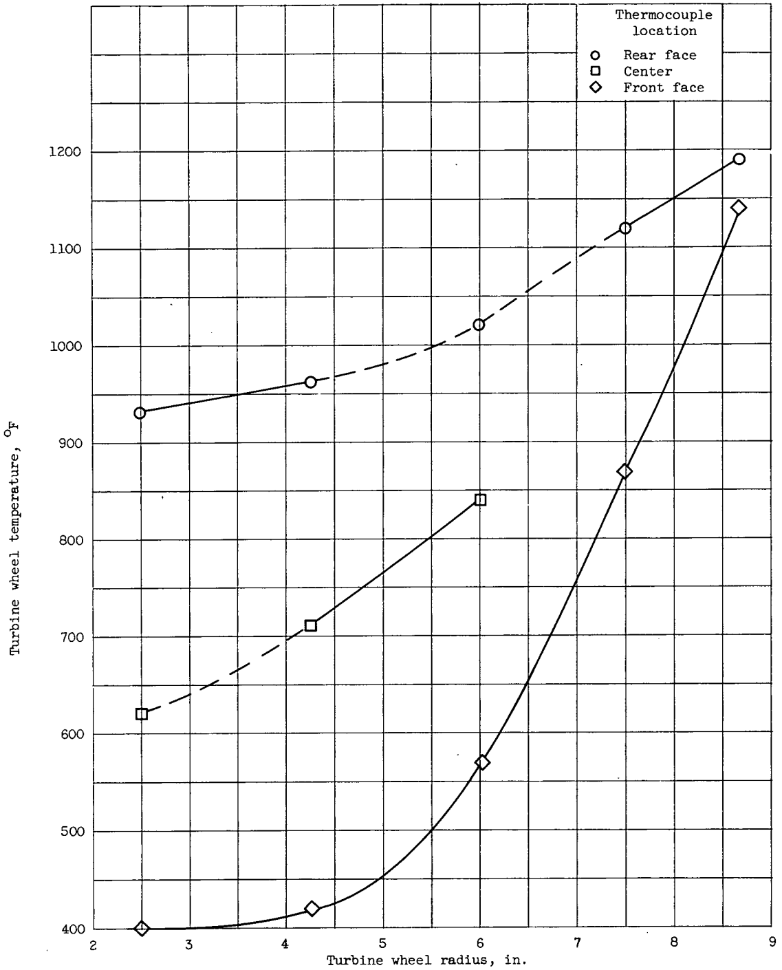
(b) J33-9 engine.
