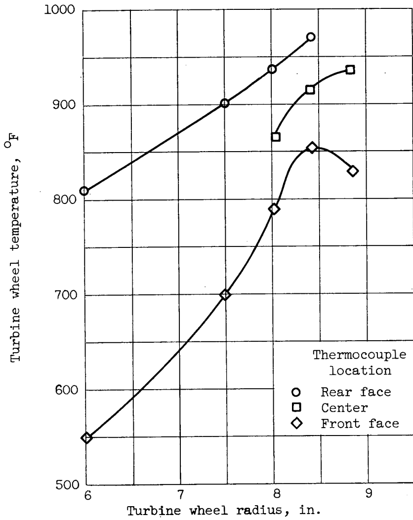
(a) Standard J33-A-33 engine.
