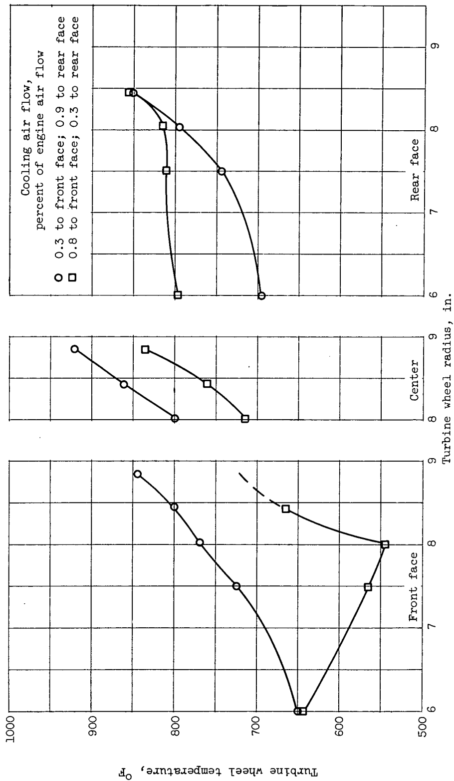
Figure 7. - Turbine wheel temperatures during runs with unbalanced cooling air flow.
