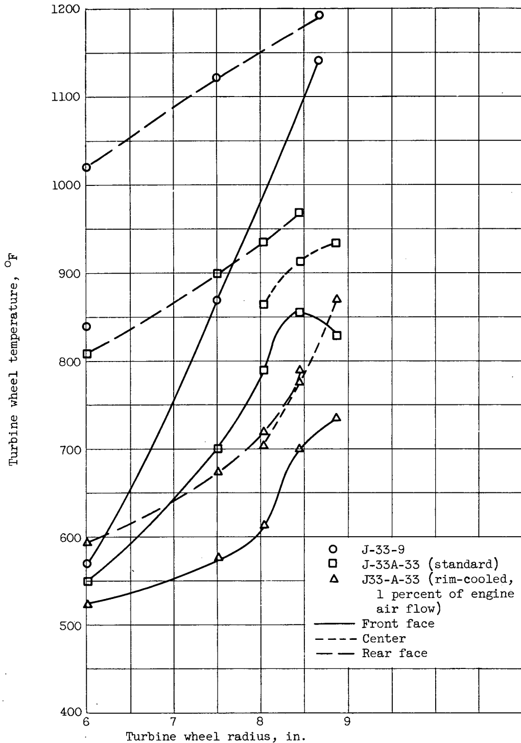
(c) Standard J33-A-33, rim-cooled J33-A-33, and J33-9 engines.
