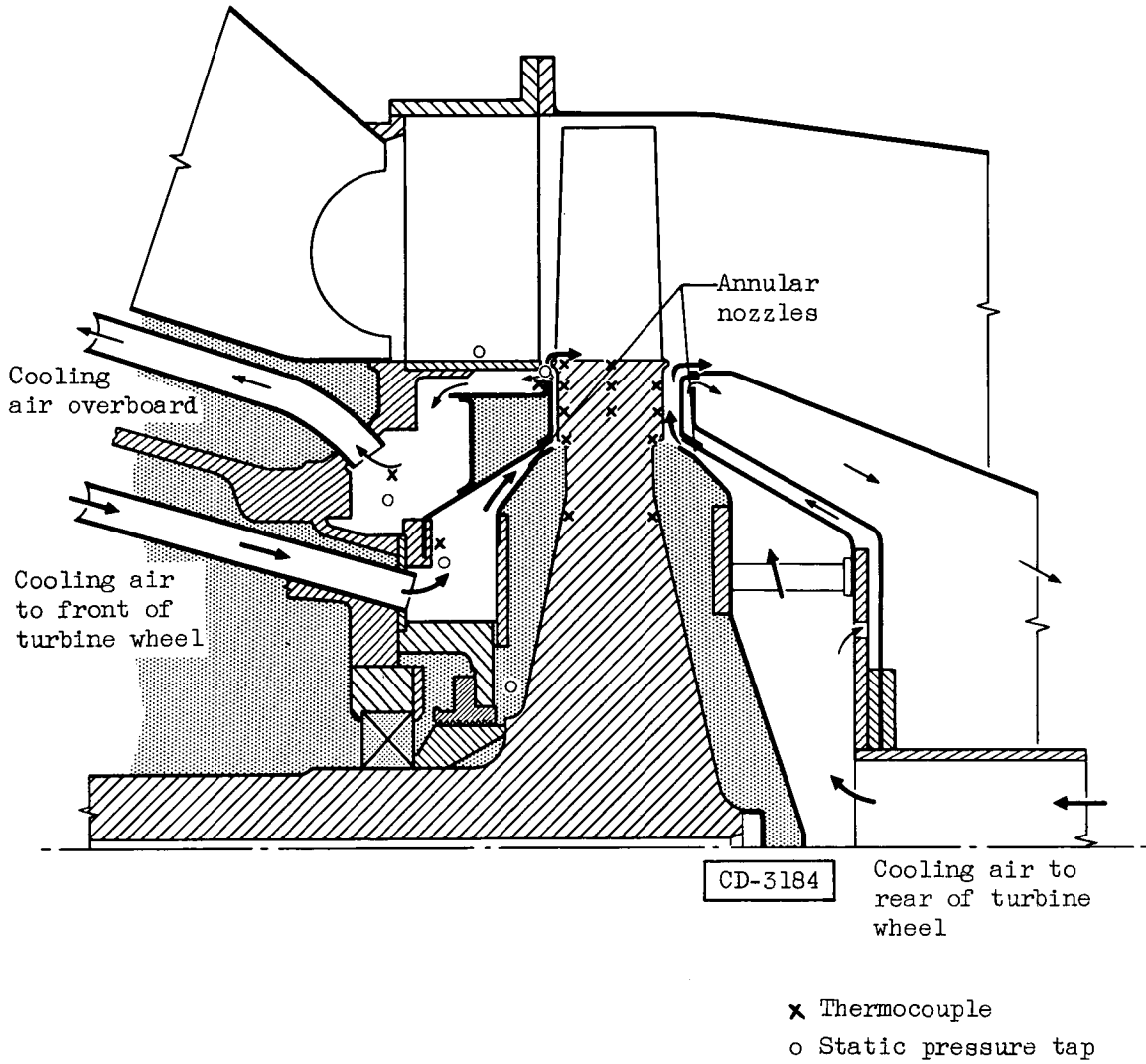
Figure 2. - Section showing turbine wheel and cooling air passages.
