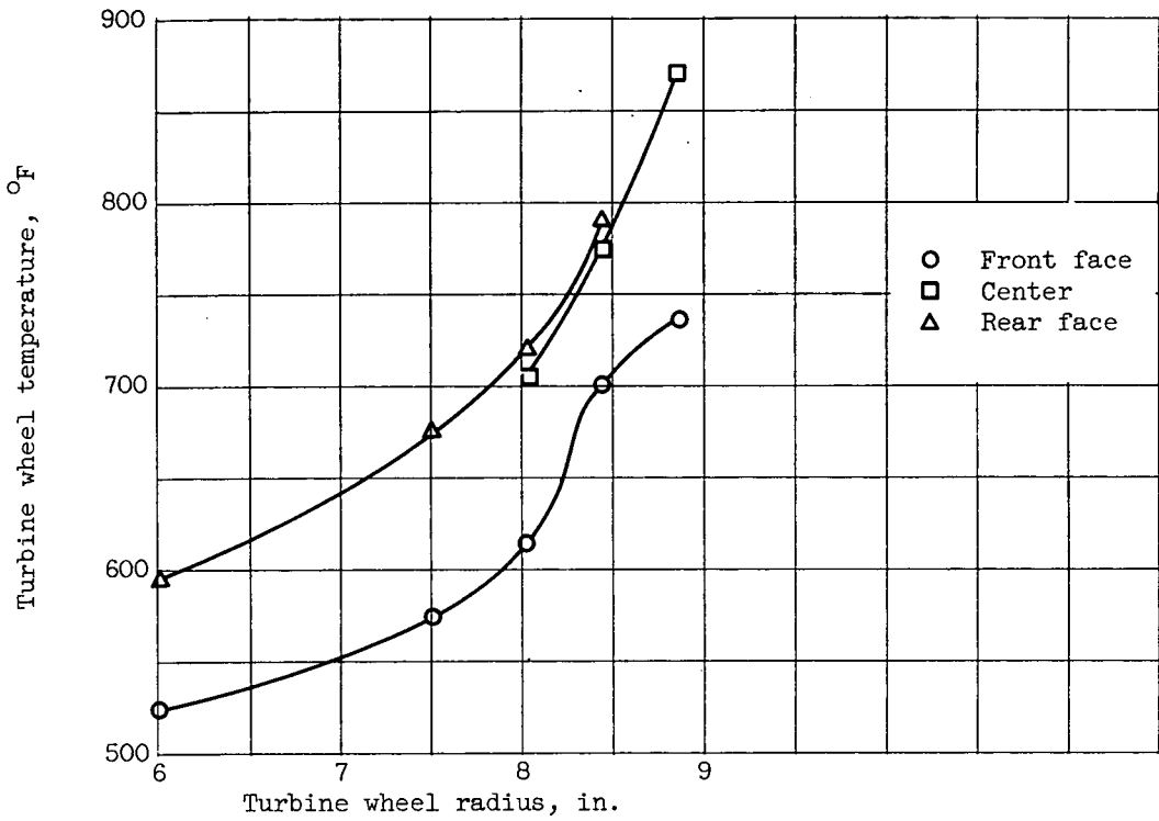
Figure 5. - Turbine wheel temperatures. Cooling air flow, 1 percent of engine air flow.
