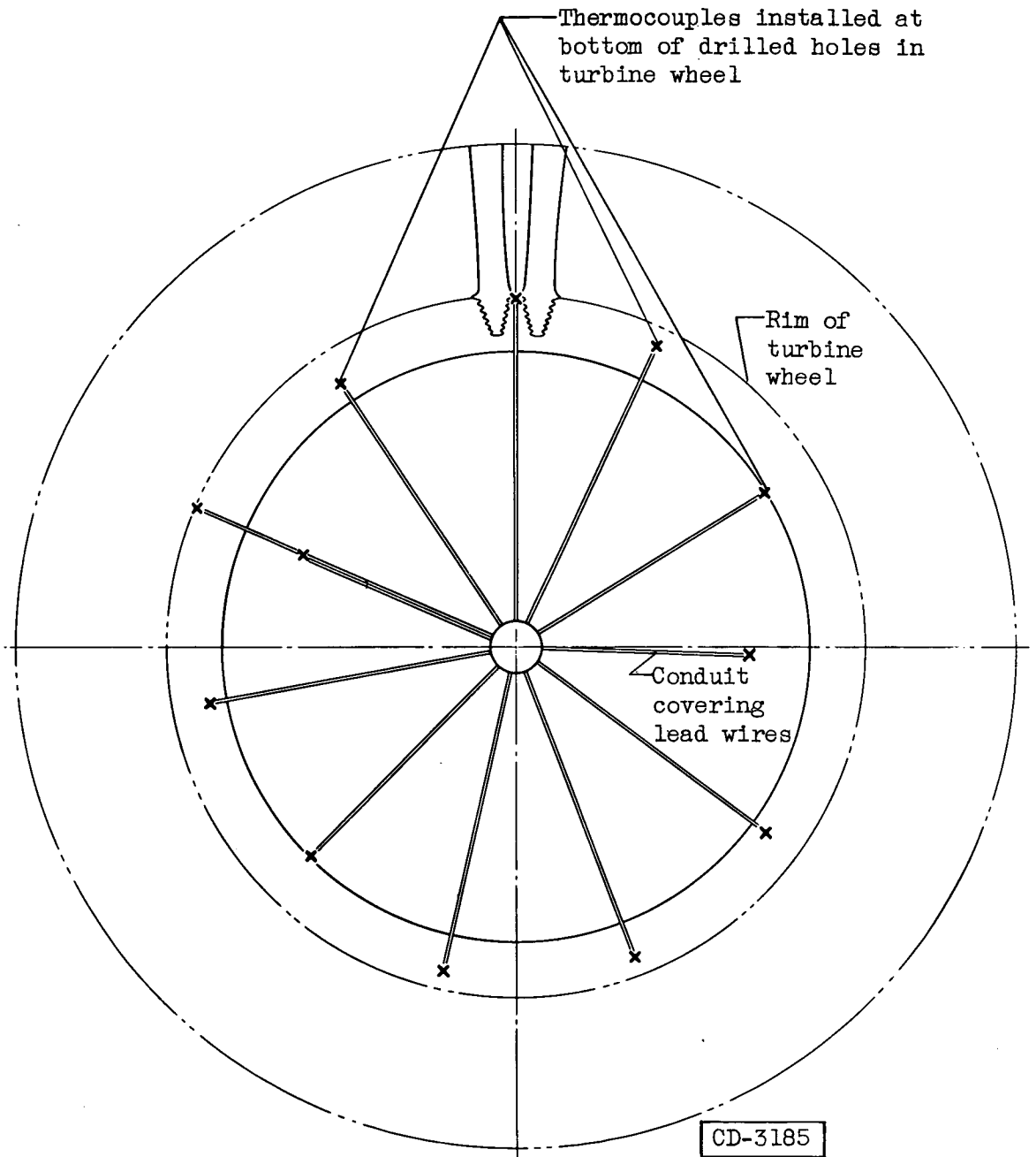
Figure 3. - Instrumentation of rear face of turbine wheel.
