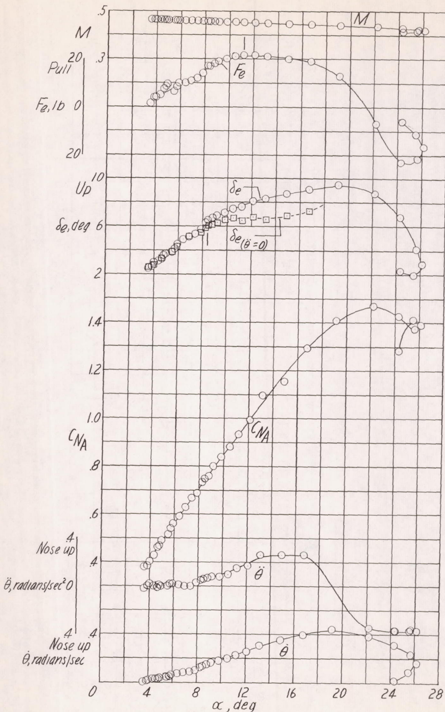
(b) h_p \approx 15,900 feet; i_t = 1.3^\circ ; center of gravity at 26.4 percent mean aerodynamic chord.
