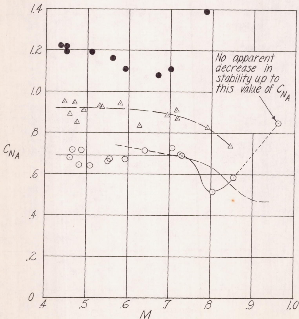
Figure 19.- Normal-force coefficient for decay in longitudinal stability as a function of Mach number for the airplane with inboard fences on the wing.
