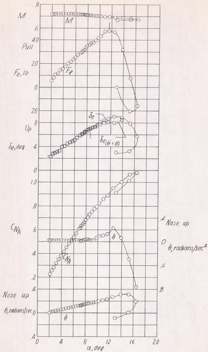
(j) h_p \approx 21,500 feet; i_t = 1.6^\circ ; center of gravity at 25.4 percent mean aerodynamic chord.
