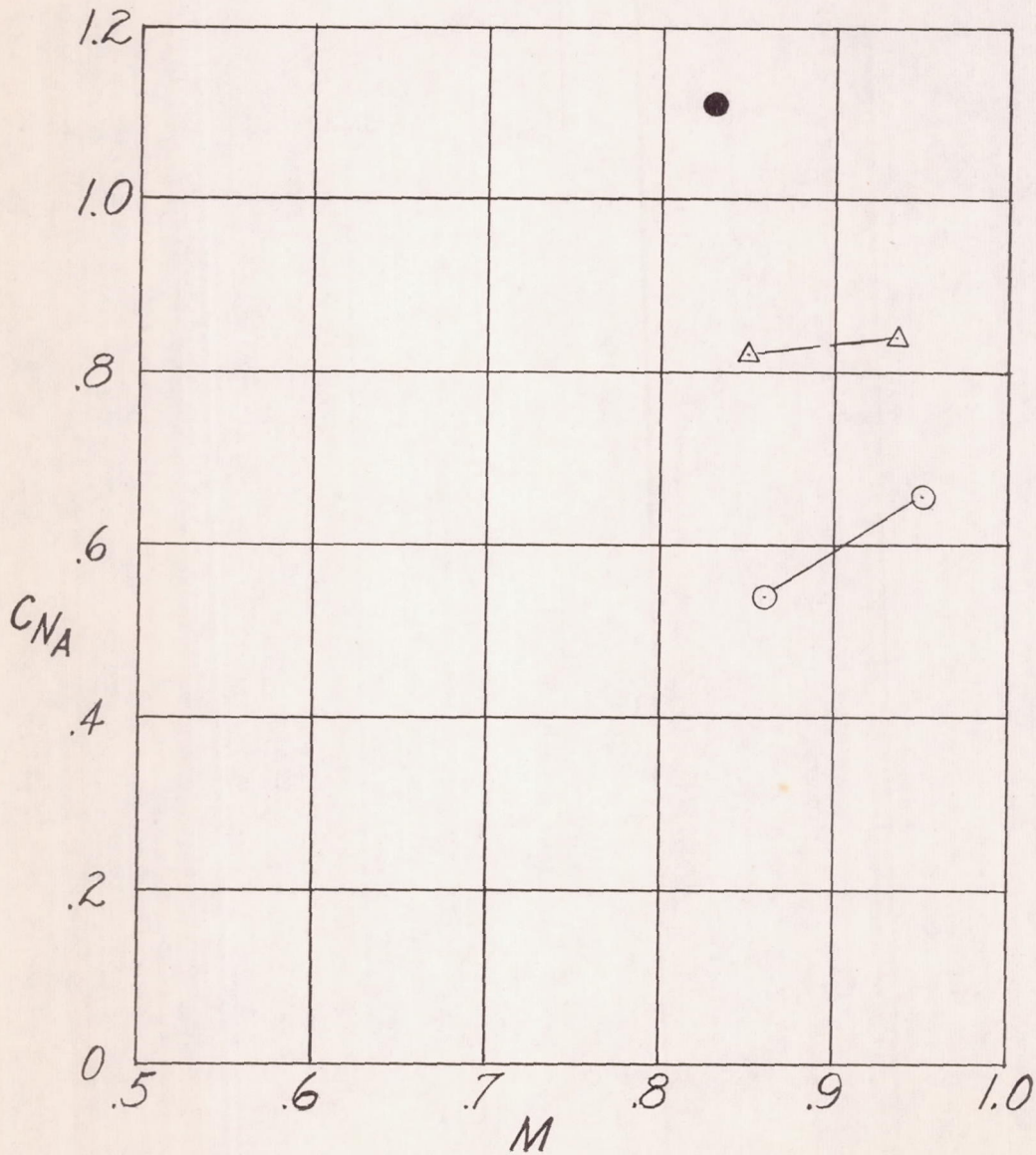
Figure 21.- Normal-force coefficient for decay in longitudinal stability as a function of Mach number for the airplane with half-extended slats and inboard wing fences removed.
