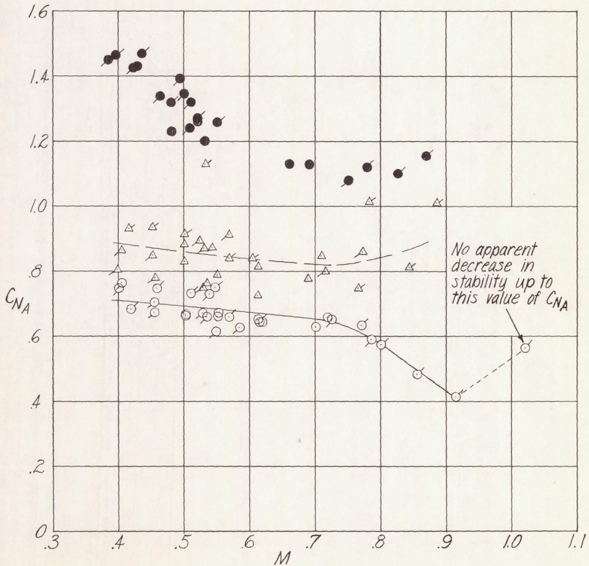
Figure 20.- Normal-force coefficient for decay in longitudinal stability as a function of Mach number for the airplane with fully extended slats and inboard wing fences removed.
