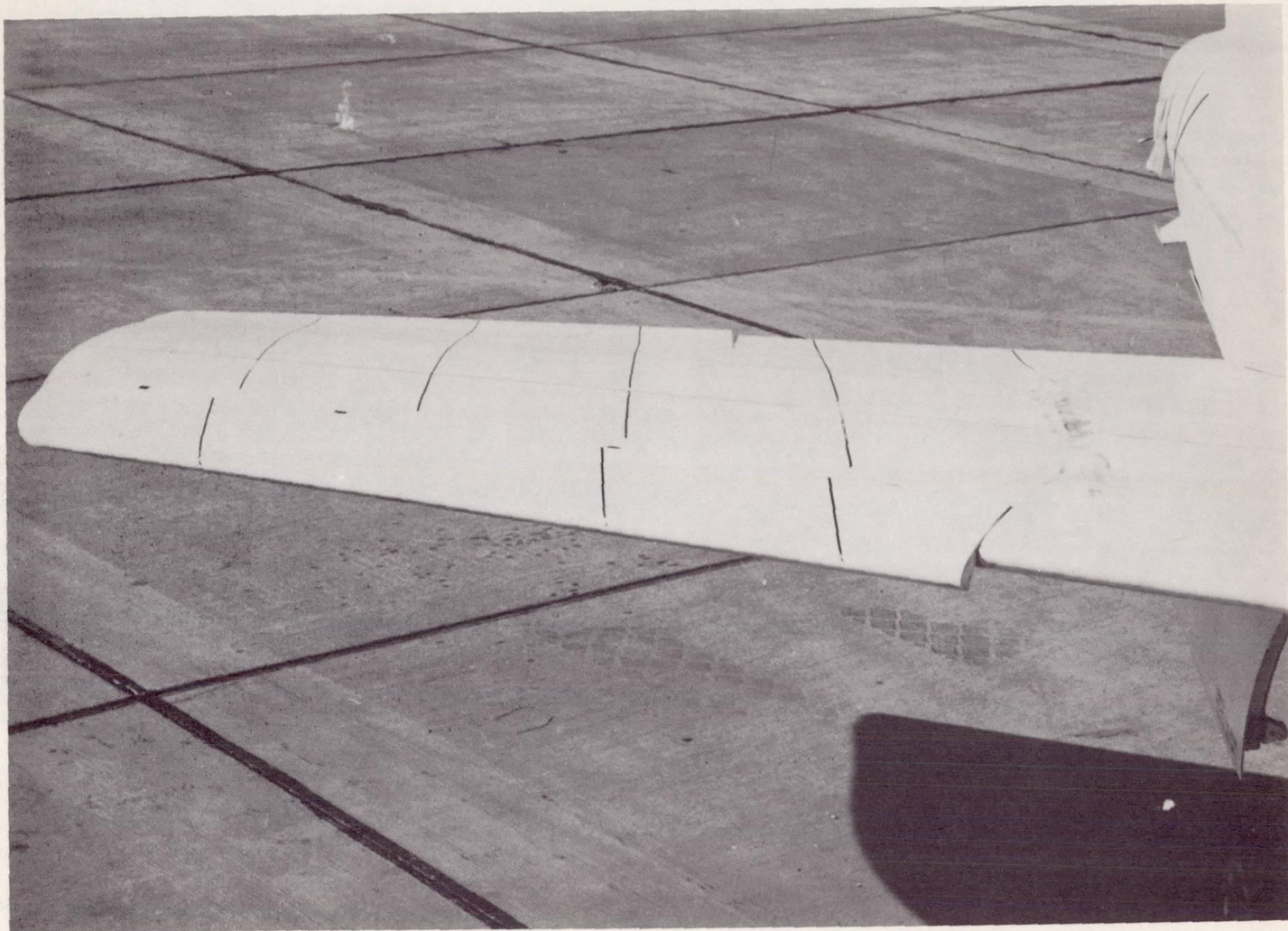
Figure 6.- Photograph of right wing of D-558-II airplane, showing slat in half-extended position with inboard wing fences removed.
