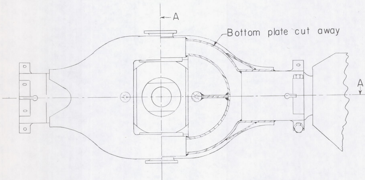
Figure 3.- Sketch of rotor-hub assembly.
