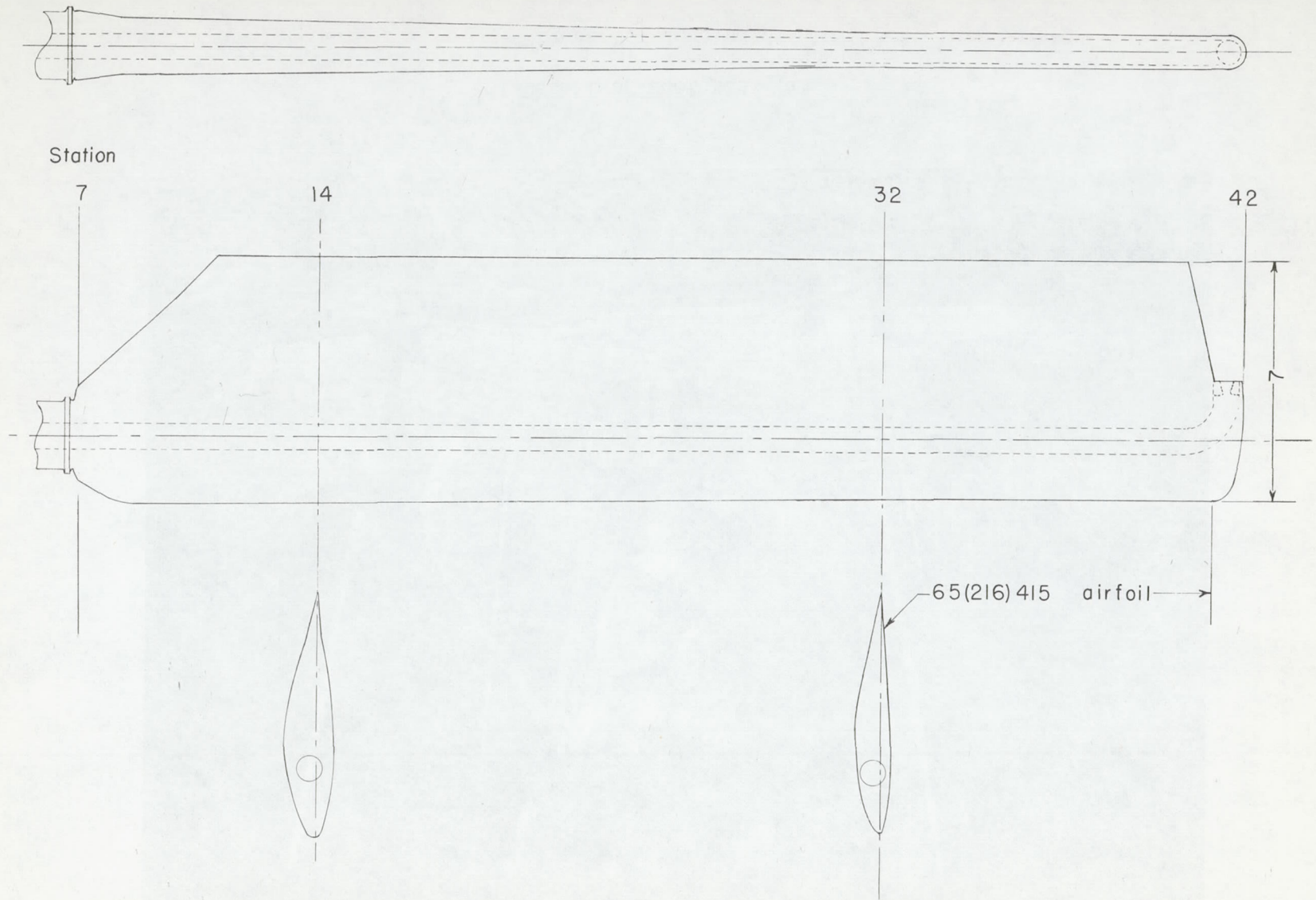
Figure 2.- Sketch of rotor blade. All dimensions are in inches.
