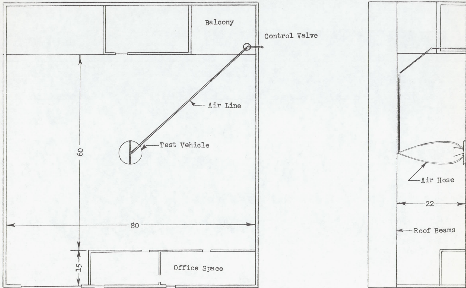
Figure 6.- Sketch of test room. Dimensions in feet.
