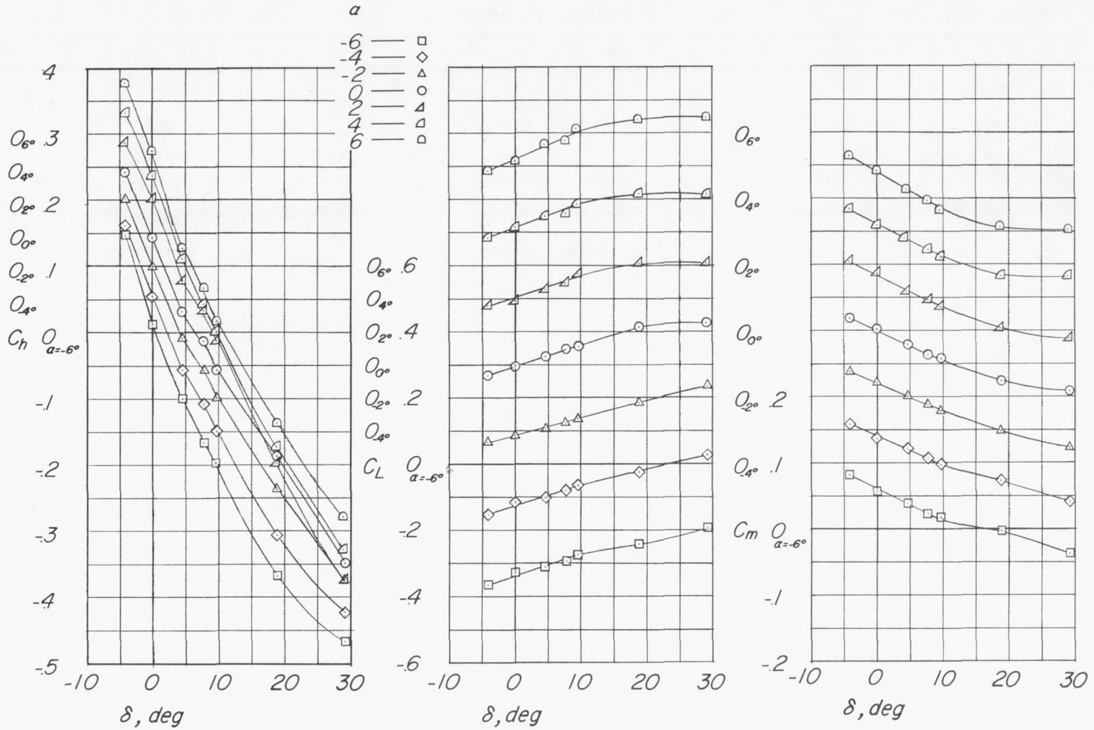
(g) M = 1.00 ; c_b/c_f = 0.32 .
