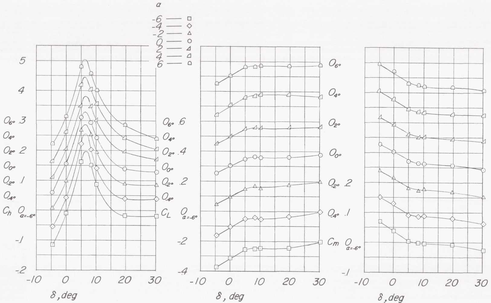
(c) M = 0.80 ; c_b/c_f = 0.79 .
