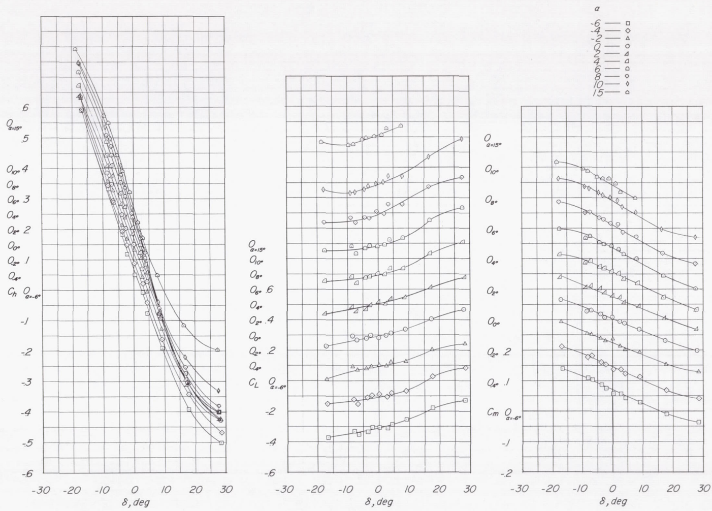
(j) M = 1.18 ; c_b/c_f = 0.07 .
