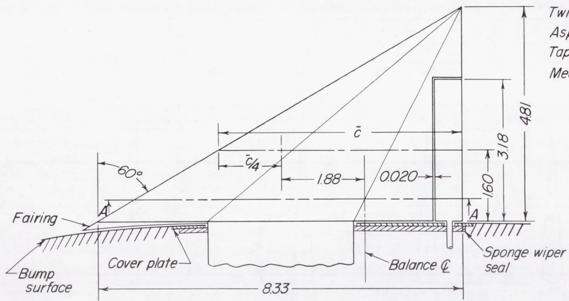
(a) Model details.
