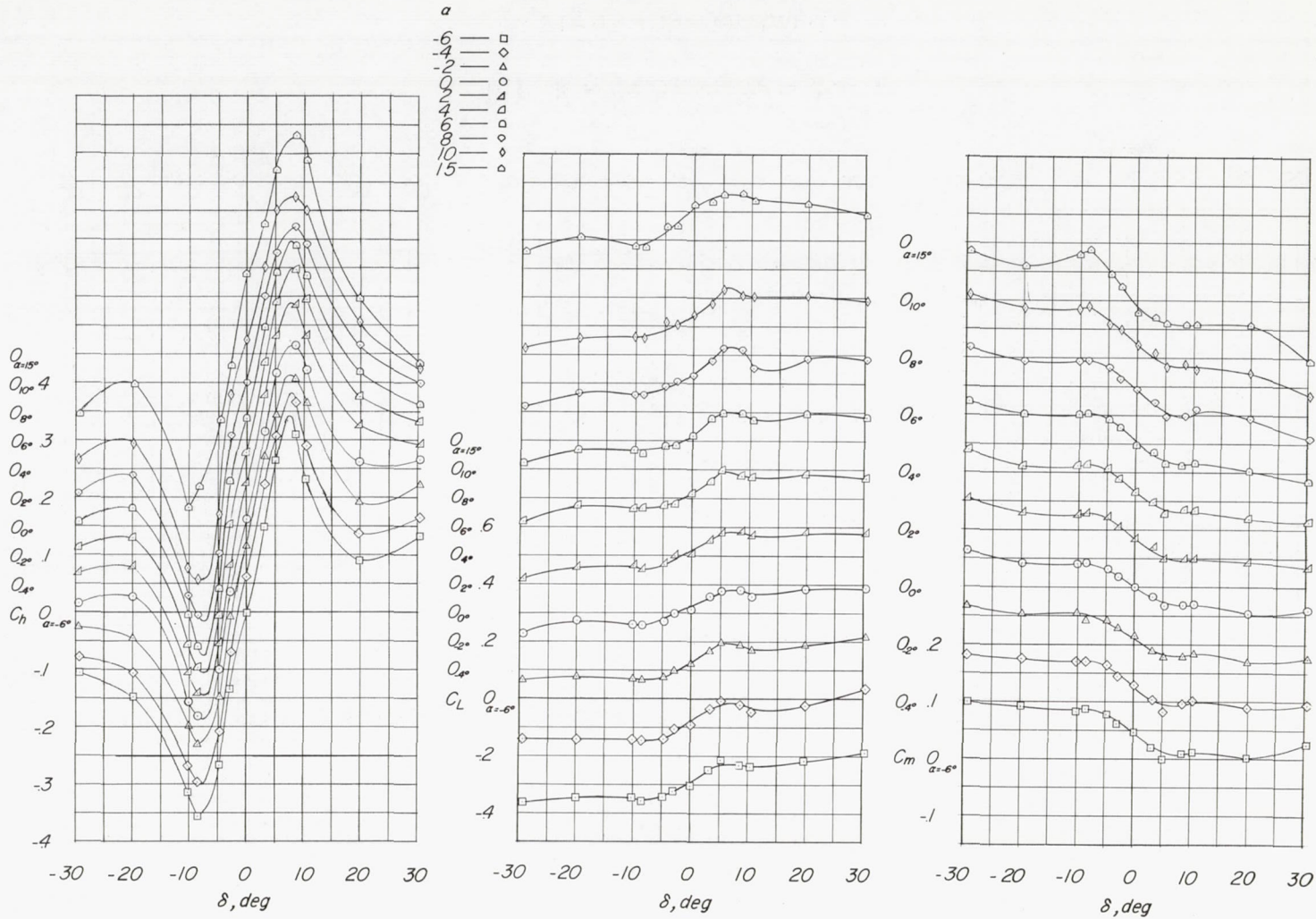
(e) M = 0.90; c_b/c_f = 1.03.
