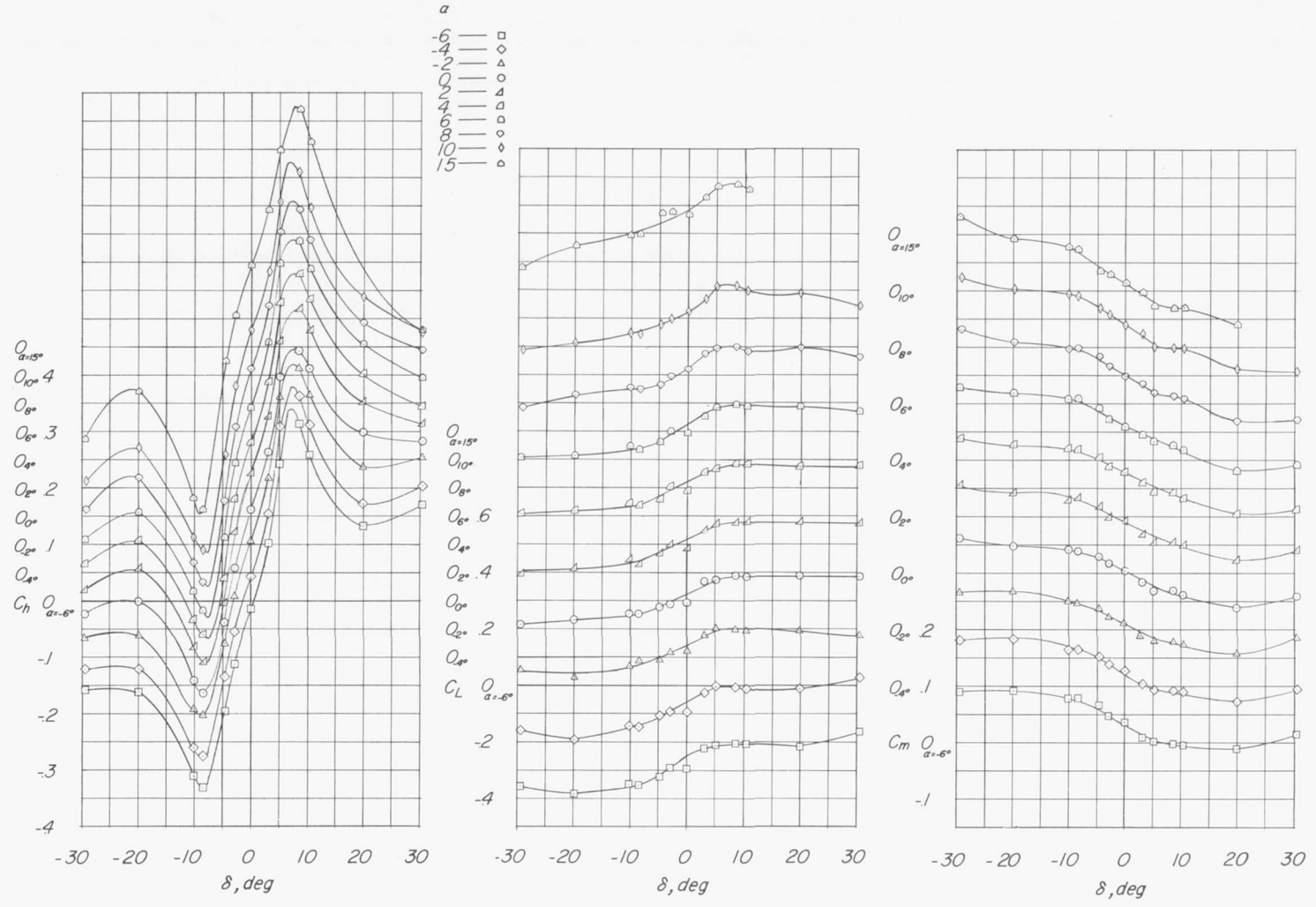
(c) M = 0.80 ; c_b/c_F = 1.03 .
