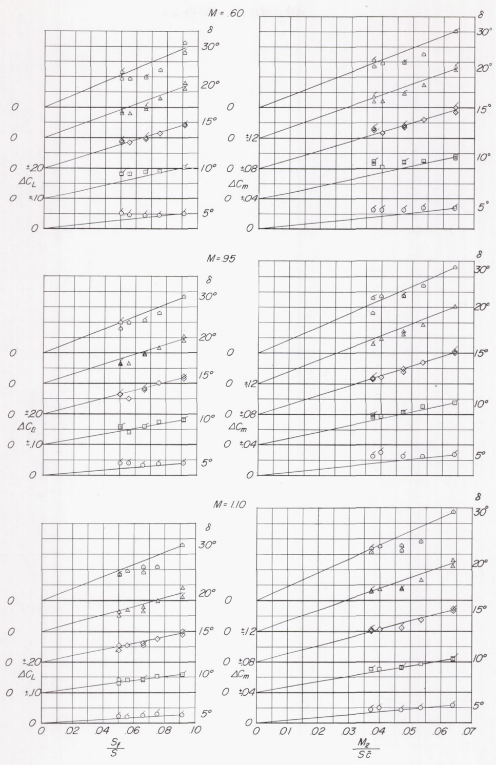
Figure 14.- Variation of \Delta C_L and \Delta C_m with a nondimensional ratio based on the area and area moment of the control area rearward of the hinge line. Flagged symbols denote negative flap deflections.
