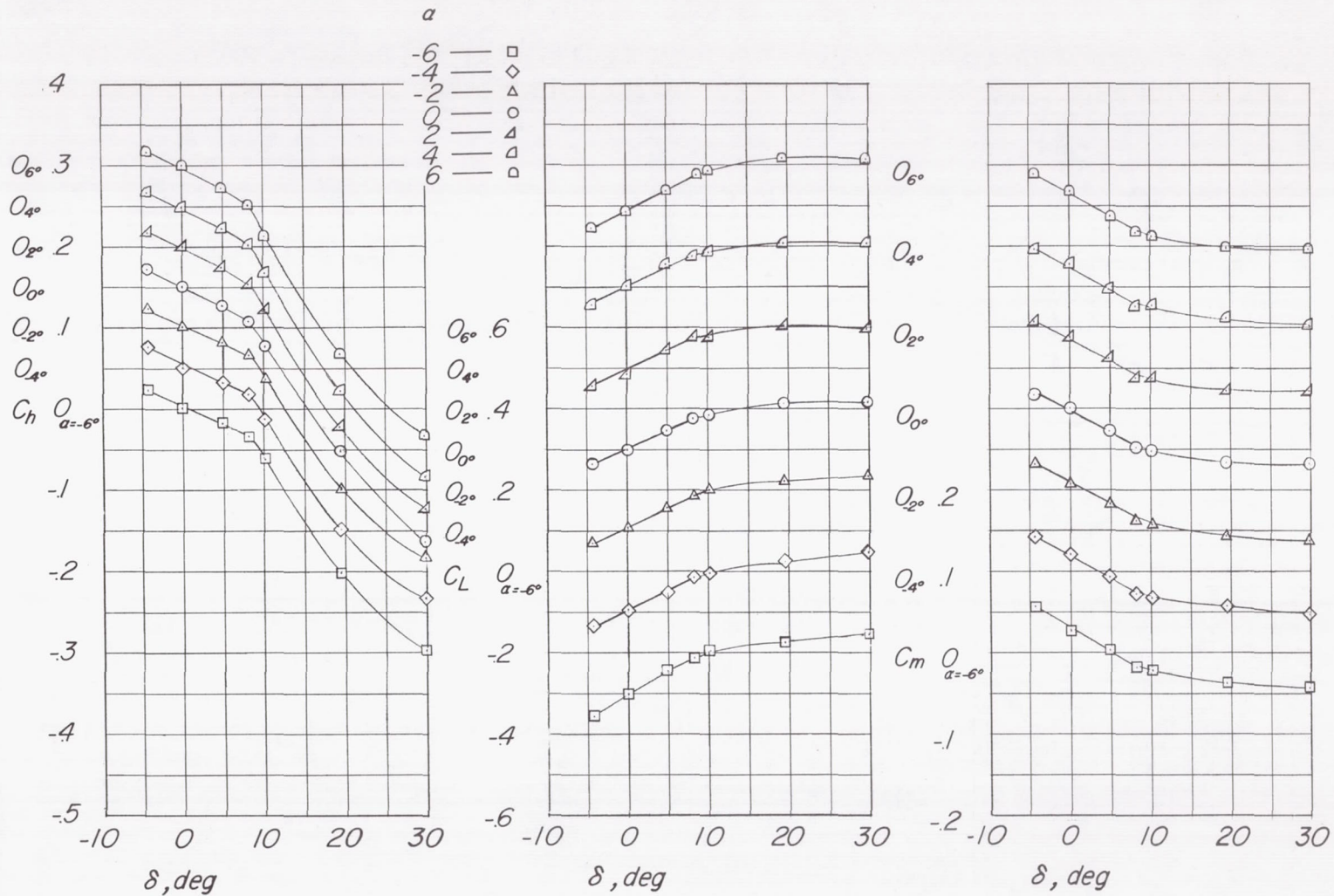
(b) M = 0.70 ; c_b/c_f = 0.32 .
