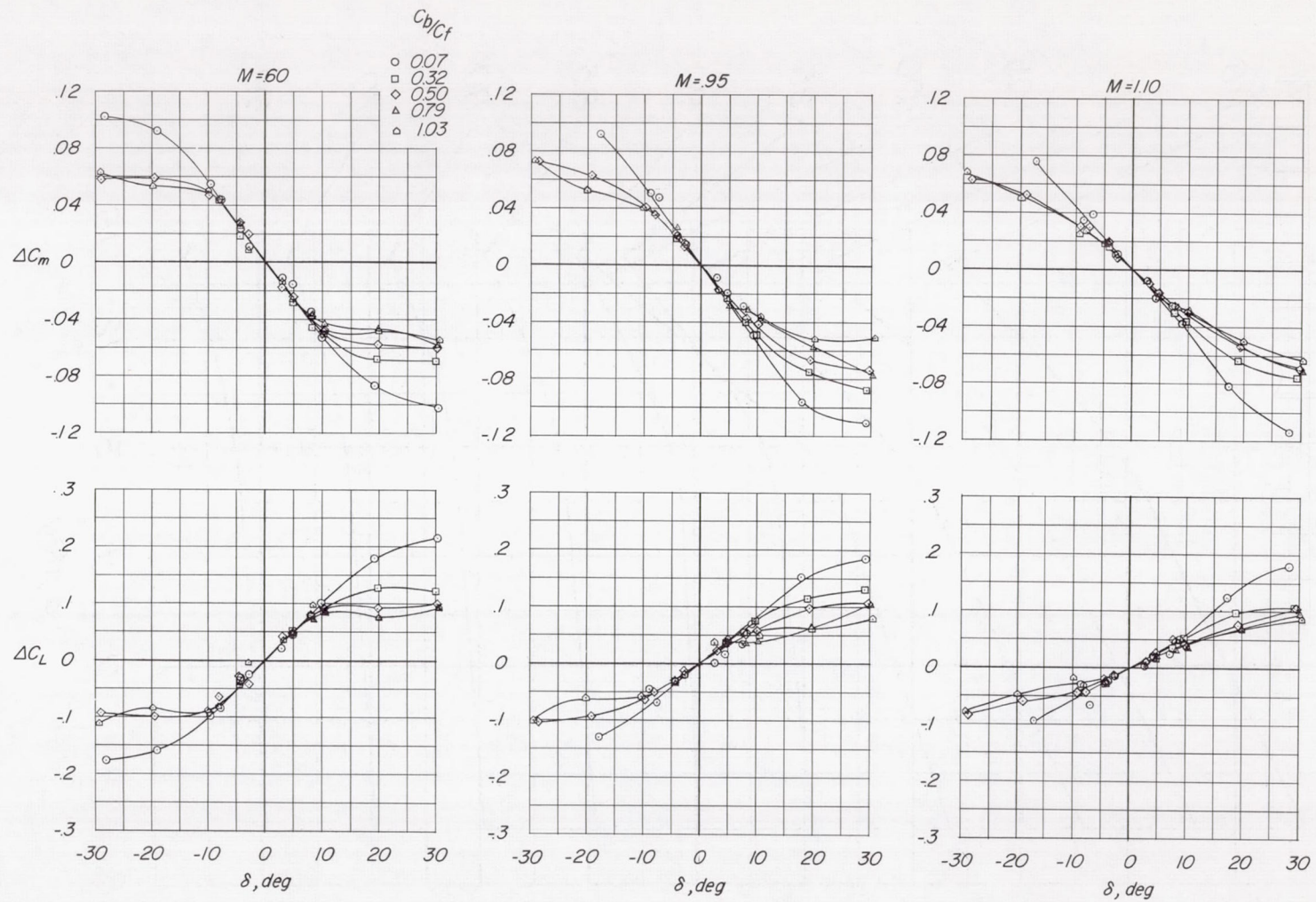
(b) \Delta C_L and \Delta C_m plotted against \delta .
