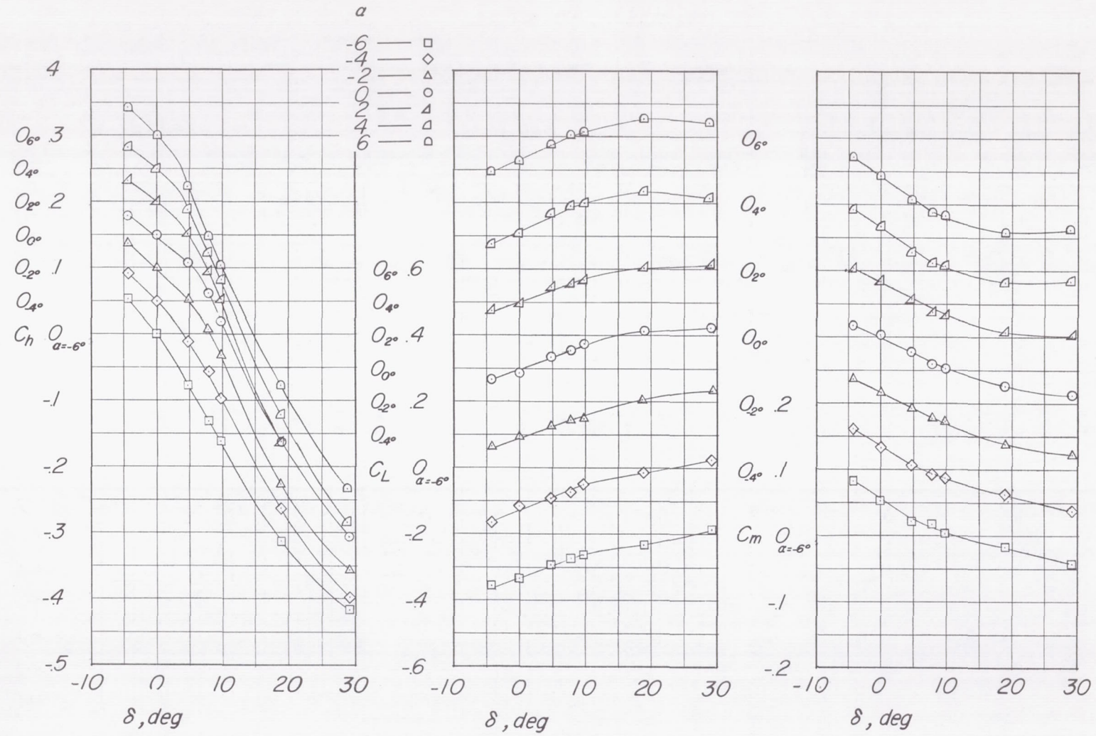
(f) M = 0.95 ; c_b/c_f = 0.32 .
