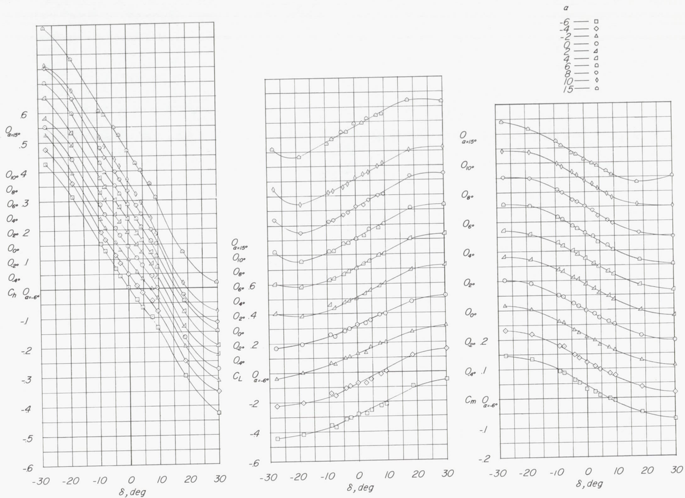
(c) M = 0.80 ; c_b/c_F = 0.07 .
