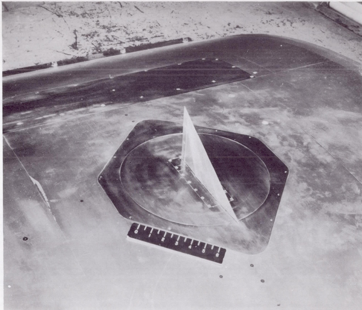
Figure 2.- Photograph of the model as mounted on the bump in the Langley high-speed 7- by 10-foot tunnel.
