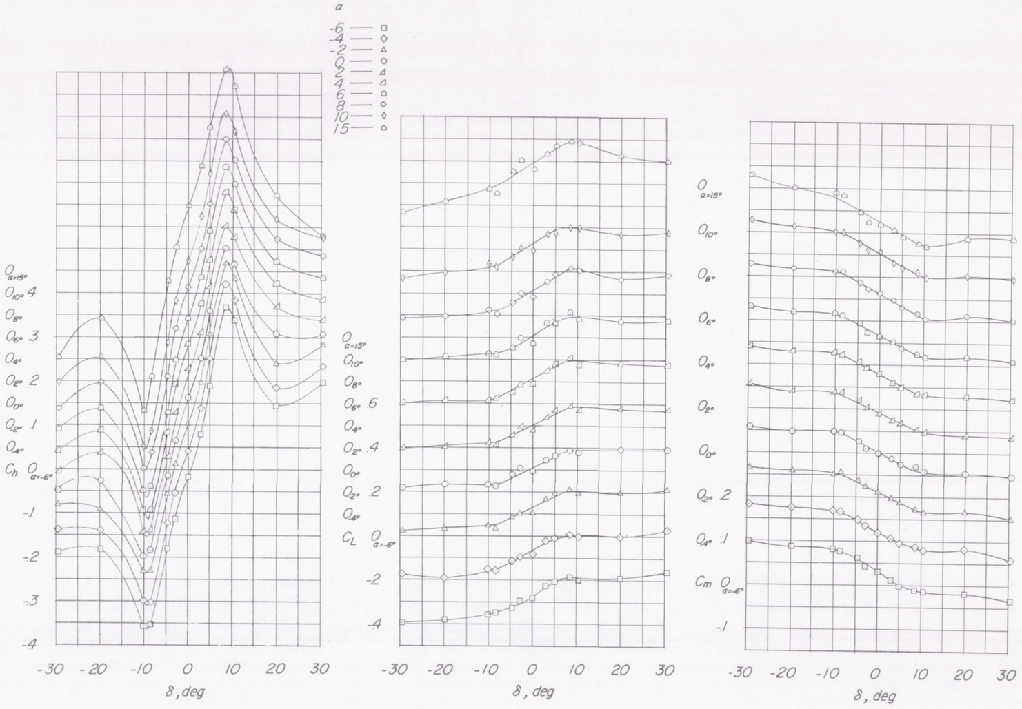
(b) M = 0.70 ; c_b/c_F = 1.03 .
