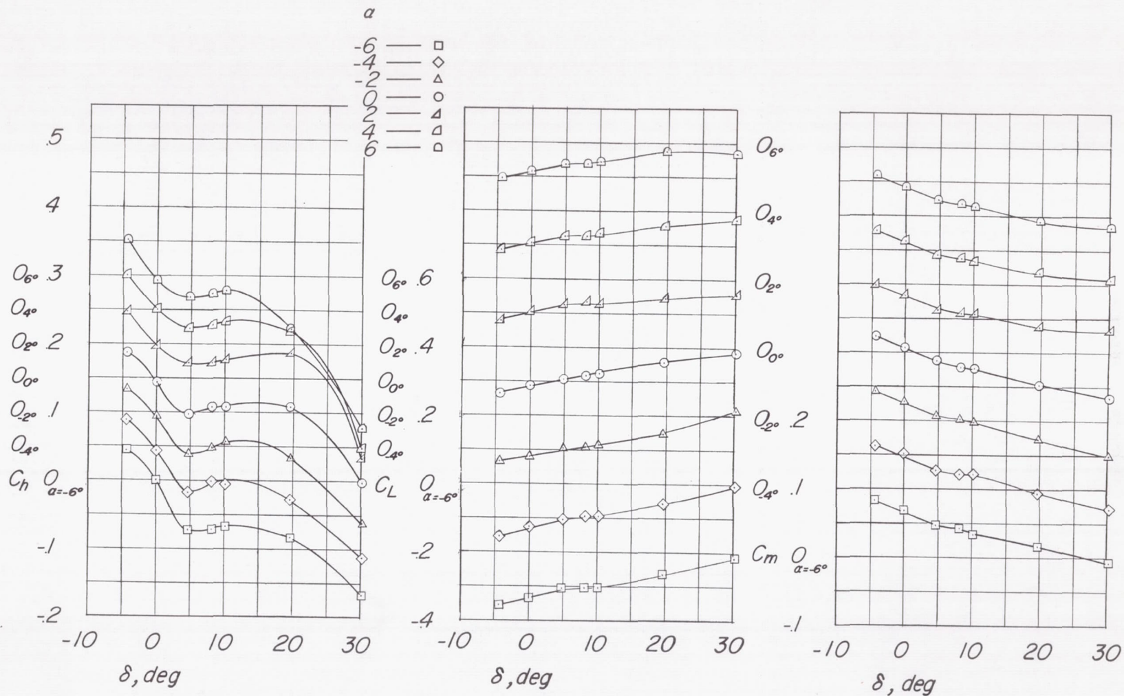
(i) M = 1.10 ; c_b/c_f = 0.79 .
