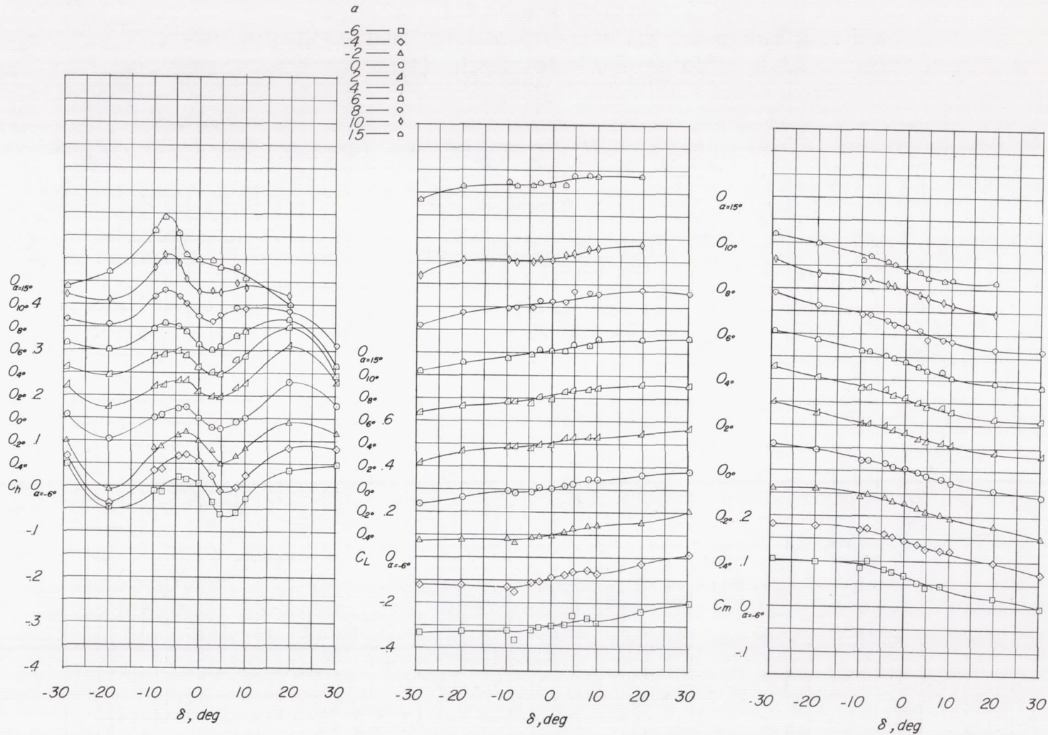
(j) M = 1.18; c_b/c_f = 1.03.
