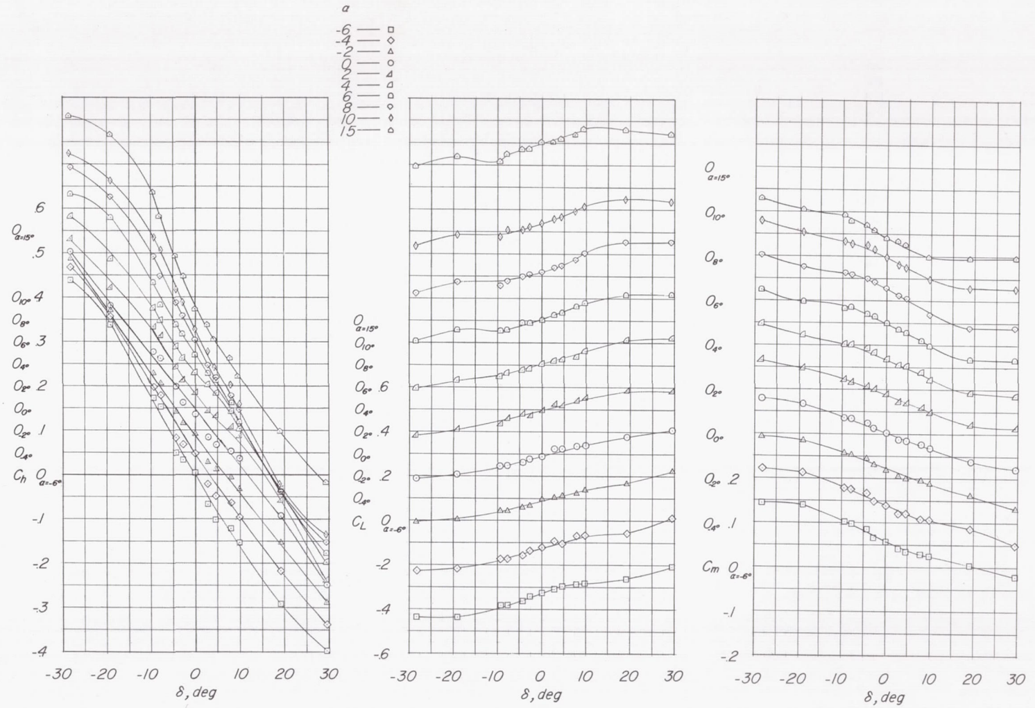
(g) M = 1.00 ; c_b/c_f = 0.50 .
