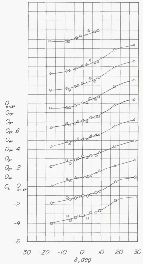
(i) M = 1.10; c_b/c_f = 0.07.
