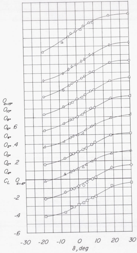
(b) M = 0.70 ; c_b/c_f = 0.07 .
