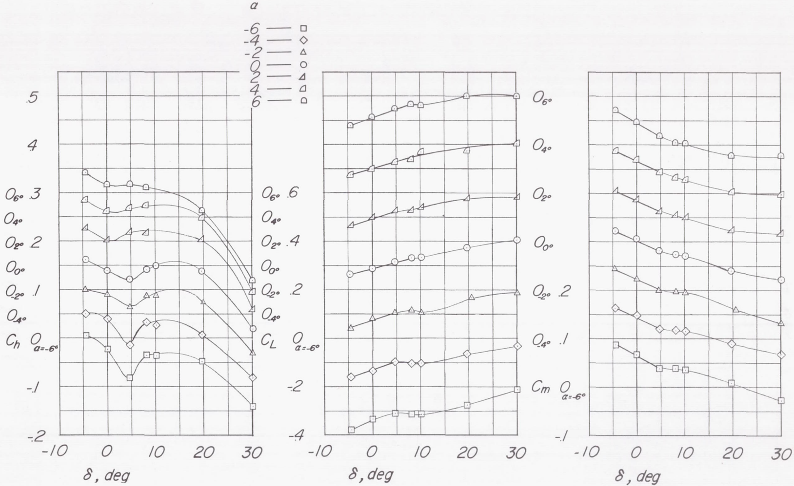
(g) M = 1.00 ; c_b/c_f = 0.79 .
