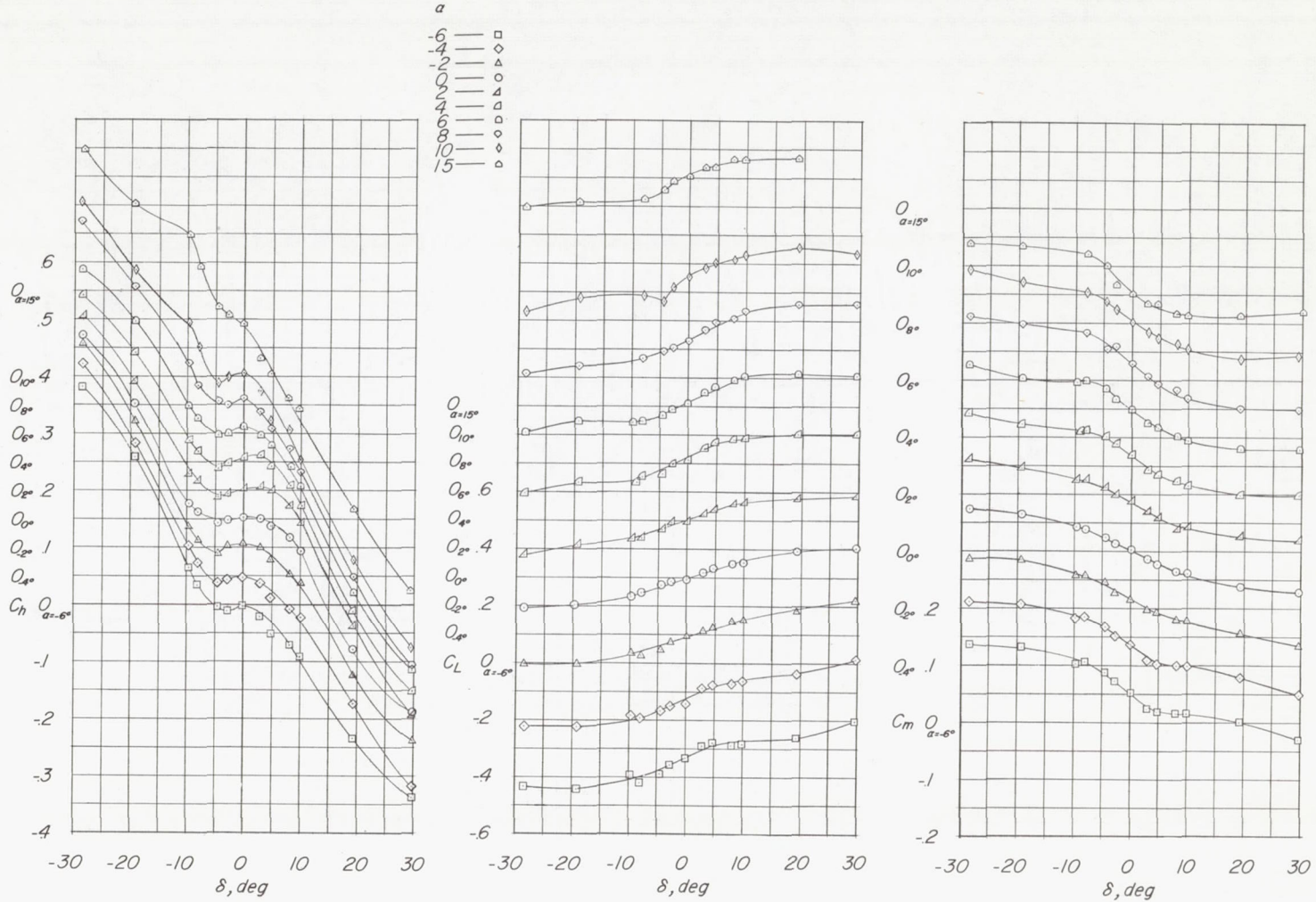
(f) M = 0.95 ; c_b/c_f = 0.50 .
