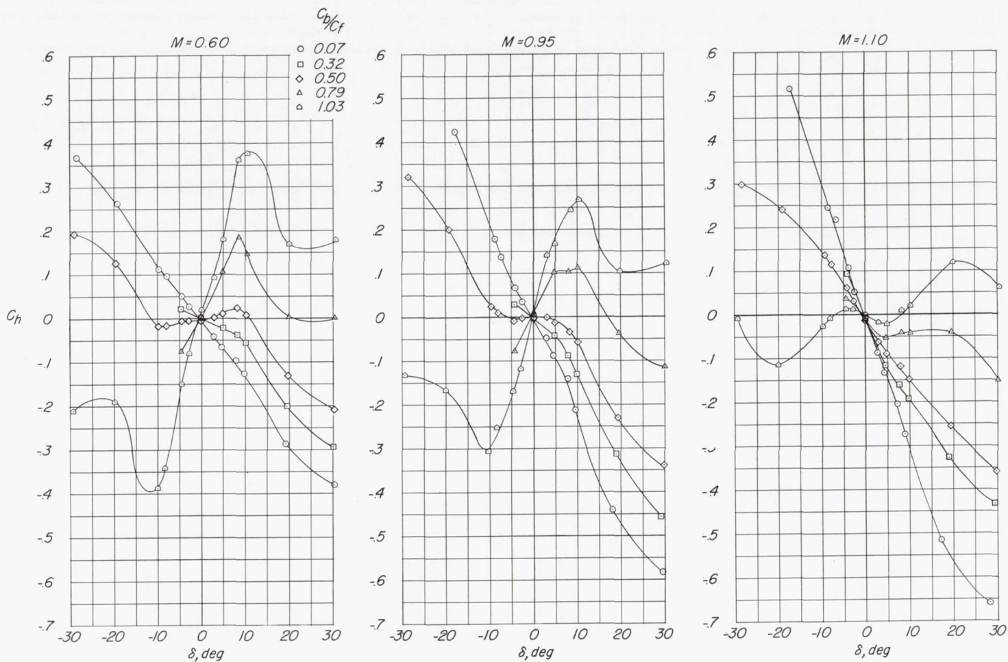
(a) C_h plotted against \delta .
