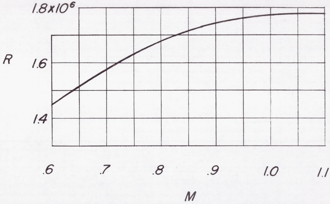
Figure 4.- Typical variation of test Reynolds number with Mach number.
