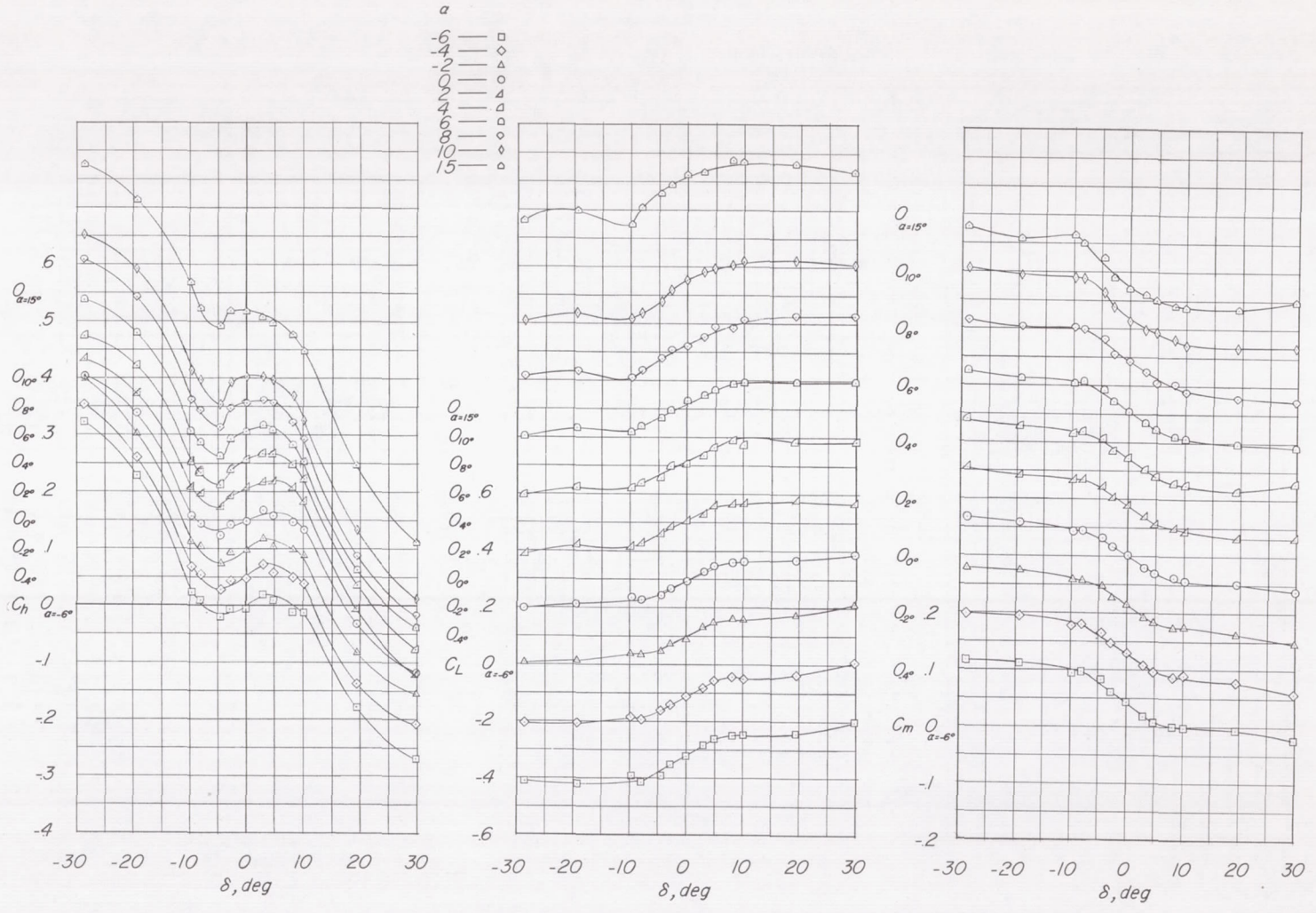
(e) M = 0.90 ; c_b/c_f = 0.50 .
