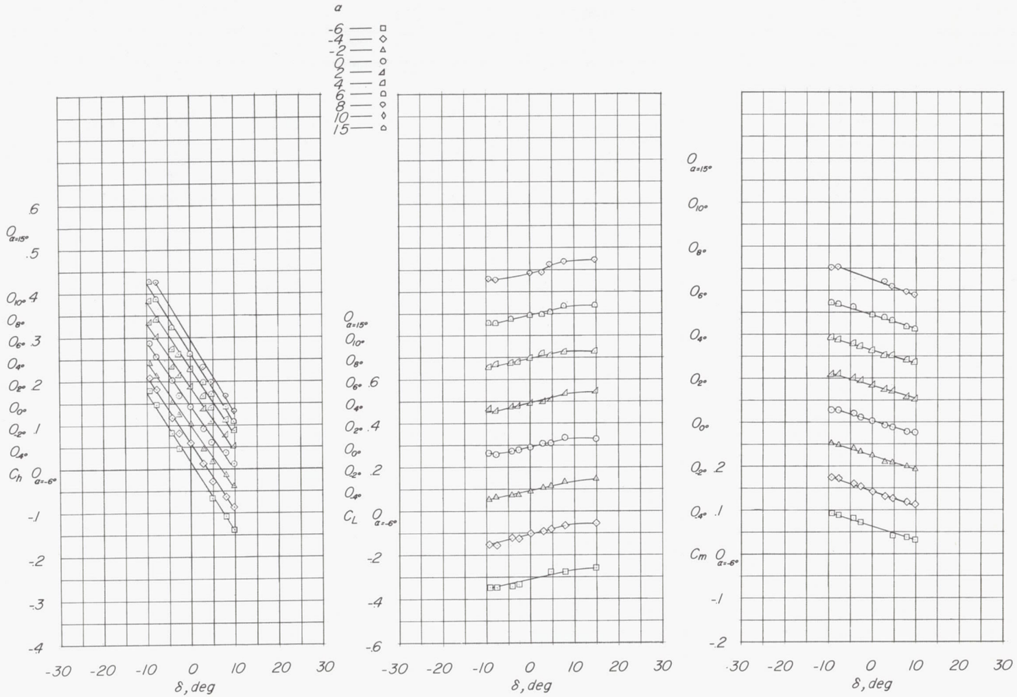
(j) M = 1.18 ; c_b/c_F = 0.50 .
