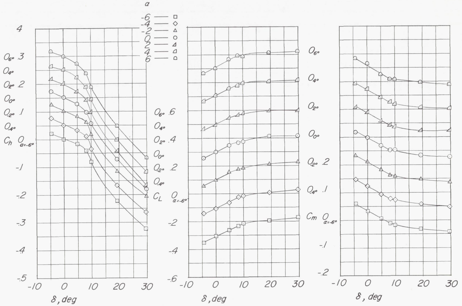
(c) M = 0.80 ; c_b/c_f = 0.32 .
