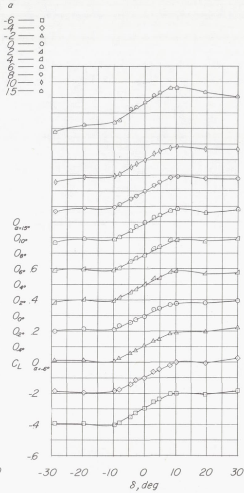
(b) M = 0.70 ; c_b/c_f = 0.50 .
