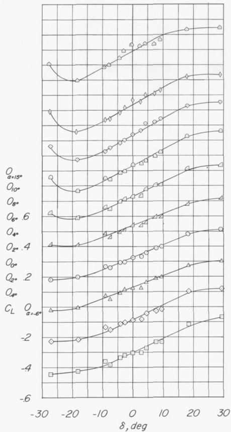
(e) M = 0.90 ; c_b/c_F = 0.07 .
