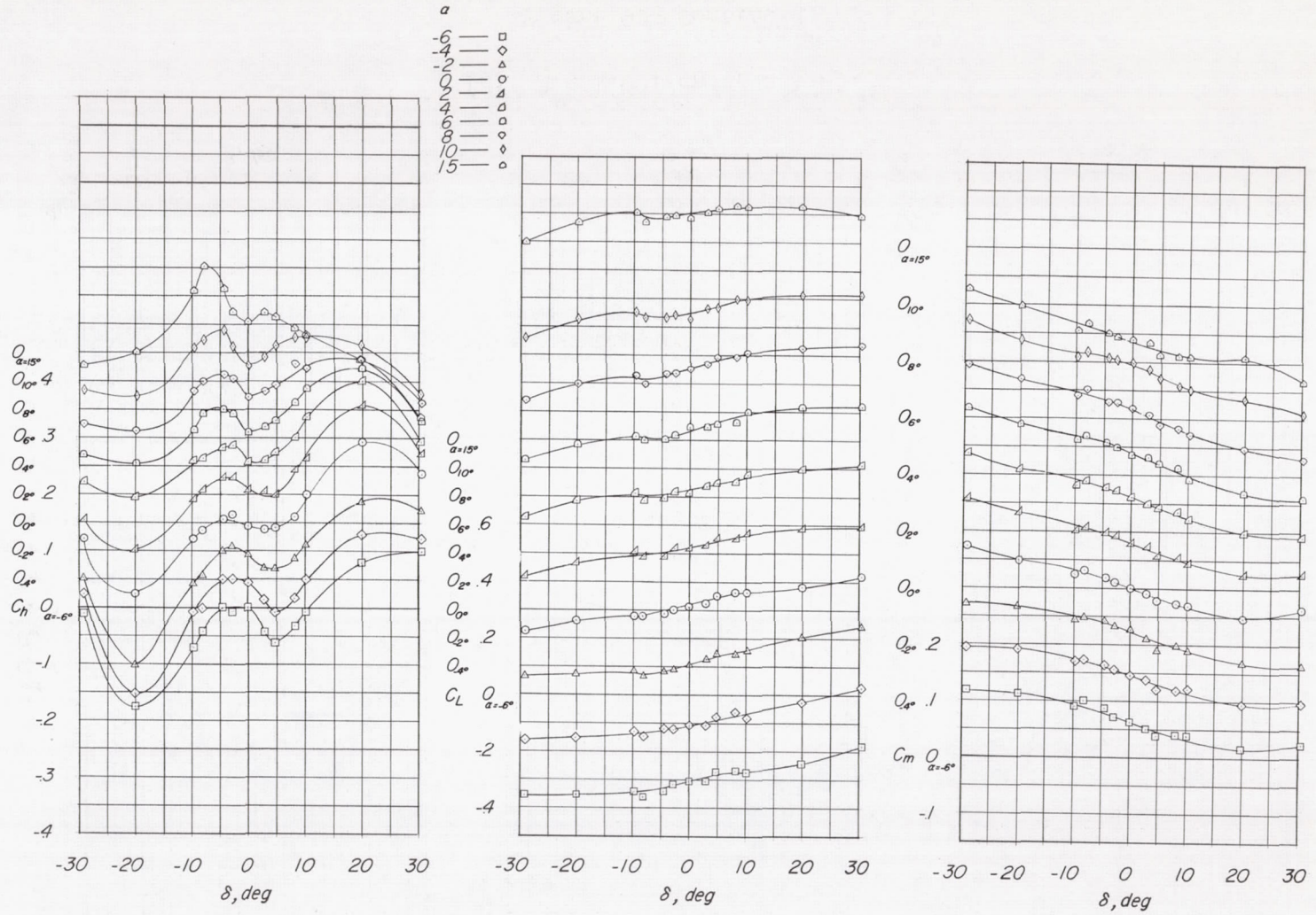
(h) M = 1.05 ; c_b/c_f = 1.03 .
