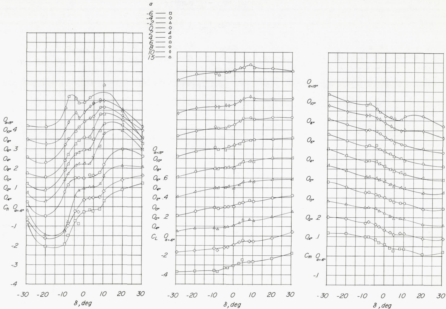
(g) M = 1.00 ; c_b/c_f = 1.03 .
