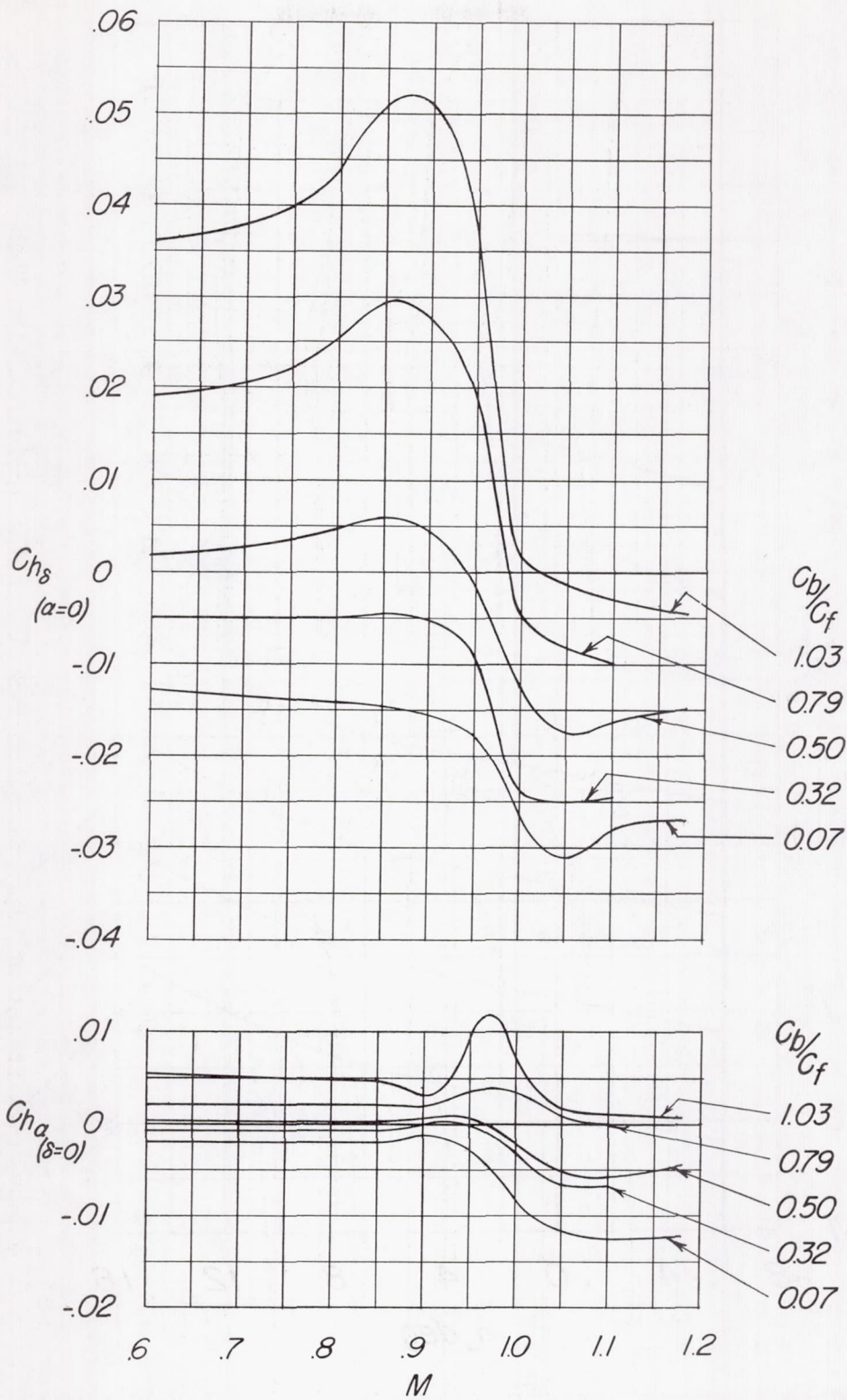
Figure 12.- Effect of hinge location on the variation with Mach number of the hinge-moment parameters C_{h\delta} and C_{h\alpha} .
