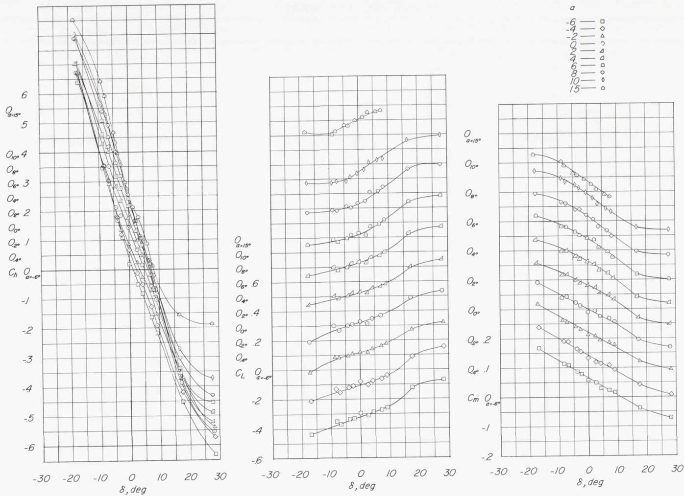
(g) M = 1.00 ; c_p/c_F = 0.07 .
