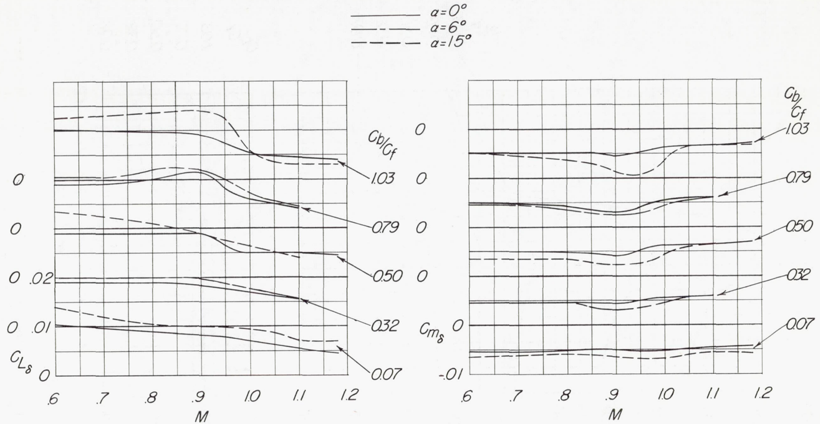
Figure 13.- Effect of hinge location and \alpha on the variation with Mach number of C_{L\delta} and C_{m\delta} .
