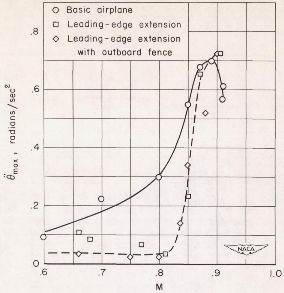
Figure 12.- Maximum pitching acceleration during stick-fixed pitch-ups.
