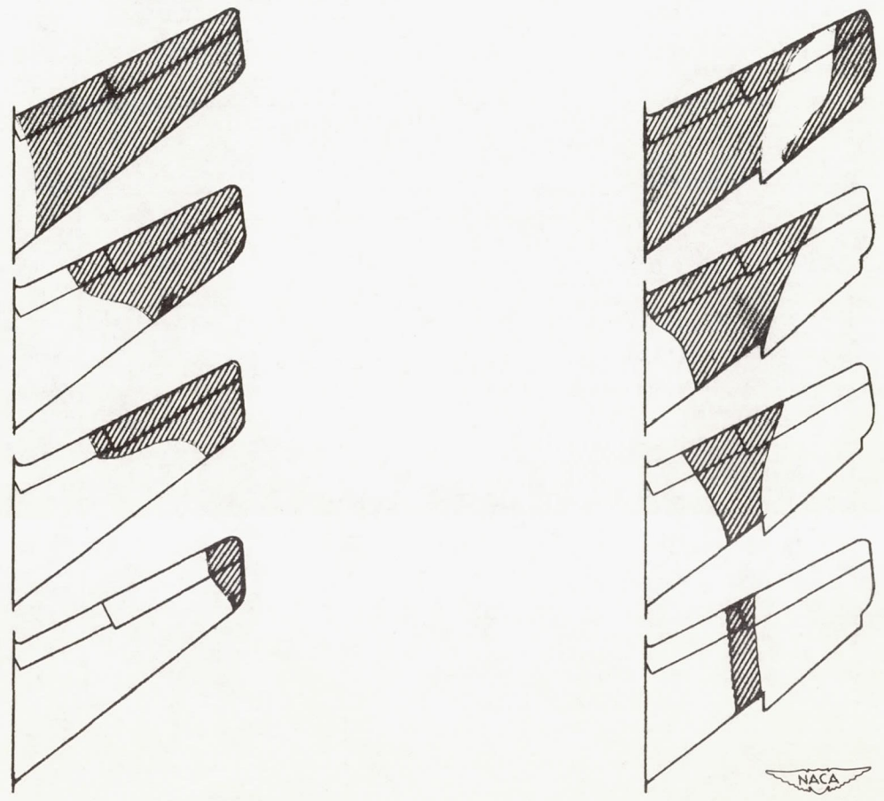
(a) Unmodified wing.
