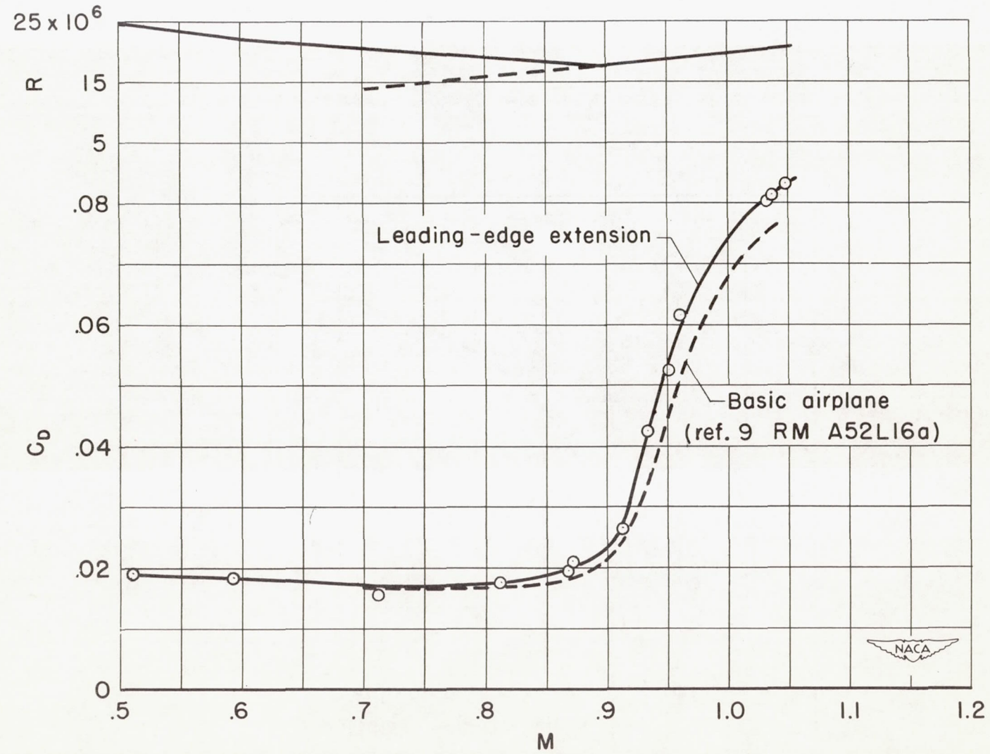
Figure 13.- Variation of drag coefficient with Mach number for C N = 0.15.
