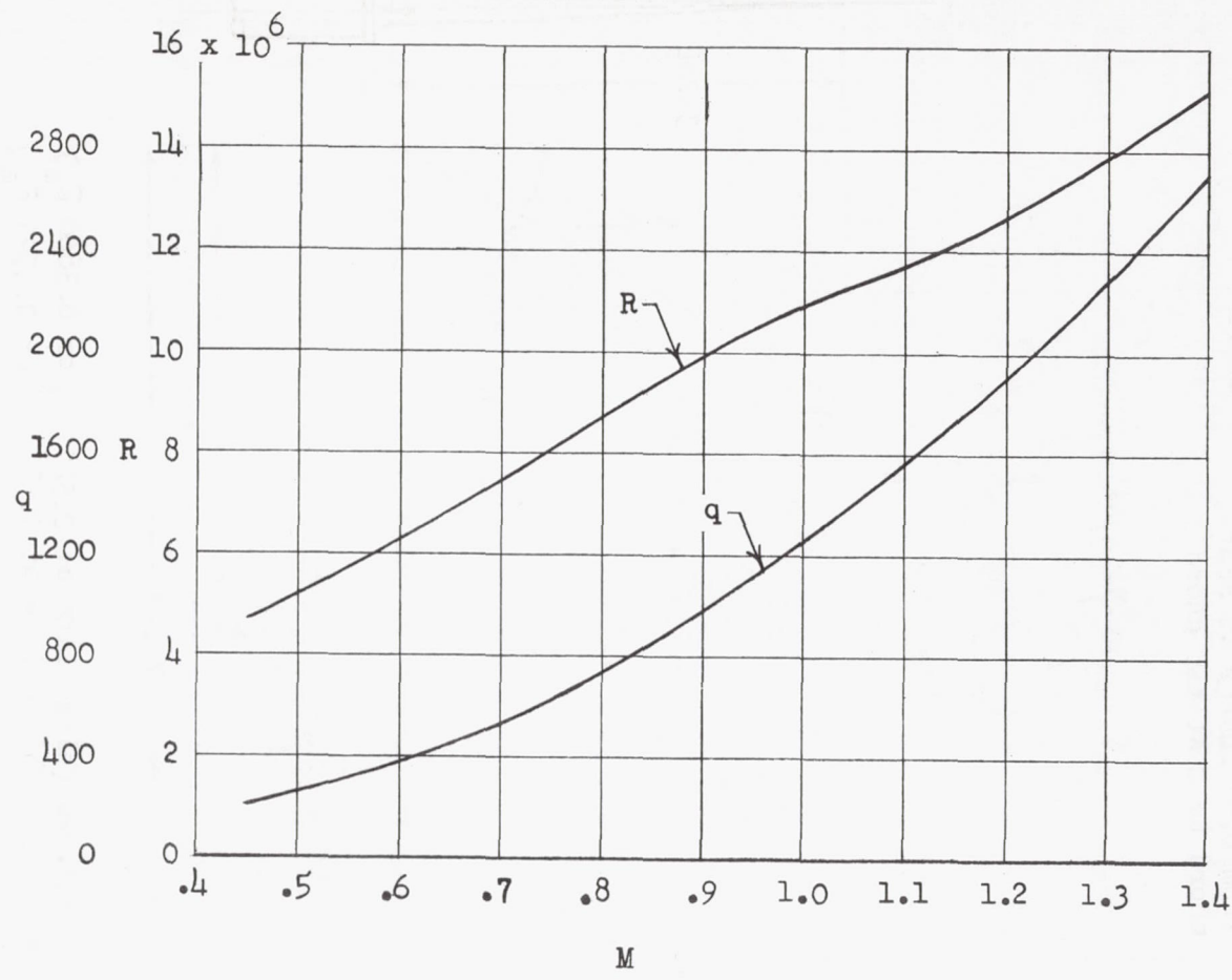
Figure 4.- Variation of Reynolds number and dynamic pressure with Mach number. Reynolds number is based on wing mean aerodynamic chord.
