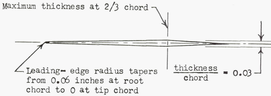
Section AA
