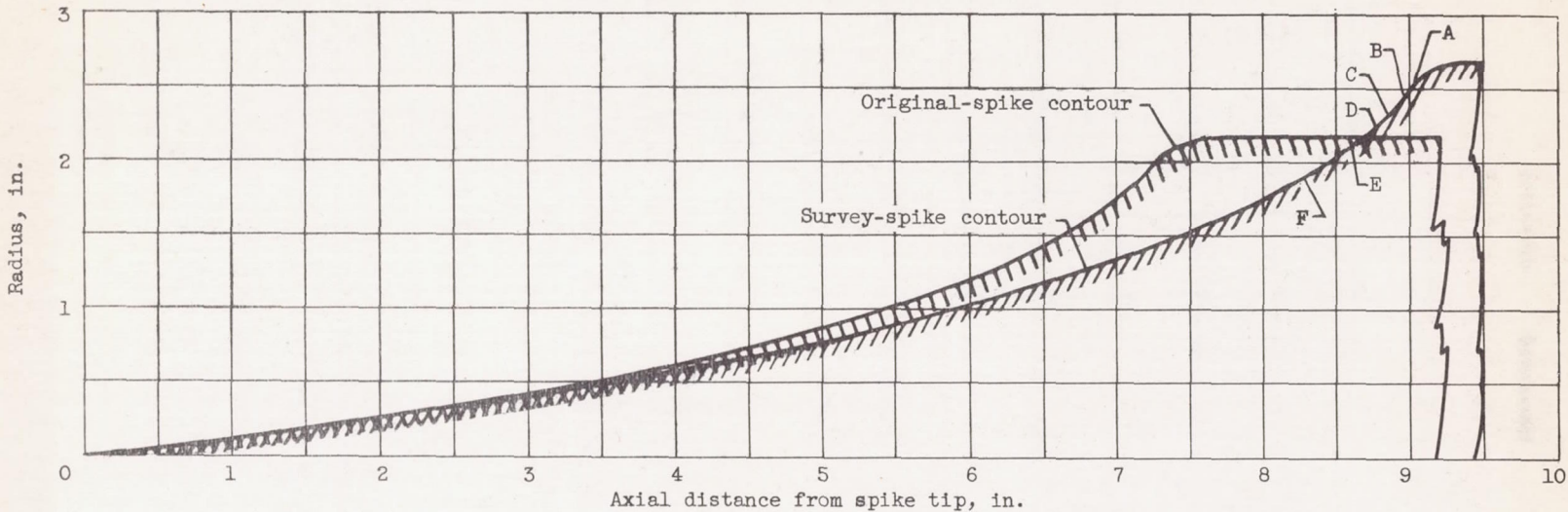
(d) Scale variation between original and survey spikes.
