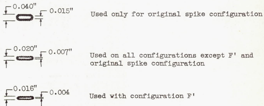
(c) Pitot-probe tip dimensions.
