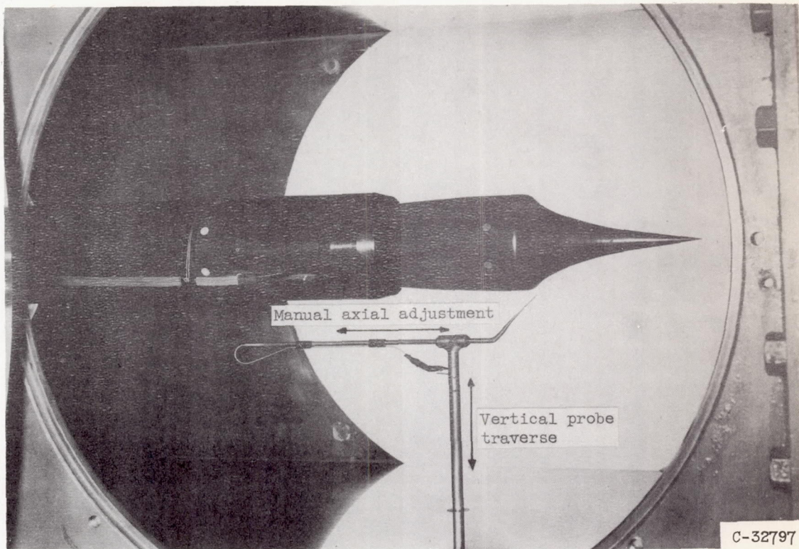
(b) Isentropic spike and pitot-probe survey mechanism in tunnel test section.
