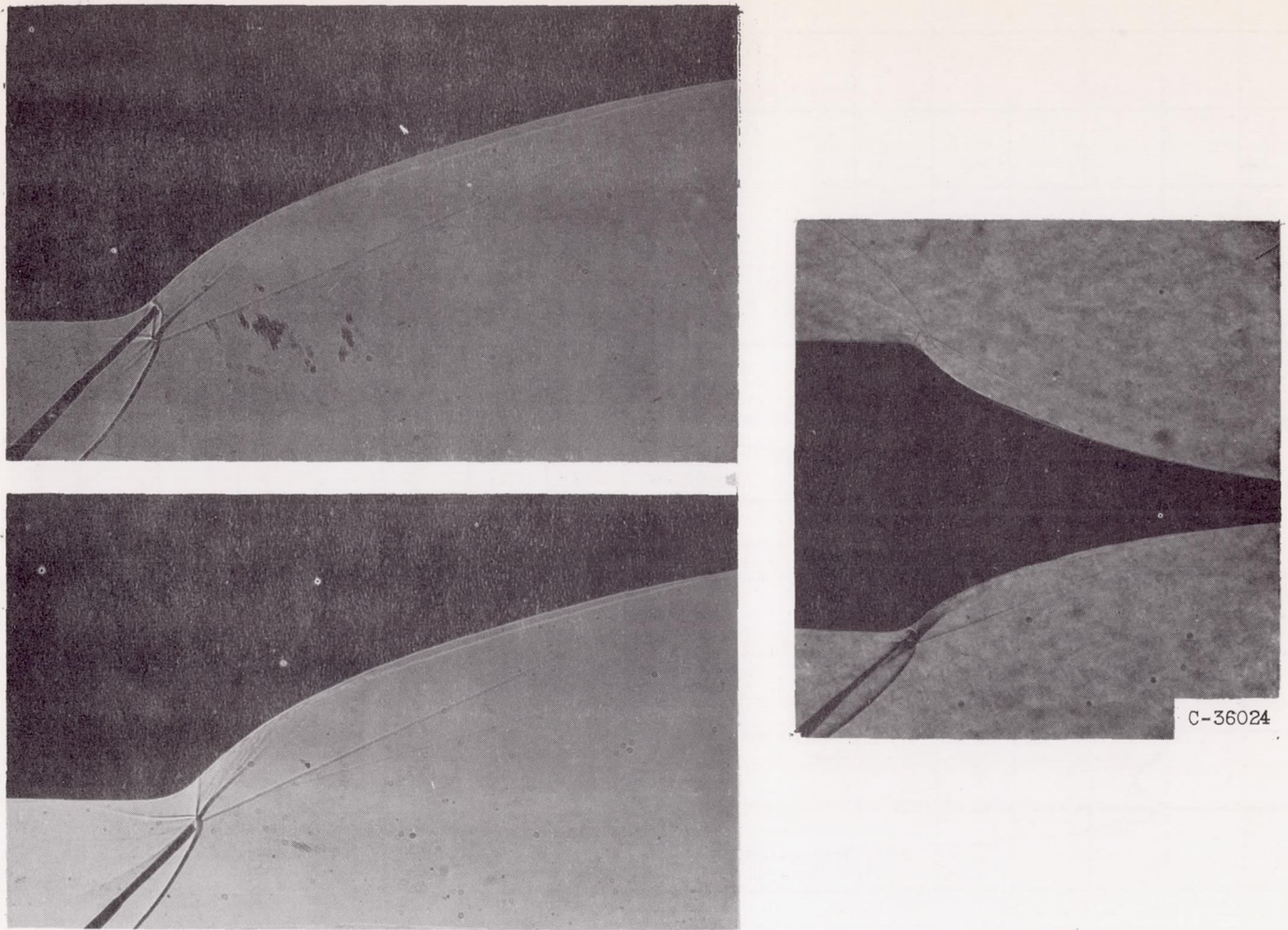
Figure 5. - Typical photographs showing probe in flow field of original isentropic spike.
