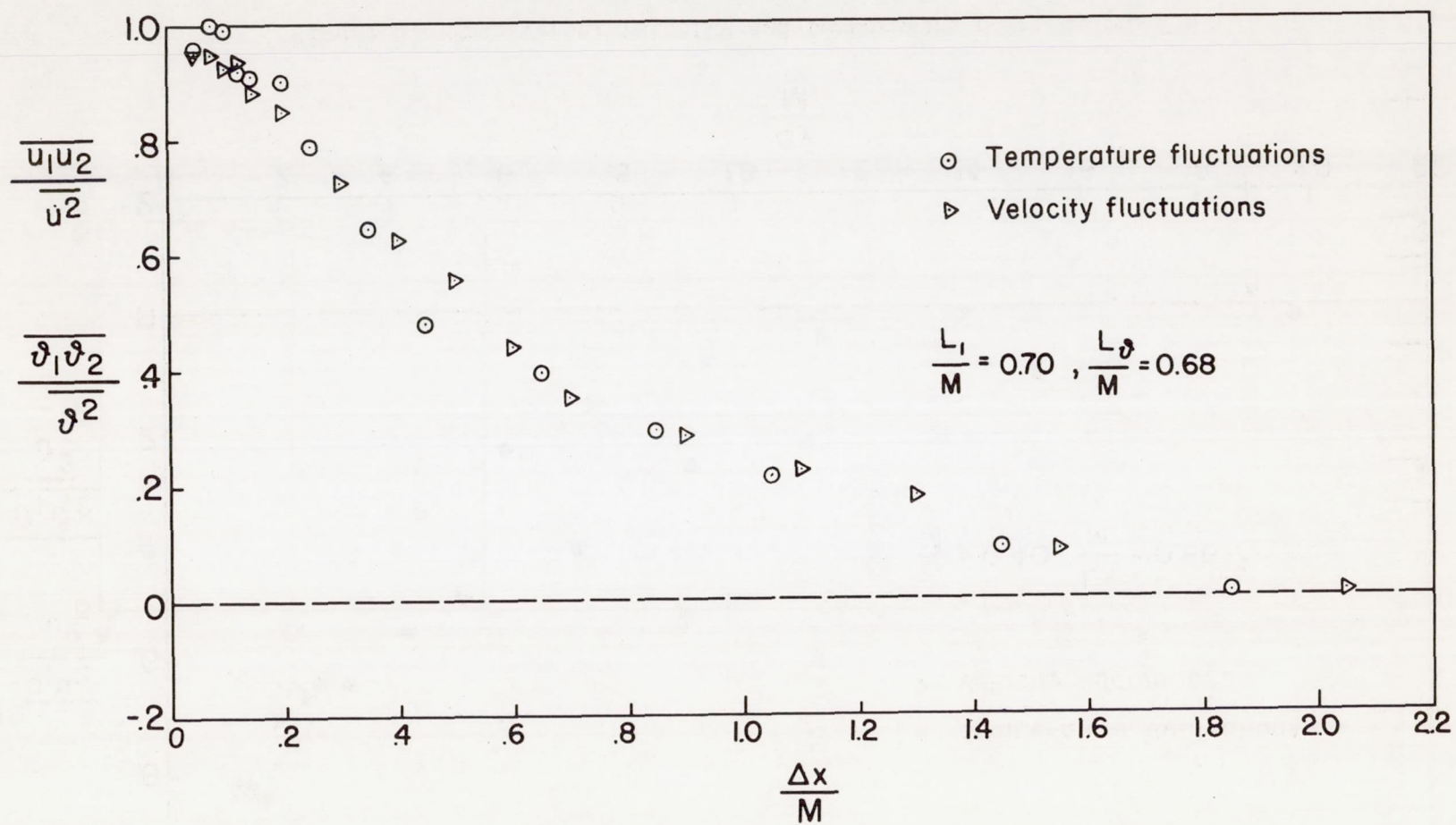
Figure 7.- Longitudinal velocity and temperature correlations.
