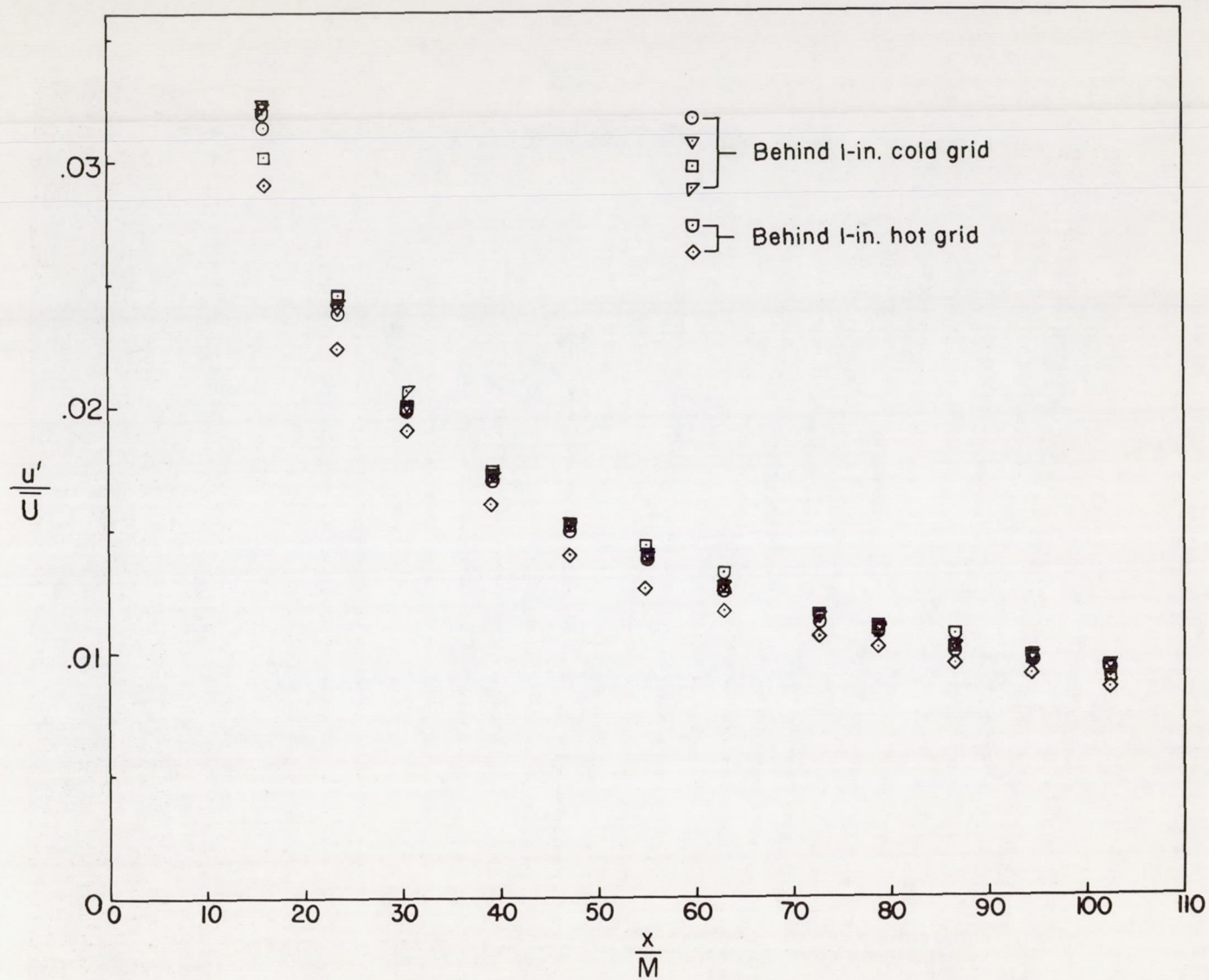
Figure 3.- Turbulence decay.
