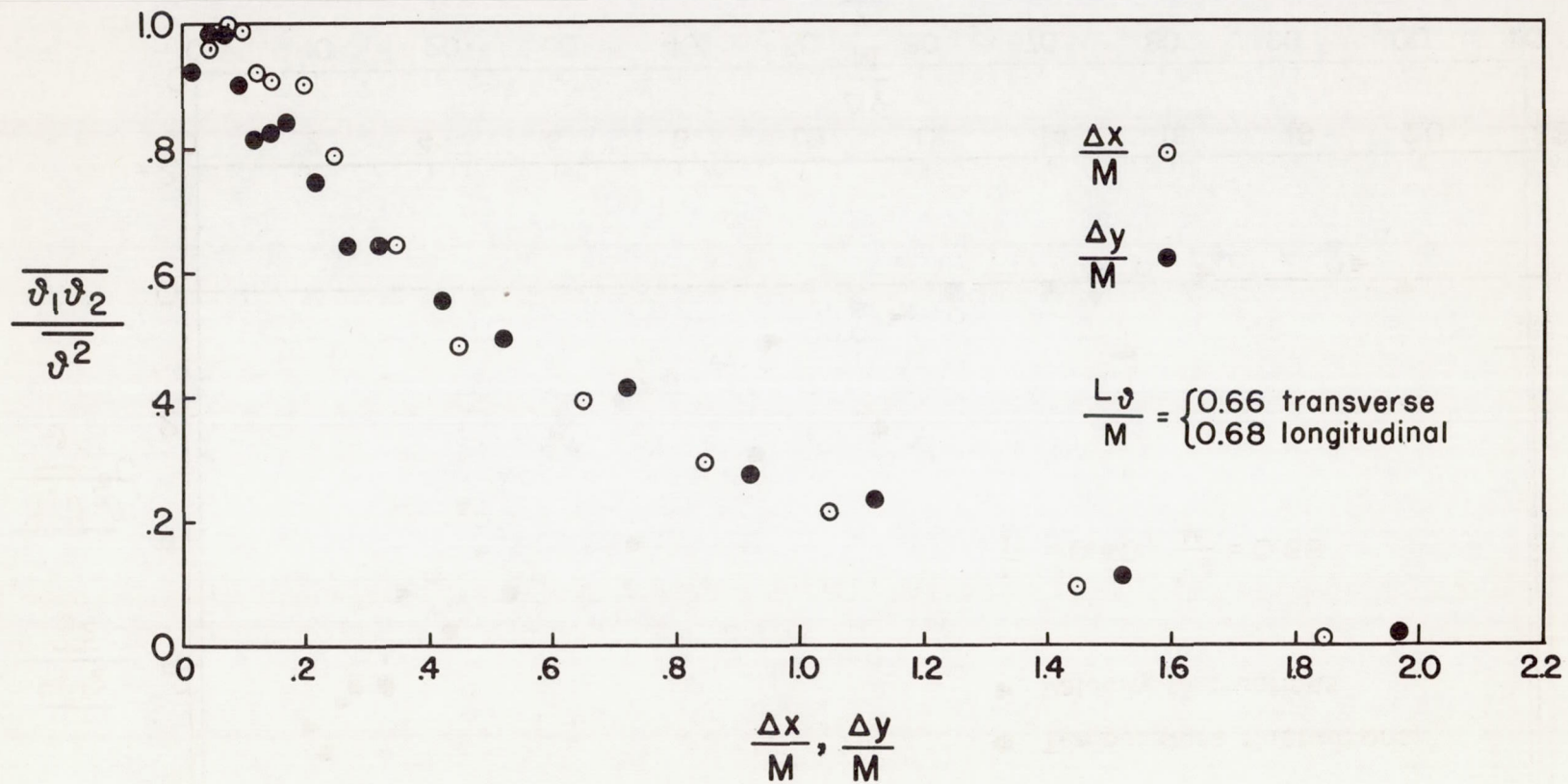
Figure 5.- Longitudinal and transversal temperature correlations.
