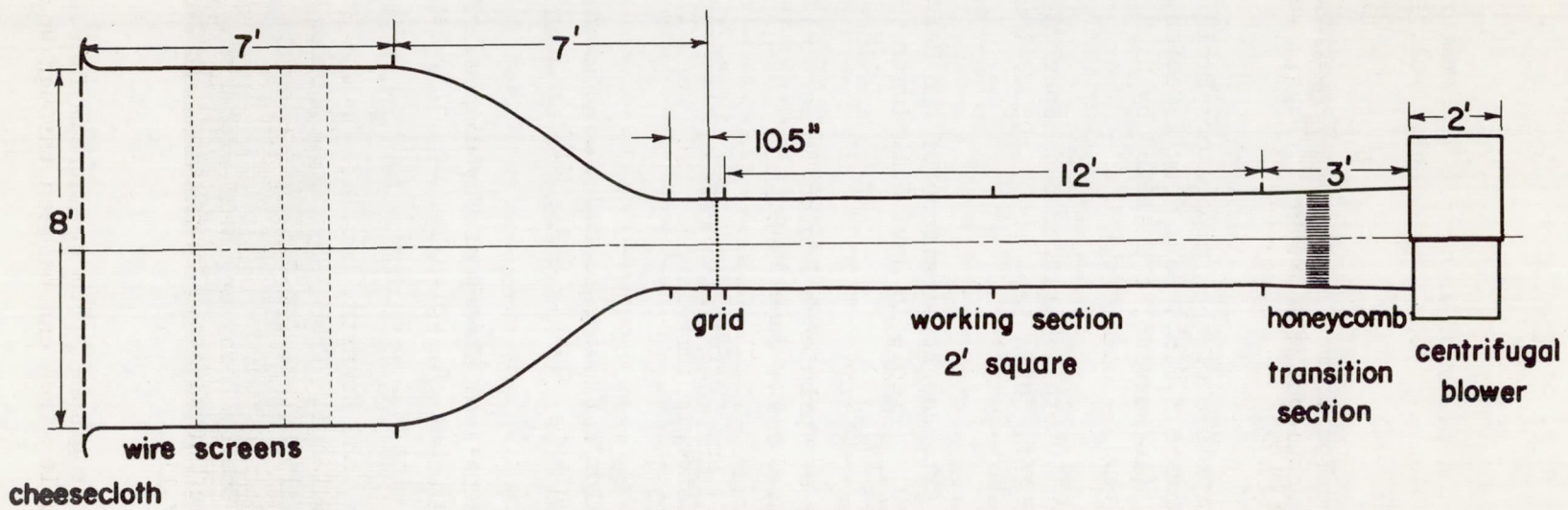
Figure 1.- Sketch of wind tunnel.
