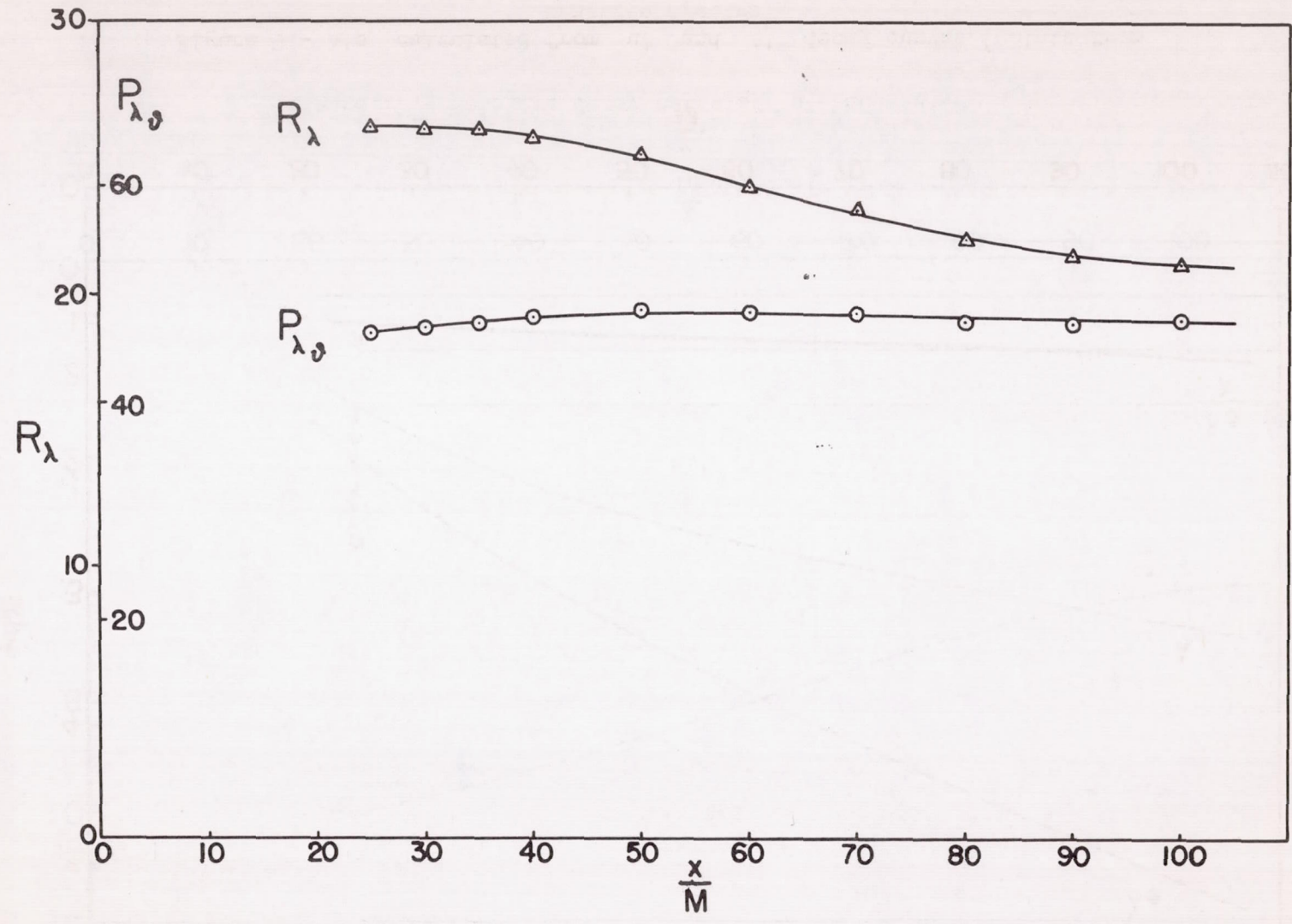
Figure 10.- Reynolds and Peclet numbers.
