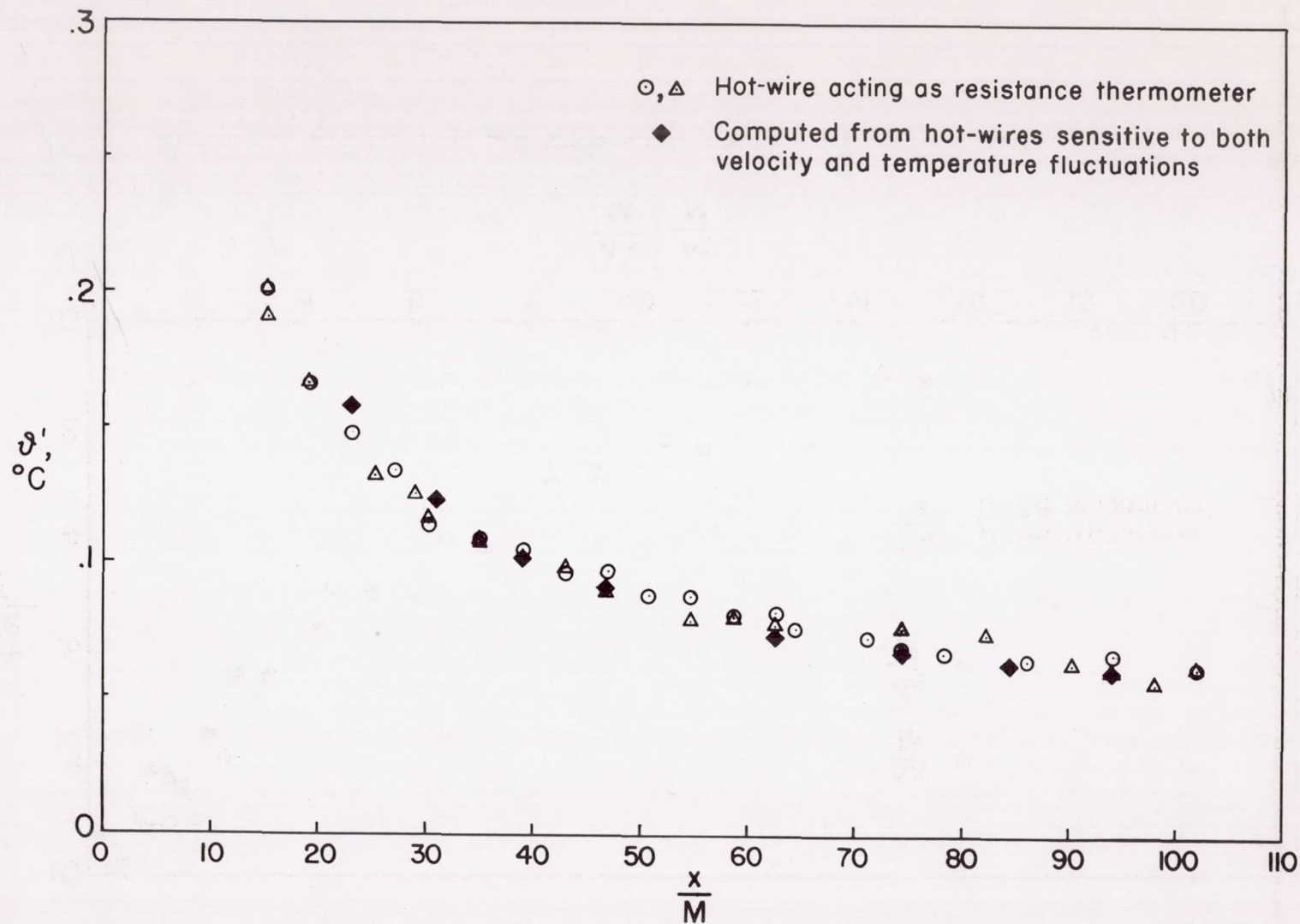
Figure 4.- Temperature fluctuation decay.
