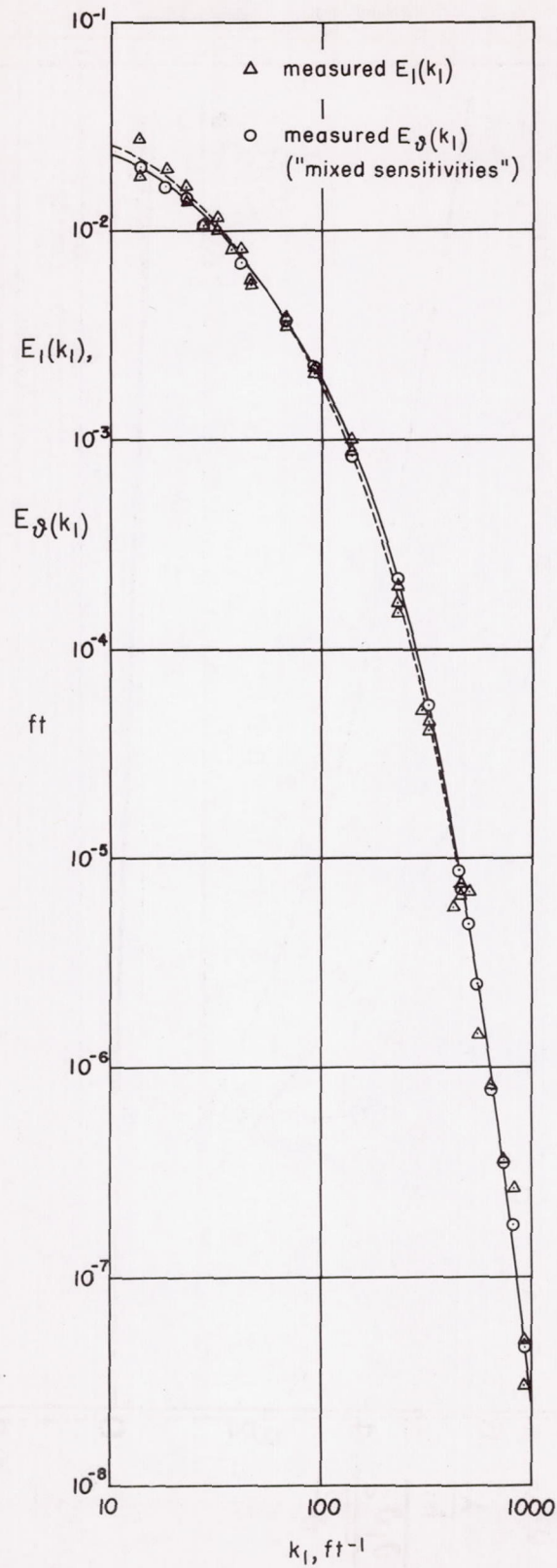
Figure 8.- u and \delta spectra at x/M = 23.1 .
