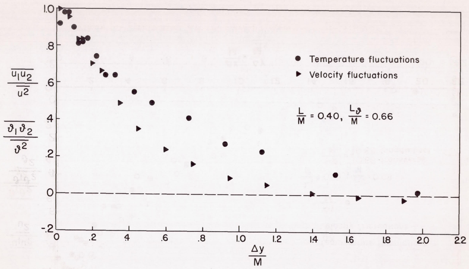
Figure 6.- Transversal velocity and temperature correlations.
