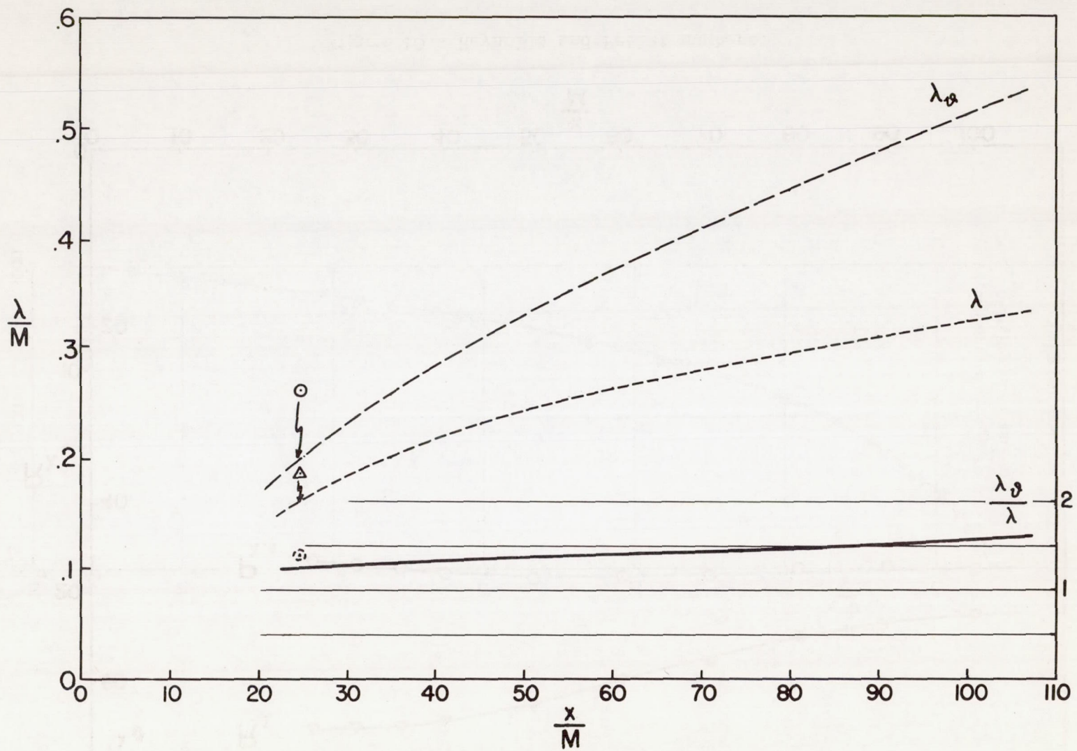
Figure 9.- \lambda 's calculated from u' and \vartheta' decay curves (points from measured spectra).
