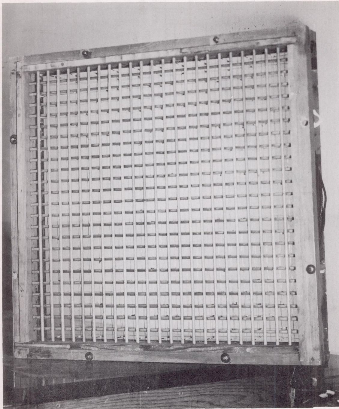
L-83689 Figure 2.- Hot grid photographed from downstream face. Parts of square heating mesh of double wires can be seen through wooden dowel grid.
