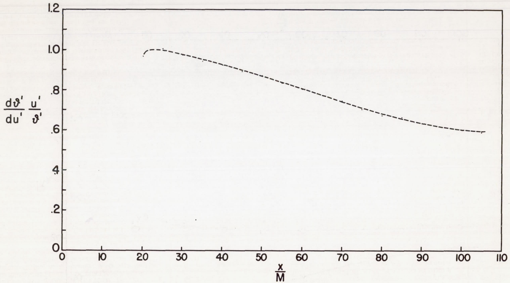
Figure 11.- Relative decay rates of u' and v' .
